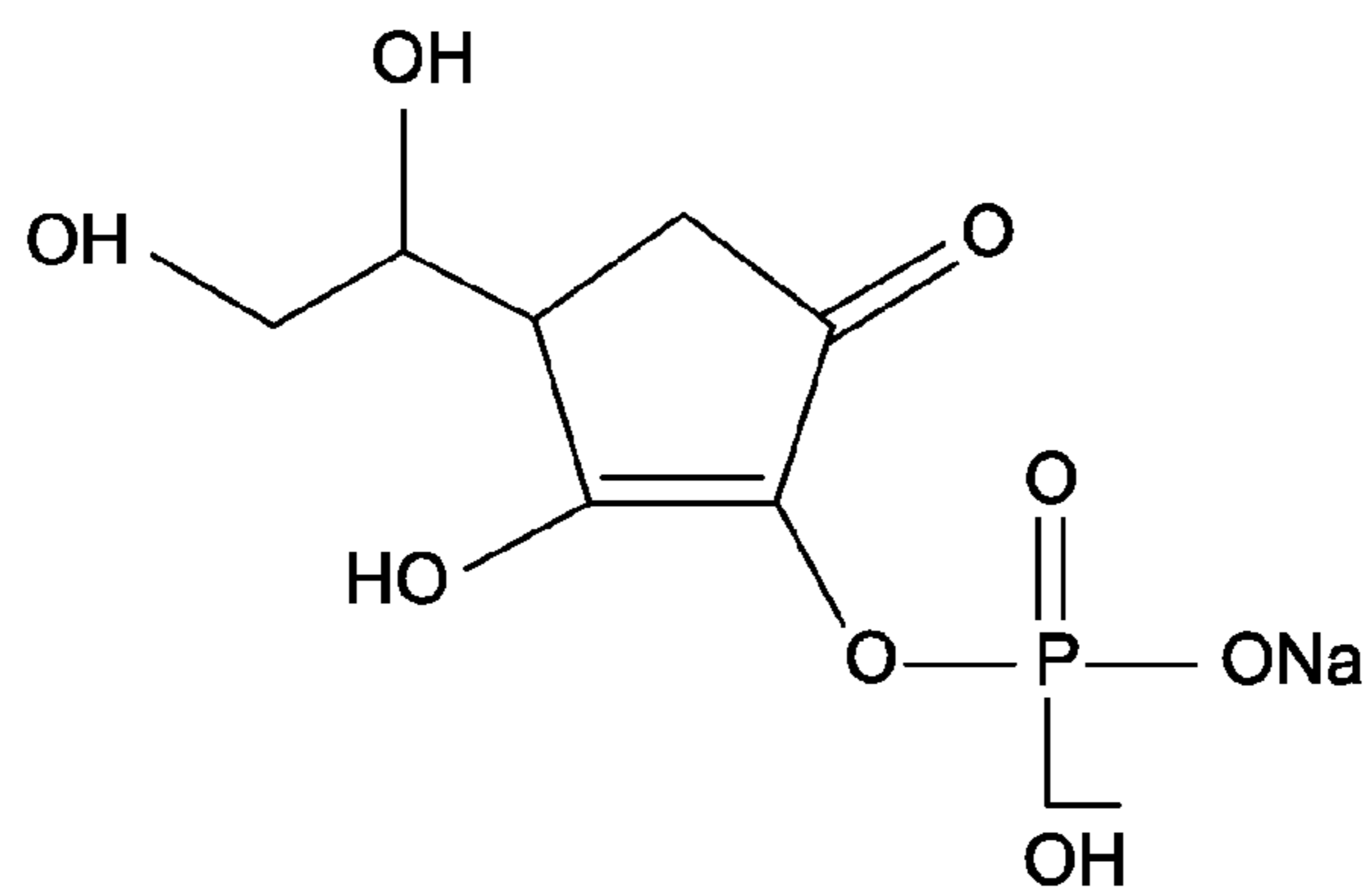
AA2P, sodium ascorbyl phosphate
