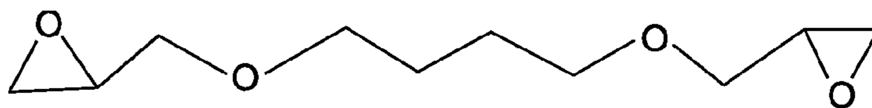
BDDE, 1,4-butanediol diglycidal ether
