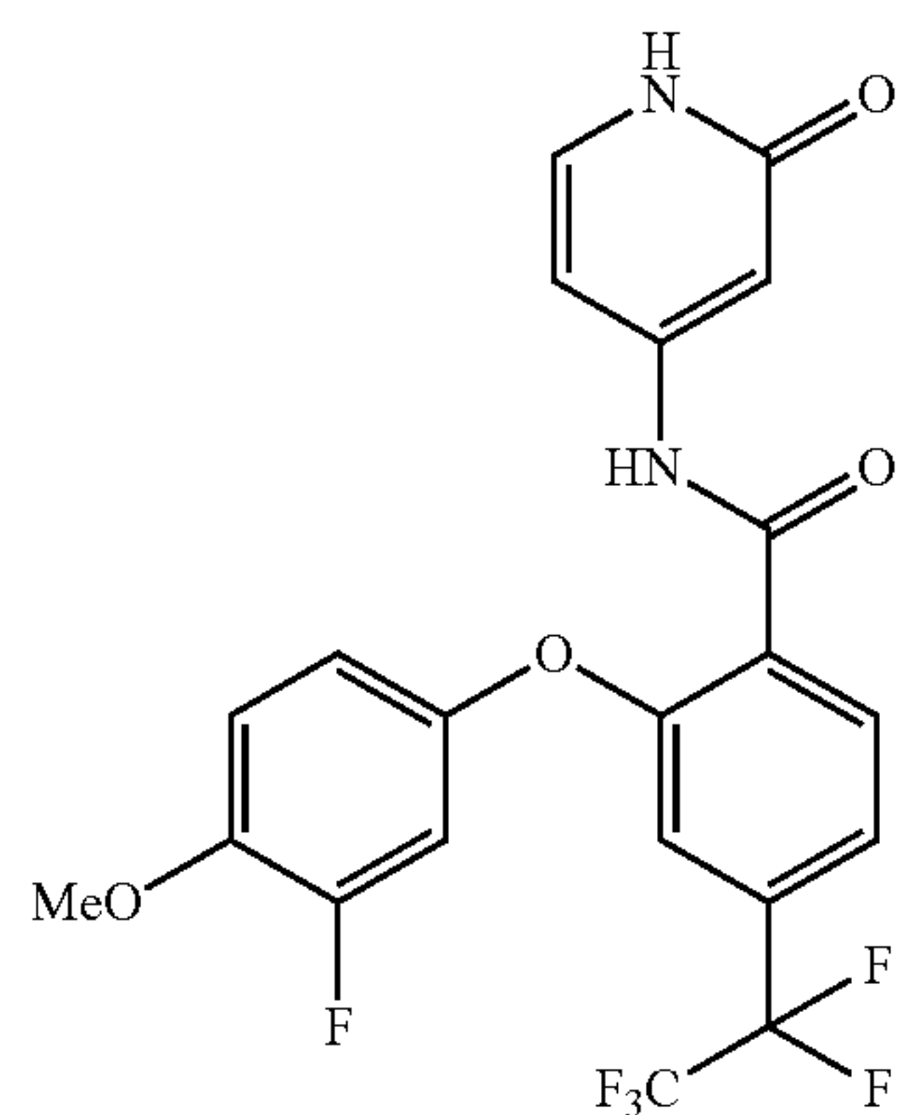
2-(3-fluoro-4-methoxyphenoxy)-N-(2-oxo-1,2-dihydropyridin-4-yl)-4-(perfluoroethyl)benzamide
