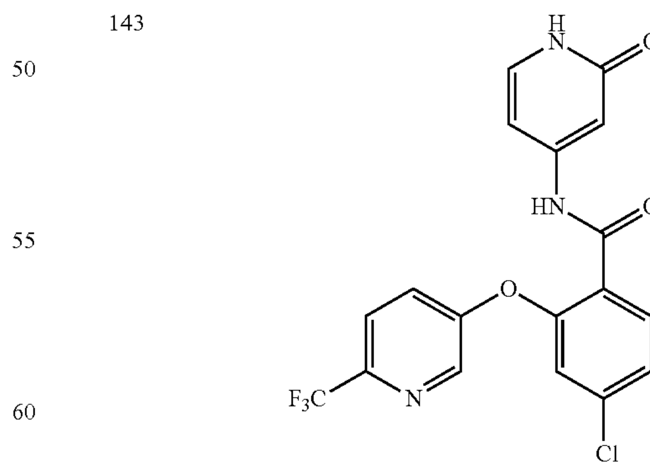
4-chloro-N-(2-oxo-1,2-dihydropyridin-4-yl)-2-((6-(trifluoromethyl)pyridin-3-yl)oxy)benzamide
