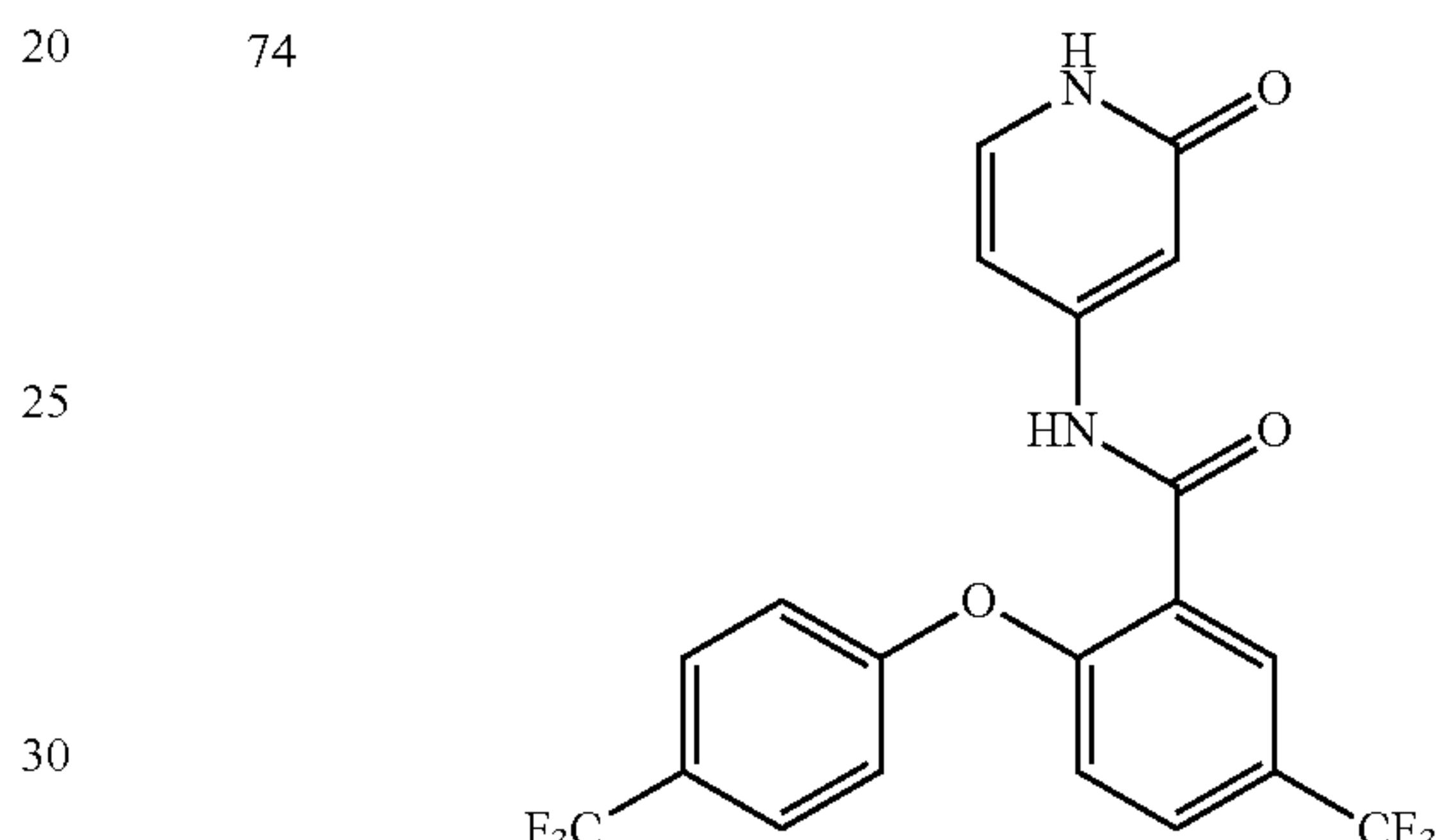
N-(2-oxo-1,2-dihydropyridin-4-yl)-5-(trifluoromethyl)-2-(4-(trifluoromethyl)phenoxy)benzamide
