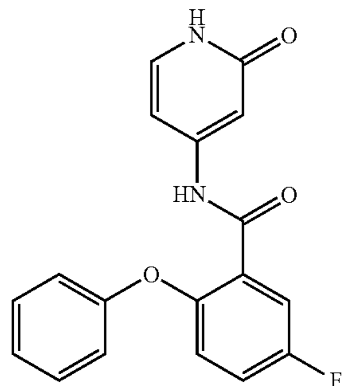
5-fluoro-N-(2-oxo-1,2-dihydropyridin-4-yl)-2-phenoxybenzamide
