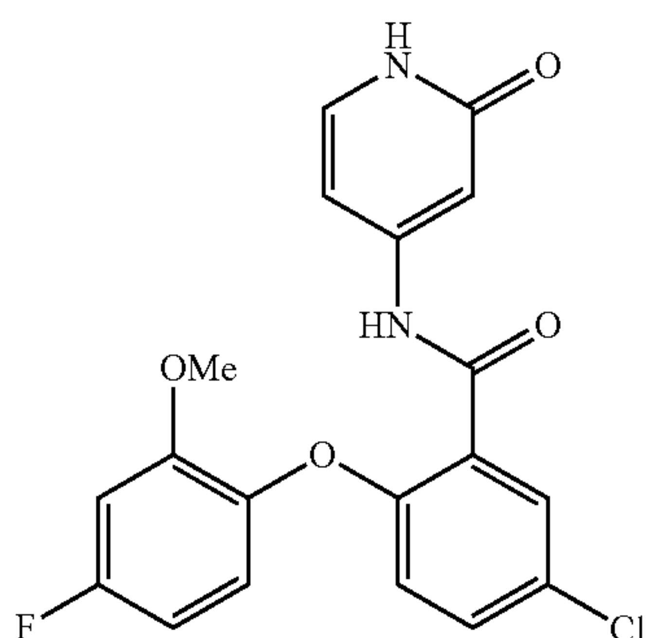
5-chloro-2-(4-fluoro-2-methoxyphenoxy)-N-(2-oxo-1,2-dihydropyridin-4-yl)benzamide
