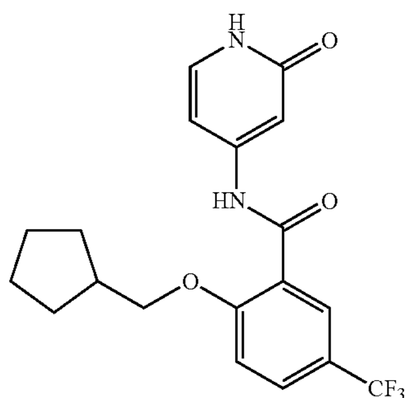
2-(cyclopentylmethoxy)-N-(2-oxo-1,2-dihydropyridin-4-yl)-5-(trifluoromethyl)benzamide
