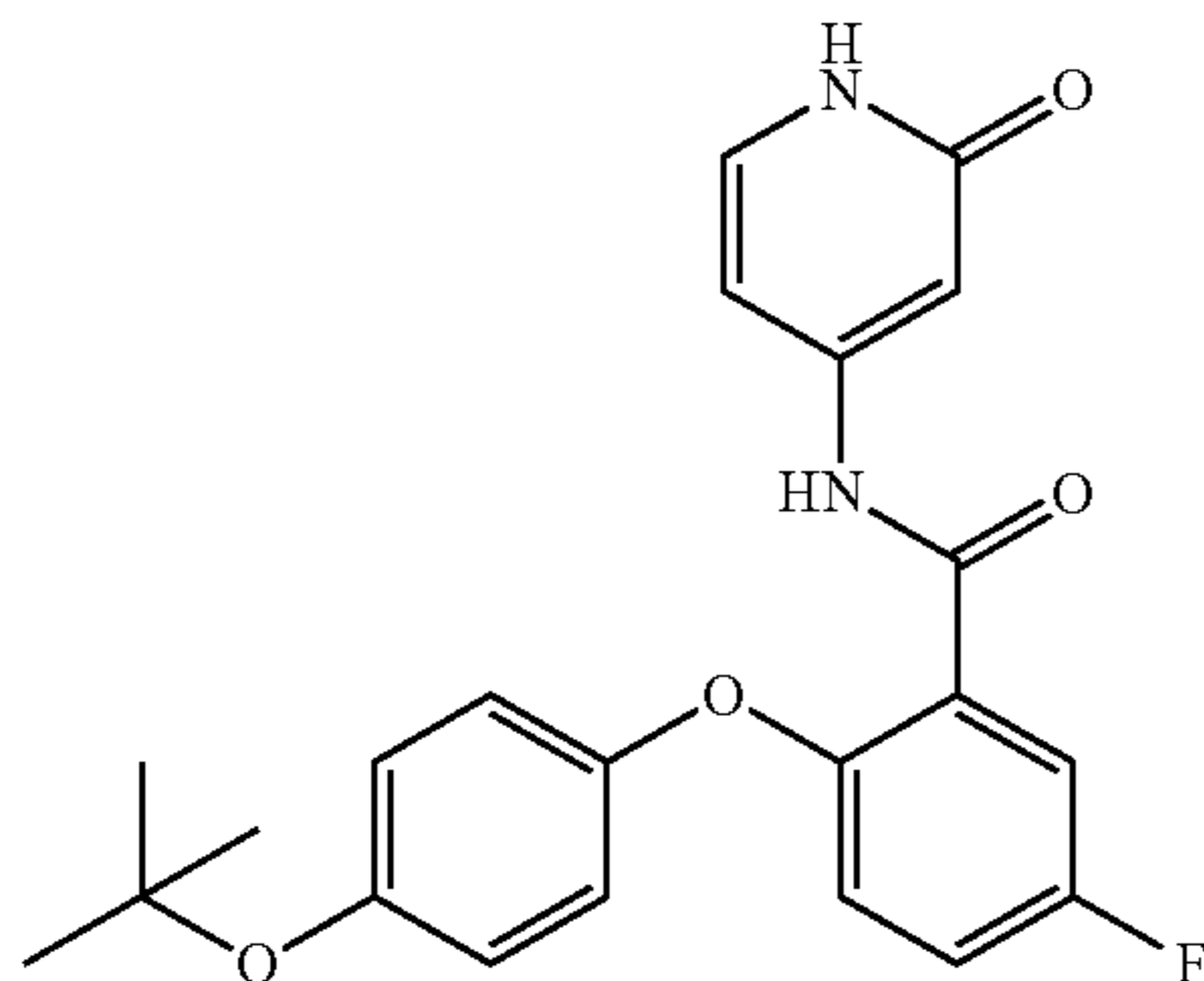
2-(4-(tert-butoxy)phenoxy)-5-fluoro-N-(2-oxo-1,2-dihydropyridin-4-yl)benzamide
