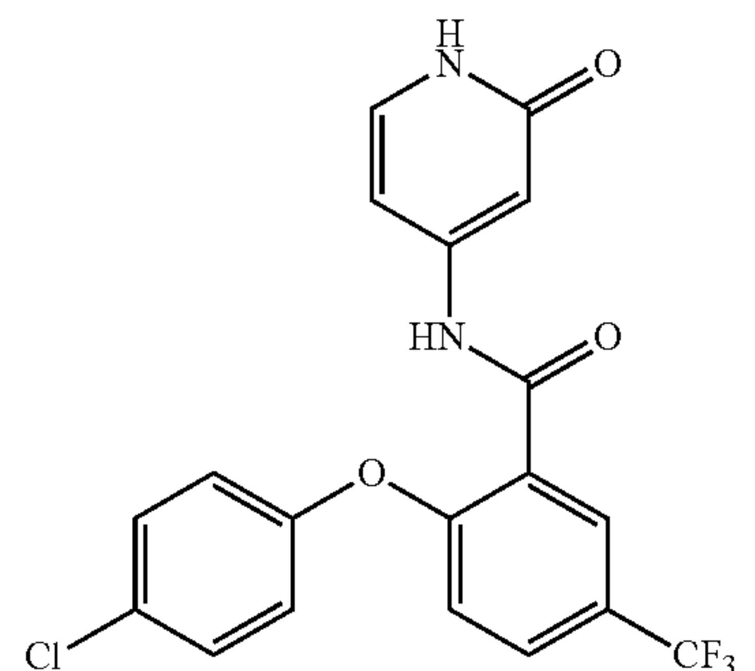
2-(4-chlorophenoxy)-N-(2-oxo-1,2-dihydropyridin-4-yl)-5-(trifluoromethyl)benzamide
