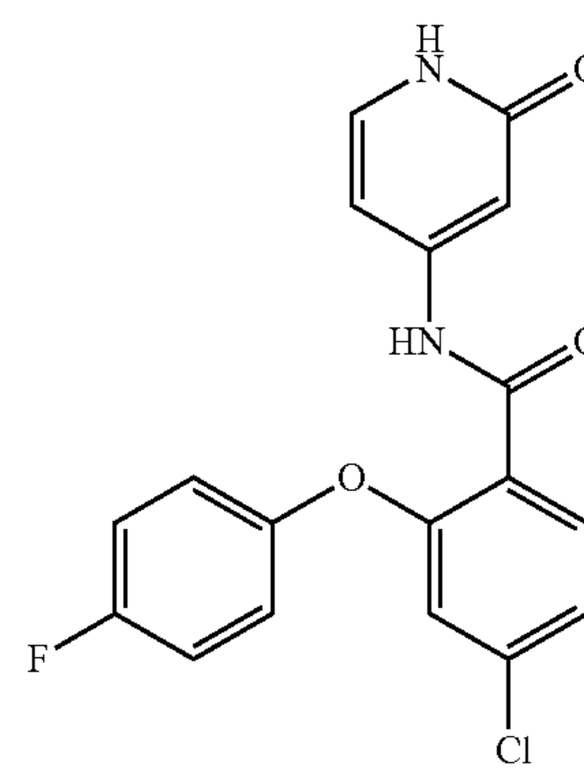
4-chloro-2-(4-fluorophenoxy)-N-(2-oxo-1,2-dihydropyridin-4-yl)benzamide
