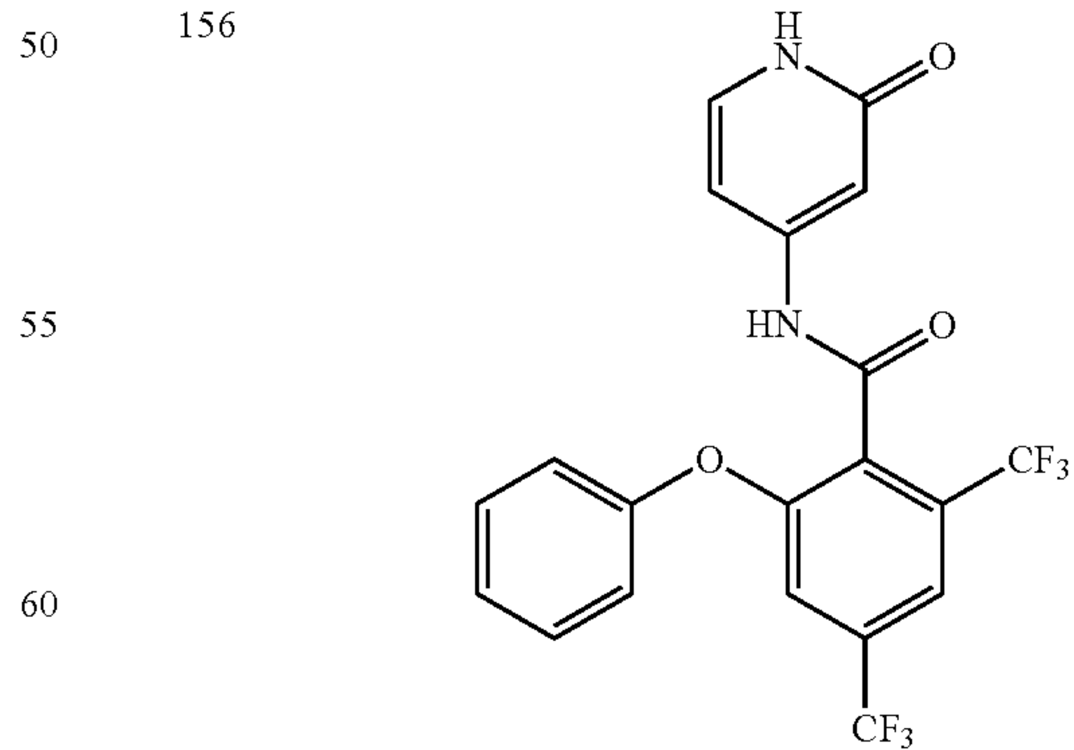
N-(2-oxo-1,2-dihydropyridin-4-yl)-2-phenoxy-4,6-bis(trifluoromethyl)benzamide
