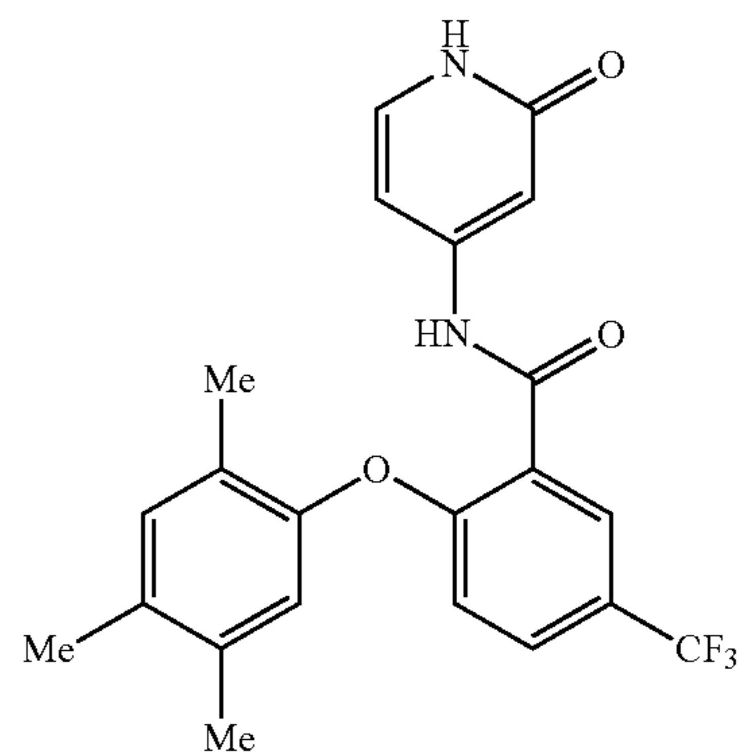
N-(2-oxo-1,2-dihydropyridin-4-yl)-5-(trifluoromethyl)-2-(2,4,5-trimethylphenoxy)benzamide
