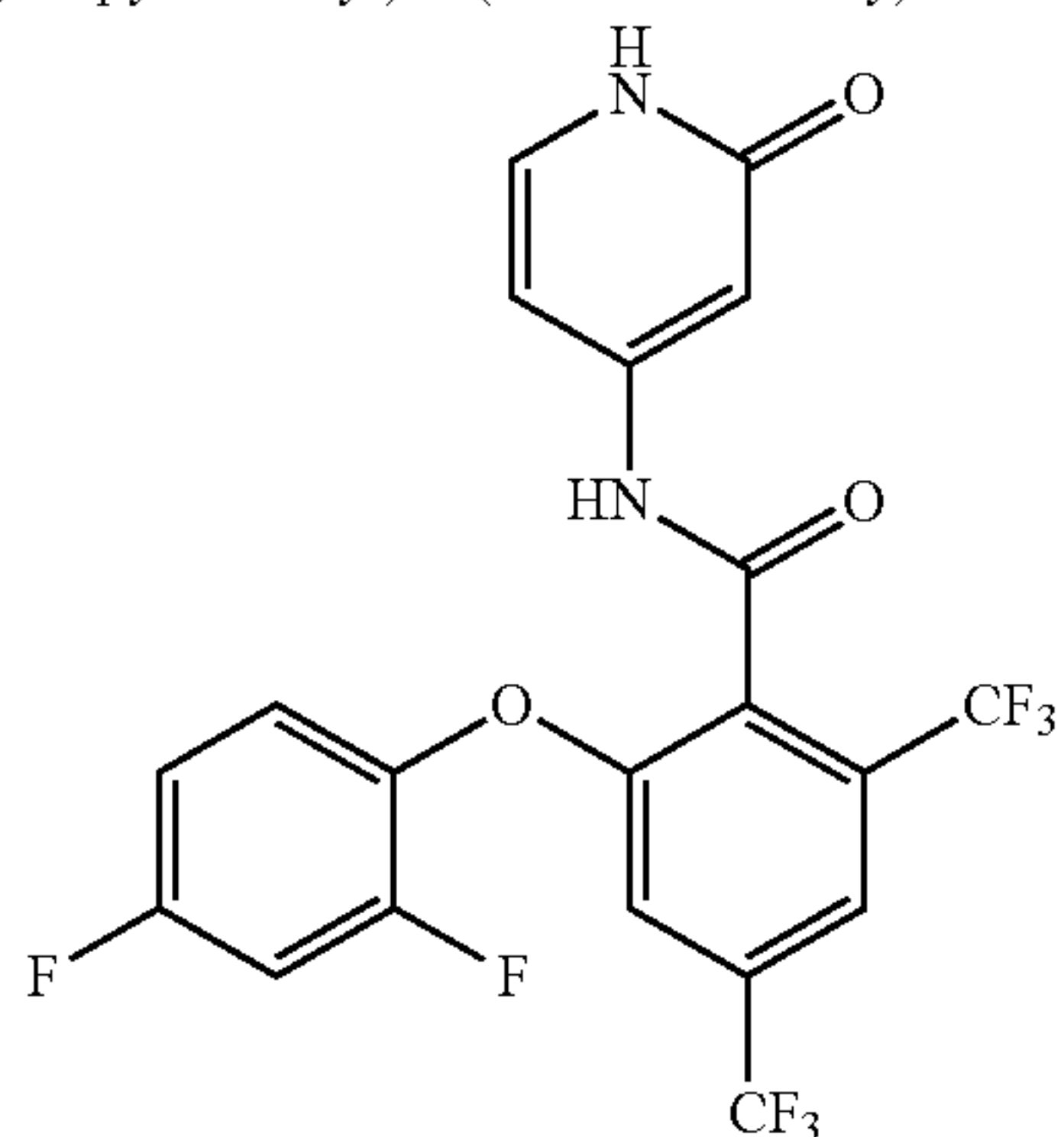
2-((2-methylpyridin-3-yl)oxy)-N-(2-oxo-1,2-dihydropyridin-4-yl)-5-(trifluoromethoxy)benzamide
