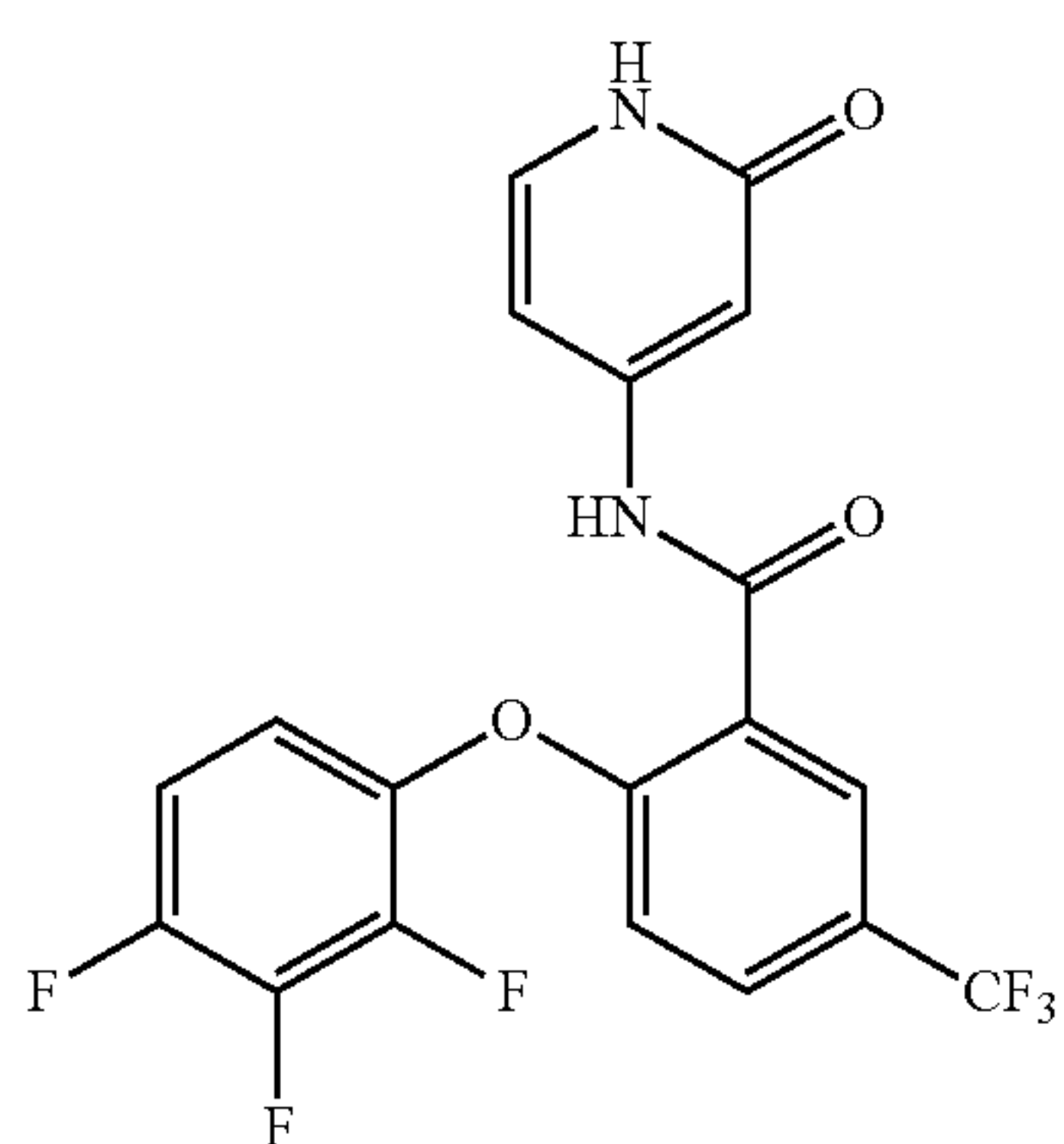
N-(2-oxo-1,2-dihydropyridin-4-yl)-5-(trifluoromethyl)-2-(2,3,4-trifluorophenoxy)benzamide
