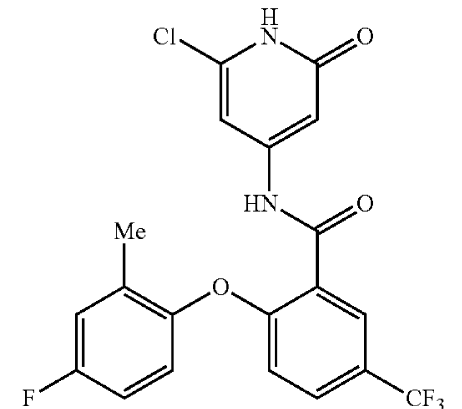
N-(6-chloro-2-oxo-1,2-dihydropyridin-4-yl)-2-(4-fluoro-2-methylphenoxy)-5-(trifluoromethyl)benzamide
