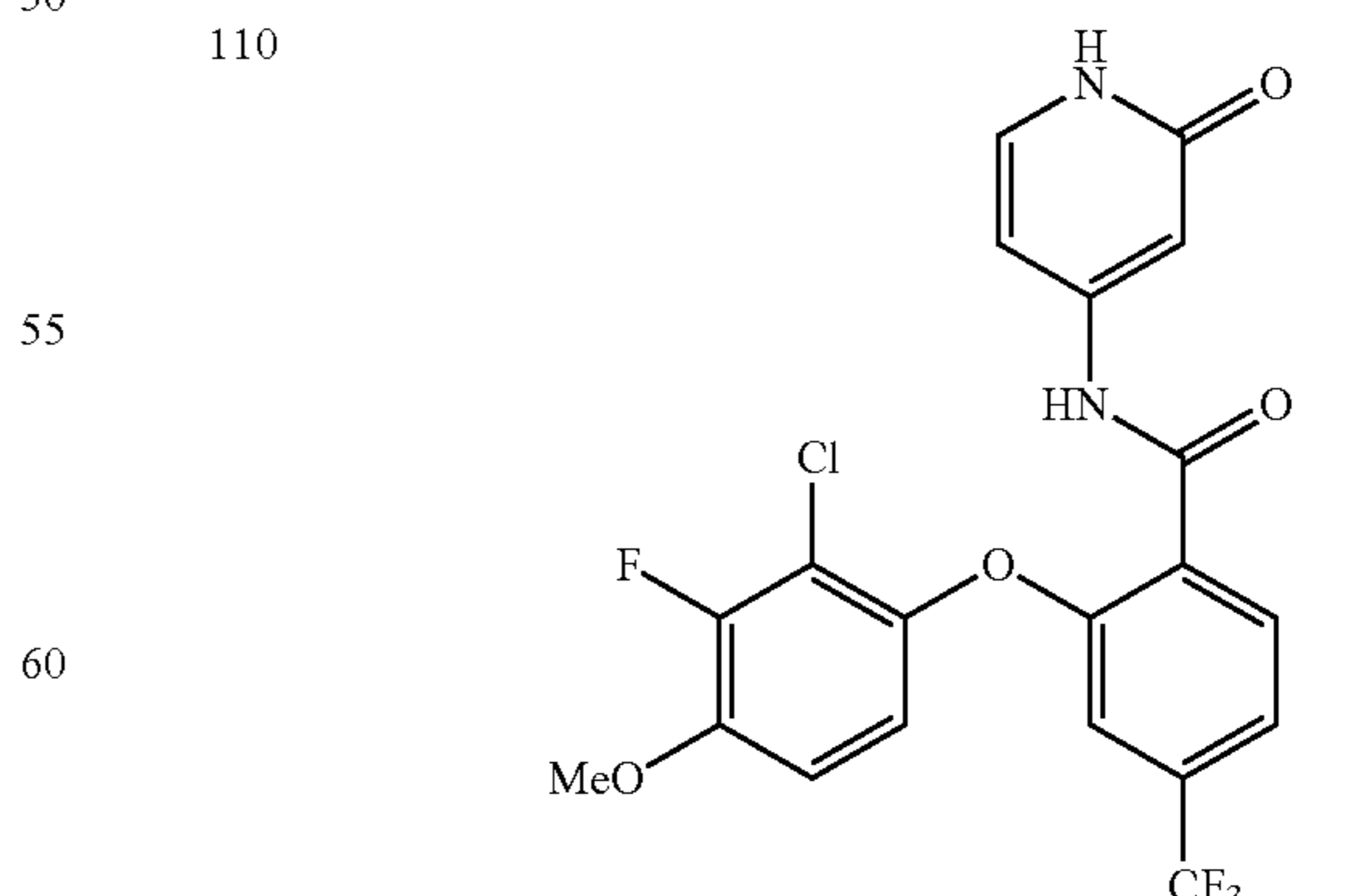
2-(2-chloro-3-fluoro-4-methoxyphenoxy)-N-(2-oxo-1,2-dihydropyridin-4-yl)-4-(trifluoromethyl)benzamide
