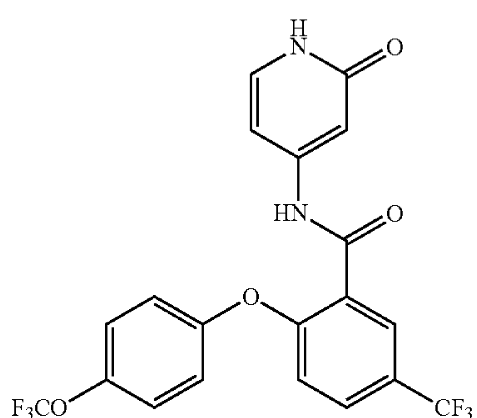
N-(2-oxo-1,2-dihydropyridin-4-yl)-2-(4-(trifluoromethoxy)phenoxy)-5-(trifluoromethyl)benzamide
