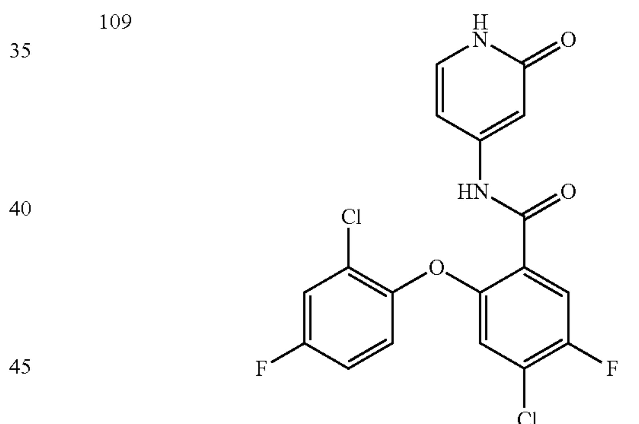
4-chloro-2-(2-chloro-4-fluorophenoxy)-5-fluoro-N-(2-oxo-1,2-dihydropyridin-4-yl)benzamide
