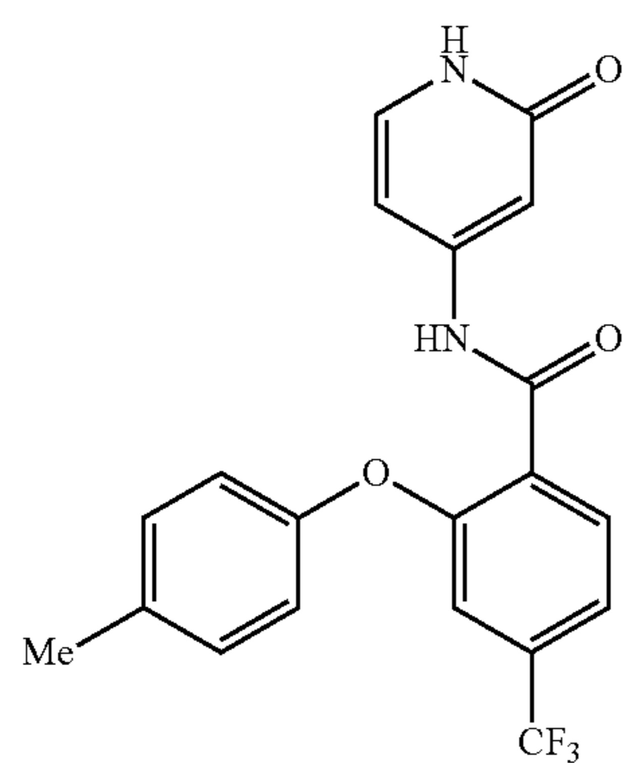
N-(2-oxo-1,2-dihydropyridin-4-yl)-2-(p-tolyloxy)-4-(trifluoromethyl)benzamide
