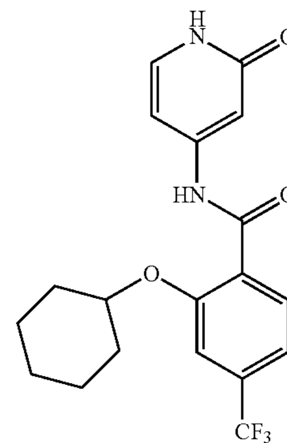
2-(cyclohexyloxy)-N-(2-oxo-1,2-dihydropyridin-4-yl)-4-(trifluoromethyl)benzamide
