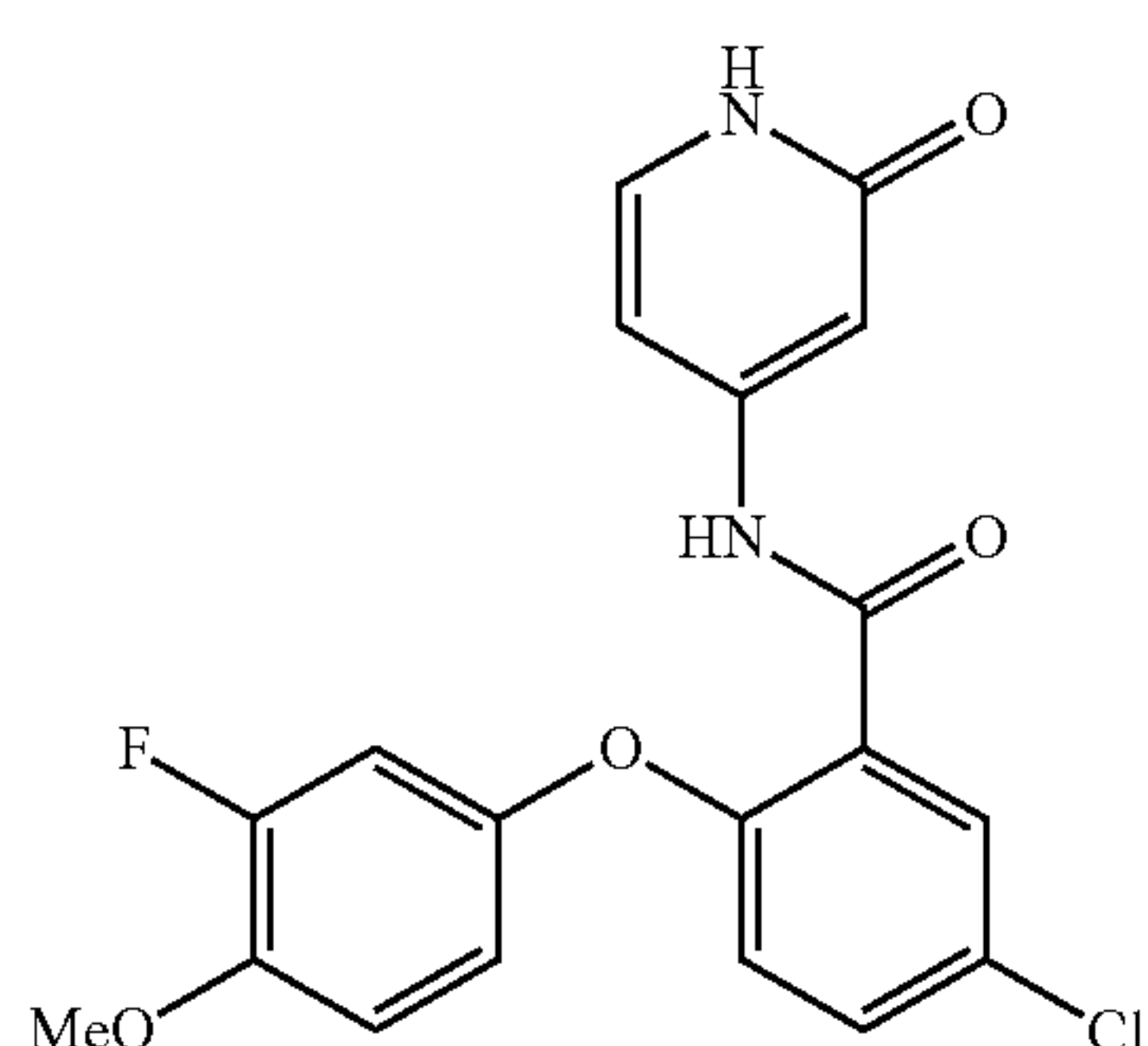
5-chloro-2-(3-fluoro-4-methoxyphenoxy)-N-(2-oxo-1,2-dihydropyridin-4-yl)benzamide
