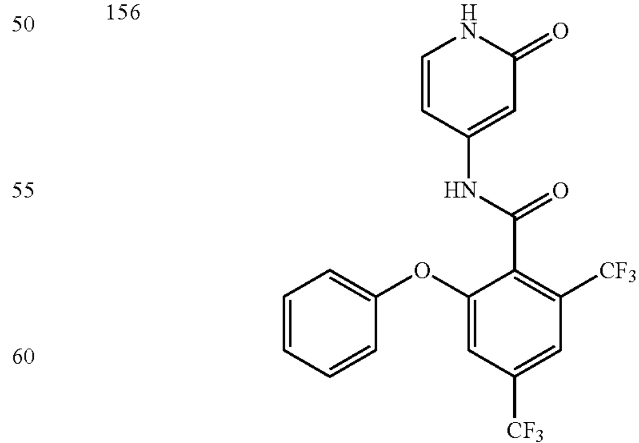
N-(2-oxo-1,2-dihydropyridin-4-yl)-2-phenoxy-4,6-bis(trifluoromethyl)benzamide
