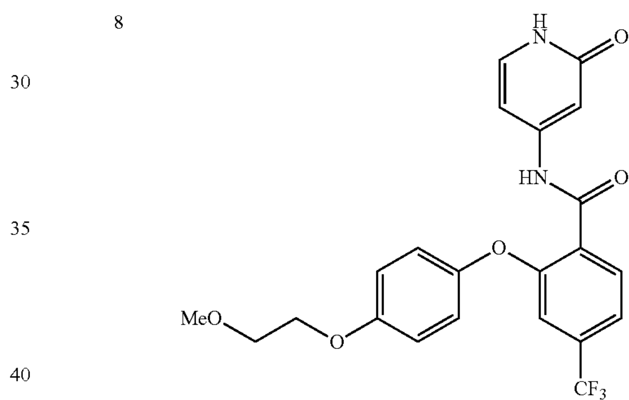
2-(2,4-difluorophenoxy)-N-(2-oxo-1,2-dihydropyridin-4-yl)-4-(trifluoromethyl)benzamide
