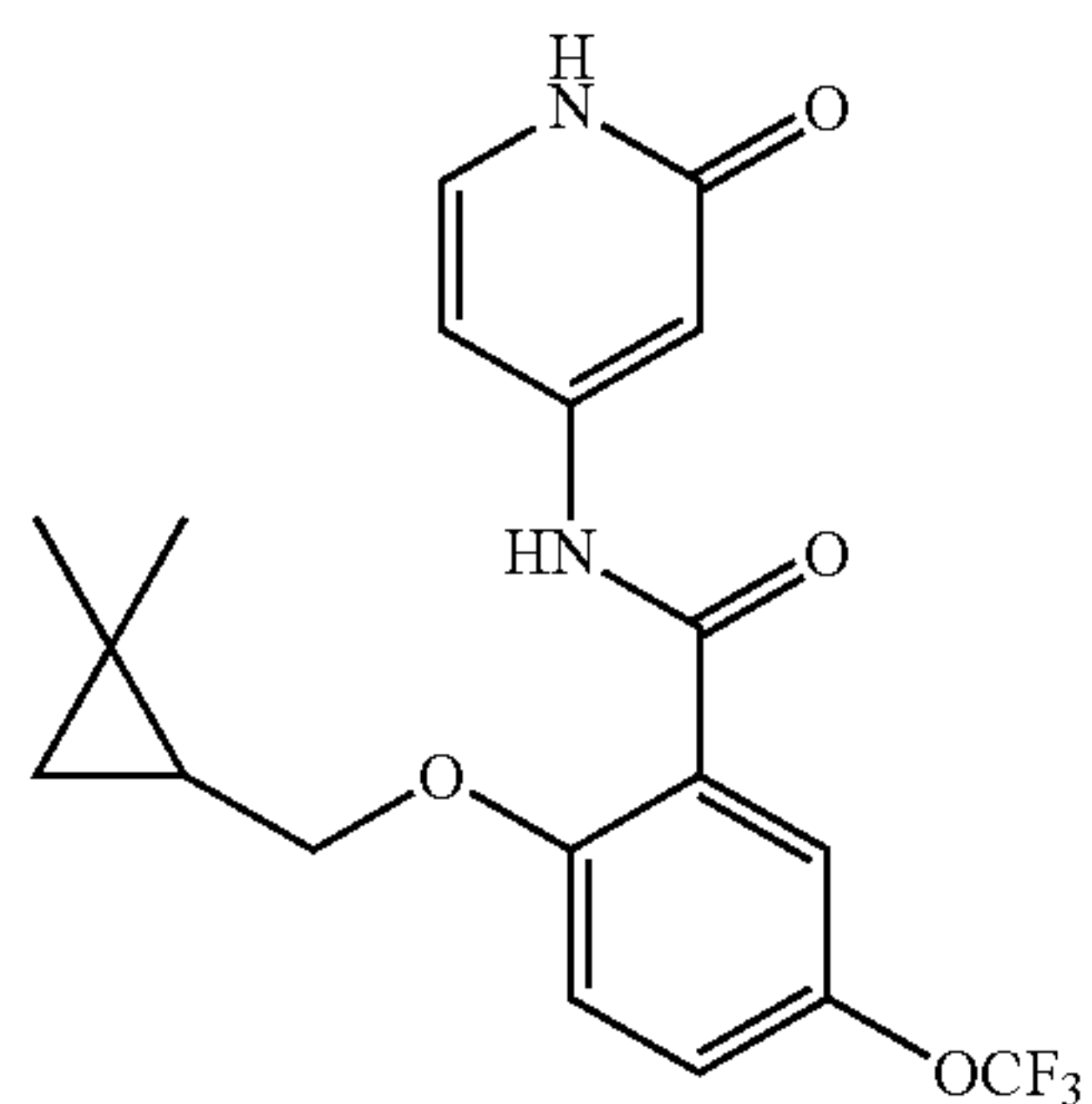
2-((2,2-dimethylcyclopropyl)methoxy)-N-(2-oxo-1,2-dihydropyridin-4-yl)-5-(trifluoromethoxy)benzamide
