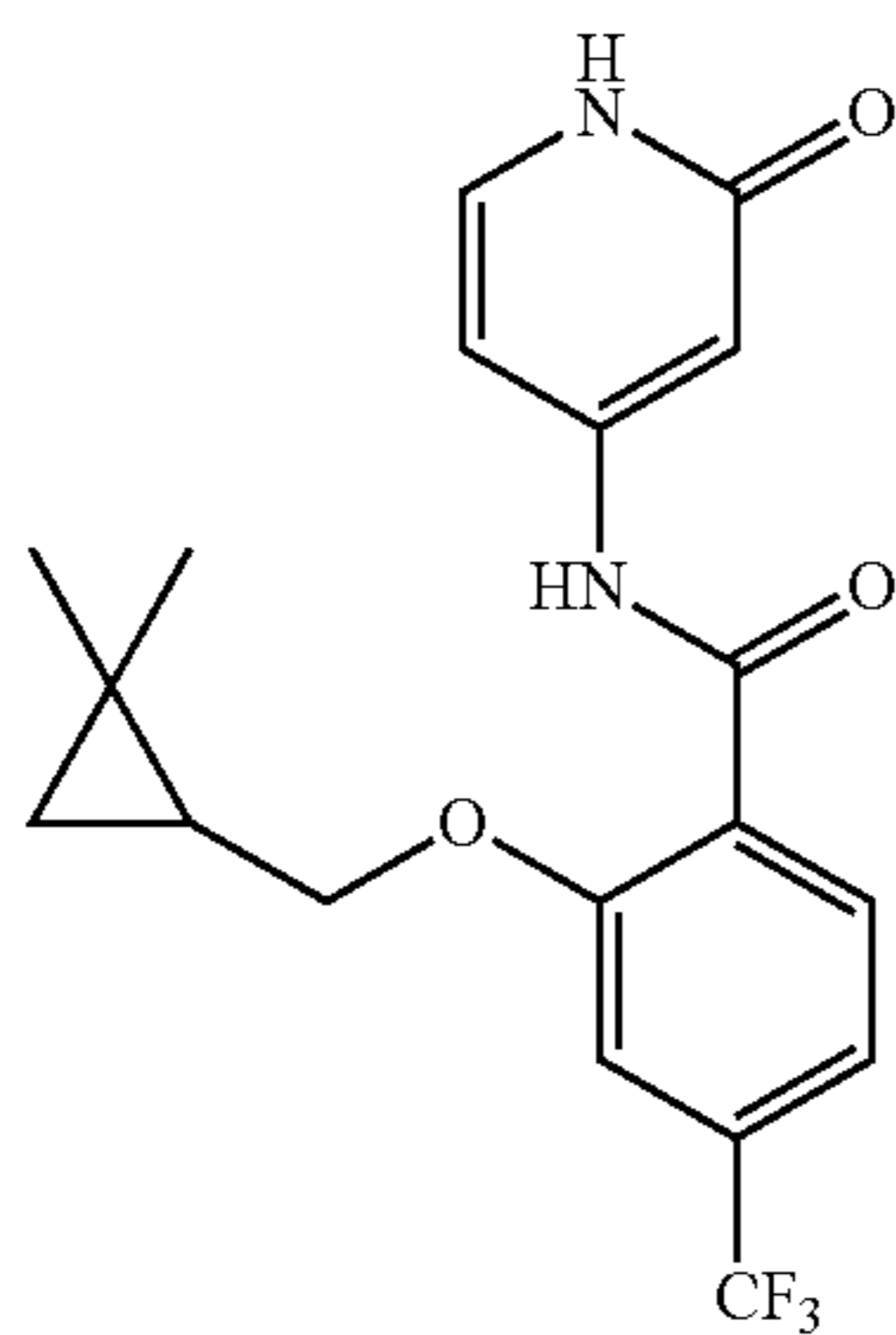
2-((2,2-dimethylcyclopropyl)methoxy)-N-(2-oxo-1,2-dihydropyridin-4-yl)-4-(trifluoromethyl)benzamide
