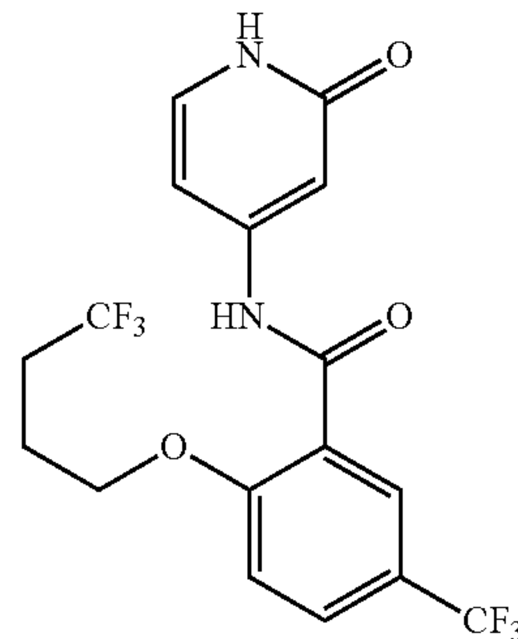
N-(2-oxo-1,2-dihydropyridin-4-yl)-2-(4,4,4-trifluorobutoxy)-5-(trifluoromethyl)benzamide
