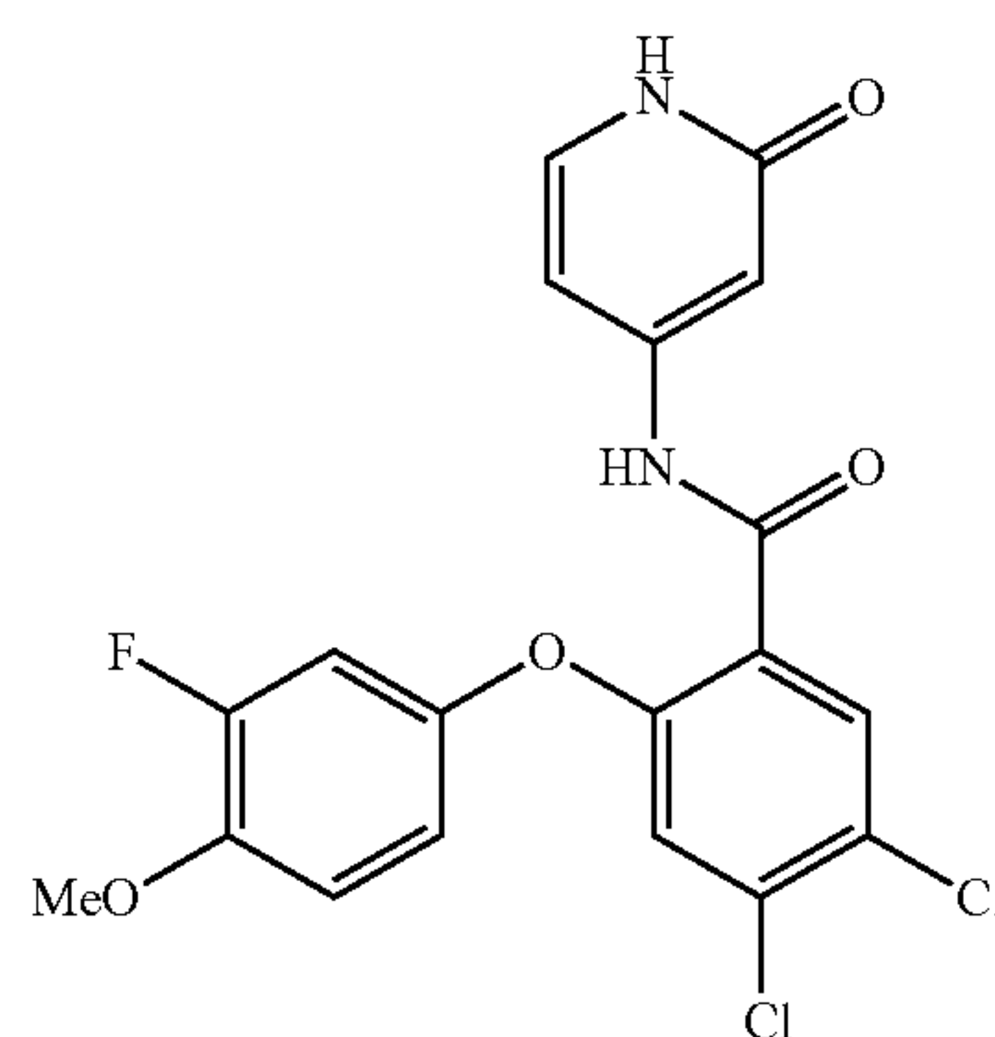
4,5-dichloro-2-(3-fluoro-4-methoxyphenoxy)-N-(2-oxo-1,2-dihydropyridin-4-yl)benzamide
