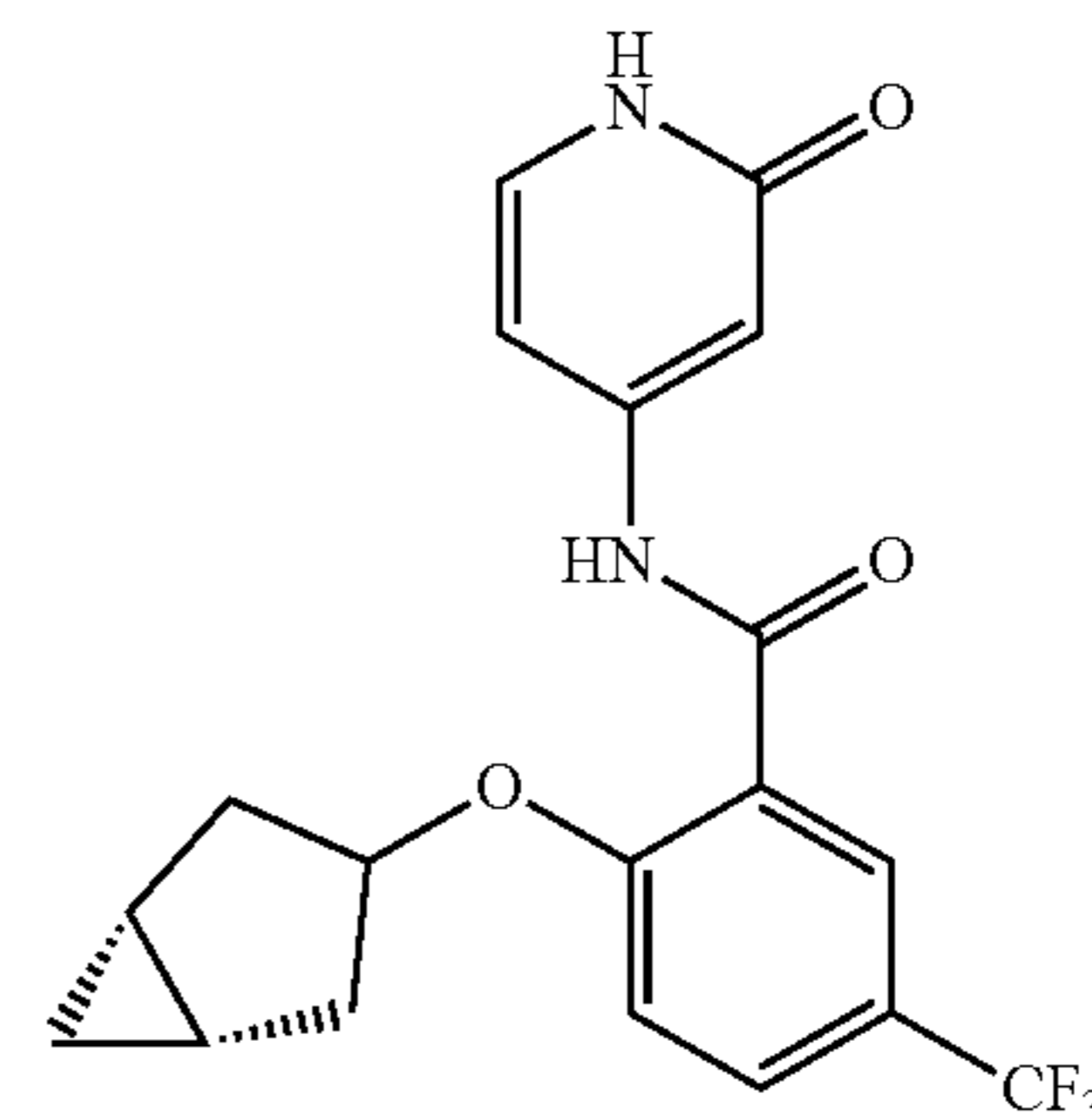
2-((1R,5S)-bicyclo[3.1.0]hexan-3-yl)oxy-N-(2-oxo-1,2-dihydropyridin-4-yl)-5-(trifluoromethyl)benzamide
