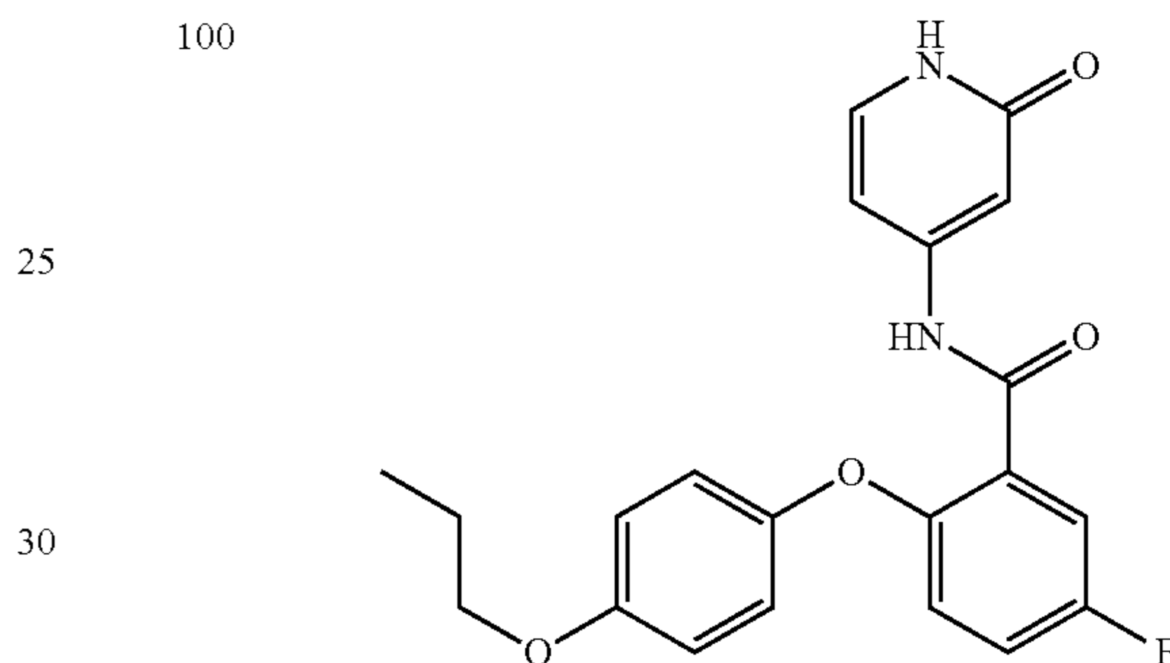
5-fluoro-N-(2-oxo-1,2-dihydropyridin-4-yl)-2-(4-propoxyphenoxy)benzamide
