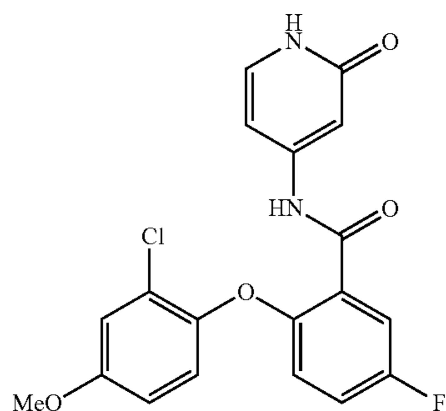
2-(2-chloro-4-methoxyphenoxy)-5-fluoro-N-(2-oxo-1,2-dihydropyridin-4-yl)benzamide
