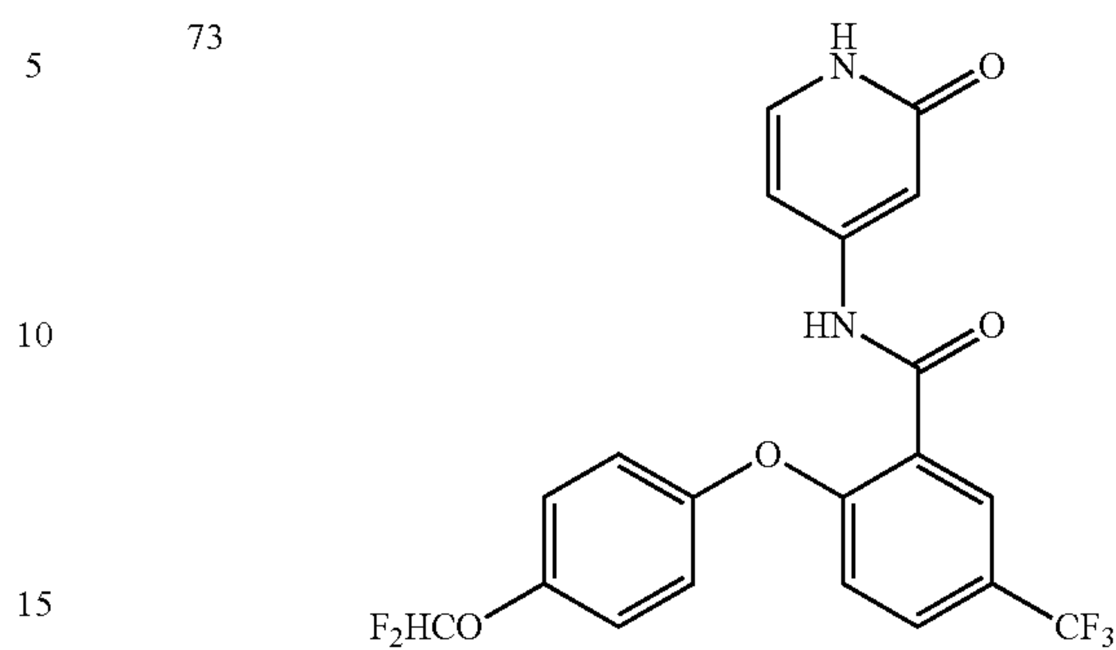
2-(4-(difluoromethoxy)phenoxy)-N-(2-oxo-1,2-dihydropyridin-4-yl)-5-(trifluoromethyl)benzamide
