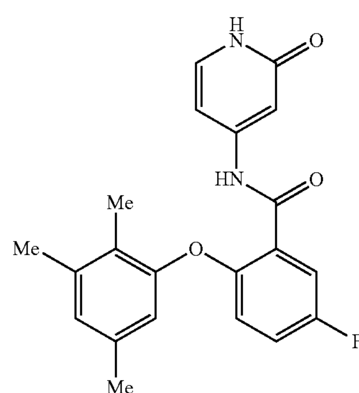
5-fluoro-N-(2-oxo-1,2-dihydropyridin-4-yl)-2-(2,3,5-trimethylphenoxy)benzamide
