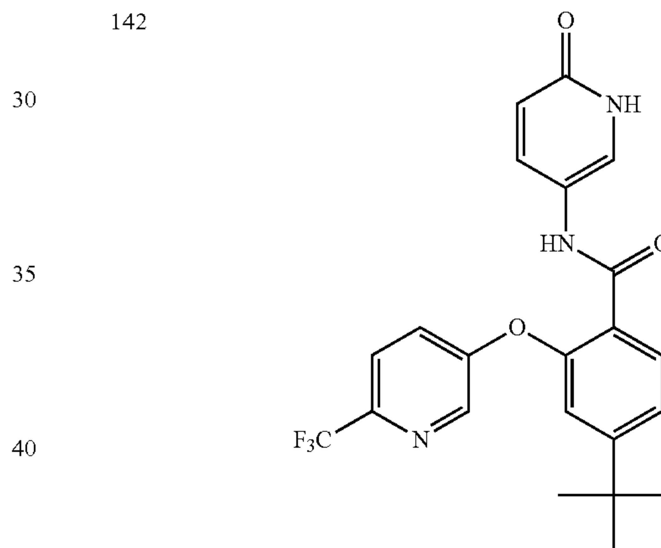
4-(tert-butyl)-N-(6-oxo-1,6-dihydropyridin-3-yl)-2-((6-(trifluoromethyl)pyridin-3-yl)oxy)benzamide
