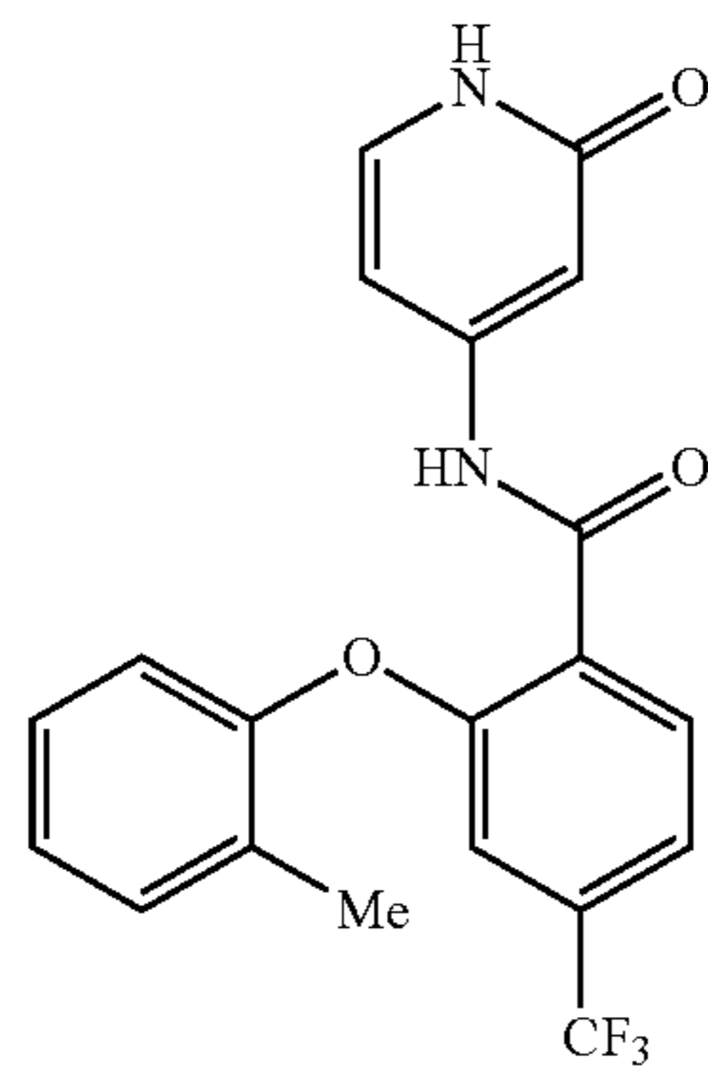
N-(2-oxo-1,2-dihydropyridin-4-yl)-2-(o-tolyloxy)-4-(trifluoromethyl)benzamide
