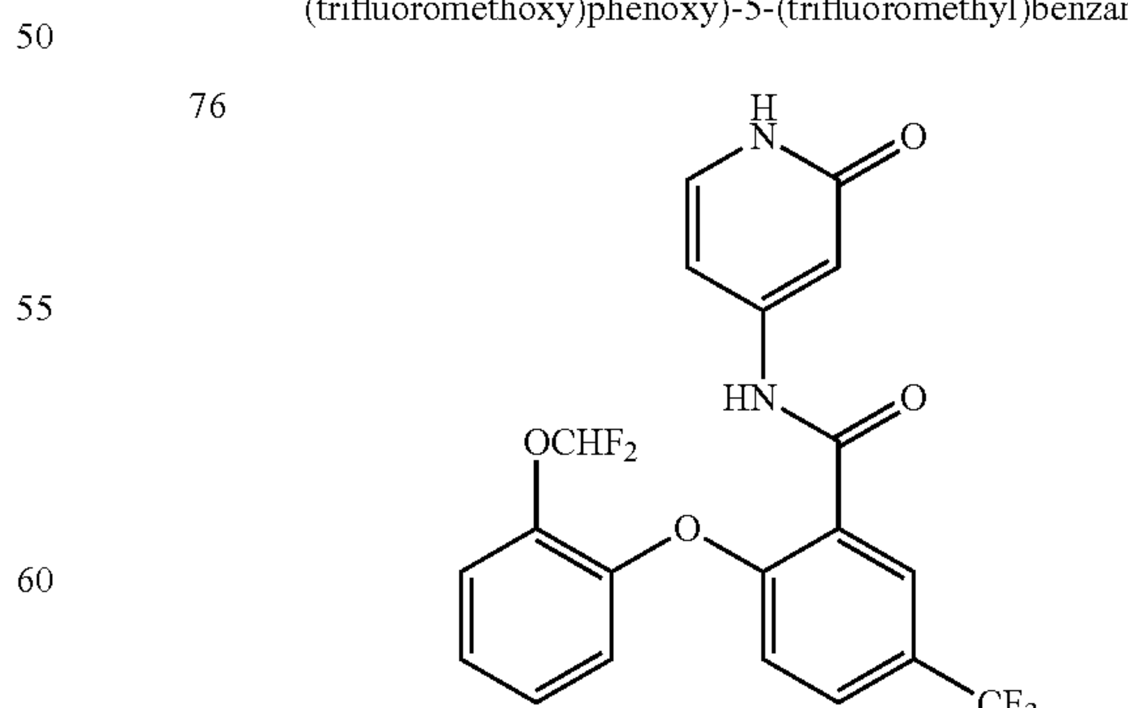
2-(2-(difluoromethoxy)phenoxy)-N-(2-oxo-1,2-dihydropyridin-4-yl)-5-(trifluoromethyl)benzamide
