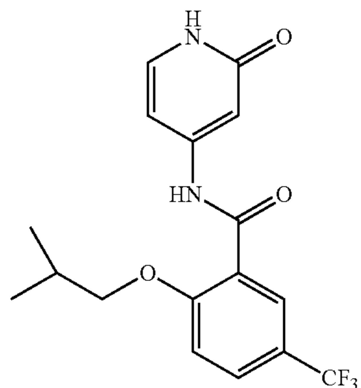
2-isobutoxy-N-(2-oxo-1,2-dihydropyridin-4-yl)-5-(trifluoromethyl)benzamide
