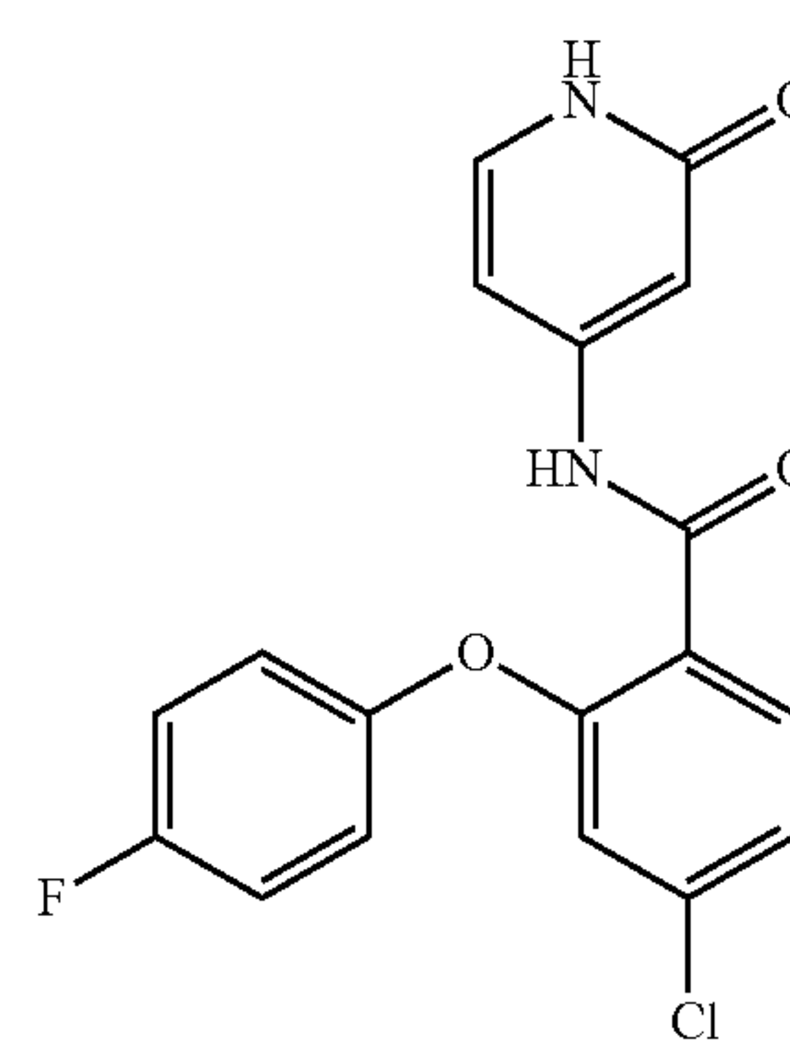
4-chloro-2-(4-fluorophenoxy)-N-(2-oxo-1,2-dihydropyridin-4-yl)benzamide
