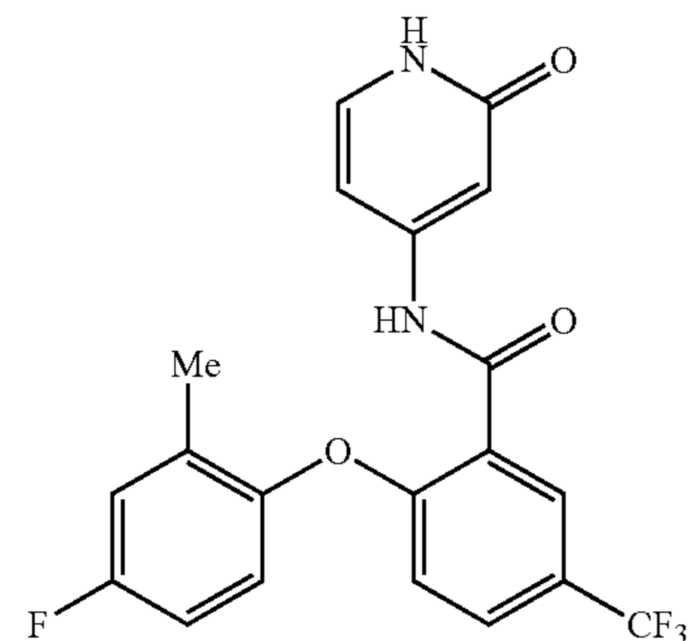
2-(4-fluoro-2-methylphenoxy)-N-(2-oxo-1,2-dihydropyridin-4-yl)-5-(trifluoromethyl)benzamide
