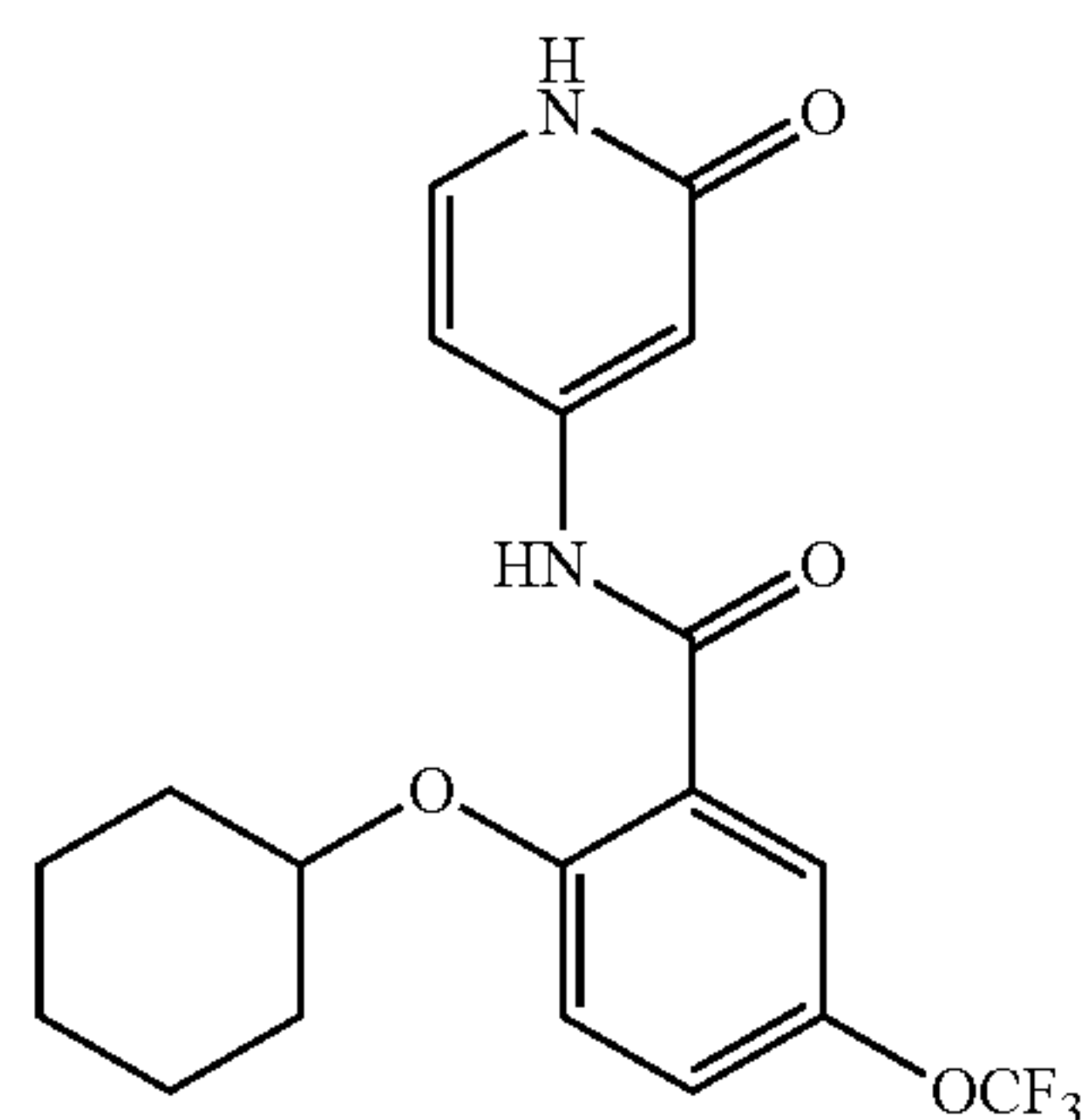
2-(cyclohexyloxy)-N-(2-oxo-1,2-dihydropyridin-4-yl)-5-(trifluoromethoxy)benzamide
