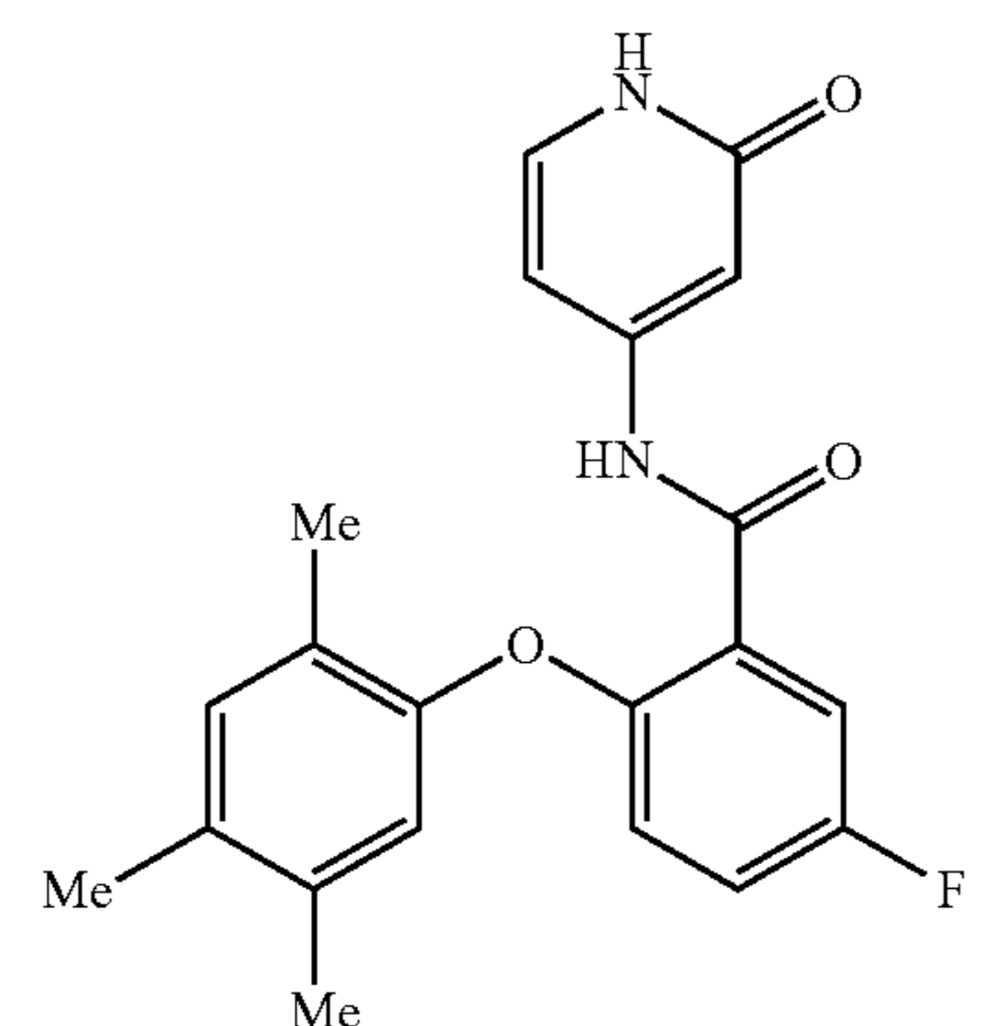
5-fluoro-N-(2-oxo-1,2-dihydropyridin-4-yl)-2-(2,4,5-trimethylphenoxy)benzamide
