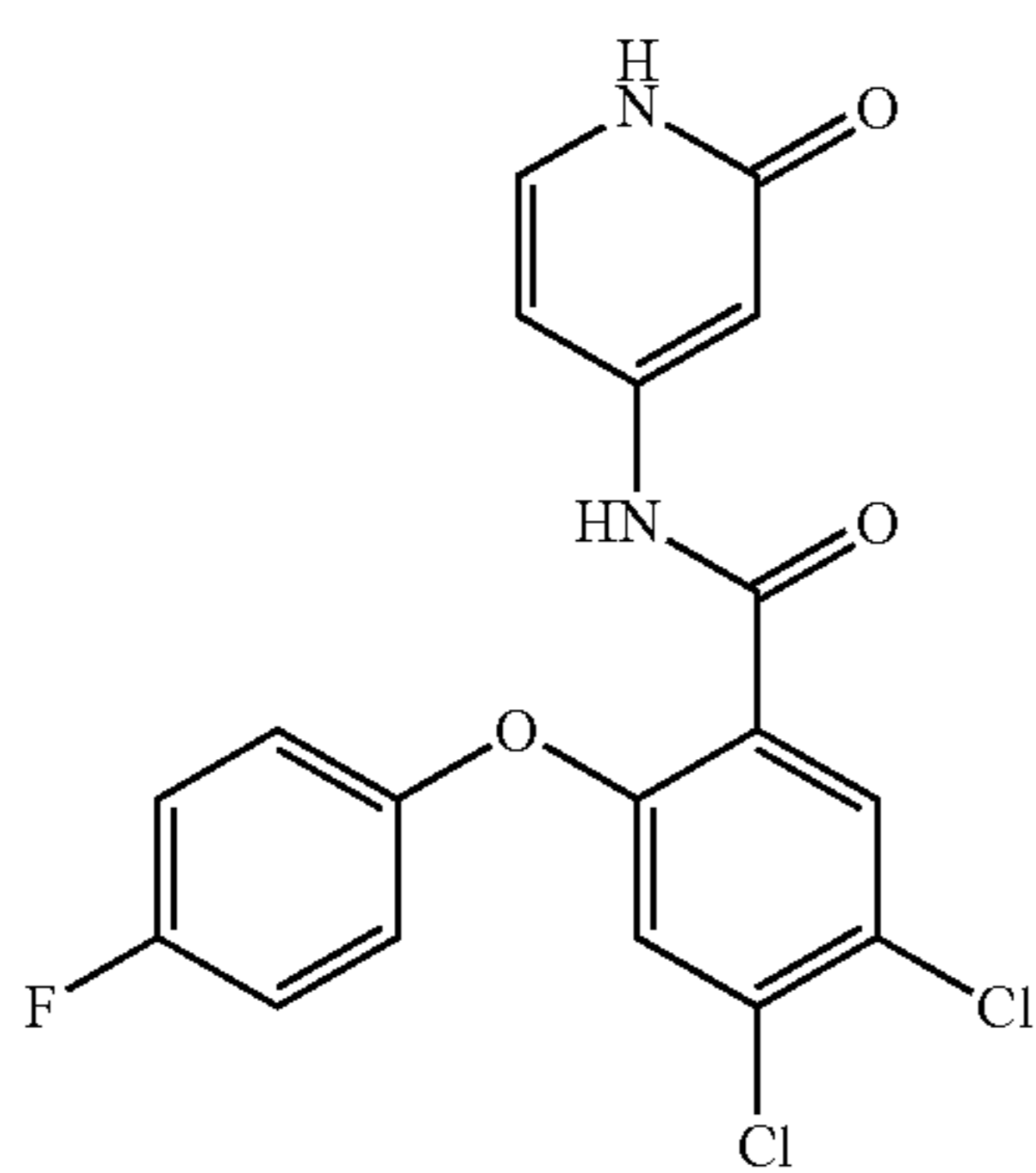
4,5-dichloro-2-(4-fluorophenoxy)-N-(2-oxo-1,2-dihydropyridin-4-yl)benzamide
