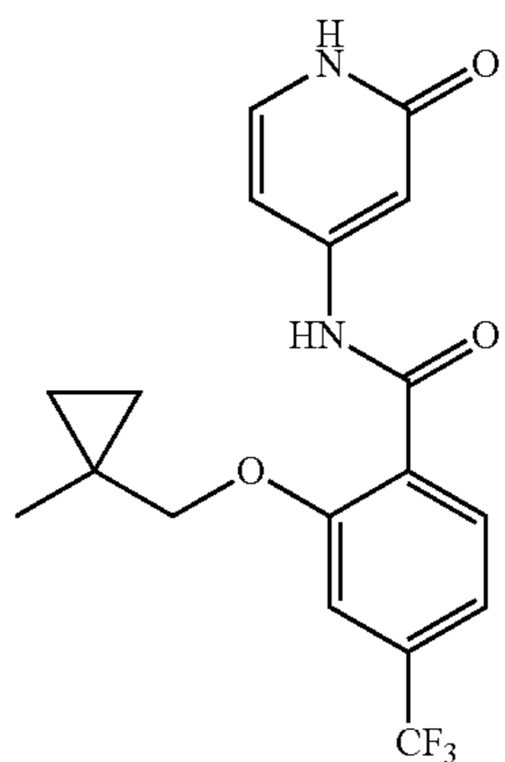
2-((1-methylcyclopropyl)methoxy)-N-(2-oxo-1,2-dihydropyridin-4-yl)-4-(trifluoromethyl)benzamide
