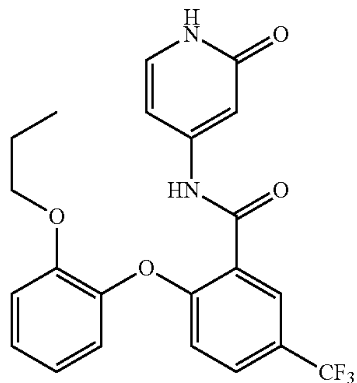
N-(2-oxo-1,2-dihydropyridin-4-yl)-2-(2-propoxyphenoxy)-5-(trifluoromethyl)benzamide
