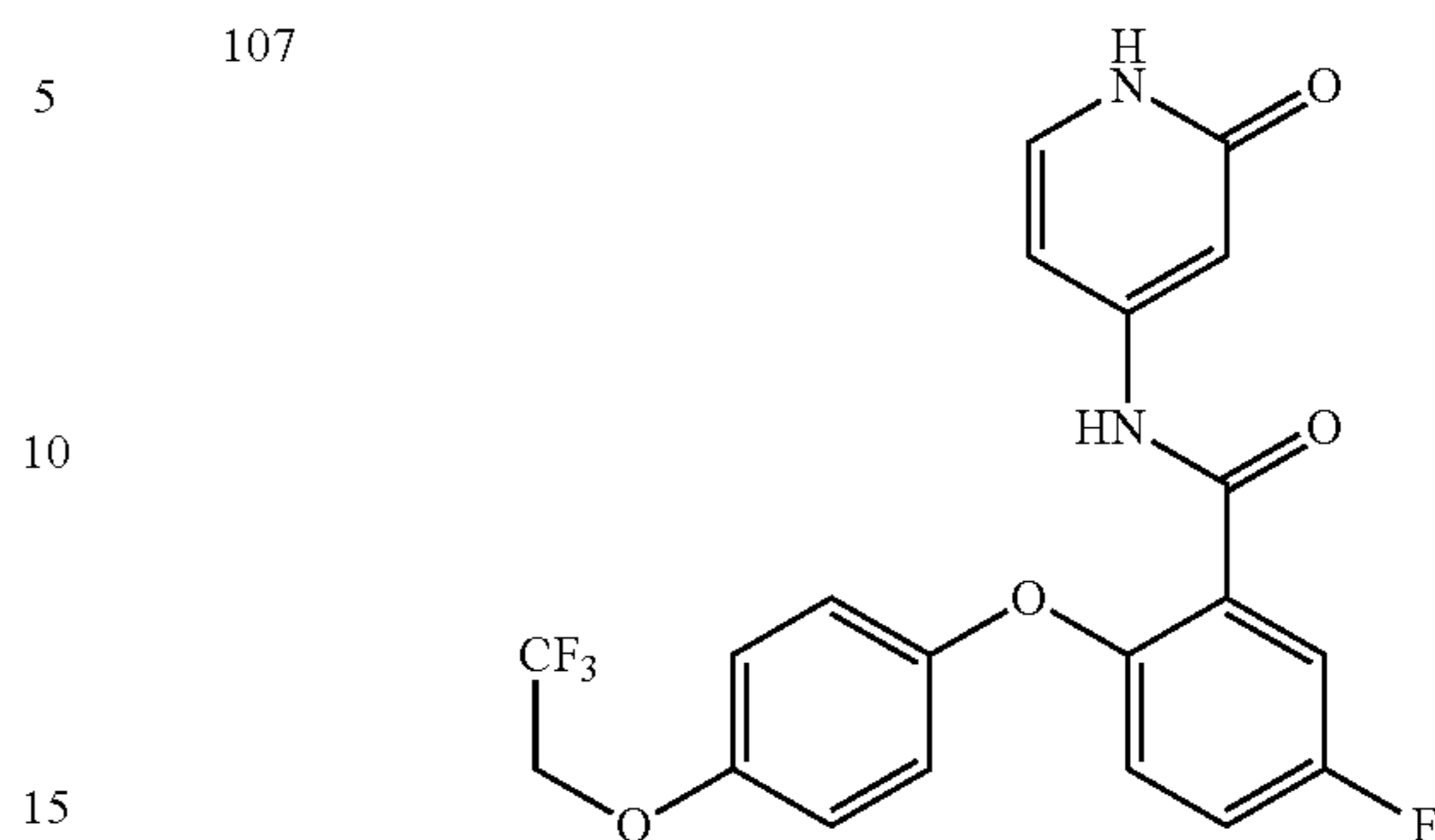
5-fluoro-N-(2-oxo-1,2-dihydropyridin-4-yl)-2-(4-(2,2,2-trifluoroethoxy)phenoxy)benzamide
