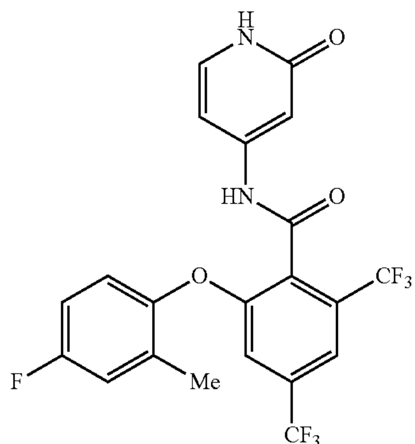
2-(4-fluoro-2-methylphenoxy)-N-(2-oxo-1,2-dihydropyridin-4-yl)-4,6-bis(trifluoromethyl)benzamide
