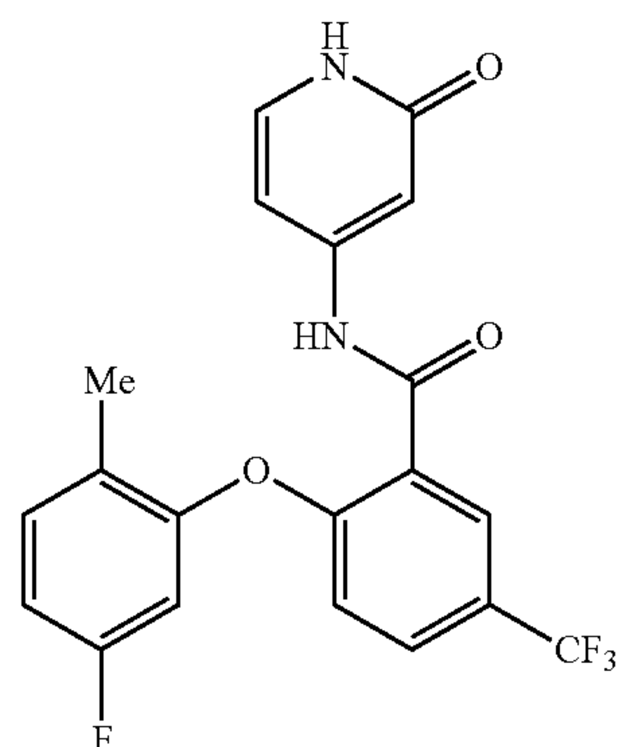
2-(5-fluoro-2-methylphenoxy)-N-(2-oxo-1,2-dihydropyridin-4-yl)-5-(trifluoromethyl)benzamide
