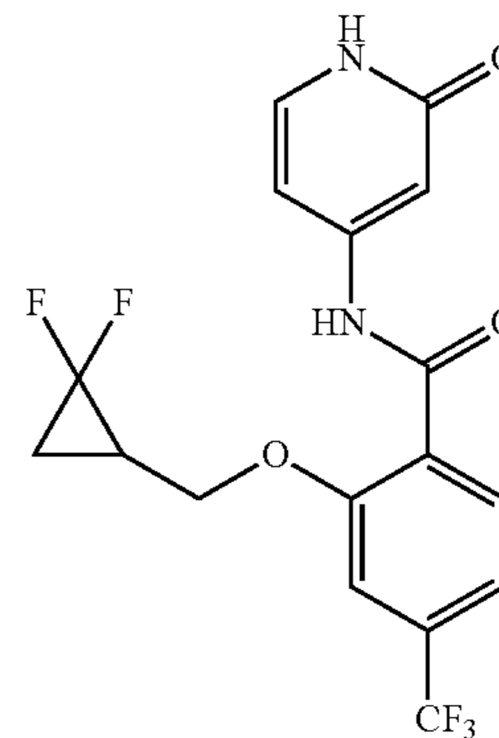
2-((2,2-difluorocyclopropyl)methoxy)-N-(2-oxo-1,2-dihydropyridin-4-yl)-4-(trifluoromethyl)benzamide
