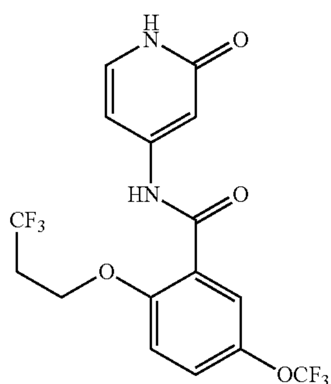
N-(2-oxo-1,2-dihydropyridin-4-yl)-5-(trifluoromethoxy)-2-(3,3,3-trifluoropropoxy)benzamide
