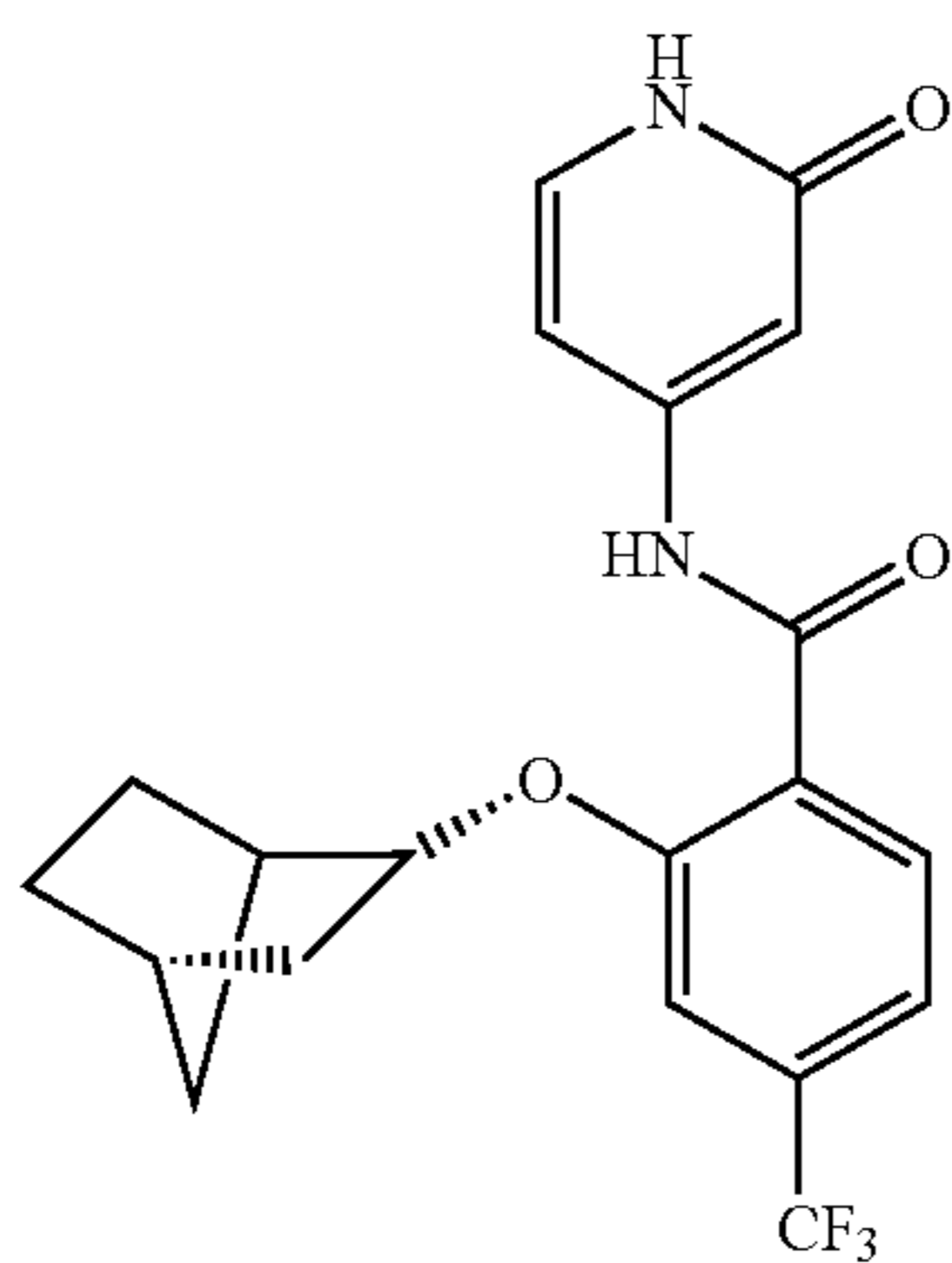
2-((2R)-bicyclo[2.2.1]heptan-2-yloxy)-N-(2-oxo-1,2-dihydropyridin-4-yl)-4-(trifluoromethyl)benzamide
