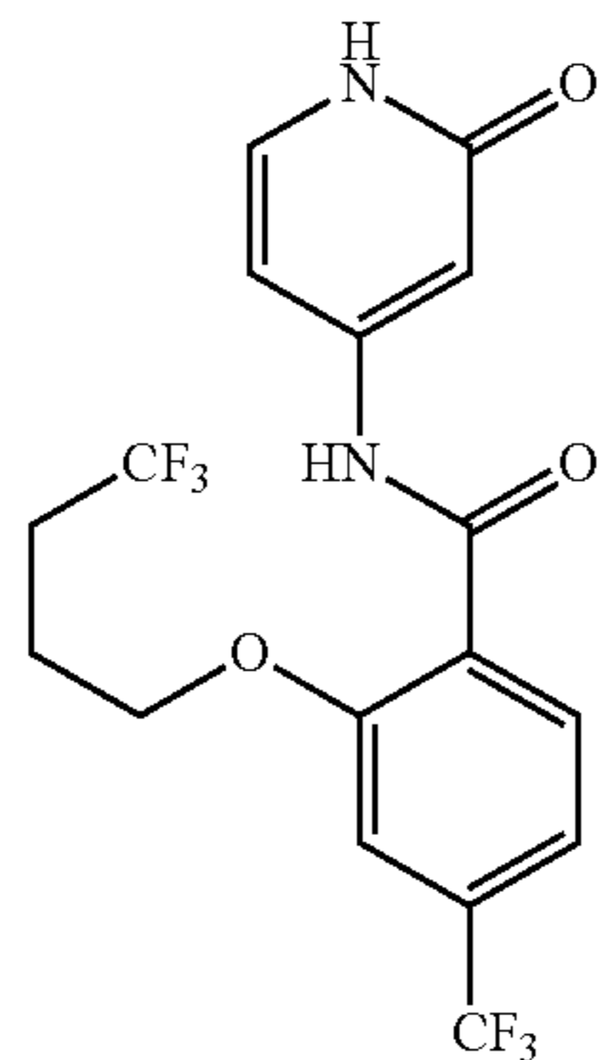
N-(2-oxo-1,2-dihydropyridin-4-yl)-2-(4,4,4-trifluorobutoxy)-4-(trifluoromethyl)benzamide
