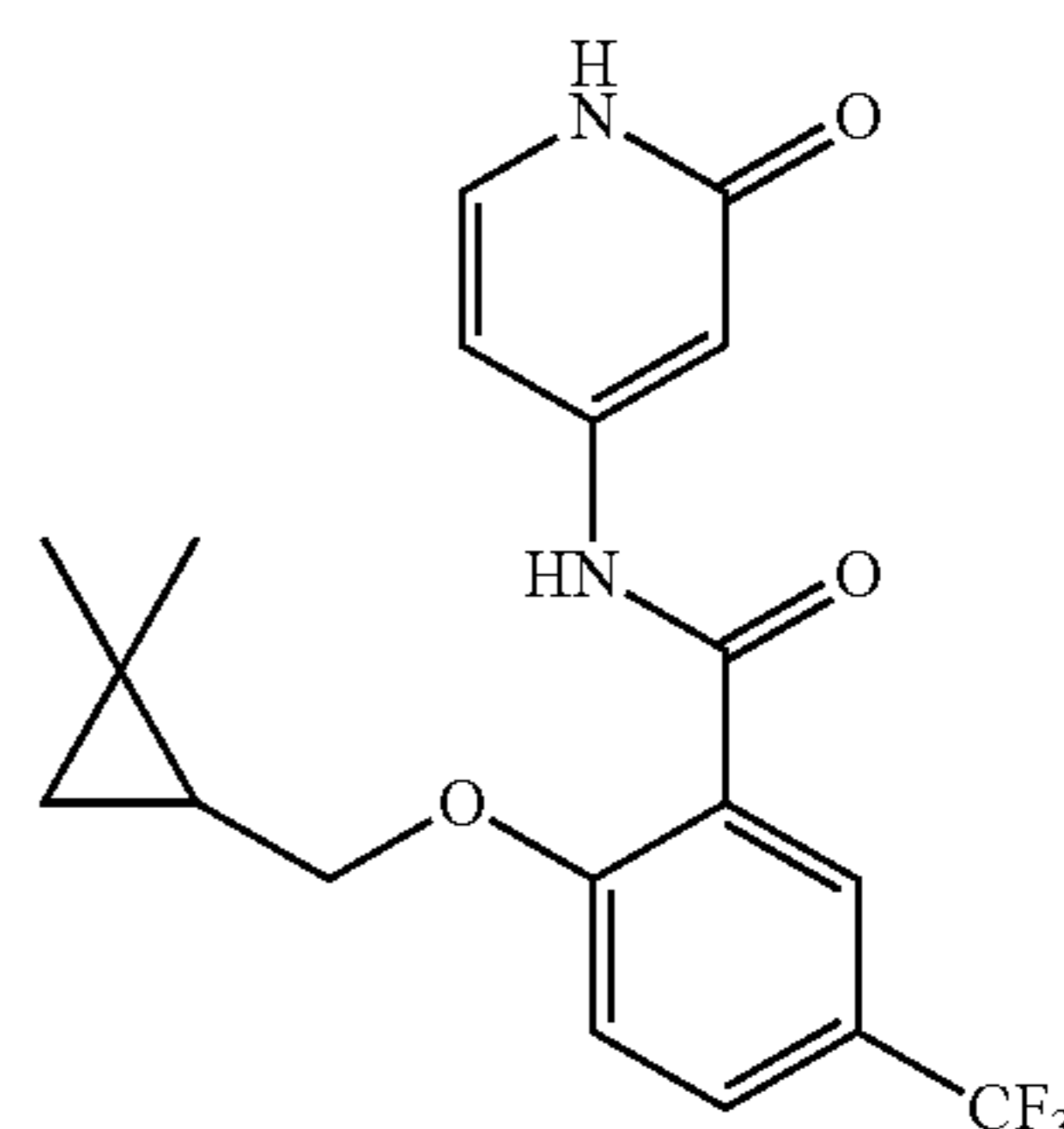
2-((2,2-dimethylcyclopropyl)methoxy)-N-(2-oxo-1,2-dihydropyridin-4-yl)-5-(trifluoromethyl)benzamide
