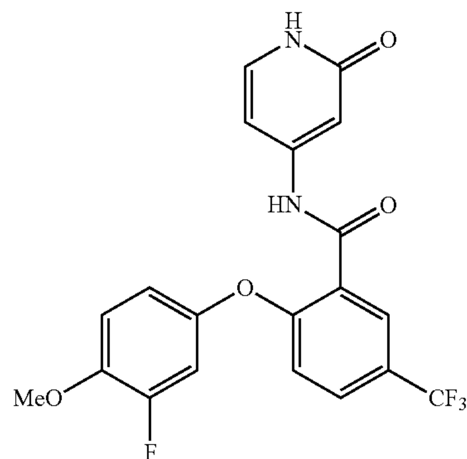
2-(3-fluoro-4-methoxyphenoxy)-N-(2-oxo-1,2-dihydropyridin-4-yl)-5-(trifluoromethyl)benzamide
