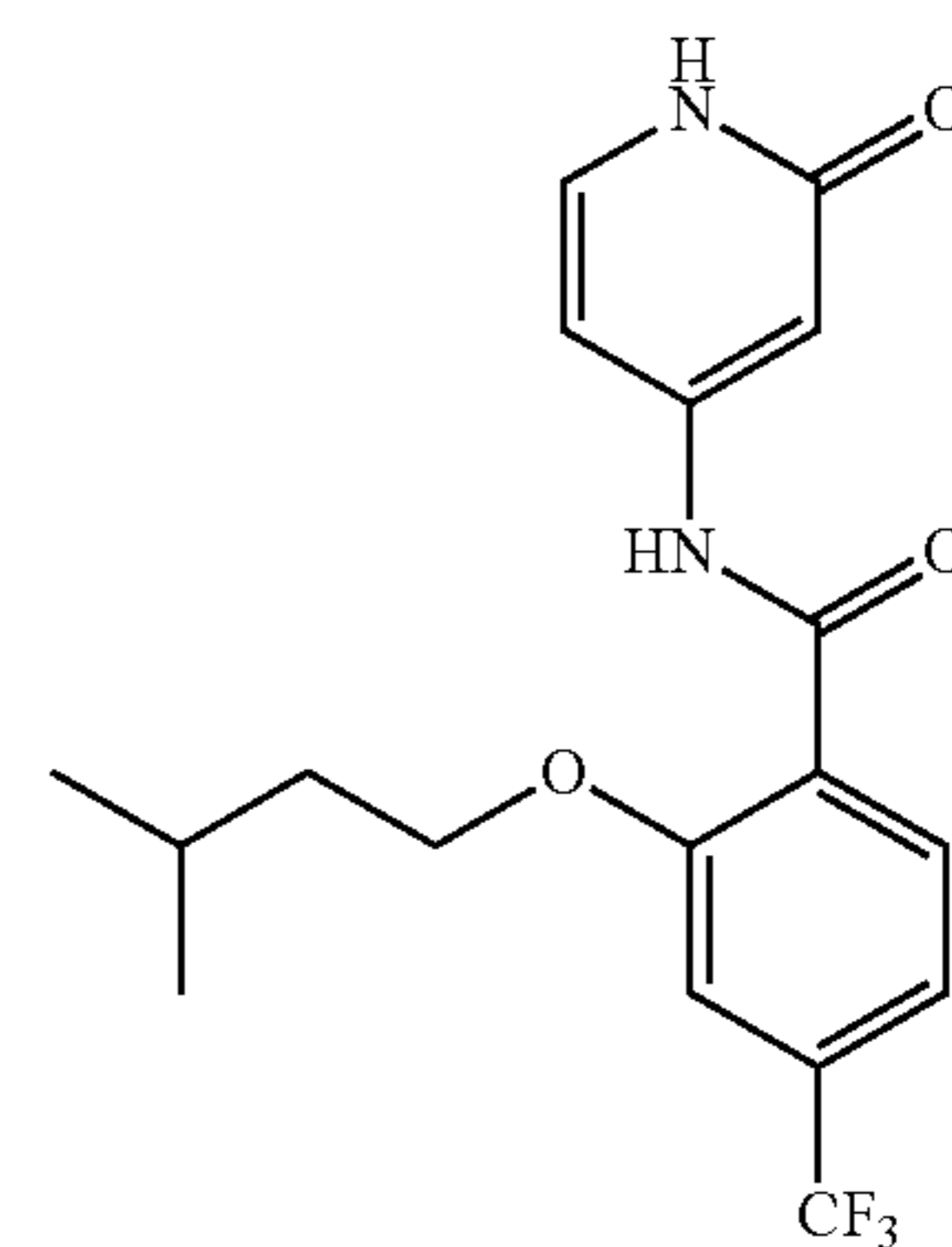
2-(isopentyloxy)-N-(2-oxo-1,2-dihydropyridin-4-yl)-4-(trifluoromethyl)benzamide
