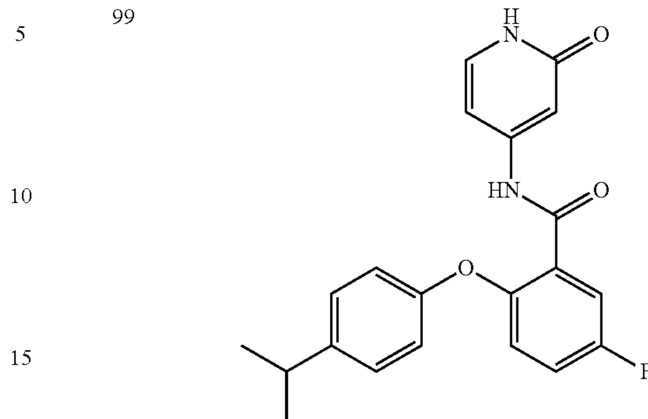
5-fluoro-2-(4-isopropylphenoxy)-N-(2-oxo-1,2-dihydropyridin-4-yl)benzamide
