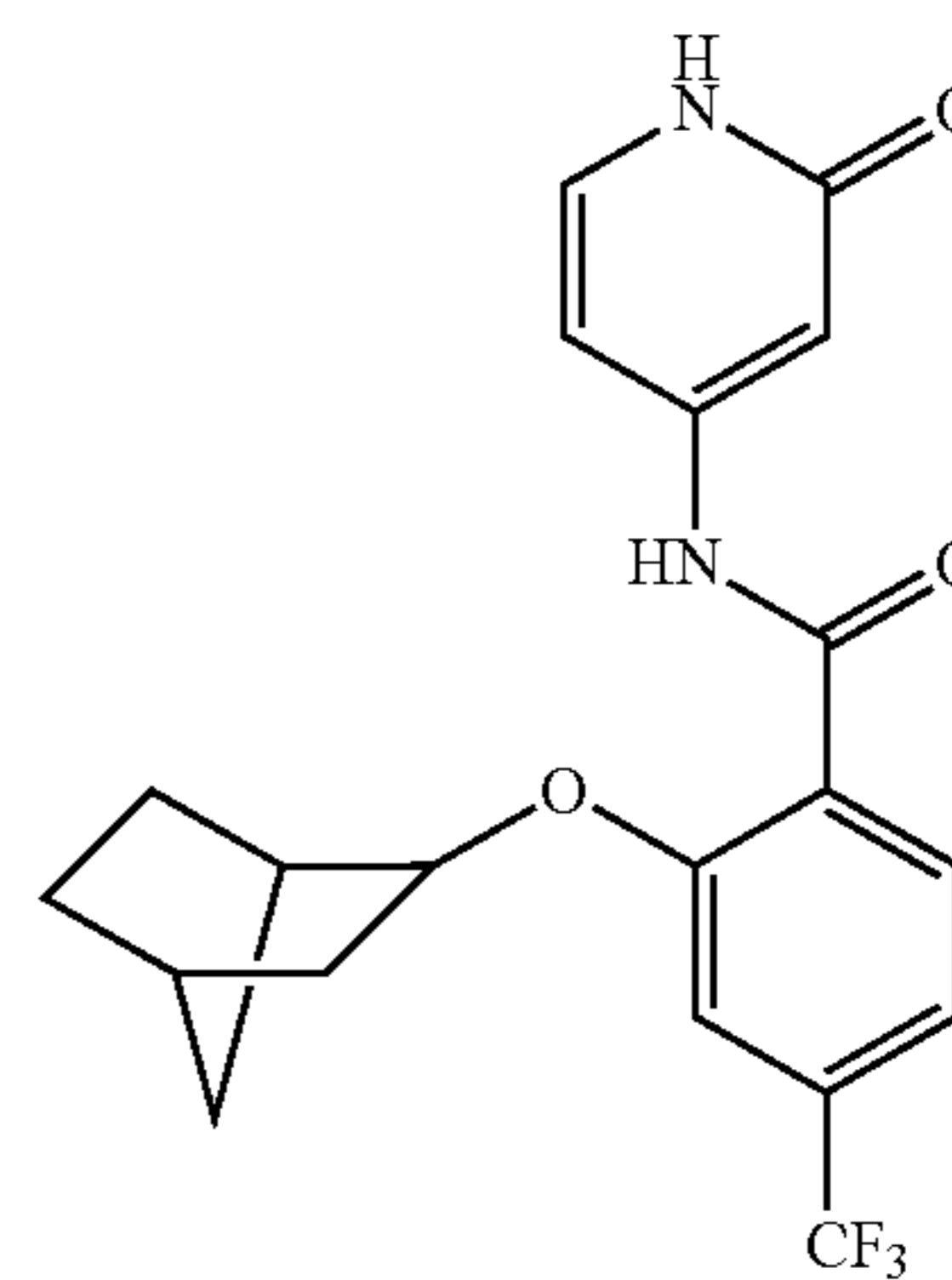
2-(bicyclo[2.2.1]heptan-2-yloxy)-N-(2-oxo-1,2-dihydropyridin-4-yl)-4-(trifluoromethyl)benzamide
