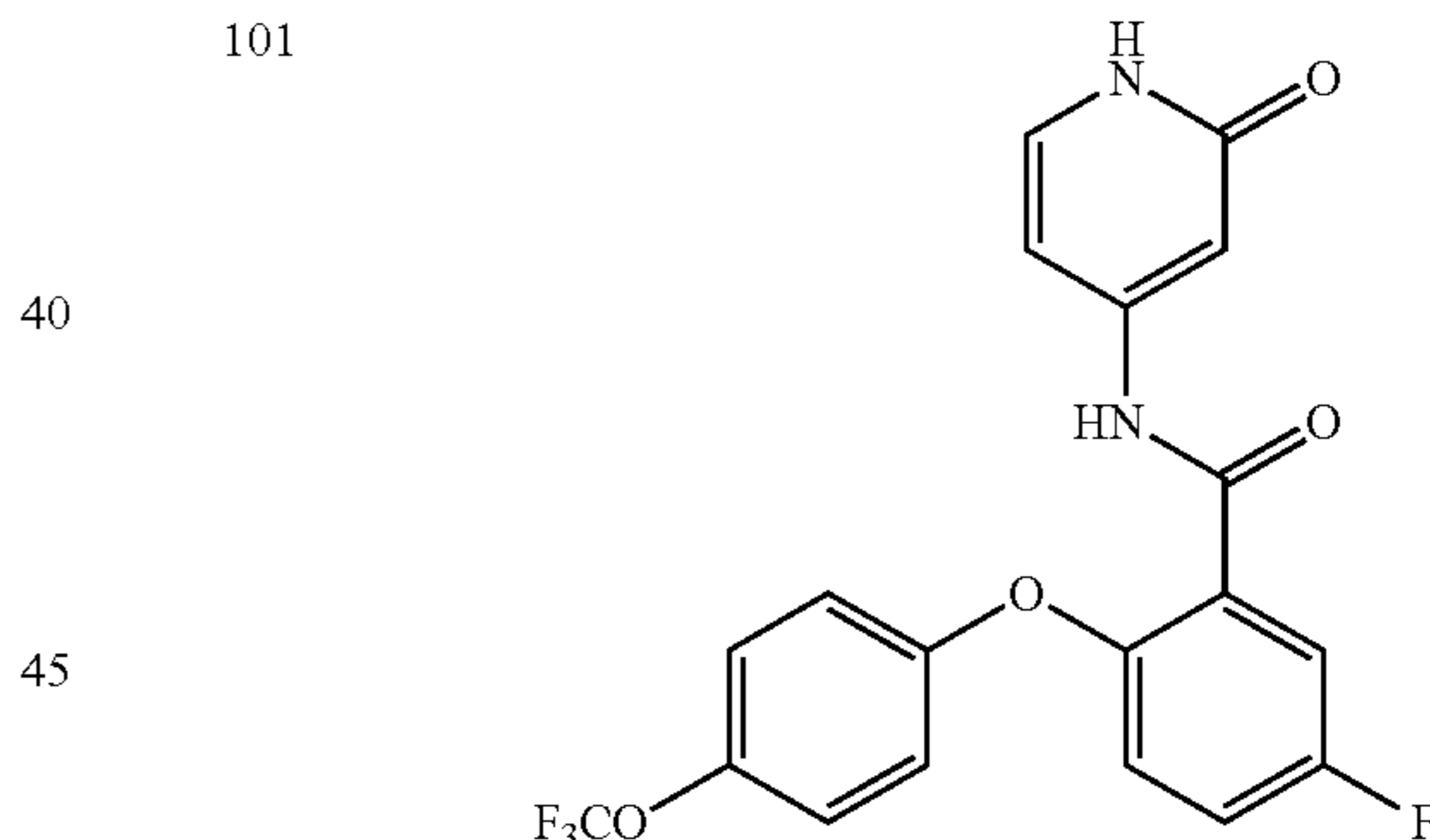
5-fluoro-N-(2-oxo-1,2-dihydropyridin-4-yl)-2-(4-(trifluoromethoxy)phenoxy)benzamide
