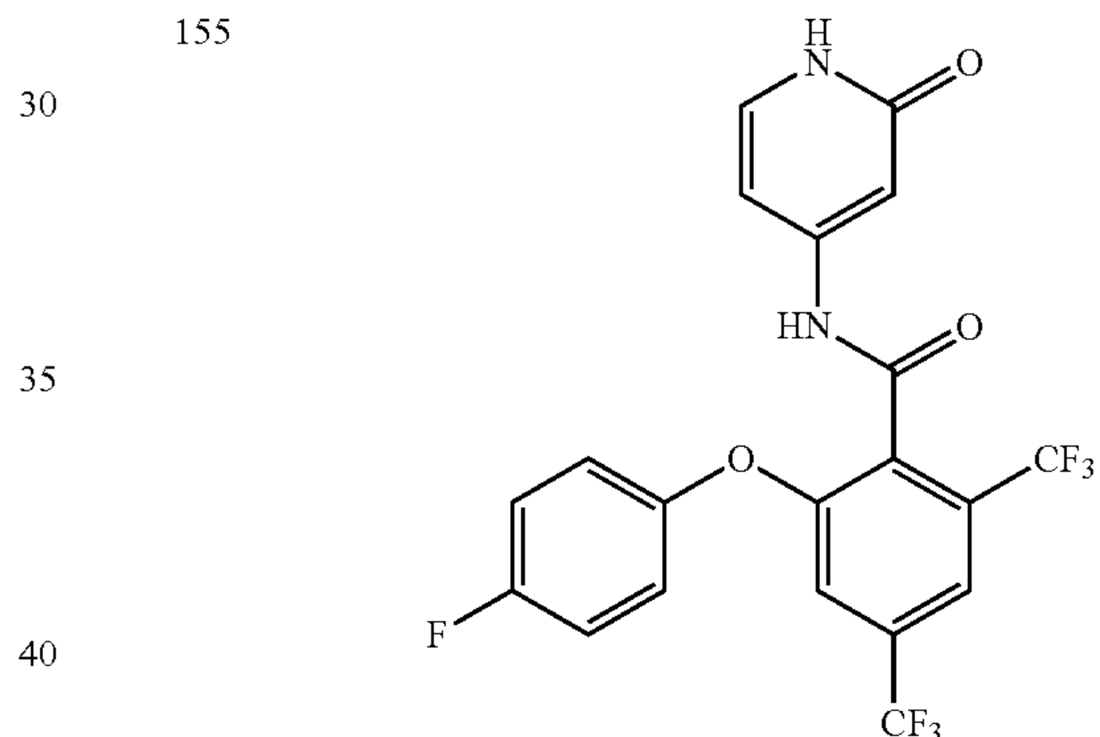
2-(4-fluorophenoxy)-N-(2-oxo-1,2-dihydropyridin-4-yl)-4,6-bis(trifluoromethyl)benzamide
