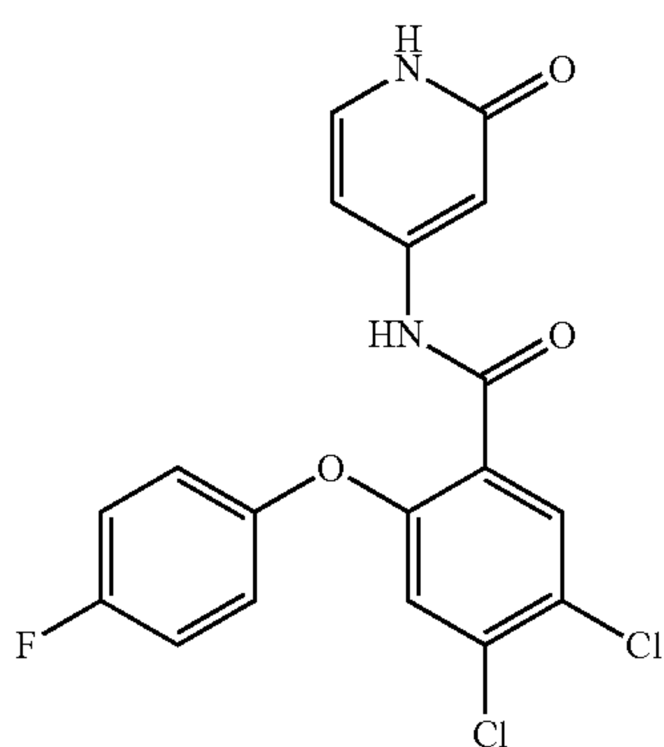
4,5-dichloro-2-(4-fluorophenoxy)-N-(2-oxo-1,2-dihydropyridin-4-yl)benzamide
