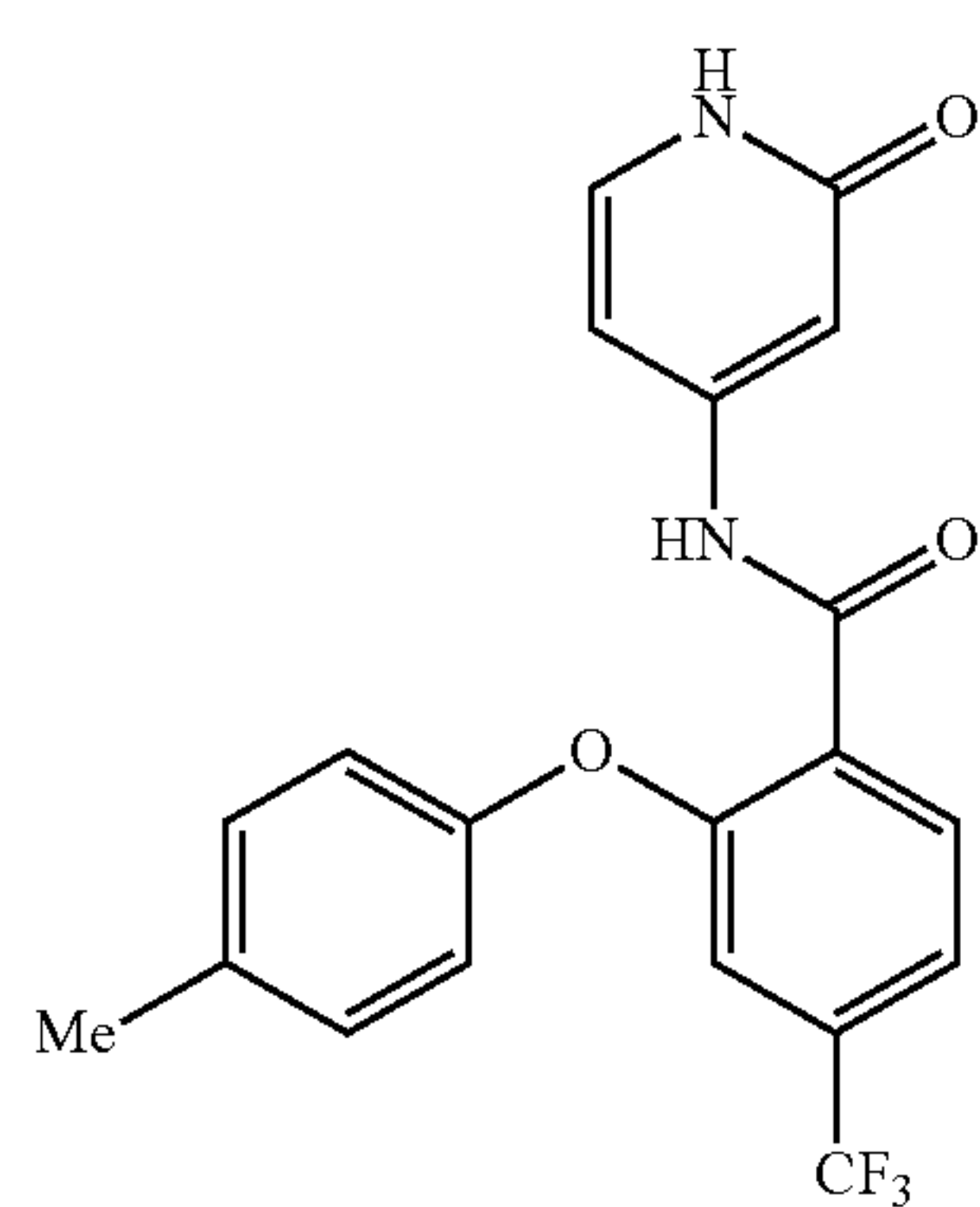
N-(2-oxo-1,2-dihydropyridin-4-yl)-2-(p-tolyloxy)-4-(trifluoromethyl)benzamide
