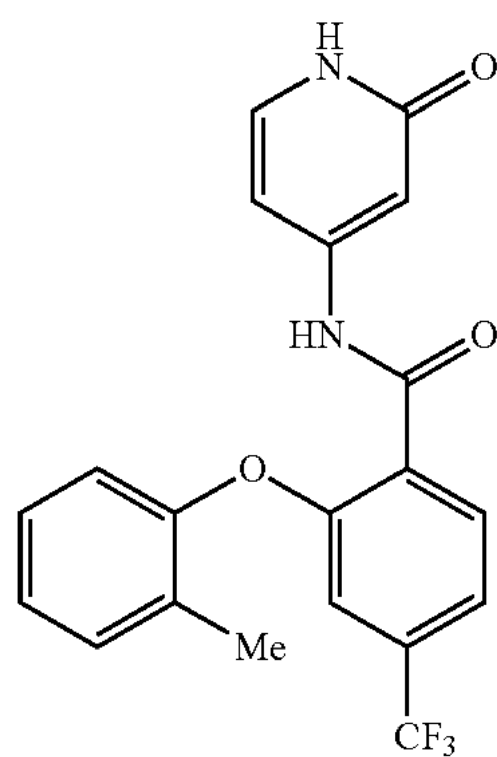
N-(2-oxo-1,2-dihydropyridin-4-yl)-2-(o-tolyloxy)-4-(trifluoromethyl)benzamide
