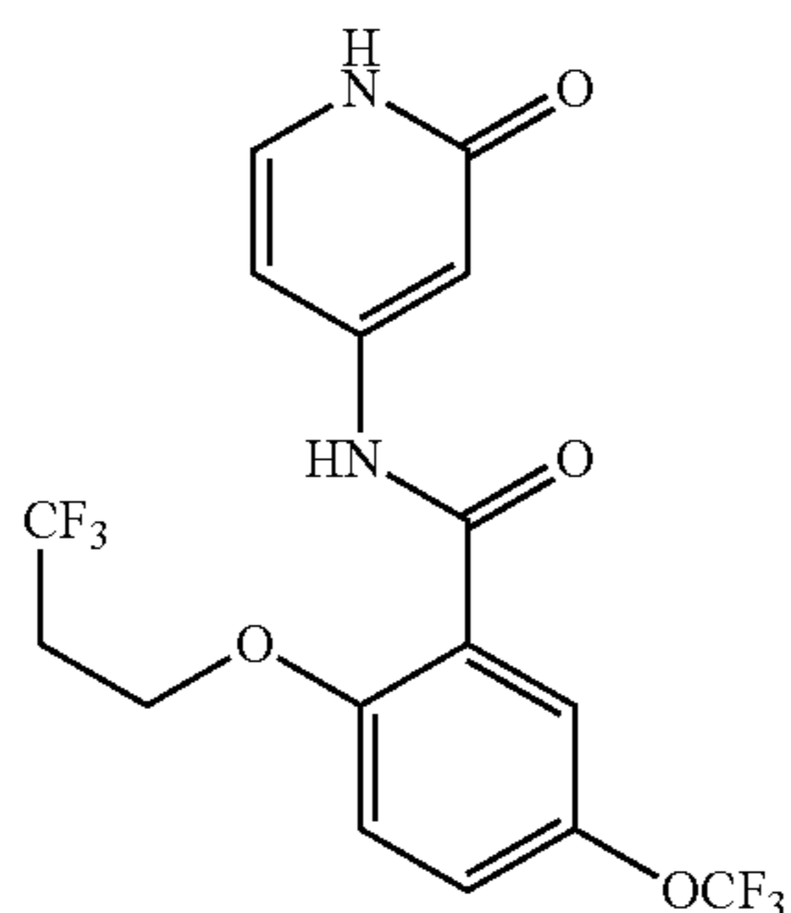
N-(2-oxo-1,2-dihydropyridin-4-yl)-5-(trifluoromethoxy)-2-(3,3,3-trifluoropropoxy)benzamide
