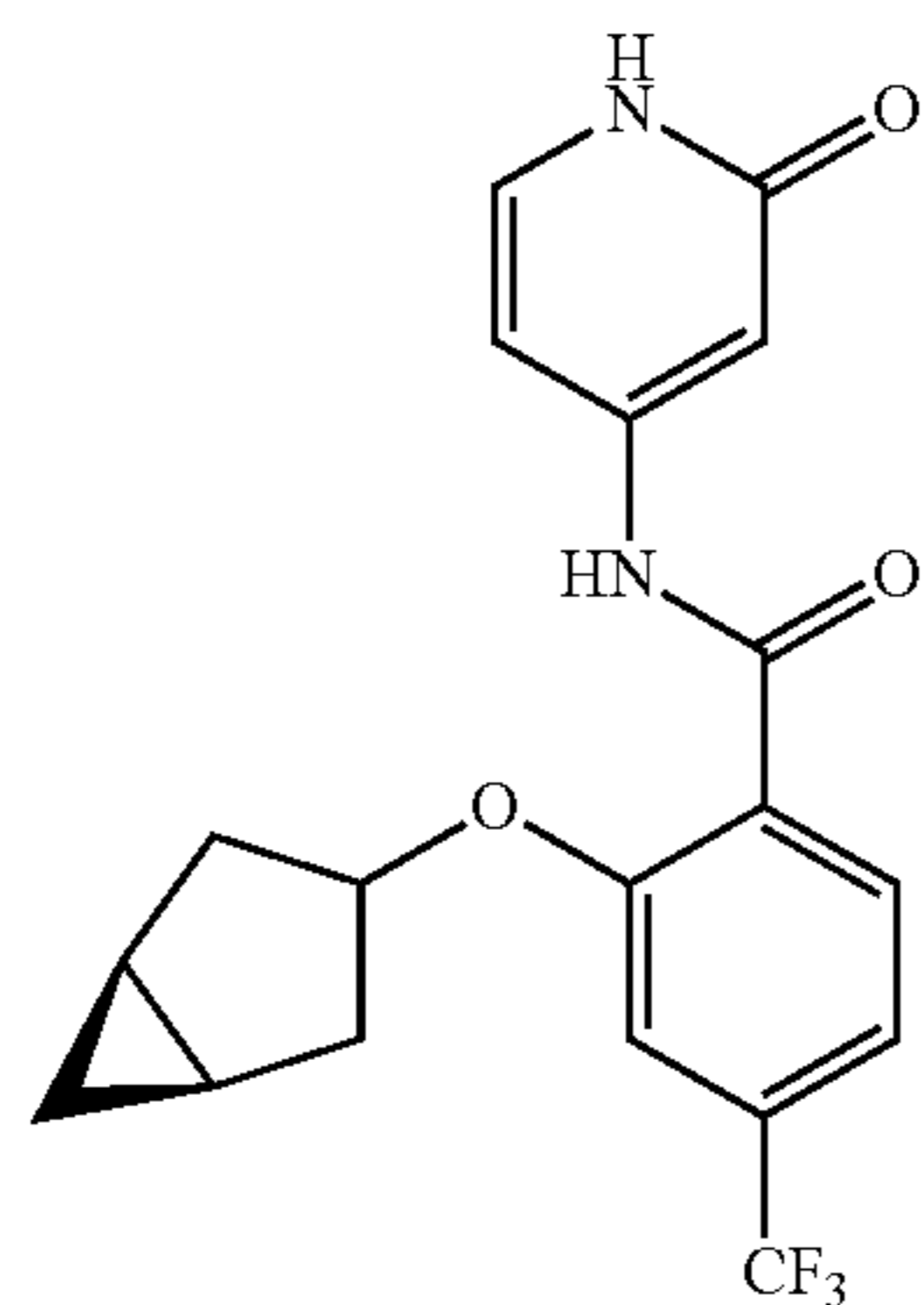
2-((1R,5S)-bicyclo[3.1.0]hexan-3-yloxy)-N-(2-oxo-1,2-dihydropyridin-4-yl)-4-(trifluoromethyl)benzamide
