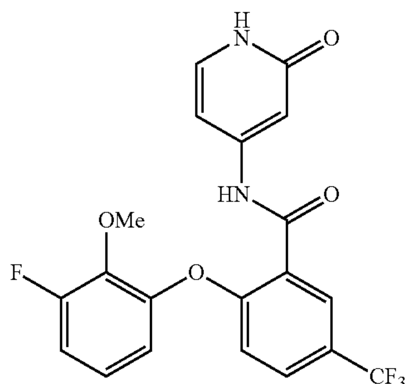
2-(3-fluoro-2-methoxyphenoxy)-N-(2-oxo-1,2-dihydropyridin-4-yl)-5-(trifluoromethyl)benzamide
