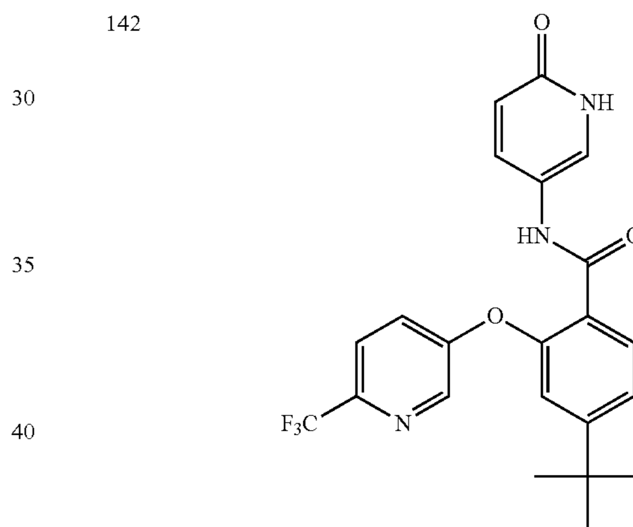
4-(tert-butyl)-N-(6-oxo-1,6-dihydropyridin-3-yl)-2-((6-(trifluoromethyl)pyridin-3-yl)oxy)benzamide
