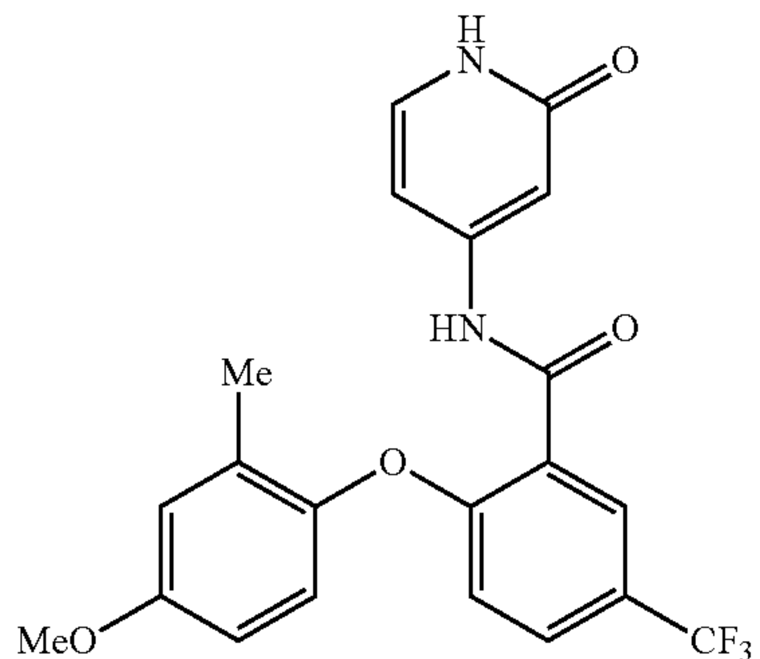
2-(4-methoxy-2-methylphenoxy)-N-(2-oxo-1,2-dihydropyridin-4-yl)-5-(trifluoromethyl)benzamide
