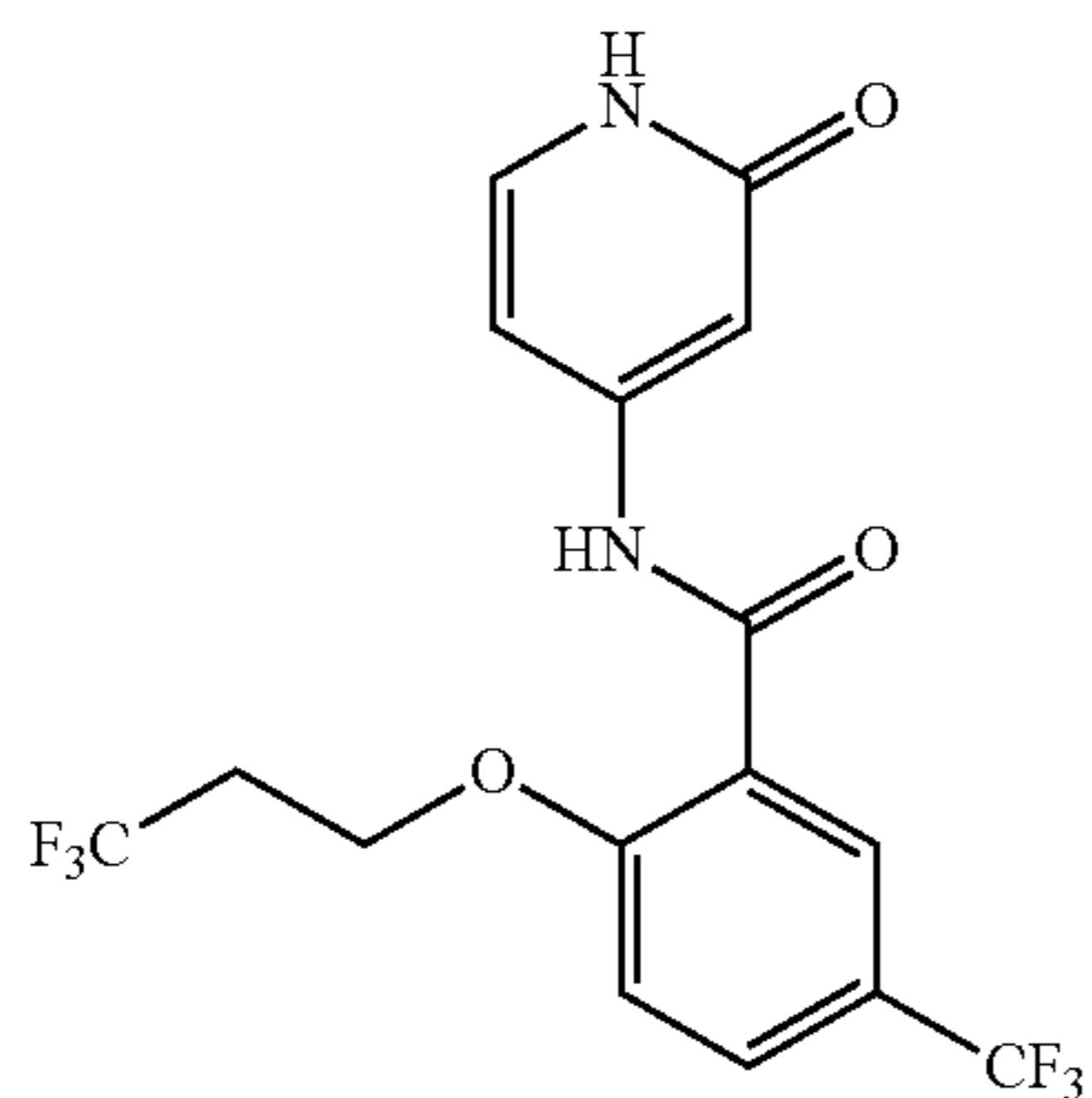
N-(2-oxo-1,2-dihydropyridin-4-yl)-5-(trifluoromethyl)-2-(3,3,3-trifluoropropoxy)benzamide
