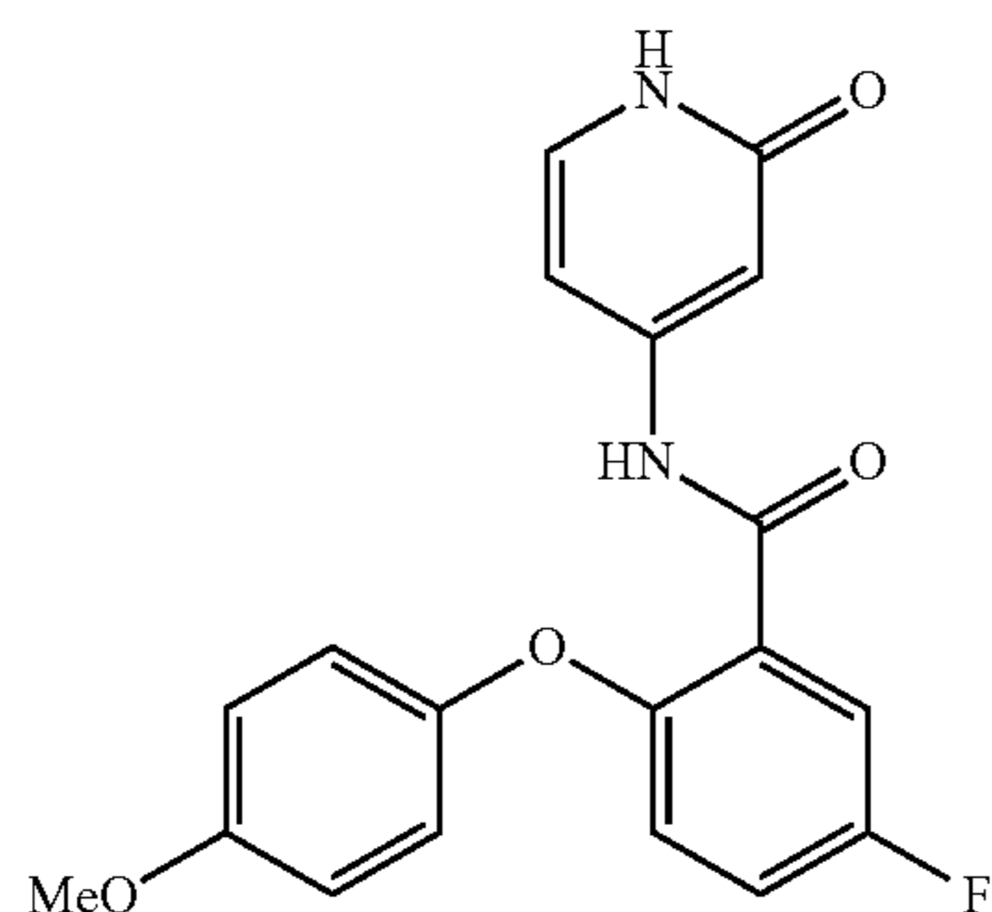
5-fluoro-2-(4-methoxyphenoxy)-N-(2-oxo-1,2-dihydropyridin-4-yl)benzamide
