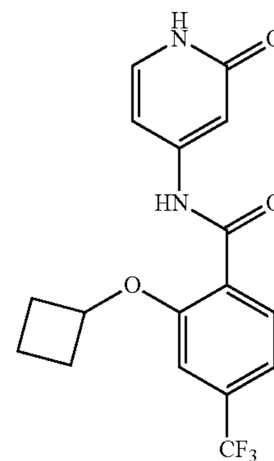
2-cyclobutoxy-N-(2-oxo-1,2-dihydropyridin-4-yl)-4-(trifluoromethyl)benzamide
