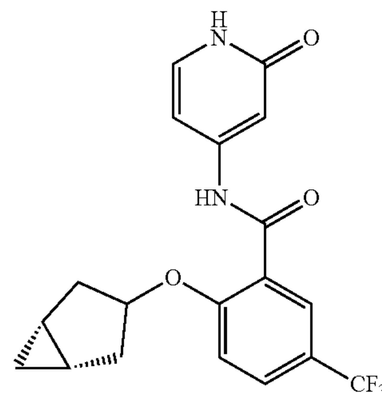
2-((1R,5S)-bicyclo[3.1.0]hexan-3-yloxy)-N-(2-oxo-1,2-dihydropyridin-4-yl)-5-(trifluoromethyl)benzamide
