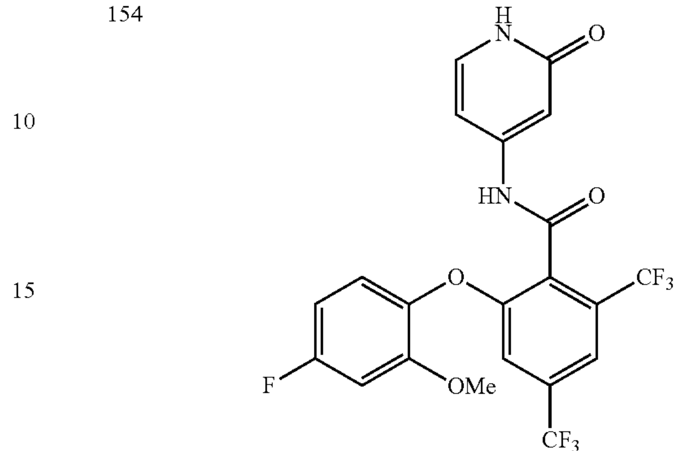
2-(4-fluoro-2-methoxyphenoxy)-N-(2-oxo-1,2-dihydropyridin-4-yl)-4,6-bis(trifluoromethyl)benzamide
