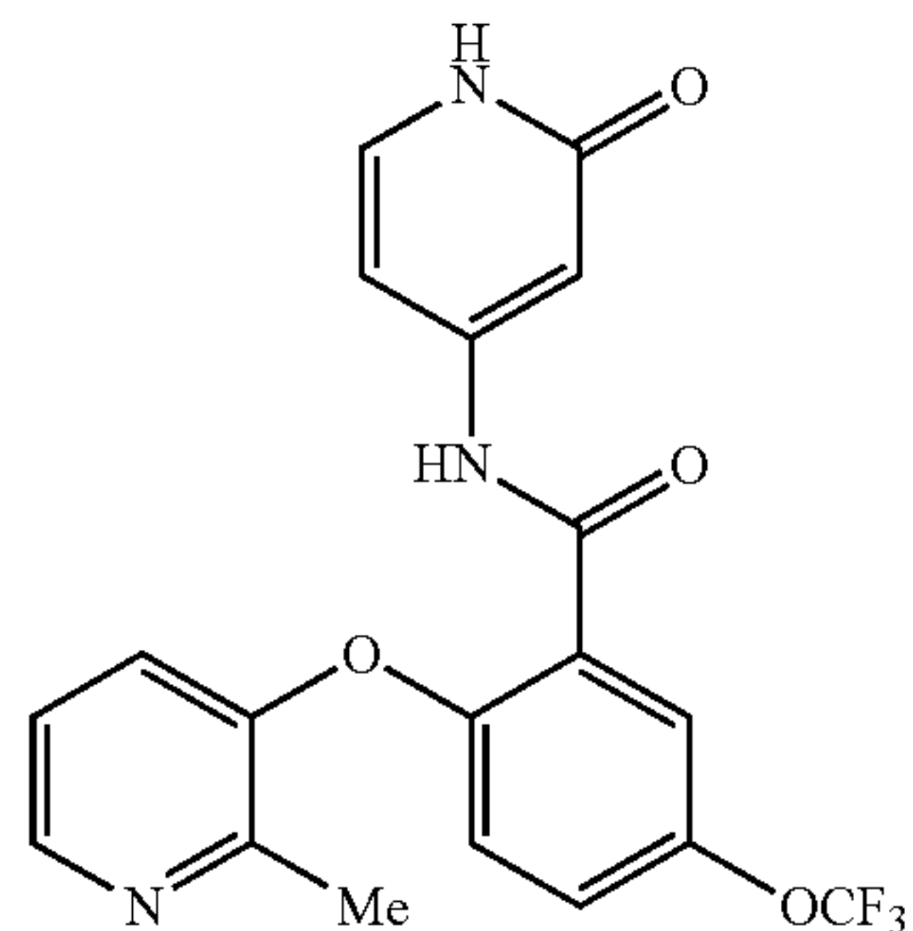
2-((2-methylpyridin-3-yl)oxy)-N-(2-oxo-1,2-dihydropyridin-4-yl)-5-(trifluoromethoxy)benzamide
