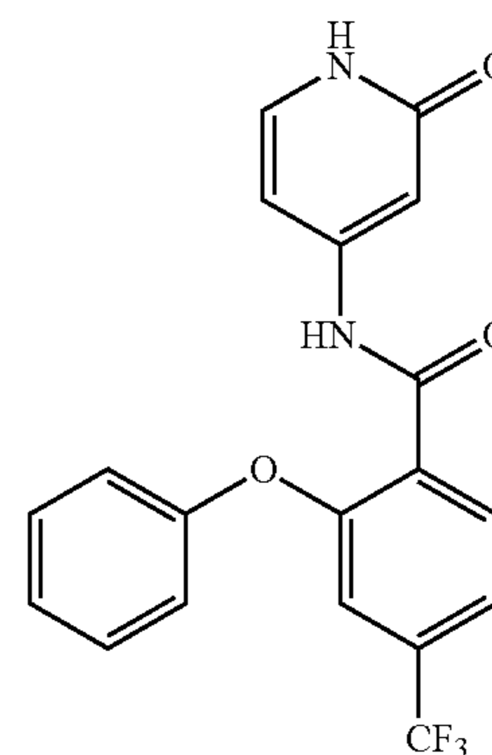
N-(2-oxo-1,2-dihydropyridin-4-yl)-2-phenoxy-4-(trifluoromethyl)benzamide
