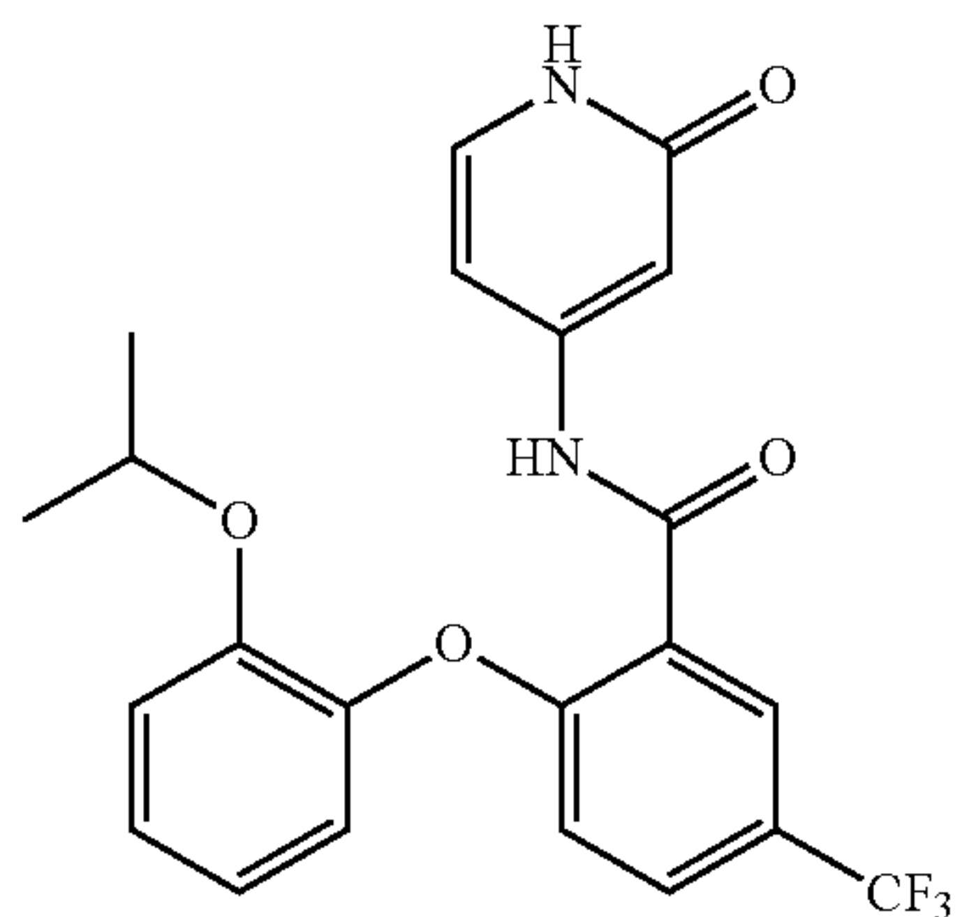
2-(2-isopropoxyphenoxy)-N-(2-oxo-1,2-dihydropyridin-4-yl)-5-(trifluoromethyl)benzamide
