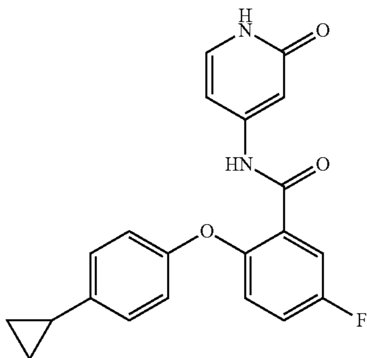
2-(4-cyclopropylphenoxy)-5-fluoro-N-(2-oxo-1,2-dihydropyridin-4-yl)benzamide
