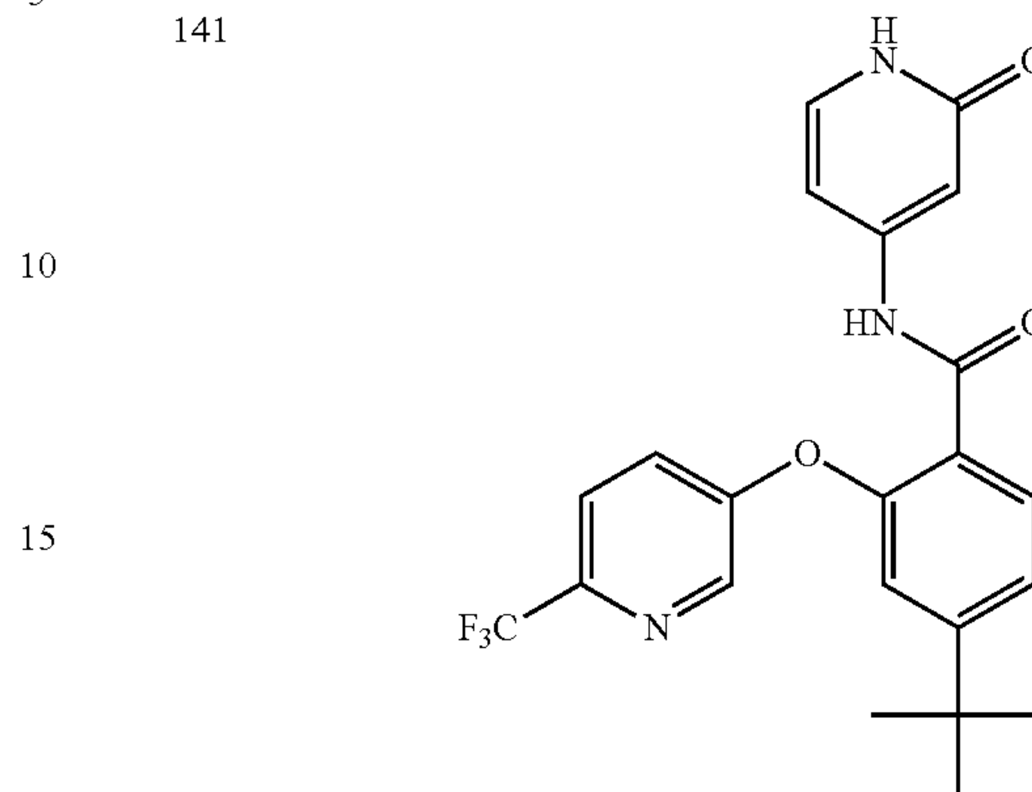
4-(tert-butyl)-N-(2-oxo-1,2-dihydropyridin-4-yl)-2-((6-(trifluoromethyl)pyridin-3-yl)oxy)benzamide
