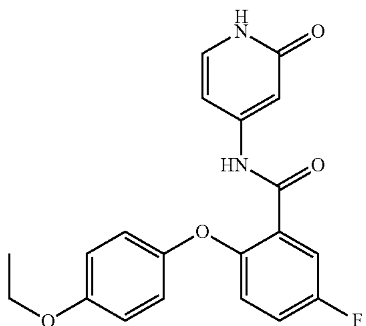
2-(4-ethoxyphenoxy)-5-fluoro-N-(2-oxo-1,2-dihydropyridin-4-yl)benzamide
