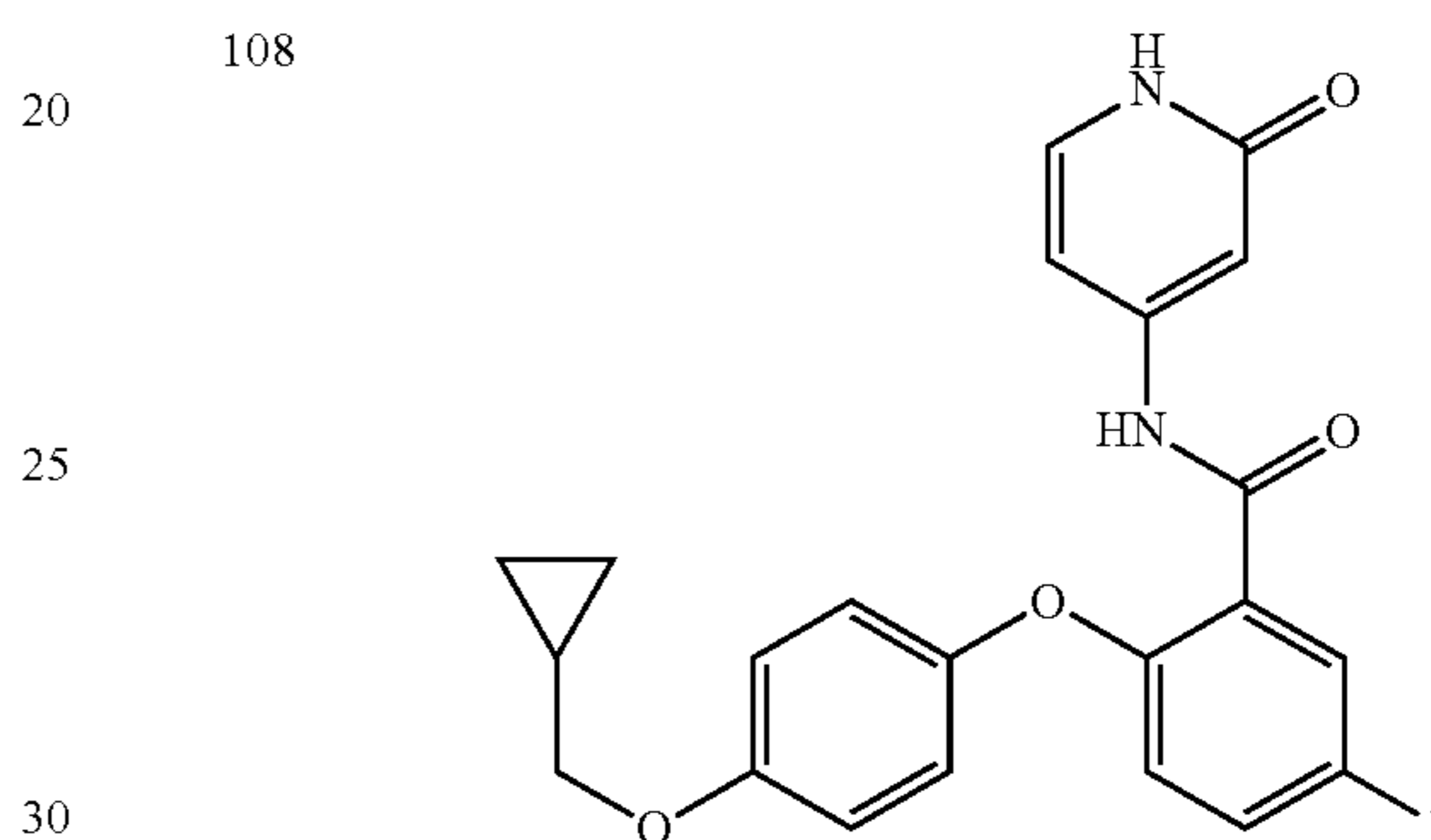
2-(4-(cyclopropylmethoxy)phenoxy)-5-fluoro-N-(2-oxo-1,2-dihydropyridin-4-yl)benzamide
