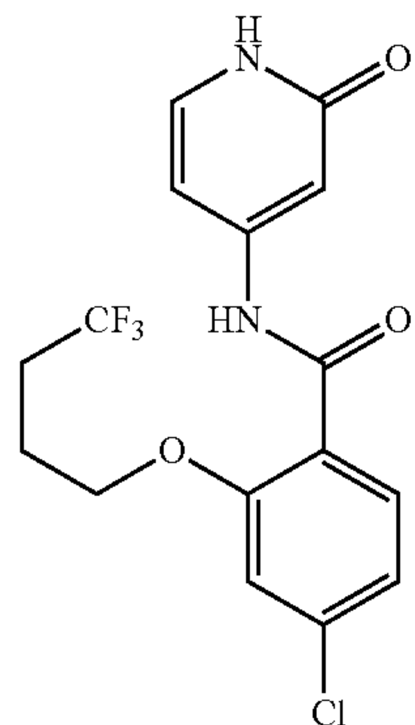
4-chloro-N-(2-oxo-1,2-dihydropyridin-4-yl)-2-(4,4,4-trifluorobutoxy)benzamide
