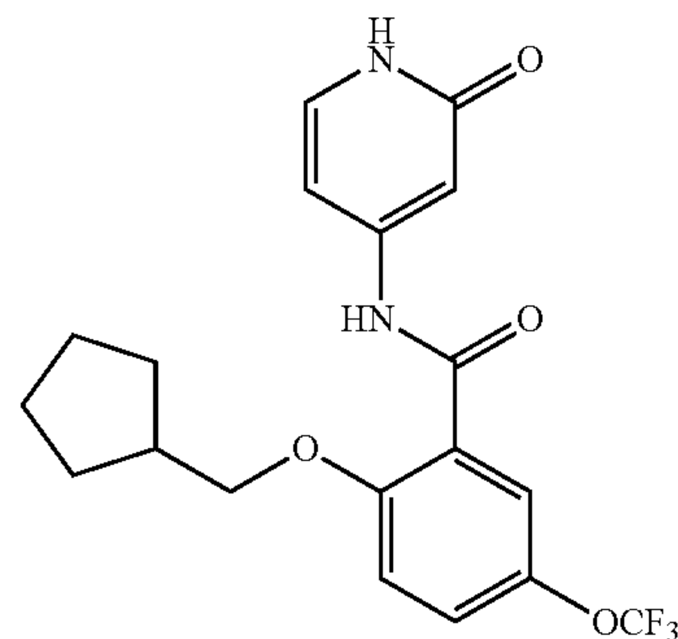
2-(cyclopentylmethoxy)-N-(2-oxo-1,2-dihydropyridin-4-yl)-5-(trifluoromethoxy)benzamide
