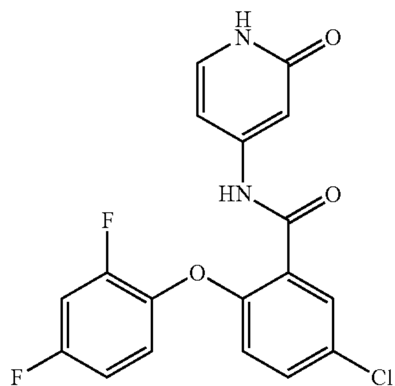
5-chloro-2-(2,4-difluorophenoxy)-N-(2-oxo-1,2-dihydropyridin-4-yl)benzamide
