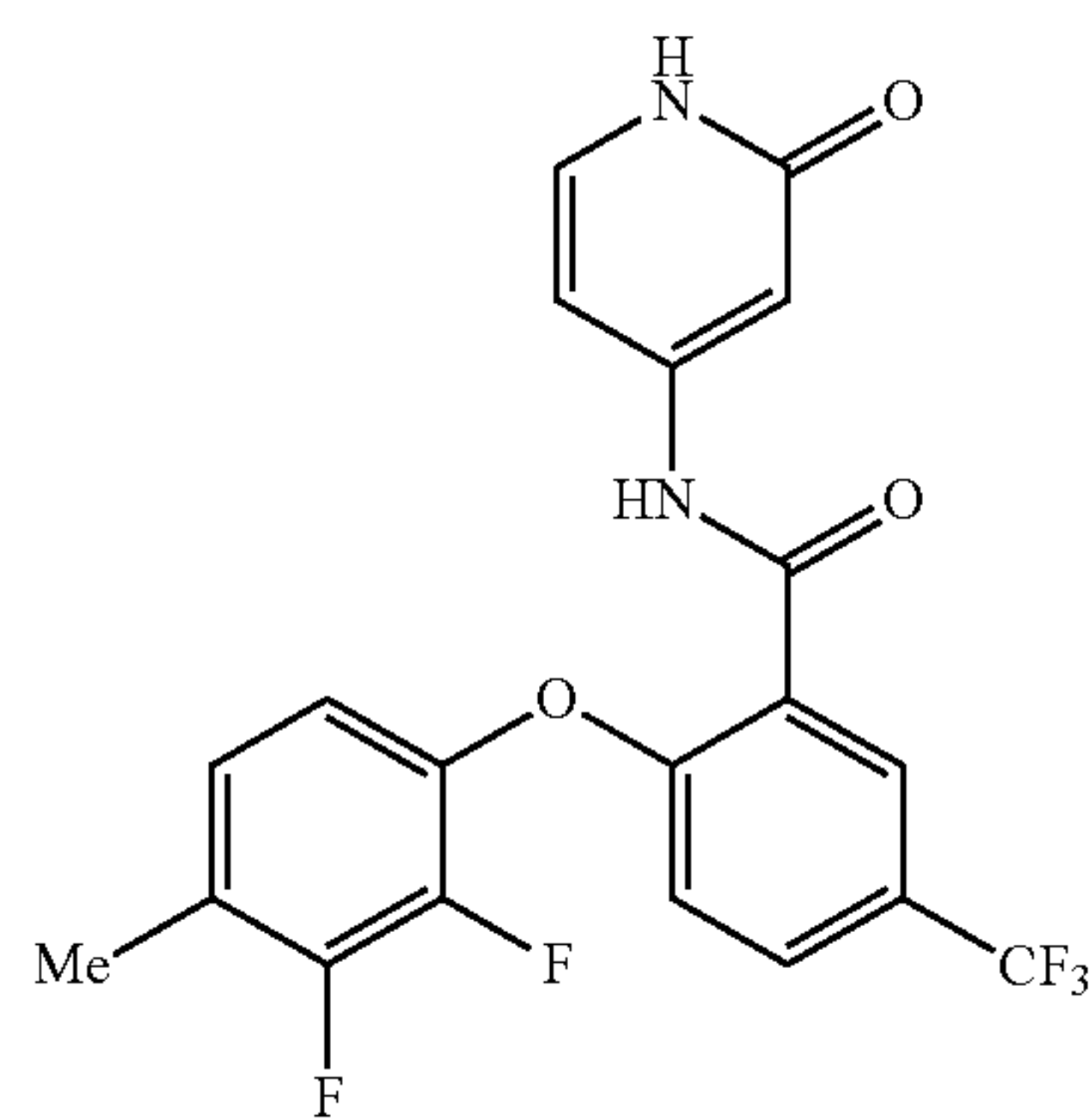
2-(2,3-difluoro-4-methylphenoxy)-N-(2-oxo-1,2-dihydropyridin-4-yl)-5-(trifluoromethyl)benzamide
