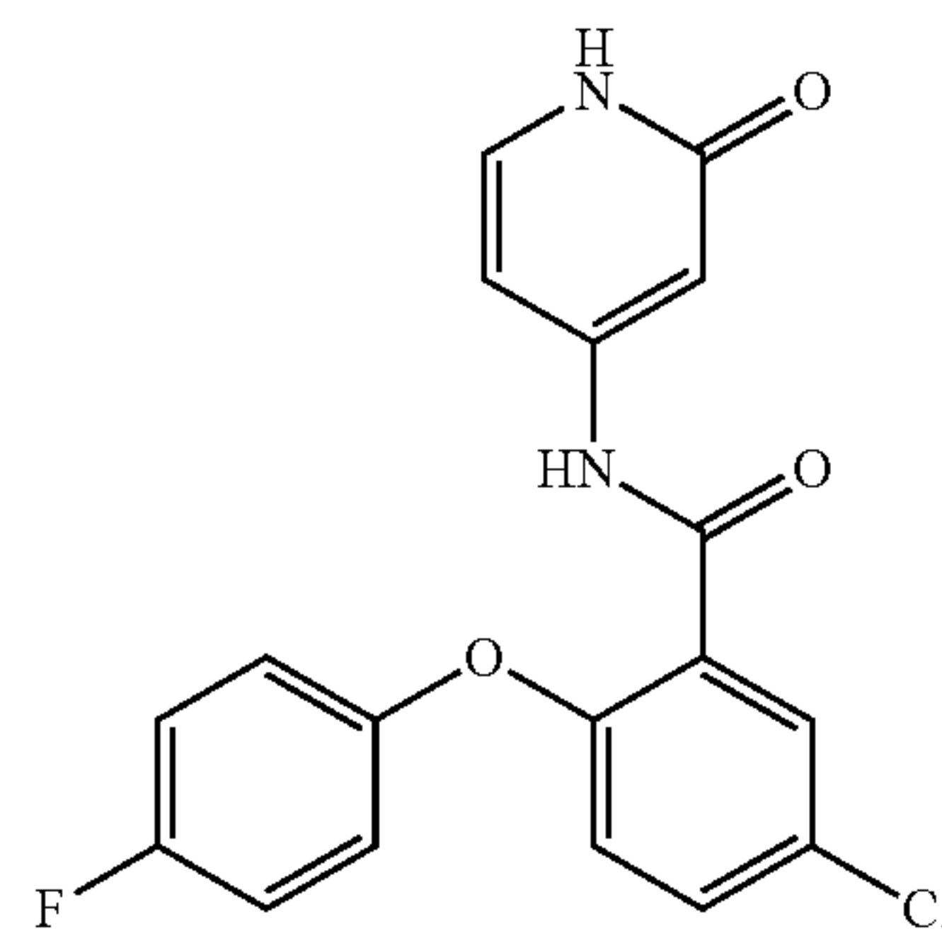
5-chloro-2-(4-fluorophenoxy)-N-(2-oxo-1,2-dihydropyridin-4-yl)benzamide
