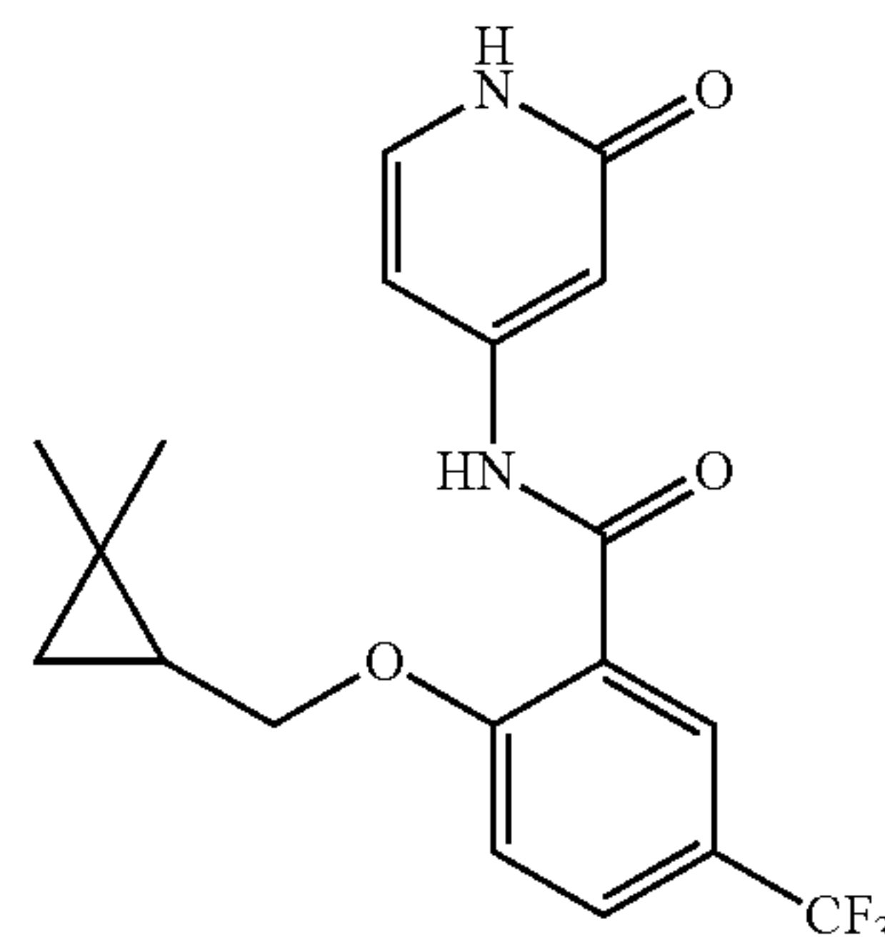
2-((2,2-dimethylcyclopropyl)methoxy)-N-(2-oxo-1,2-dihydropyridin-4-yl)-5-(trifluoromethyl)benzamide
