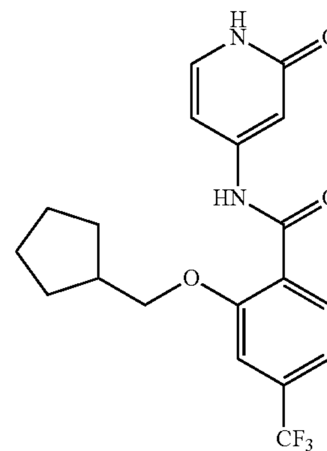
2-(cyclopentylmethoxy)-N-(2-oxo-1,2-dihydropyridin-4-yl)-4-(trifluoromethyl)benzamide
