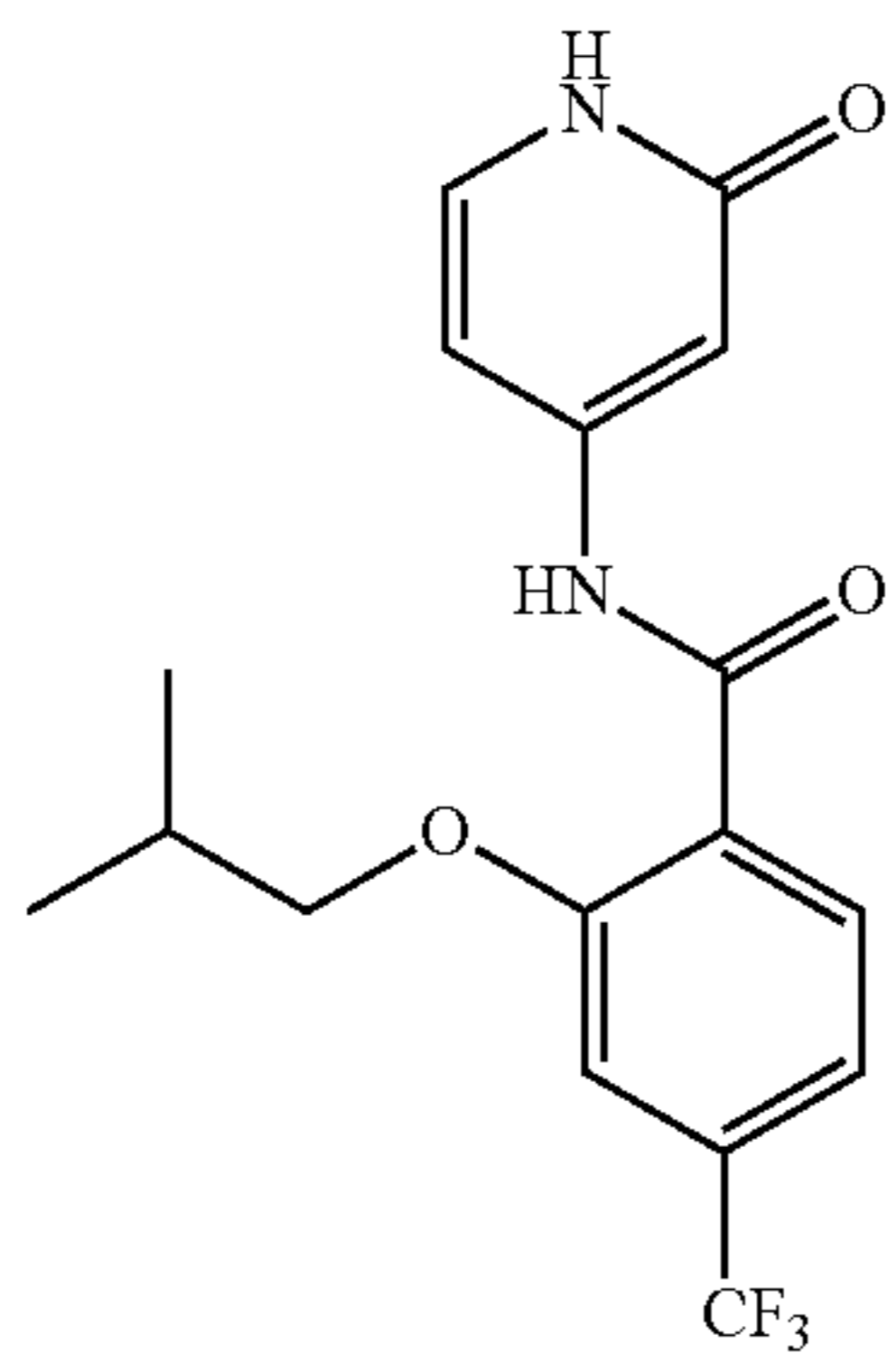
2-isobutoxy-N-(2-oxo-1,2-dihydropyridin-4-yl)-4-(trifluoromethyl)benzamide
