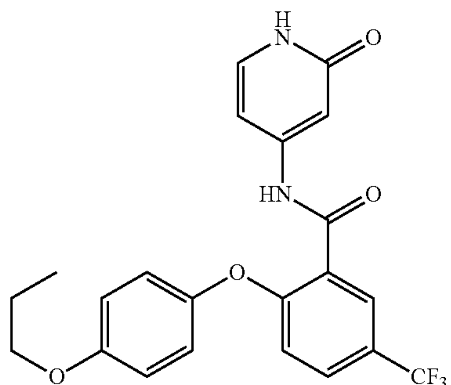
N-(2-oxo-1,2-dihydropyridin-4-yl)-2-(4-propoxyphenoxy)-5-(trifluoromethyl)benzamide
