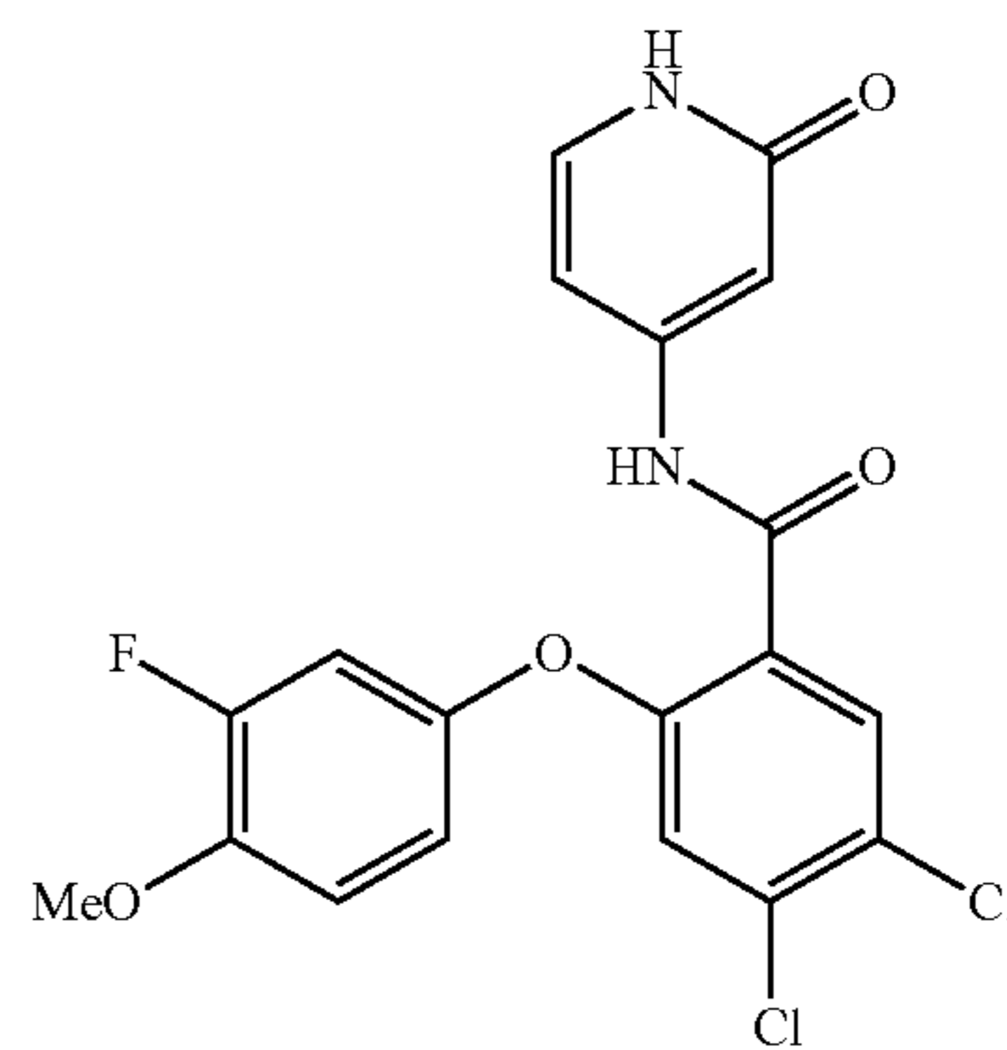
4,5-dichloro-2-(3-fluoro-4-methoxyphenoxy)-N-(2-oxo-1,2-dihydropyridin-4-yl)benzamide
