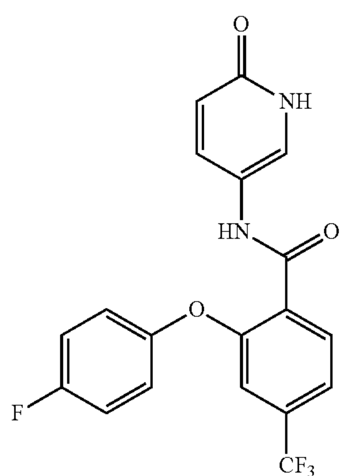
2-(4-fluorophenoxy)-N-(6-oxo-1,6-dihydropyridin-3-yl)-4-(trifluoromethyl)benzamide
