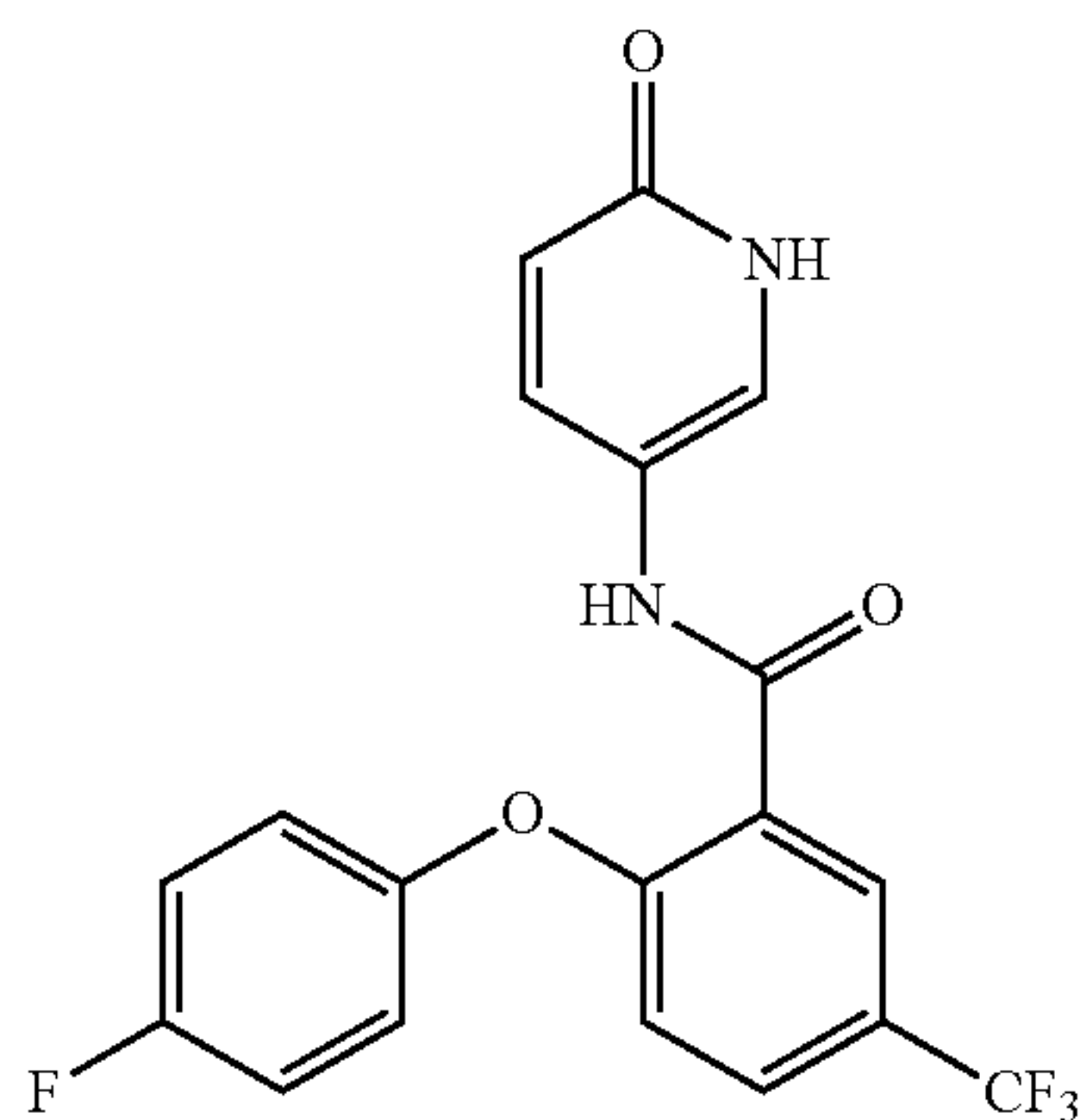
2-(4-fluorophenoxy)-N-(6-oxo-1,6-dihydropyridin-3-yl)-5-(trifluoromethyl)benzamide
