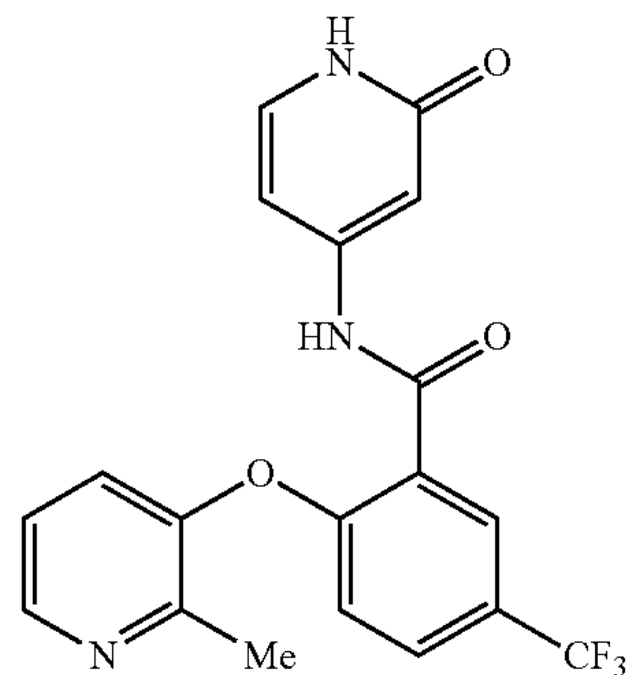
2-(2-methylpyridin-3-yl)oxy)-N-(2-oxo-1,2-dihydropyridin-4-yl)-5-(trifluoromethyl)benzamide
