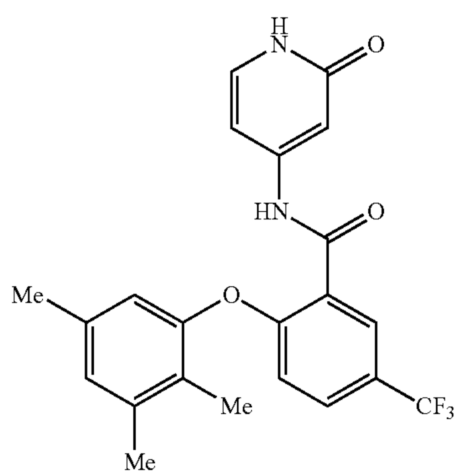
N-(2-oxo-1,2-dihydropyridin-4-yl)-5-(trifluoromethyl)-2-(2,3,5-trimethylphenoxy)benzamide
