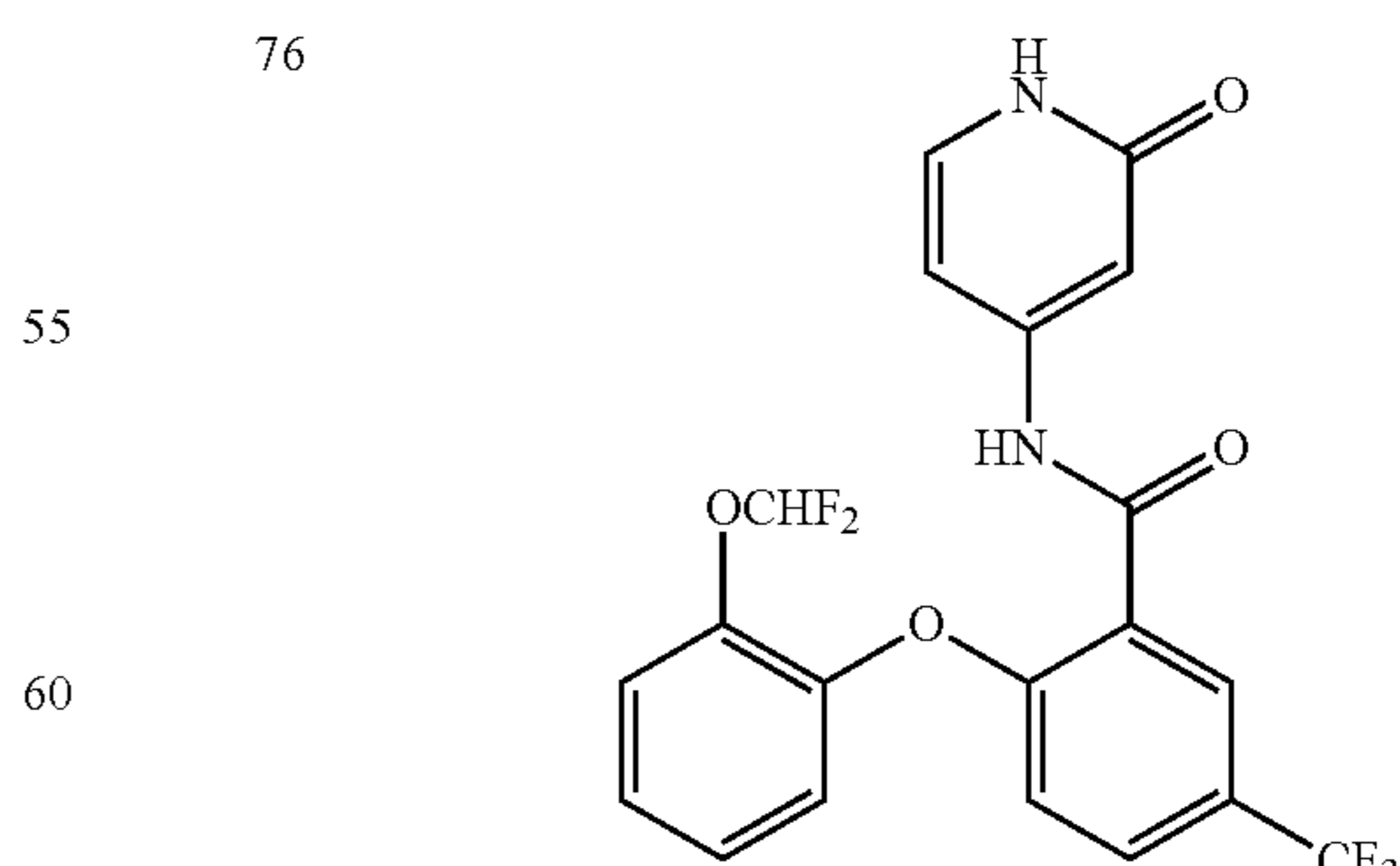
2-(2-(difluoromethoxy)phenoxy)-N-(2-oxo-1,2-dihydropyridin-4-yl)-5-(trifluoromethyl)benzamide
