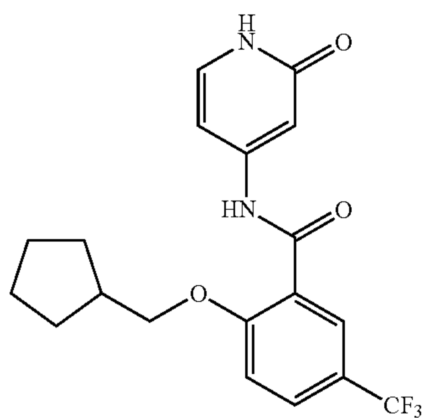
2-(cyclopentylmethoxy)-N-(2-oxo-1,2-dihydropyridin-4-yl)-5-(trifluoromethyl)benzamide
