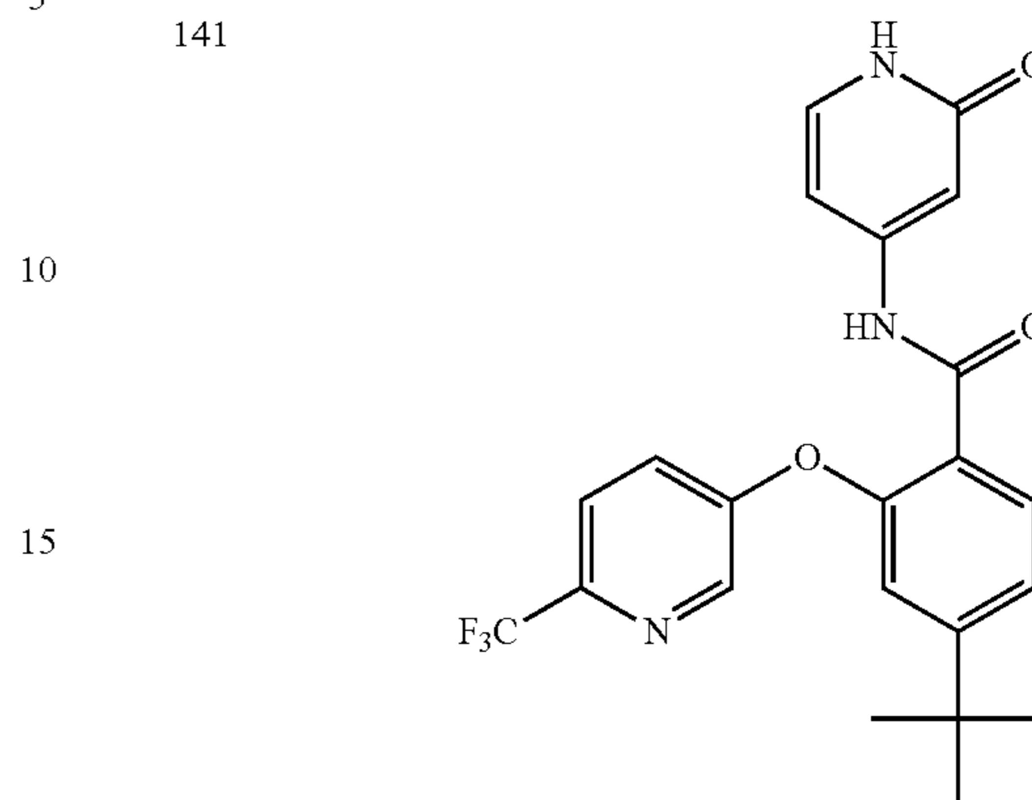
4-(tert-butyl)-N-(2-oxo-1,2-dihydropyridin-4-yl)-2-((6-(trifluoromethyl)pyridin-3-yl)oxy)benzamide
