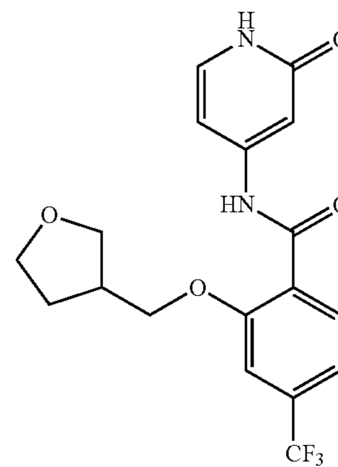
N-(2-oxo-1,2-dihydropyridin-4-yl)-2-((tetrahydrofuran-3-yl)methoxy)-4-(trifluoromethyl)benzamide
