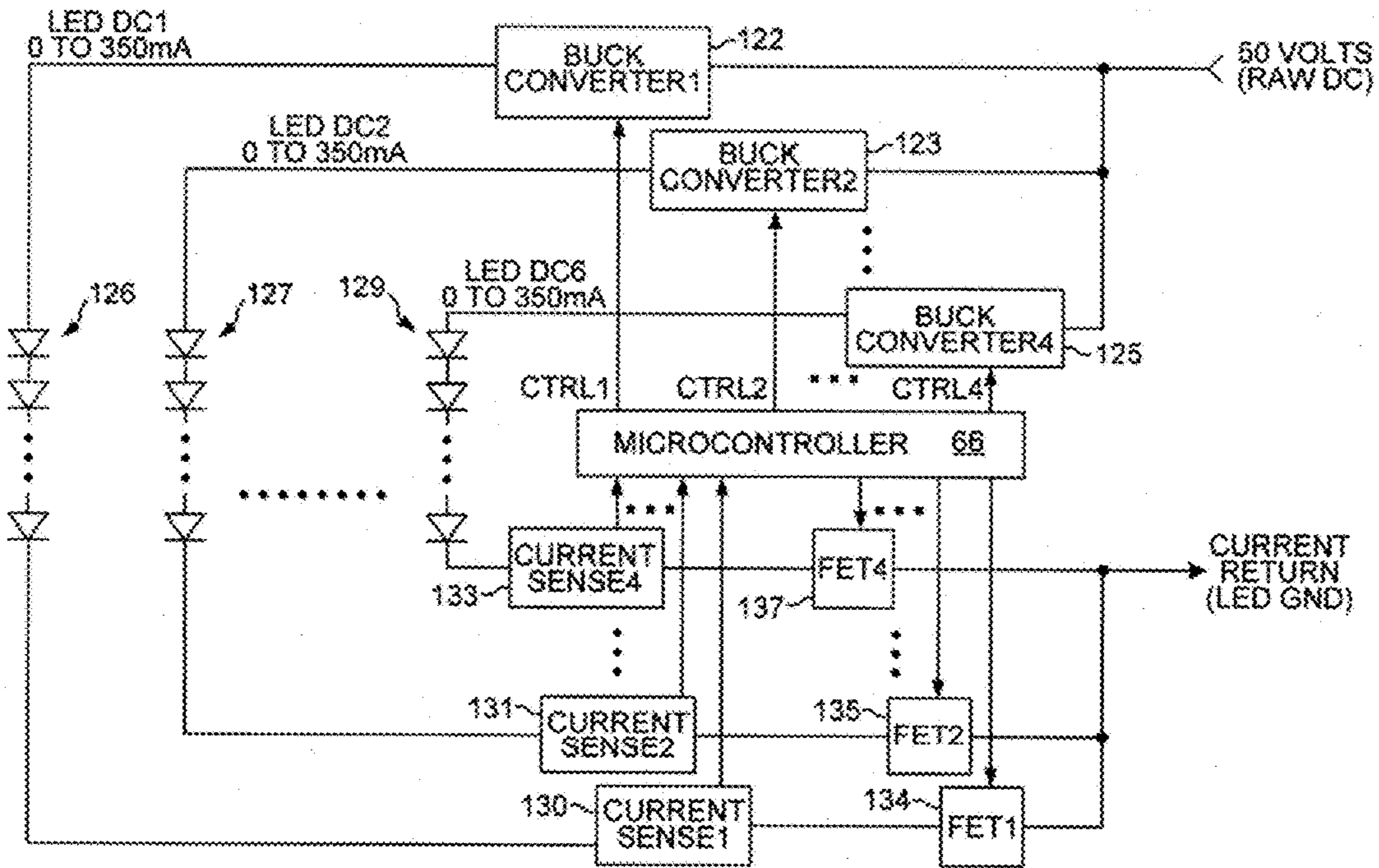
ANOTHER WAY TO DRIVE MULTIPLE STRINGS OF LED JUNCTINS WITH MULTIPLE BUCK CONVERTERS
