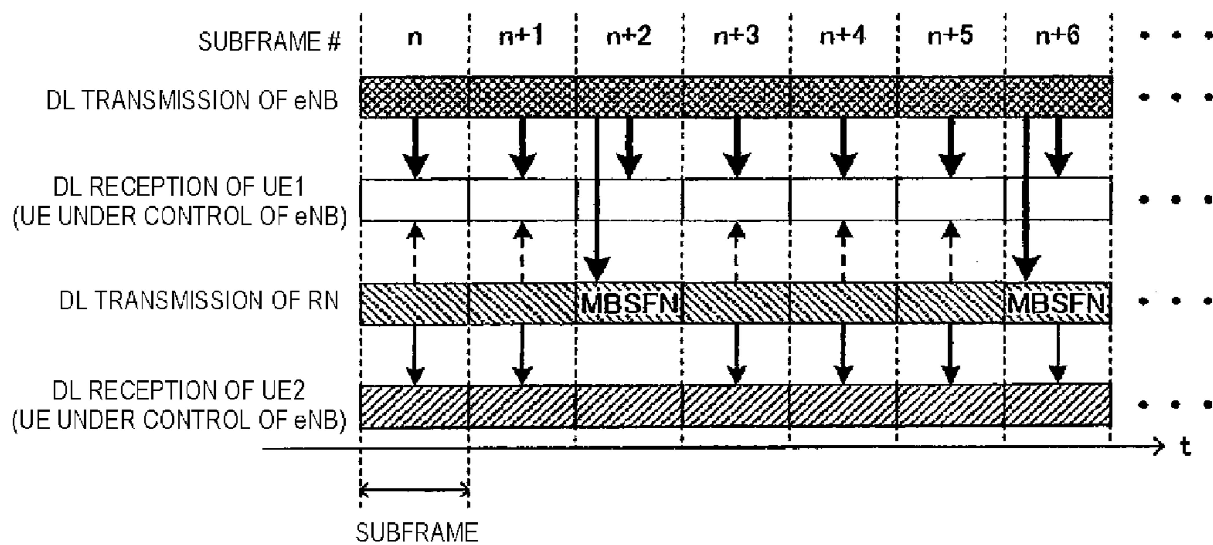
FIG.21 (PRIOR ART)
