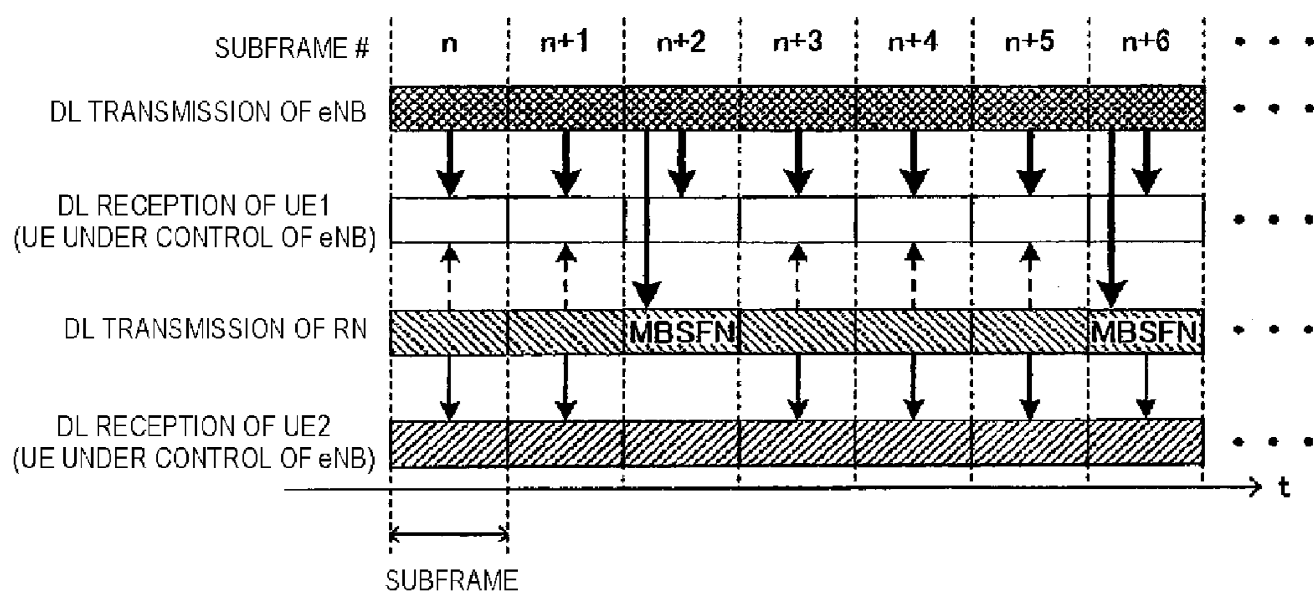
FIG. 21 (PRIOR ART)
