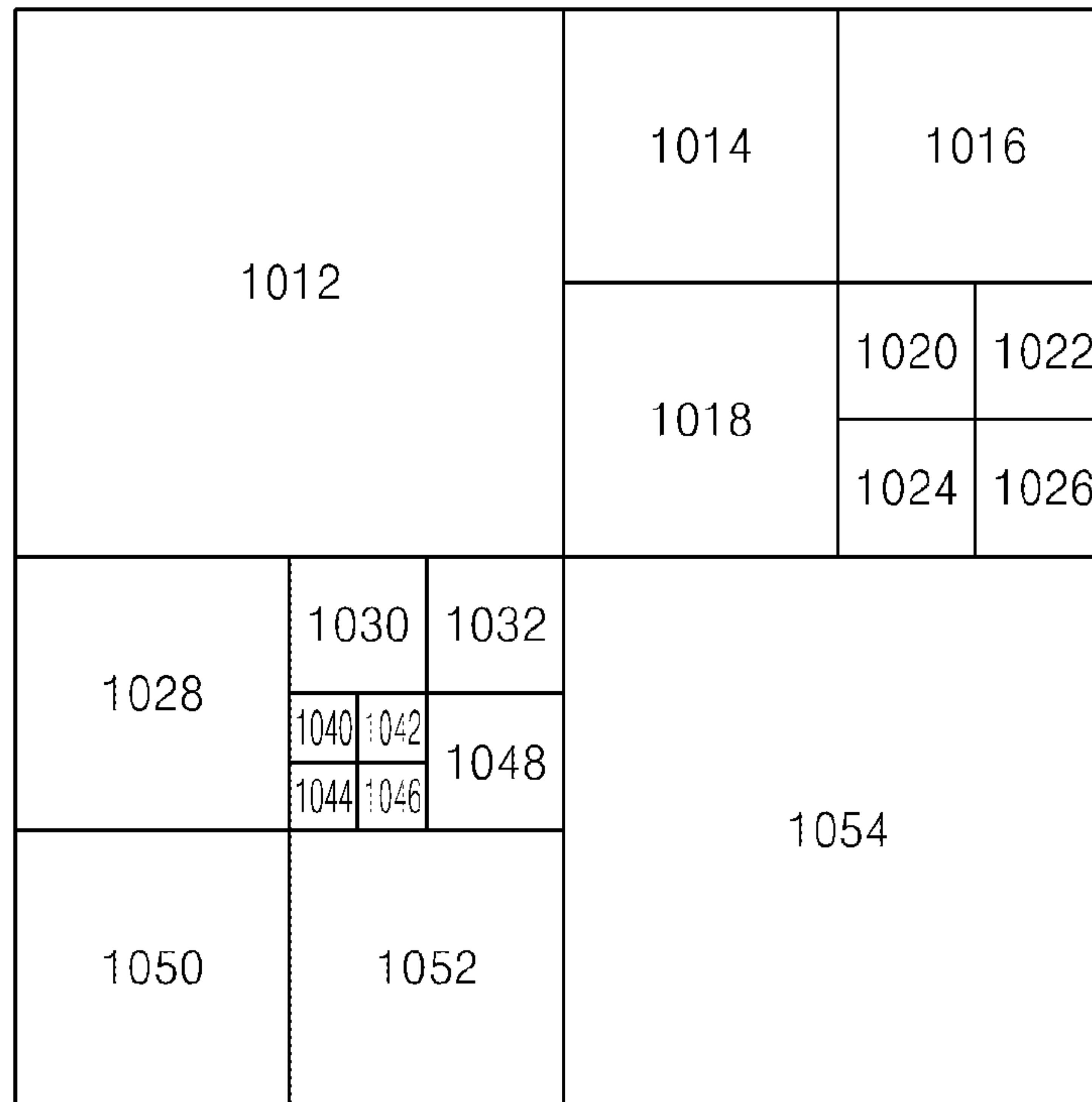
CODING UNIT (1010)
