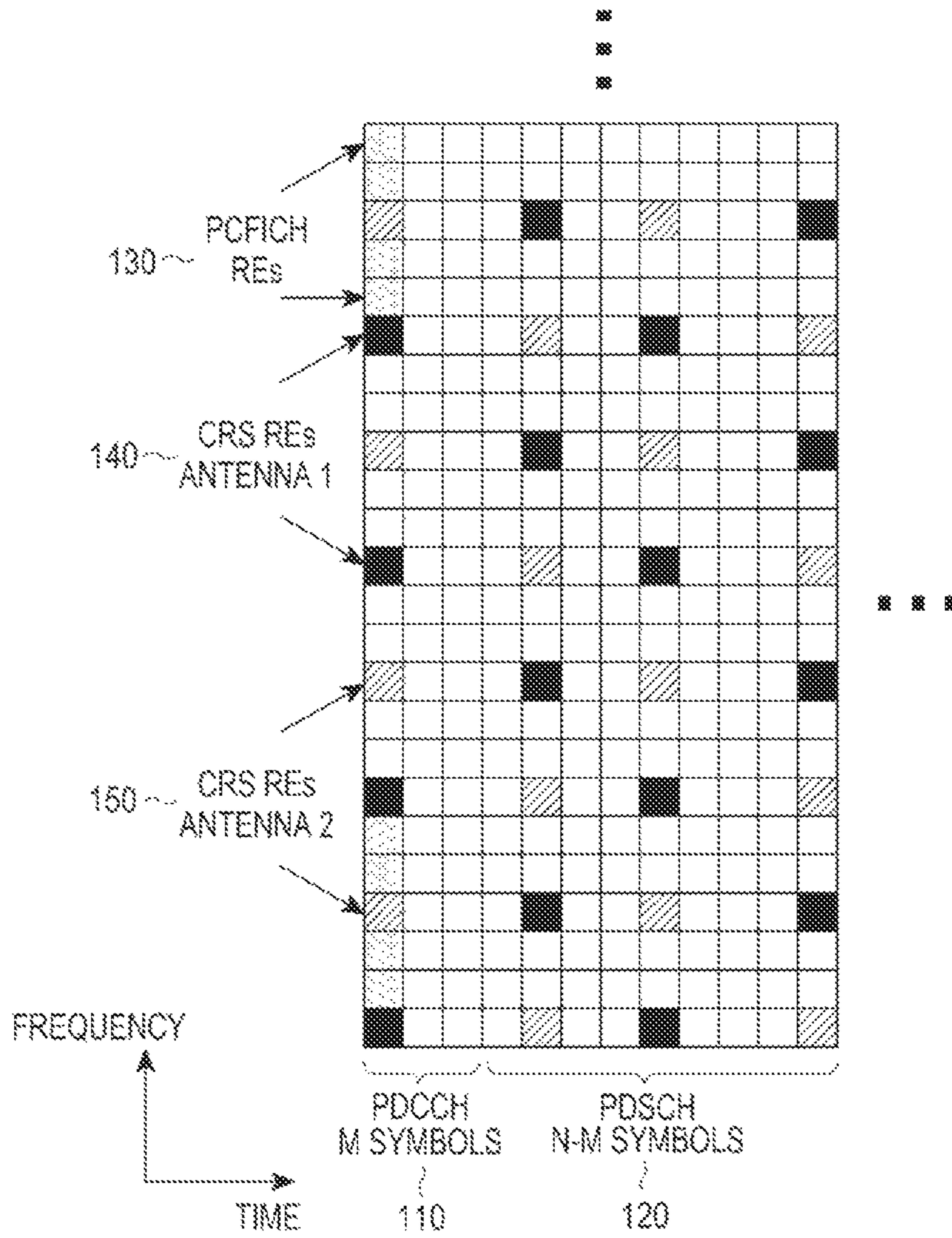
FIG. 1 (PRIOR ART)
