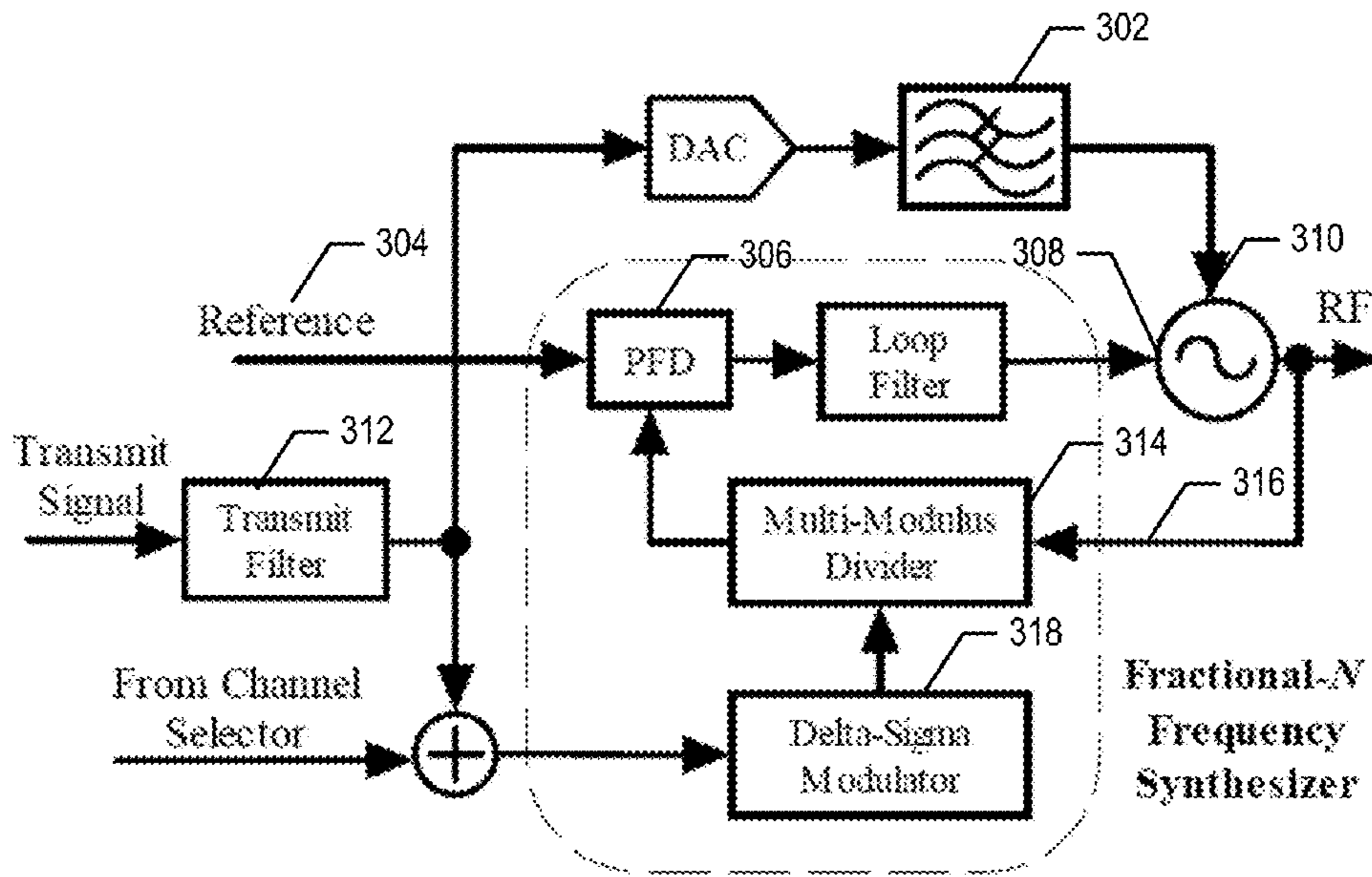
Fig. 3 (Prior Art)
