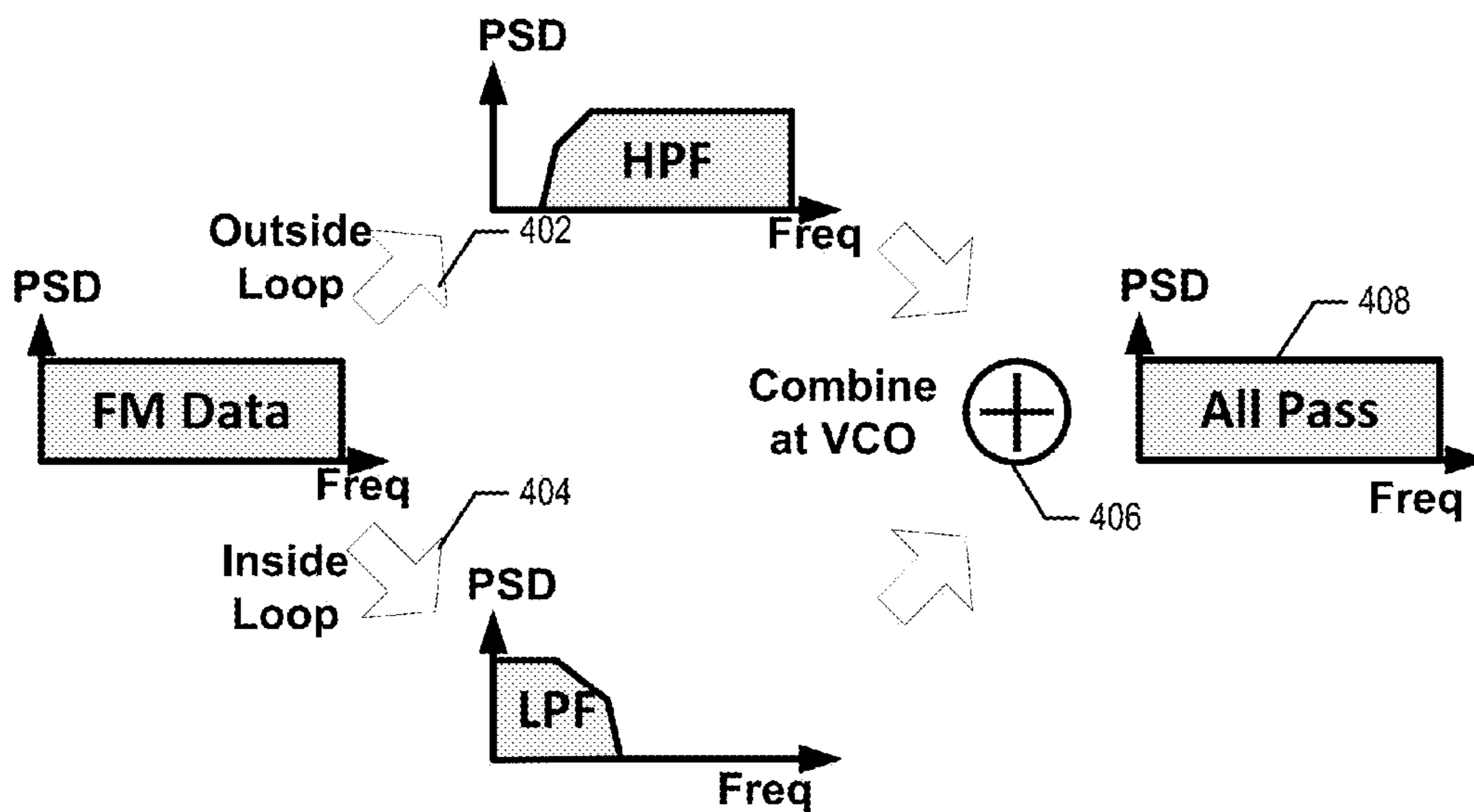
Fig. 4 (Prior Art)
