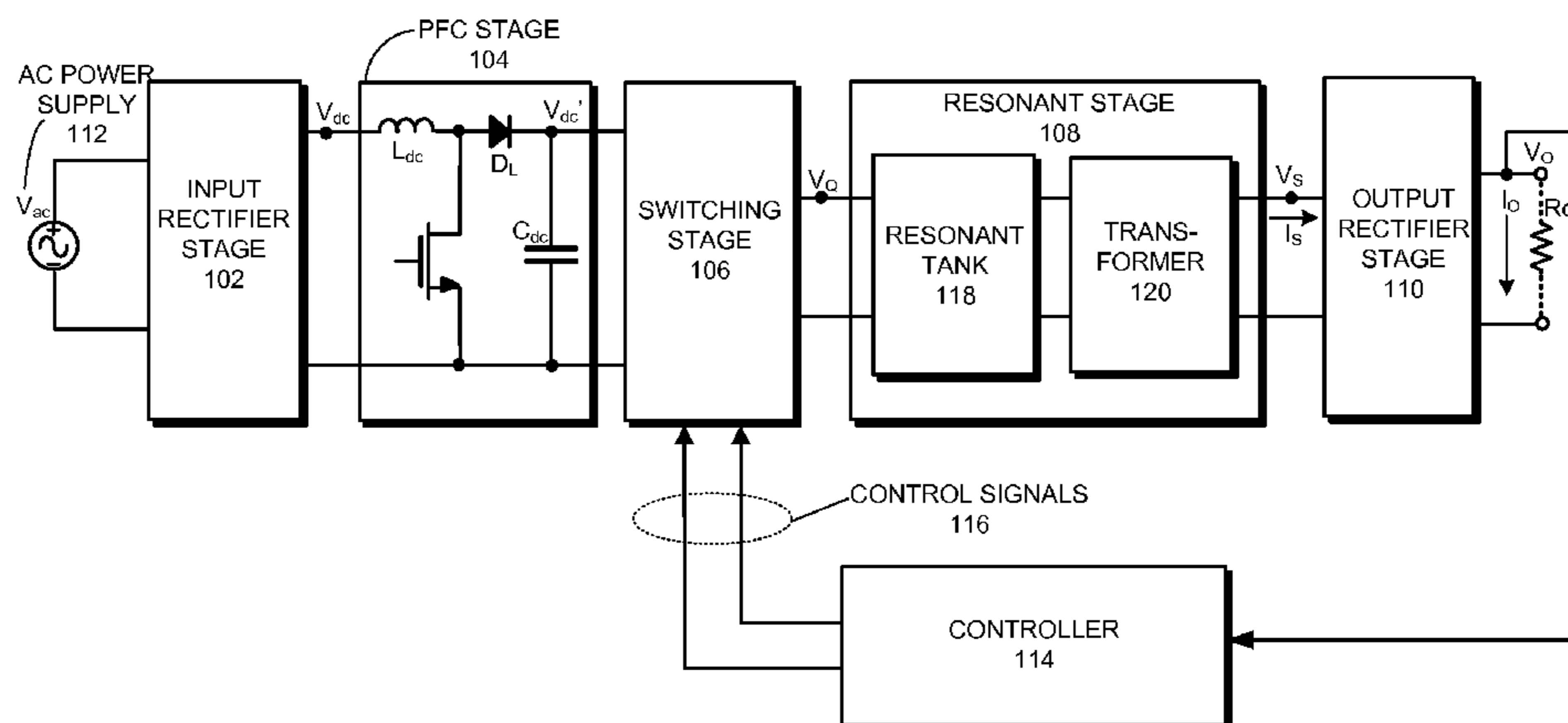
AC/DC CONVERTER 100
