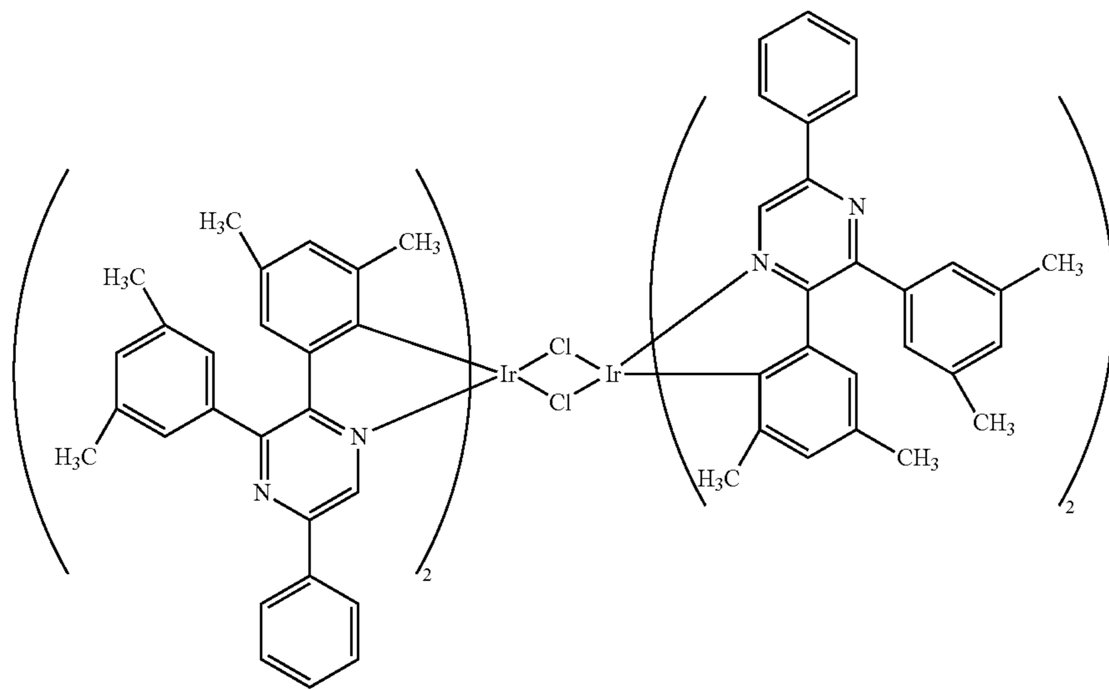
[Ir(dmdppr-P) 2 Cl] 2
