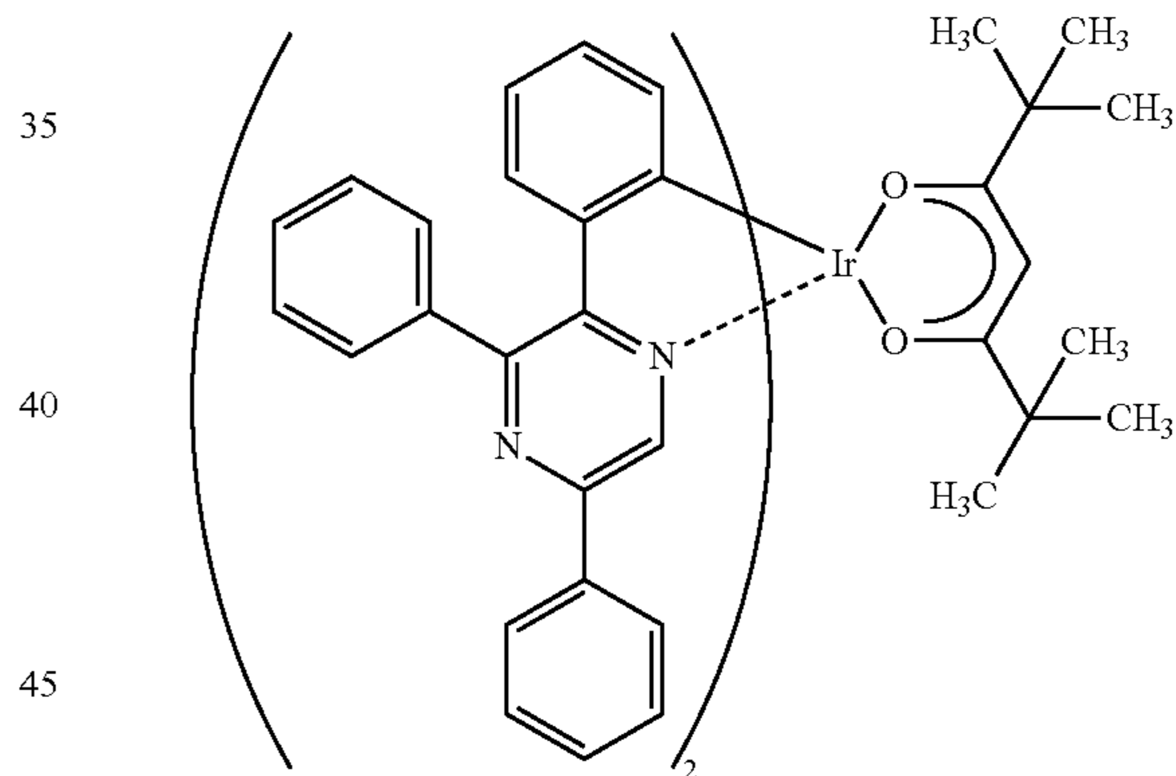
[Ir(tppr) 2 (dpm)]
