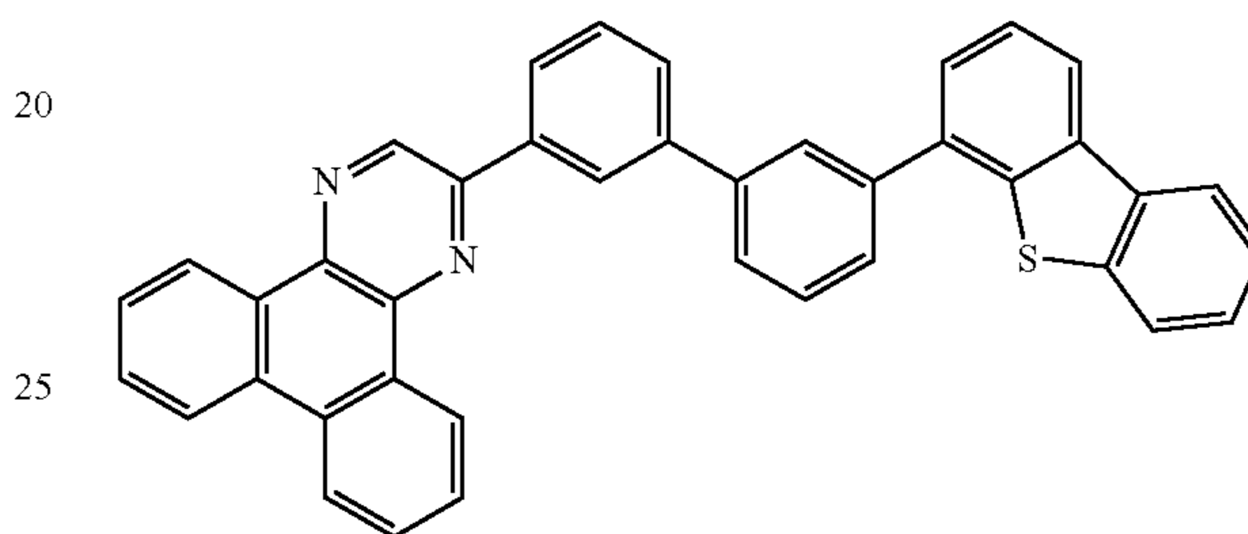
2mDBTBPDq-II
