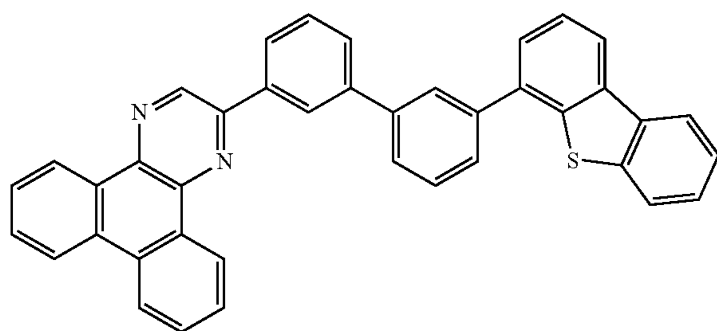
2mDBTBPDBq-II
