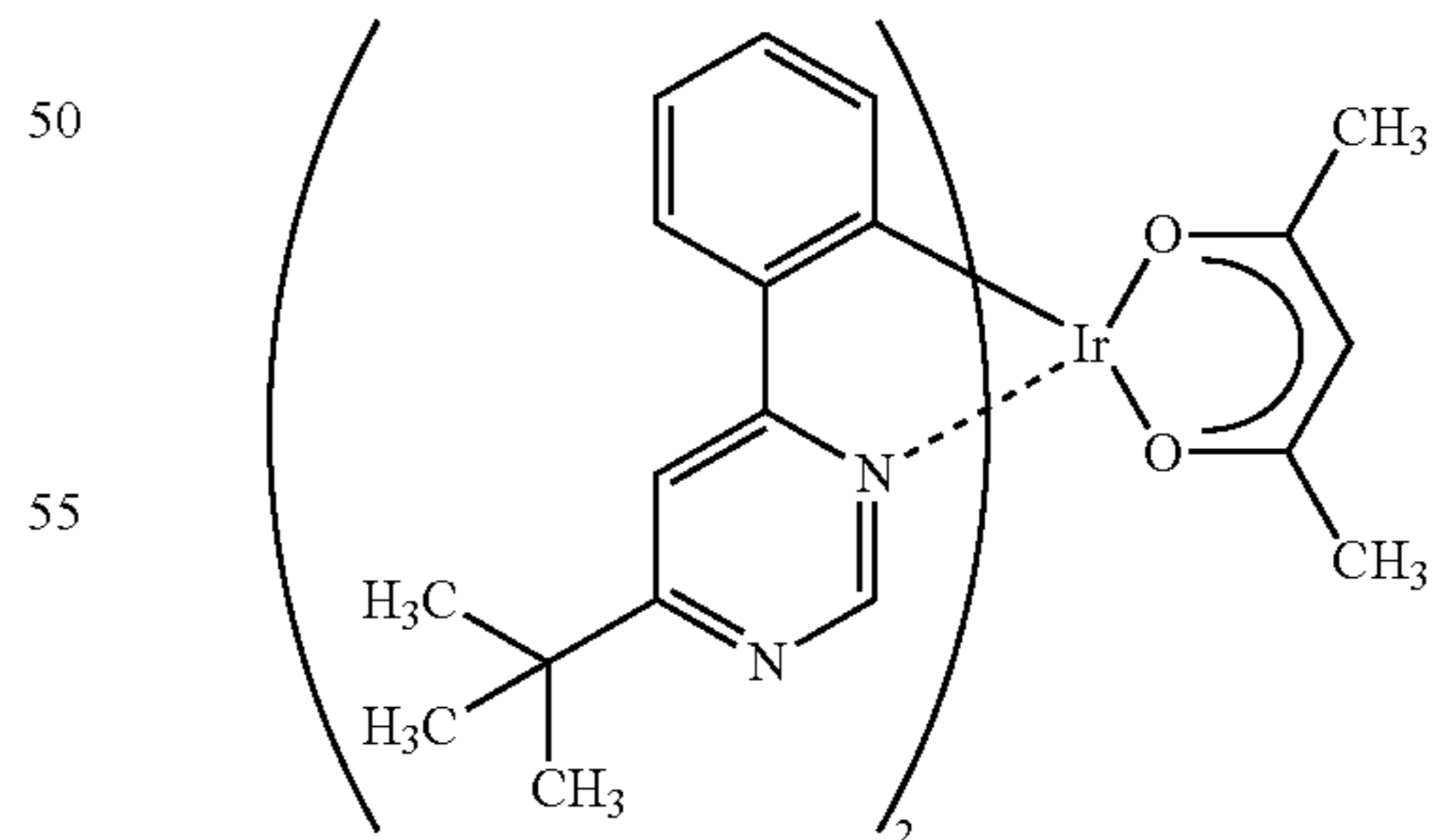
[Ir(tBuppm) 2 (acac)]
