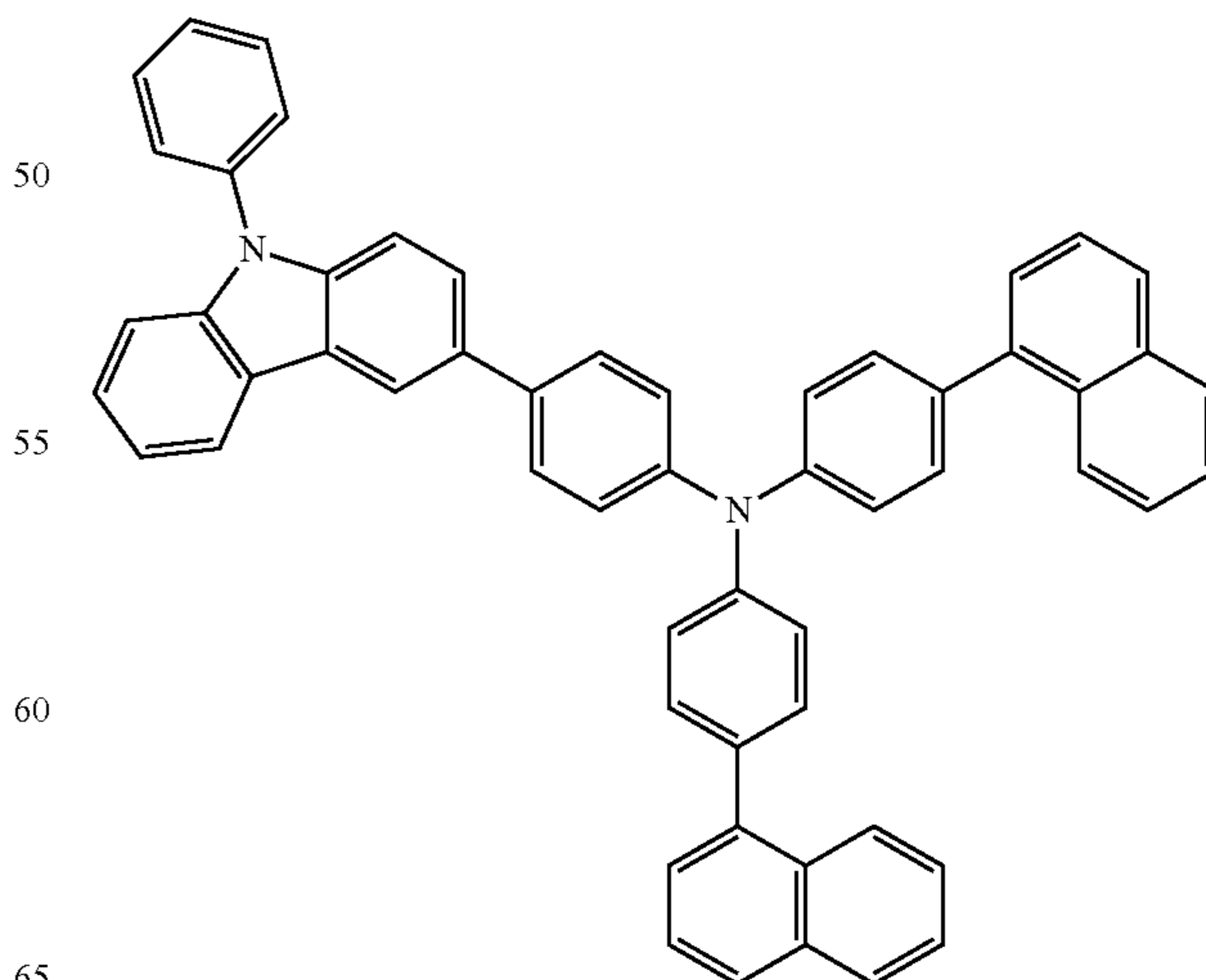
PCBNBB
