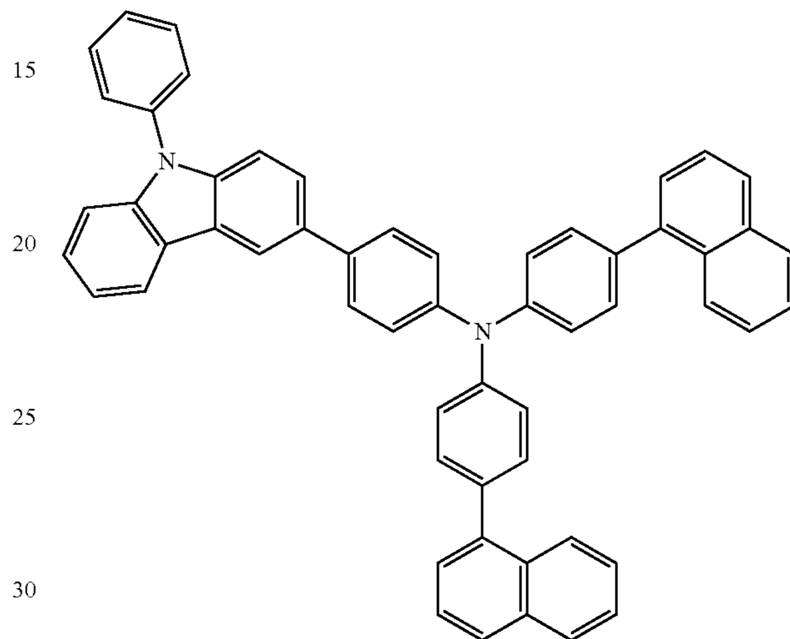
PCBNBB
