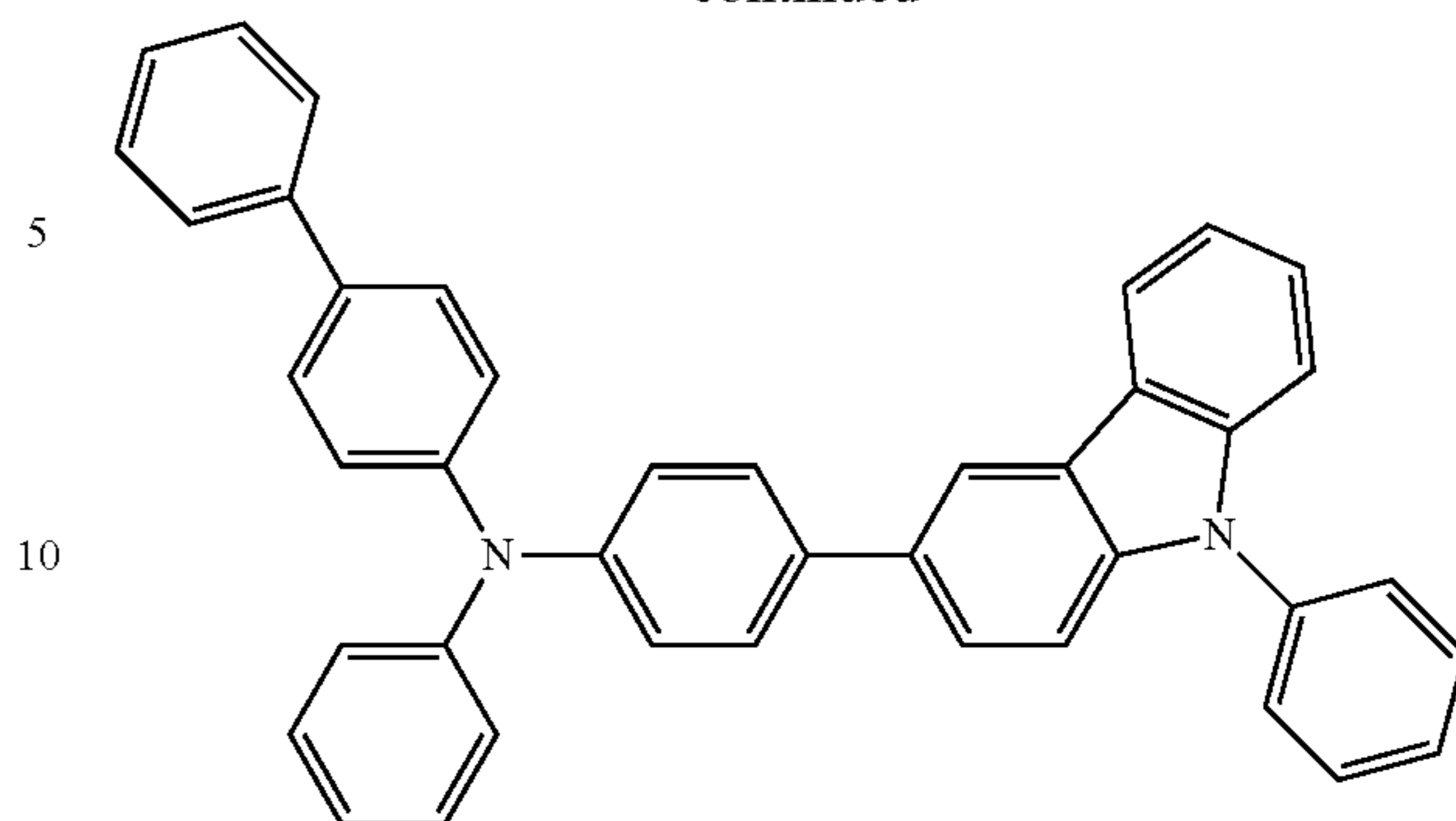
PCBA1BP
