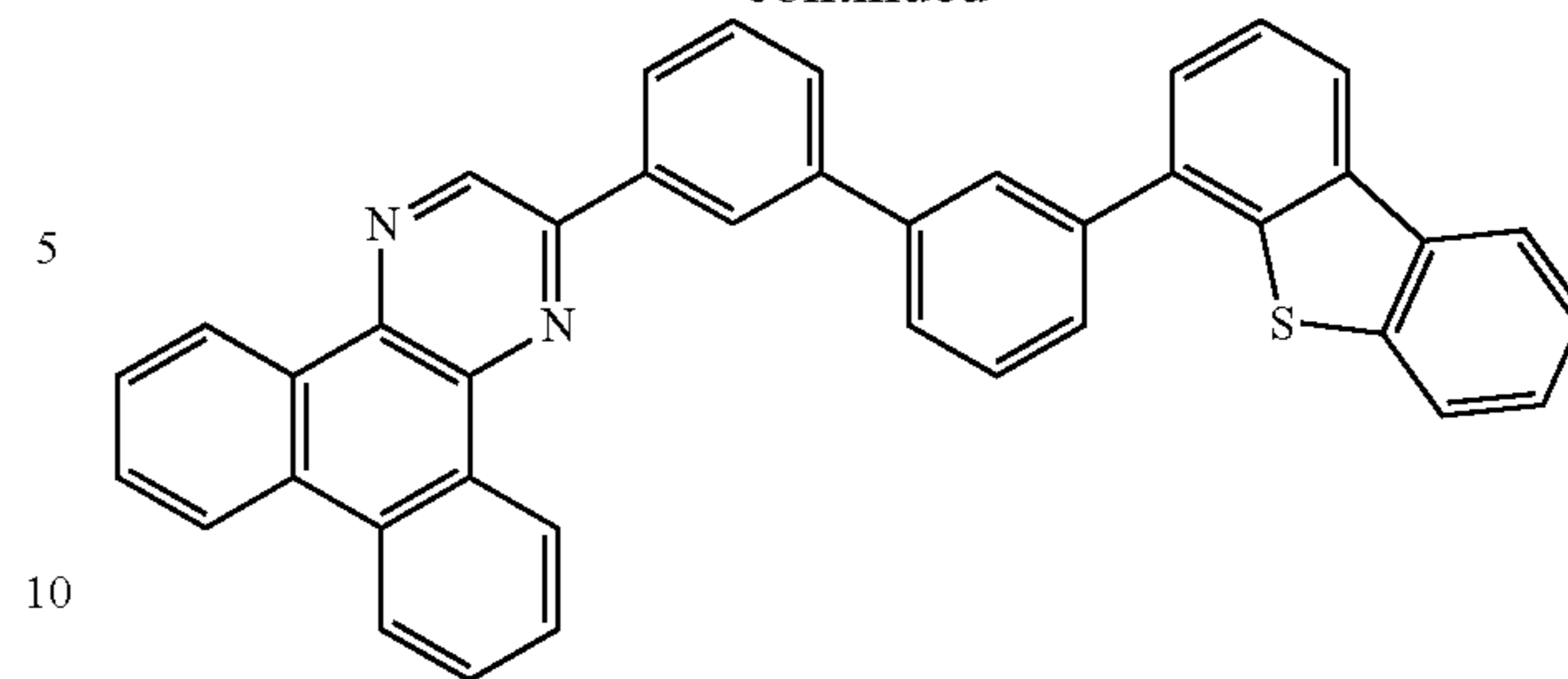
2mDBTBPDBq-II
