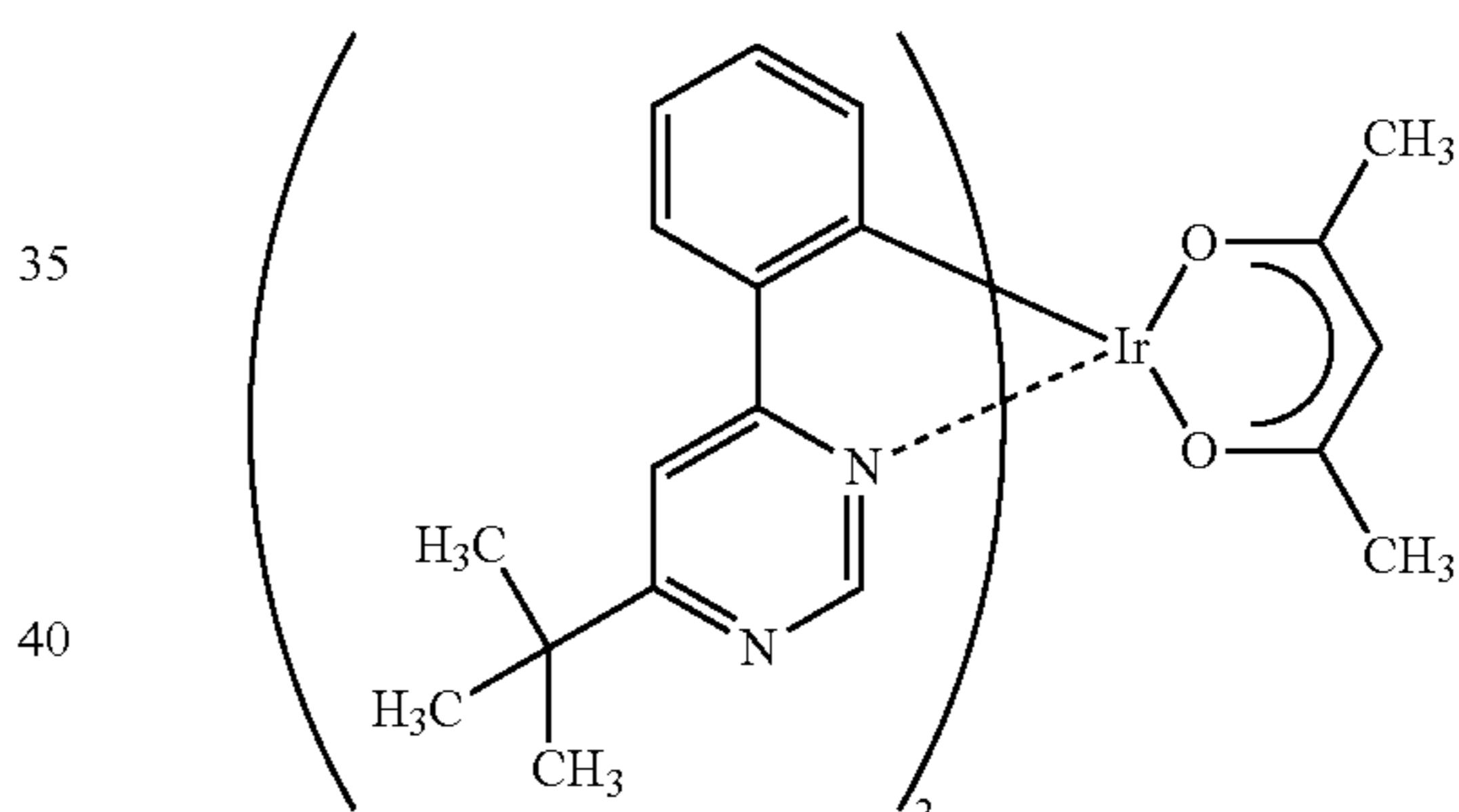
[Ir(tBuppm) 2 (acac)]
