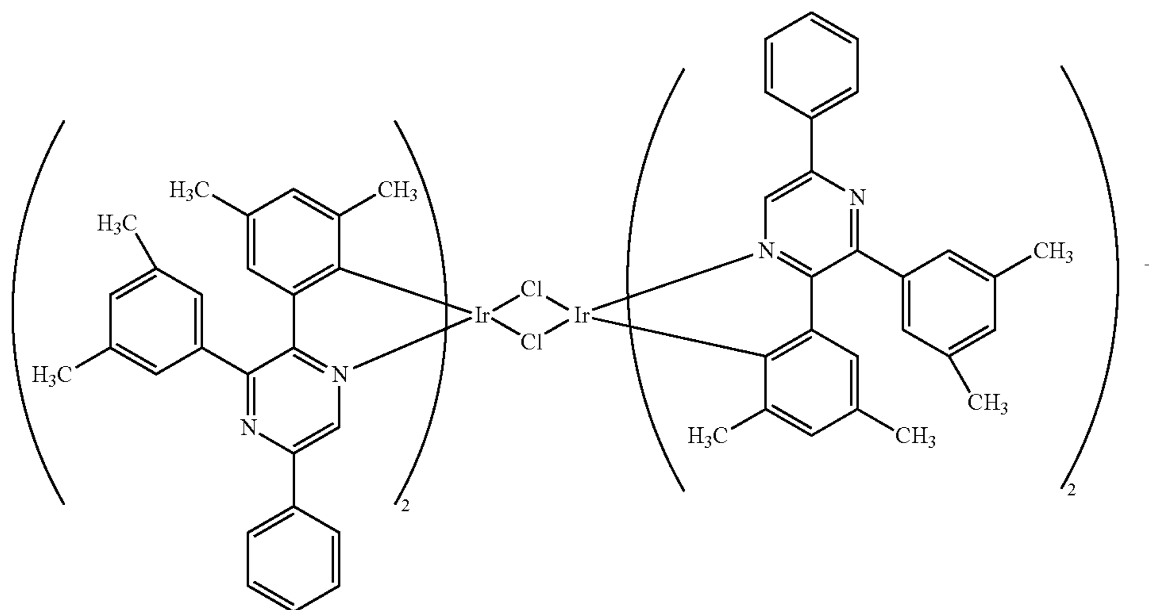
[Ir(dmdppr-P) 2 Cl] 2
