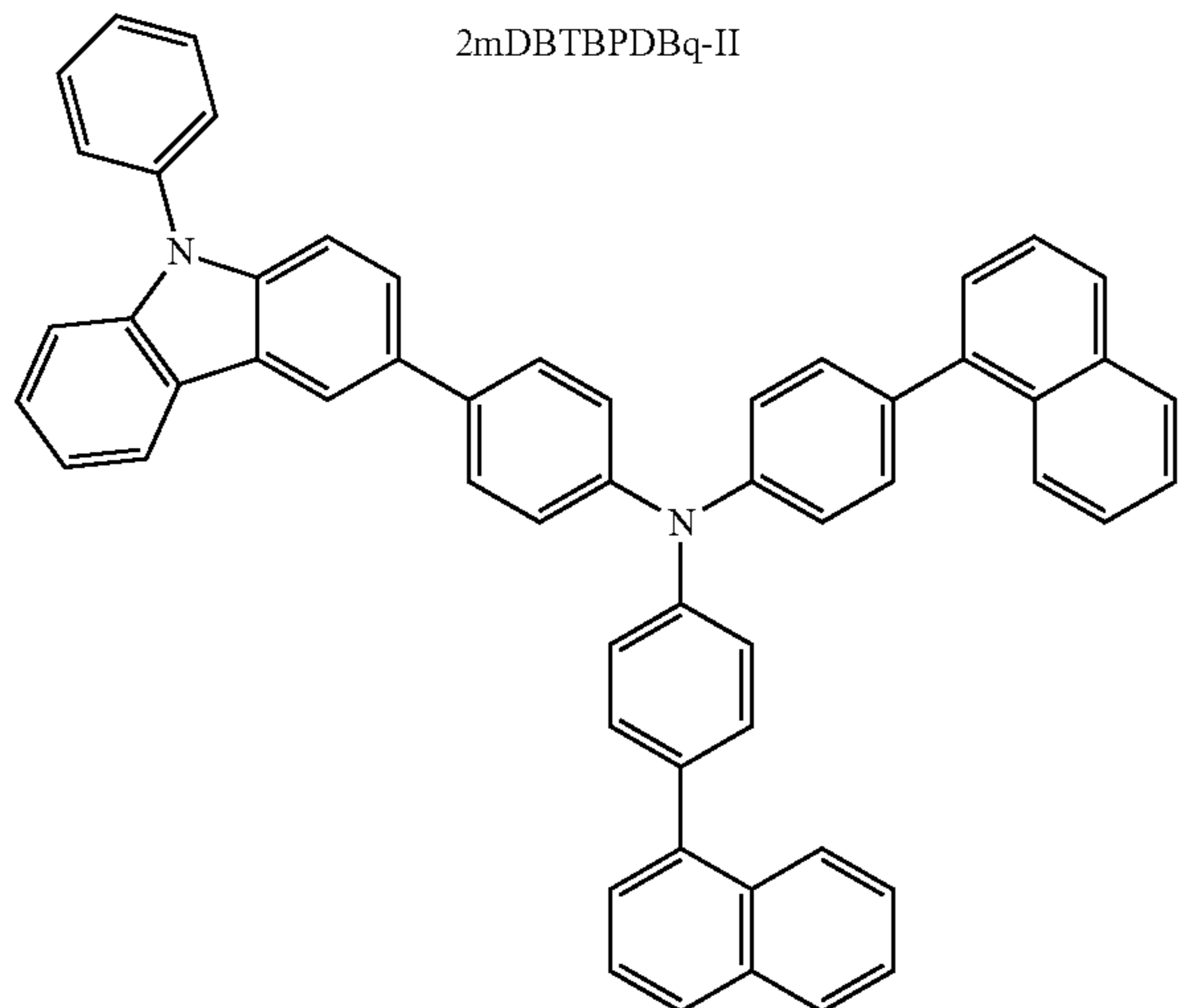
PCBNBB
