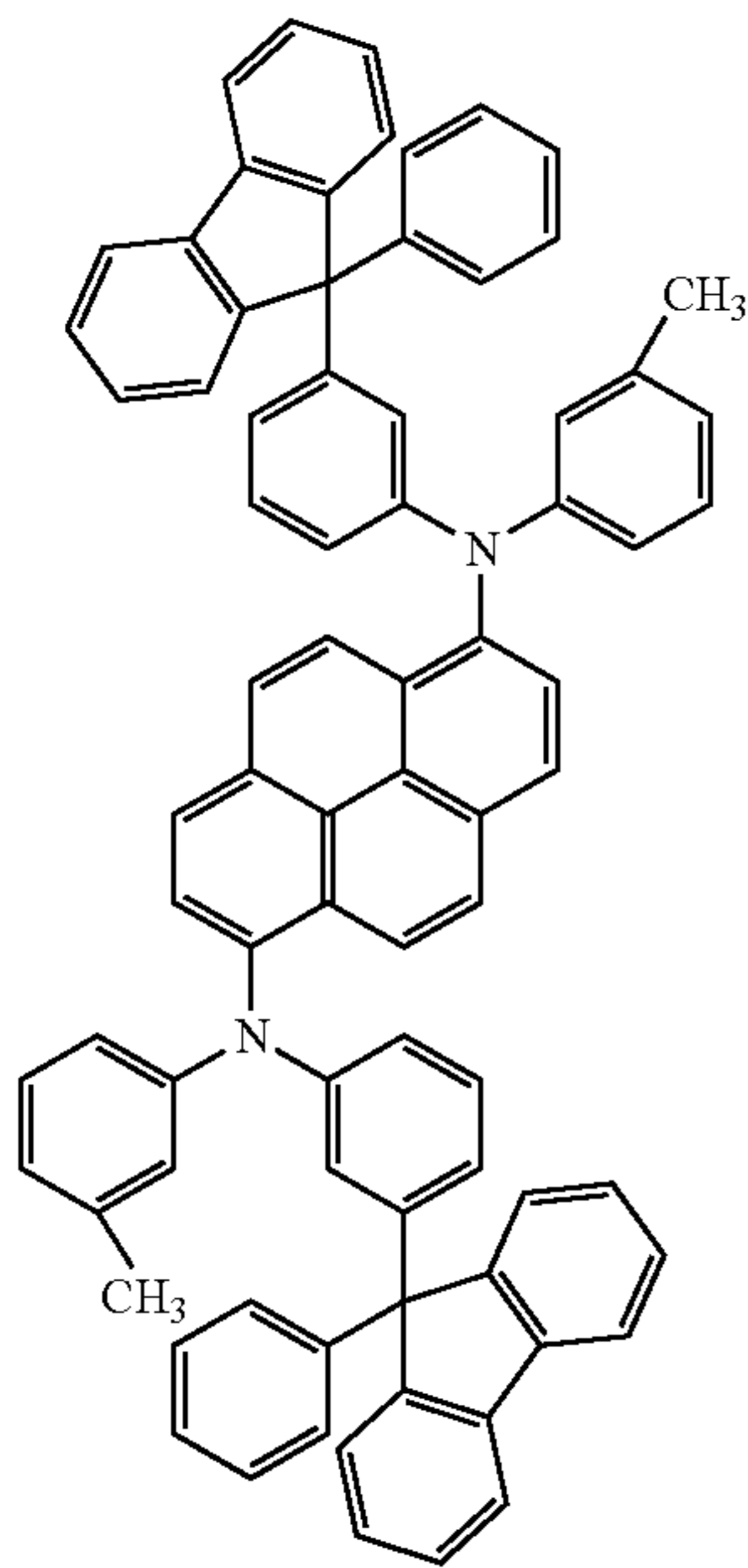
1,6mMemFLPAPm
