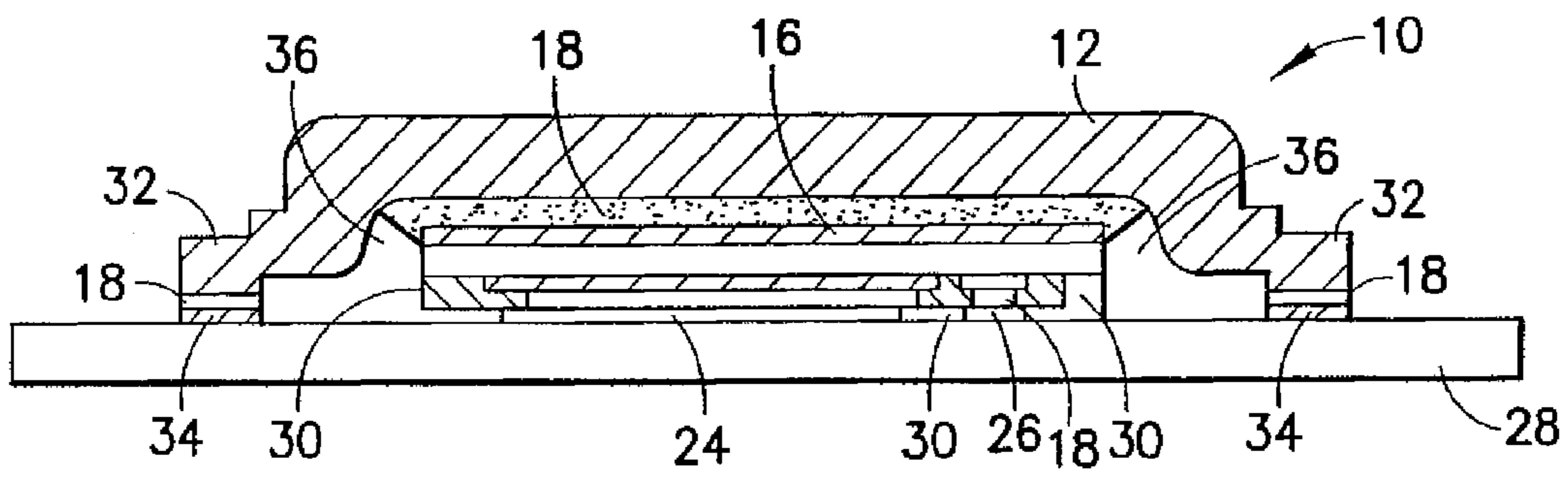
FIG. 4 PRIOR ART
