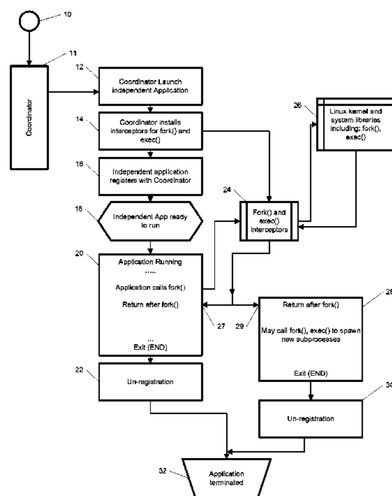
Core operation of fork()
