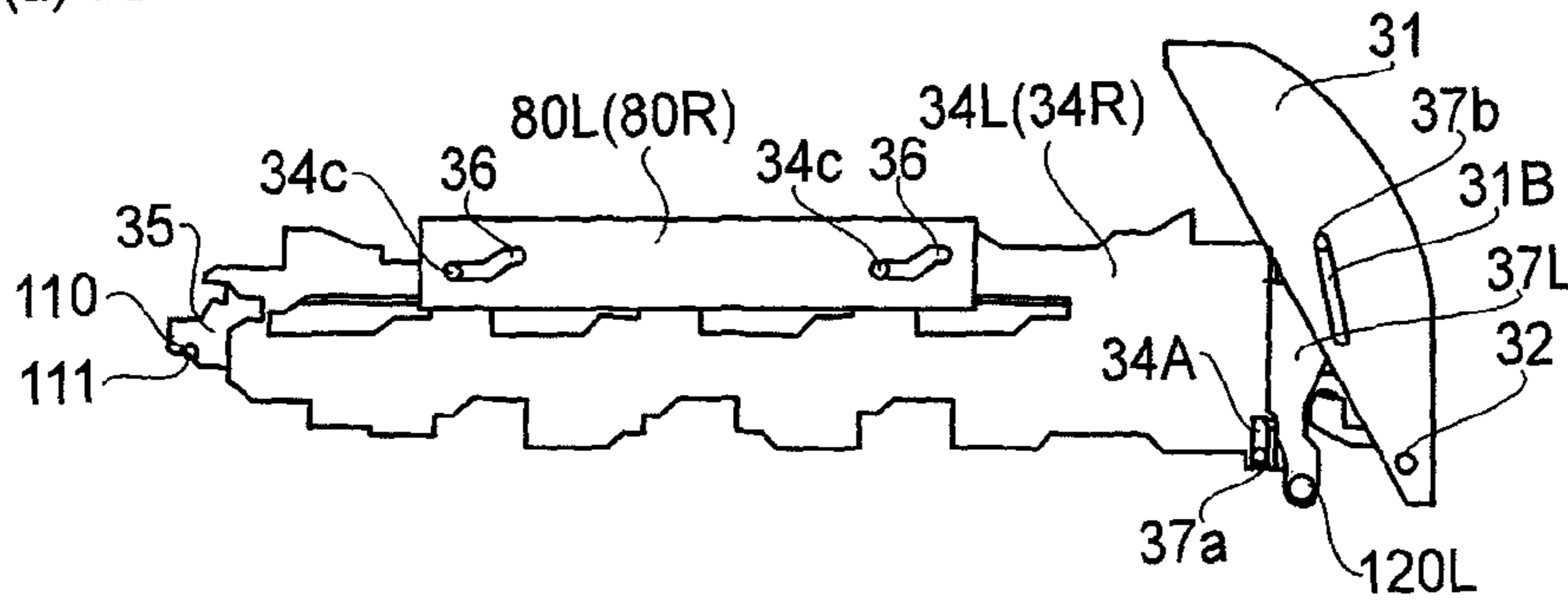
(a) CLOSED
