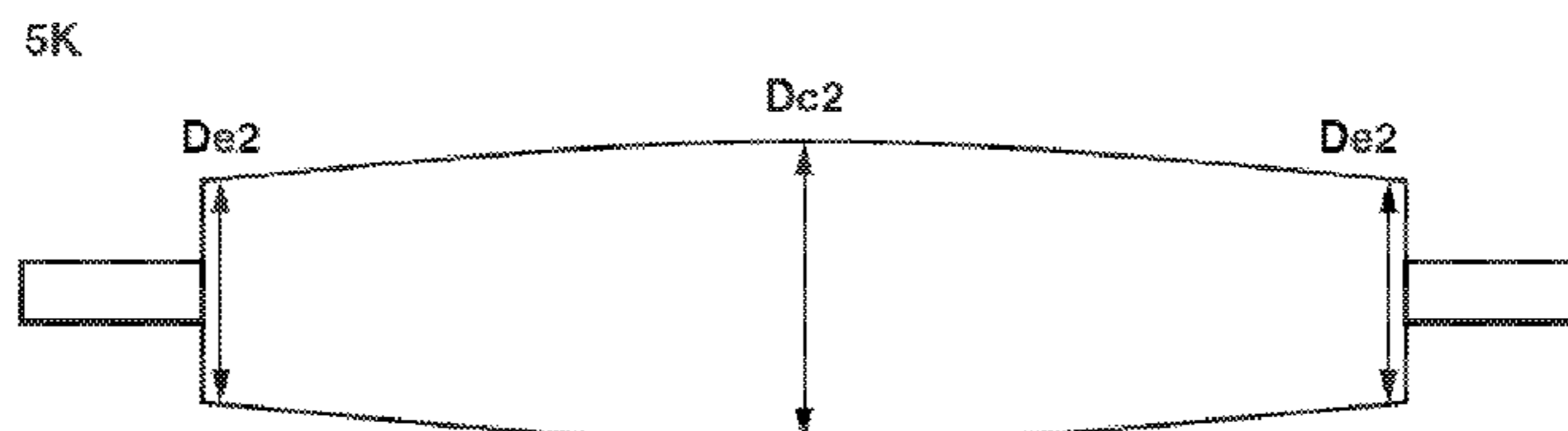
A CROWN AMOUNT: (Dc2 - De2)
