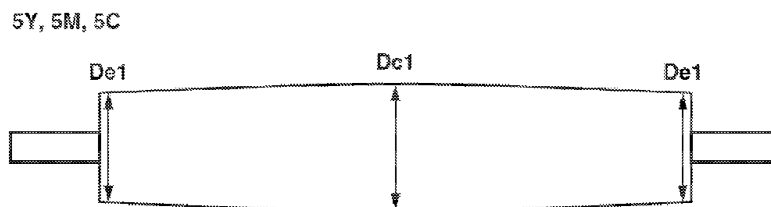
A CROWN AMOUNT: (Dc1 - De1)
