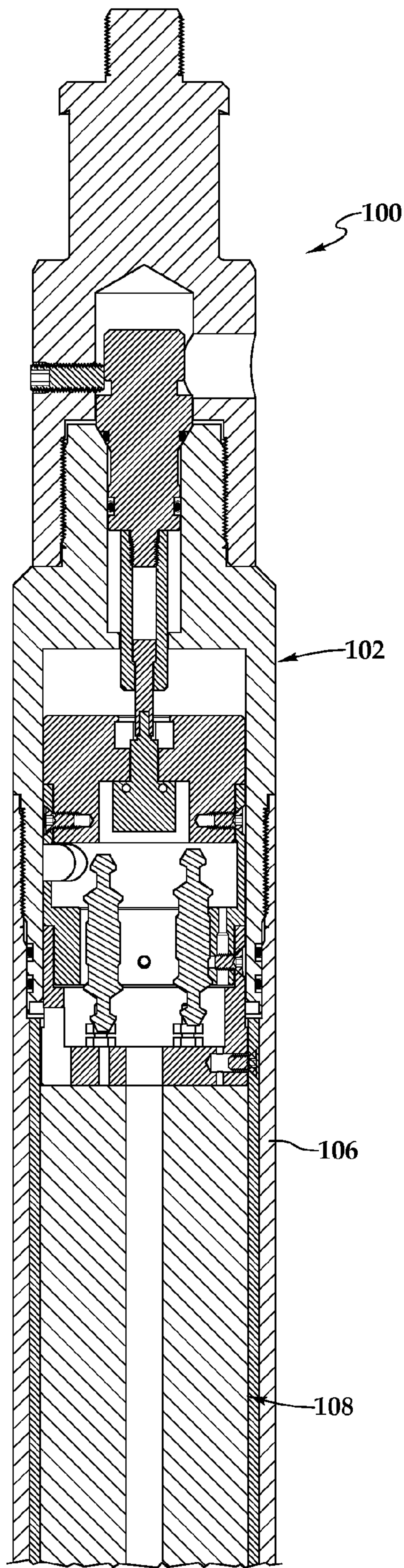
Fig.2A
