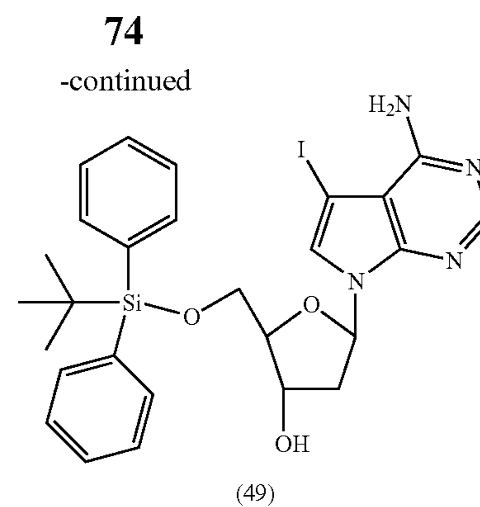
7-Deaza-5'-O-diphenylsilyl-7-iodo-2'-deoxyadenosine (49)
