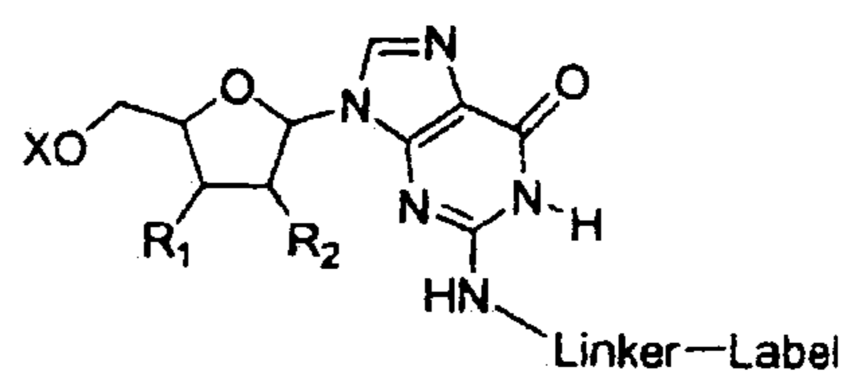
Guanosine N2-linker
