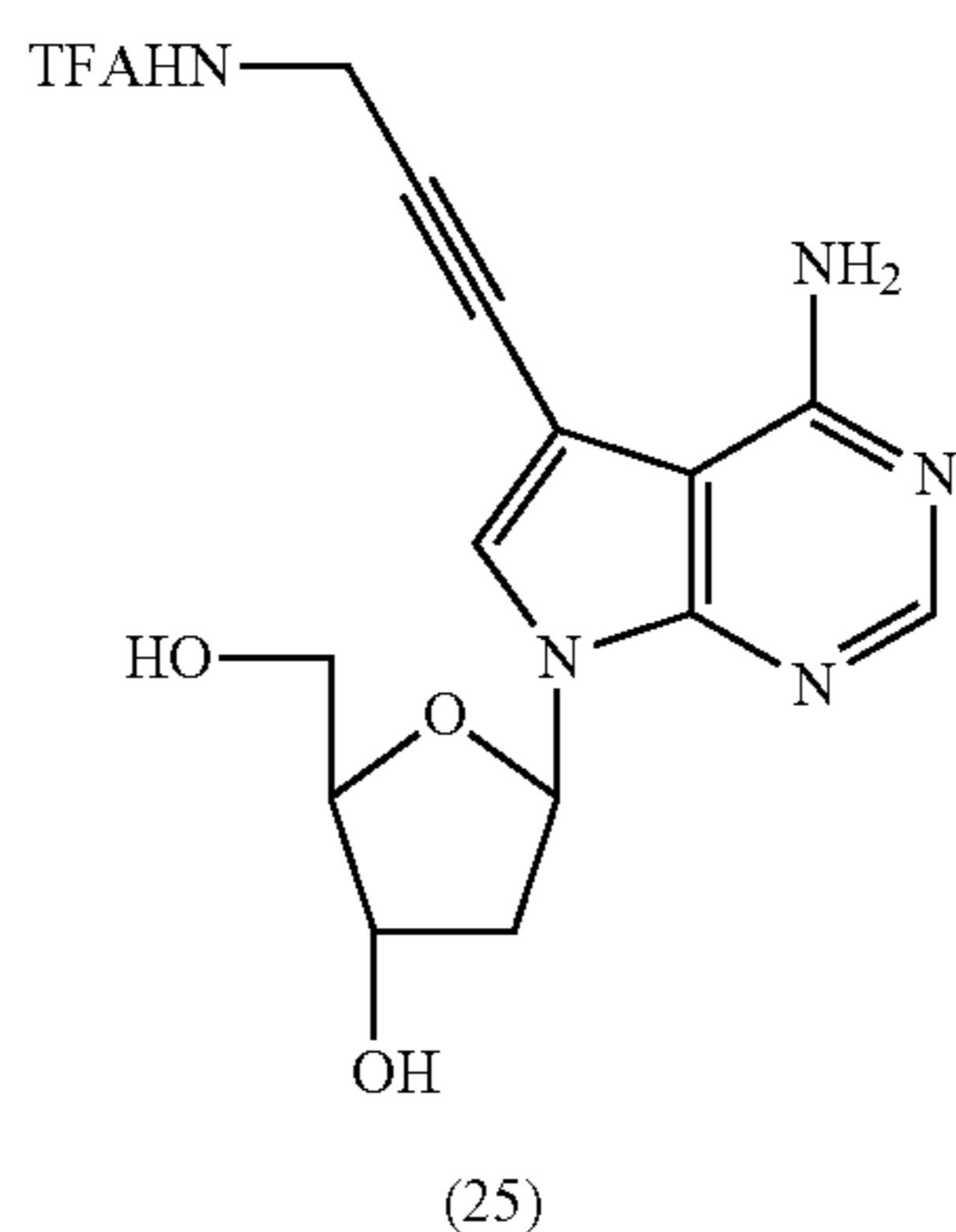
7-Deaza-7-[3-(2,2,2-trifluoroacetamido)-prop-1-ynyl]-2'-deoxyadenosine (25)
