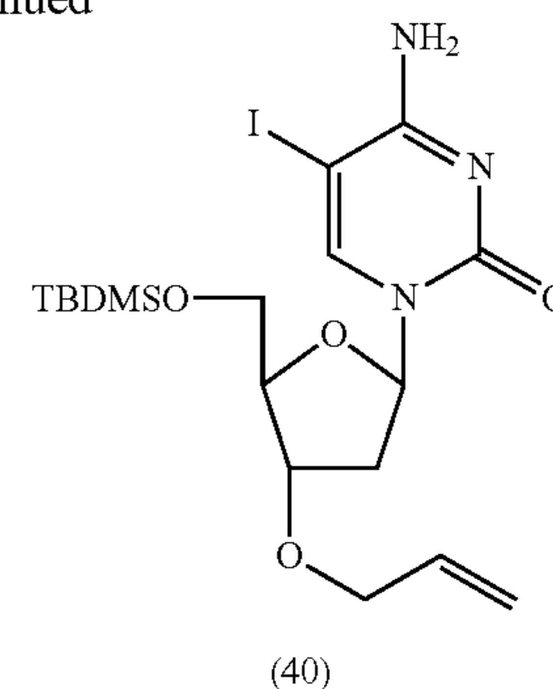
3'-O-Allyl-5'-O-(tert-butyldimethylsilyl)-5-iodo-2'-deoxycytidine (40)
