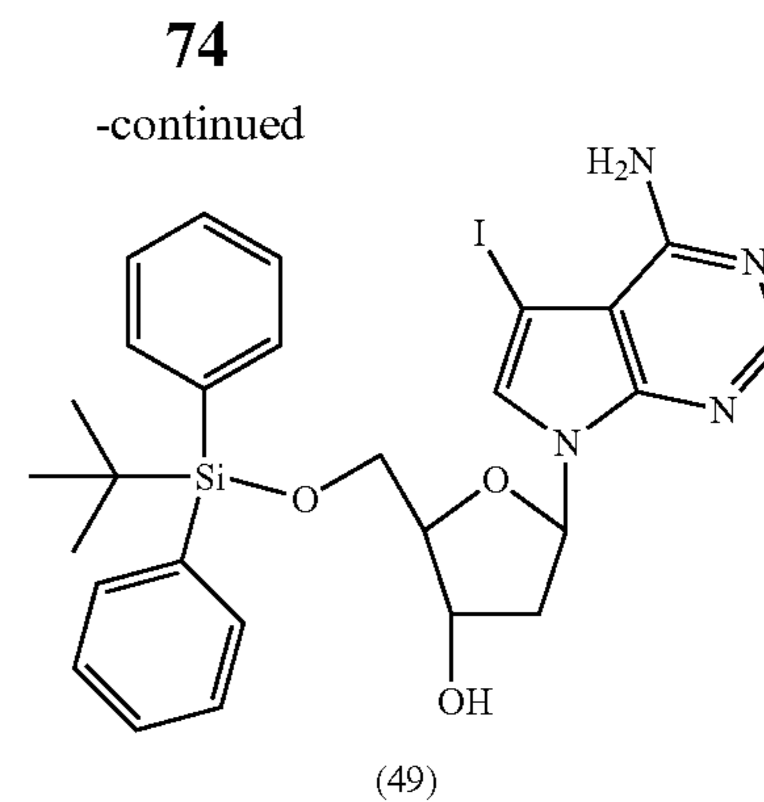
7-Deaza-5'-O-diphenylsilyl-7-iodo-2'-deoxyadenosine (49)
