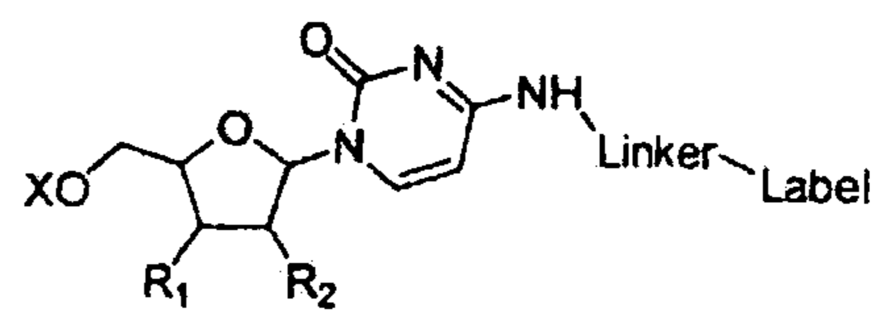
Cytidine N4-linker
