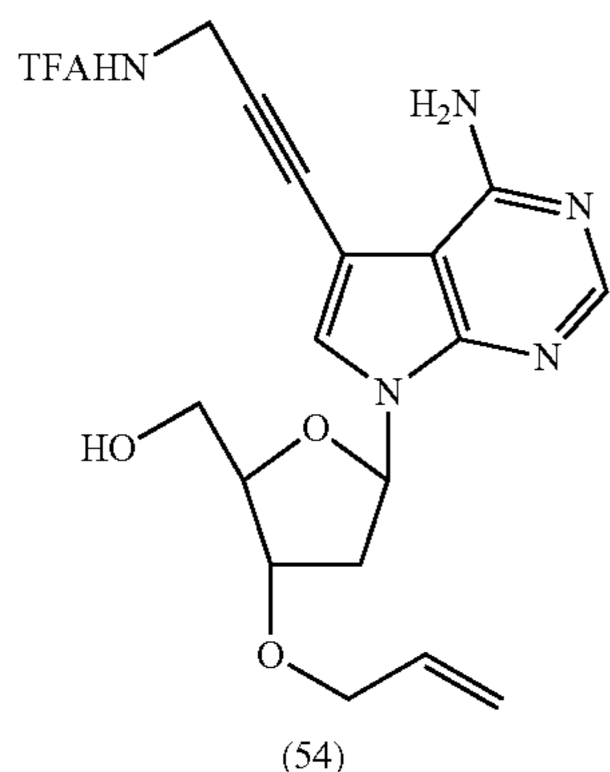
3'-O-Allyl-7-deaza-7-[3-(2,2,2-trifluoroacetamide)]-2'-deoxyadenosine (54)
