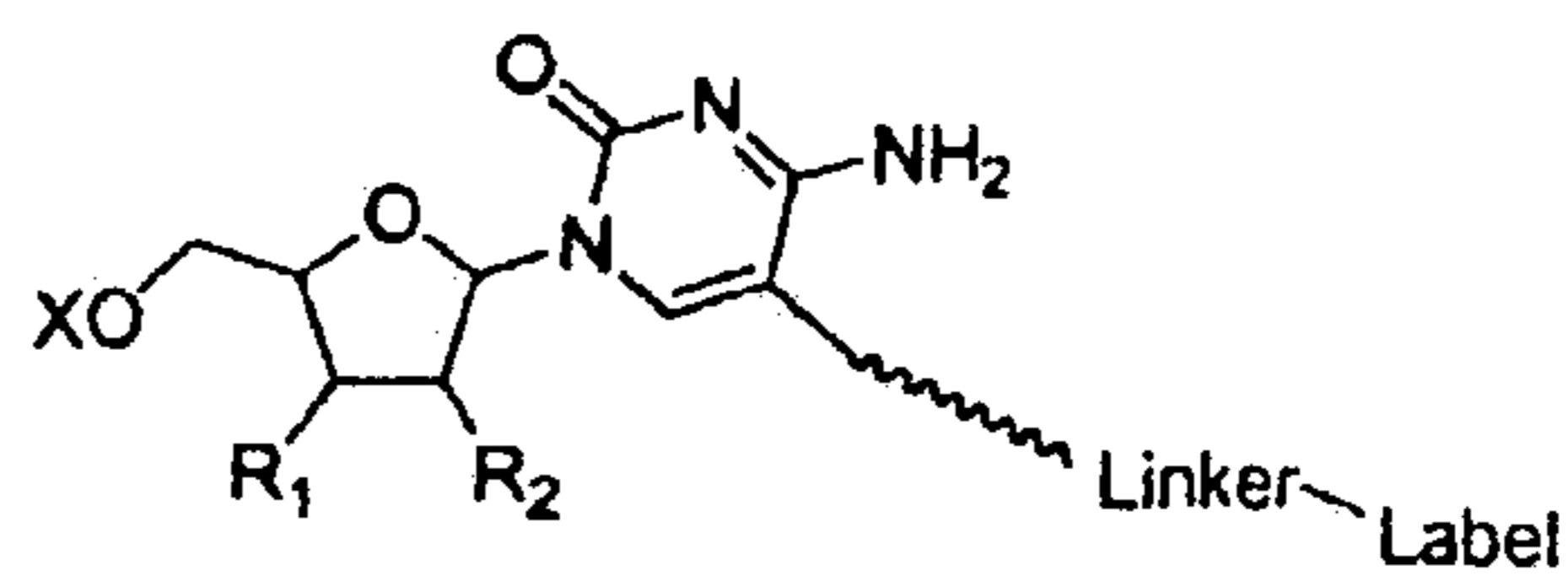
Cytidine C5-linker
