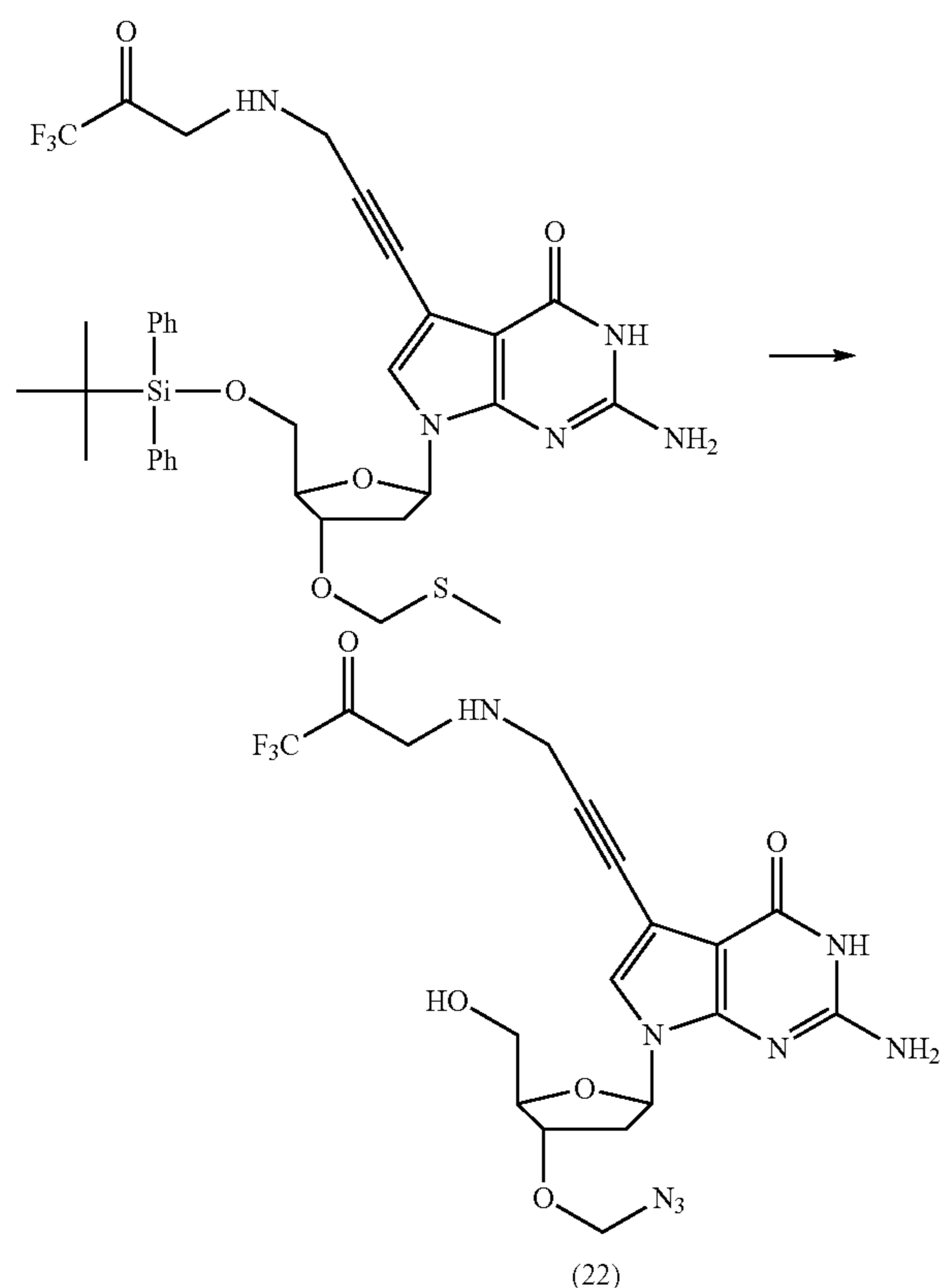
3'-O-Azidomethyl-7-deaza-7-[3-(2,2,2-trifluoroacetamido)-prop-1-ynyl]-2'-deoxyguanosine (22)
