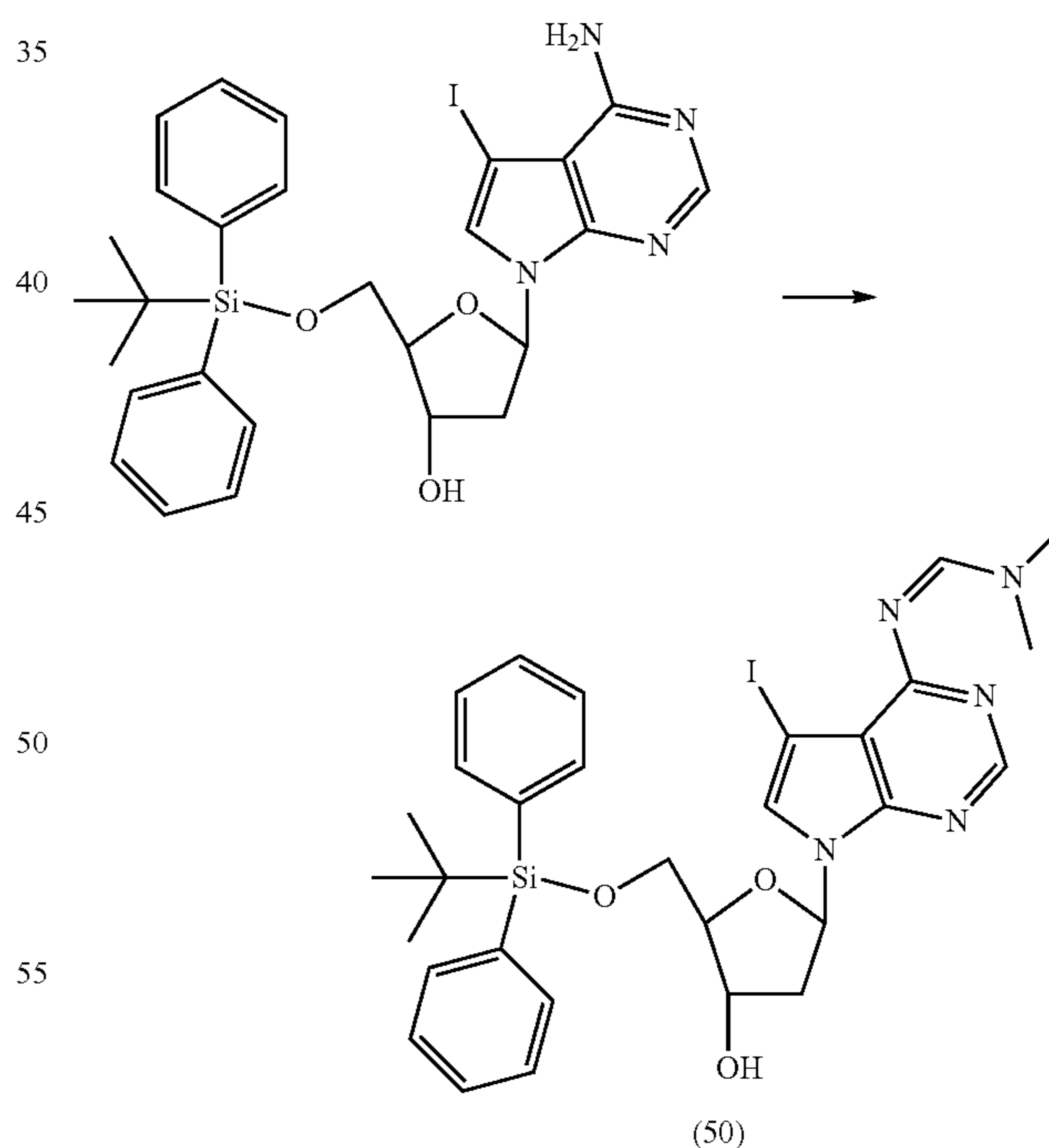
7-Deaza-6-N,N-dimethylformadine-5'-O-diphenylsilyl-7-iodo-2'-deoxyadenosine (50)
