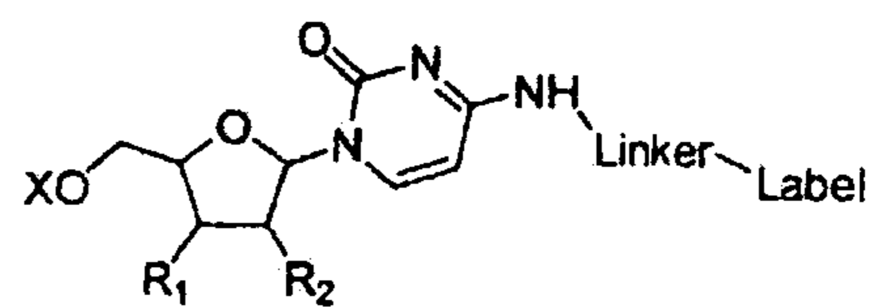
Cytidine N4-linker
