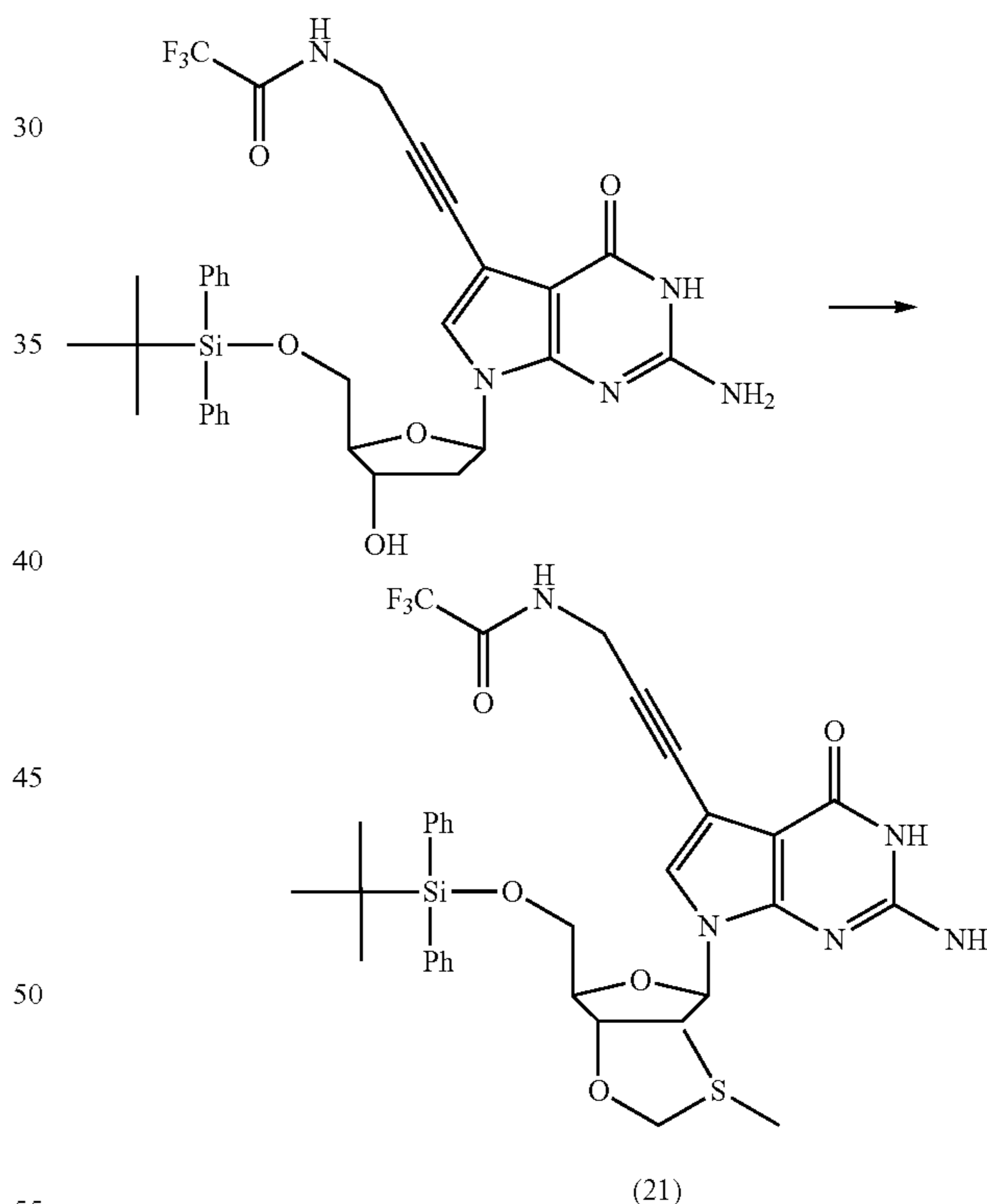
5'-O-(tert-Butyldiphenyl)-7-deaza-3'-O-methylthiol-methyl-7-[3-(2,2,2-trifluoroacetamido)-prop-1-ynyl]-2'-deoxyguanosine (21)
