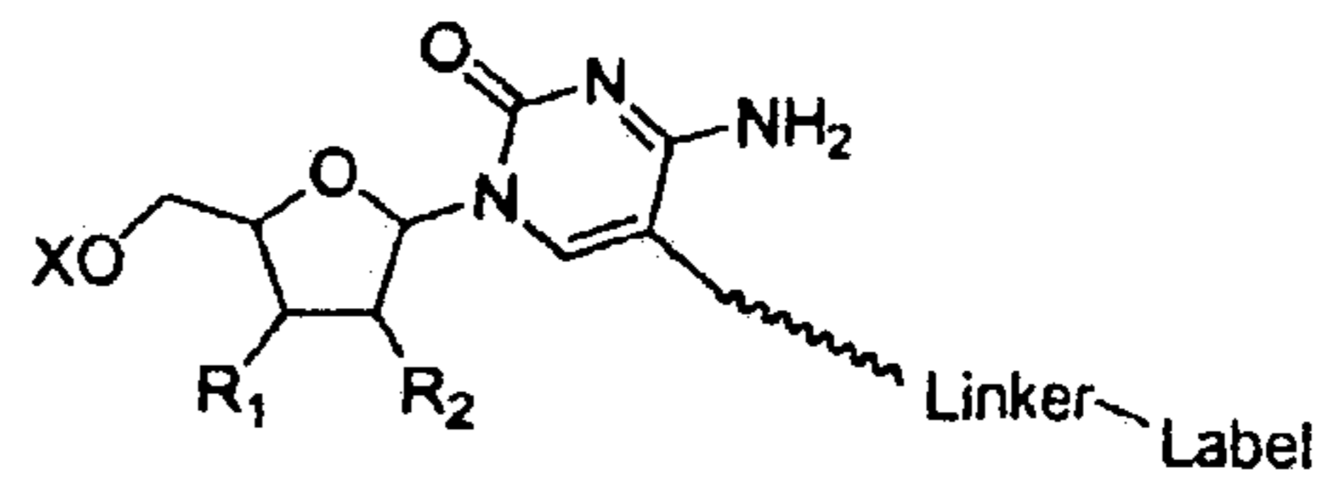
Cytidine C5-linker
