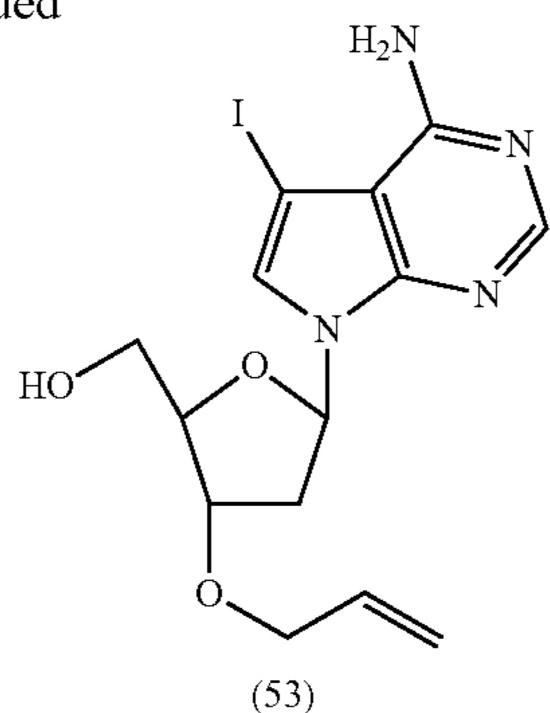
3'-O-Allyl-7-deaza-7-iodo-2'-deoxyadenosine (53)
