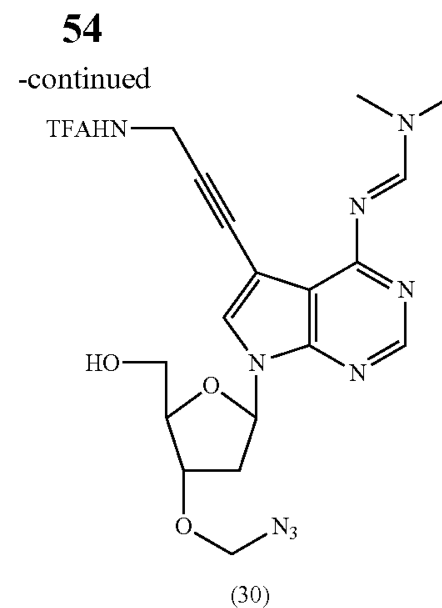
3'-O-Azidomethyl-7-deaza-4-N,N-dimethylformadin-7-[3-(2,2,2-trifluoroacetamido)-prop-1-ynyl]-2'-deoxyadenosine (30)
