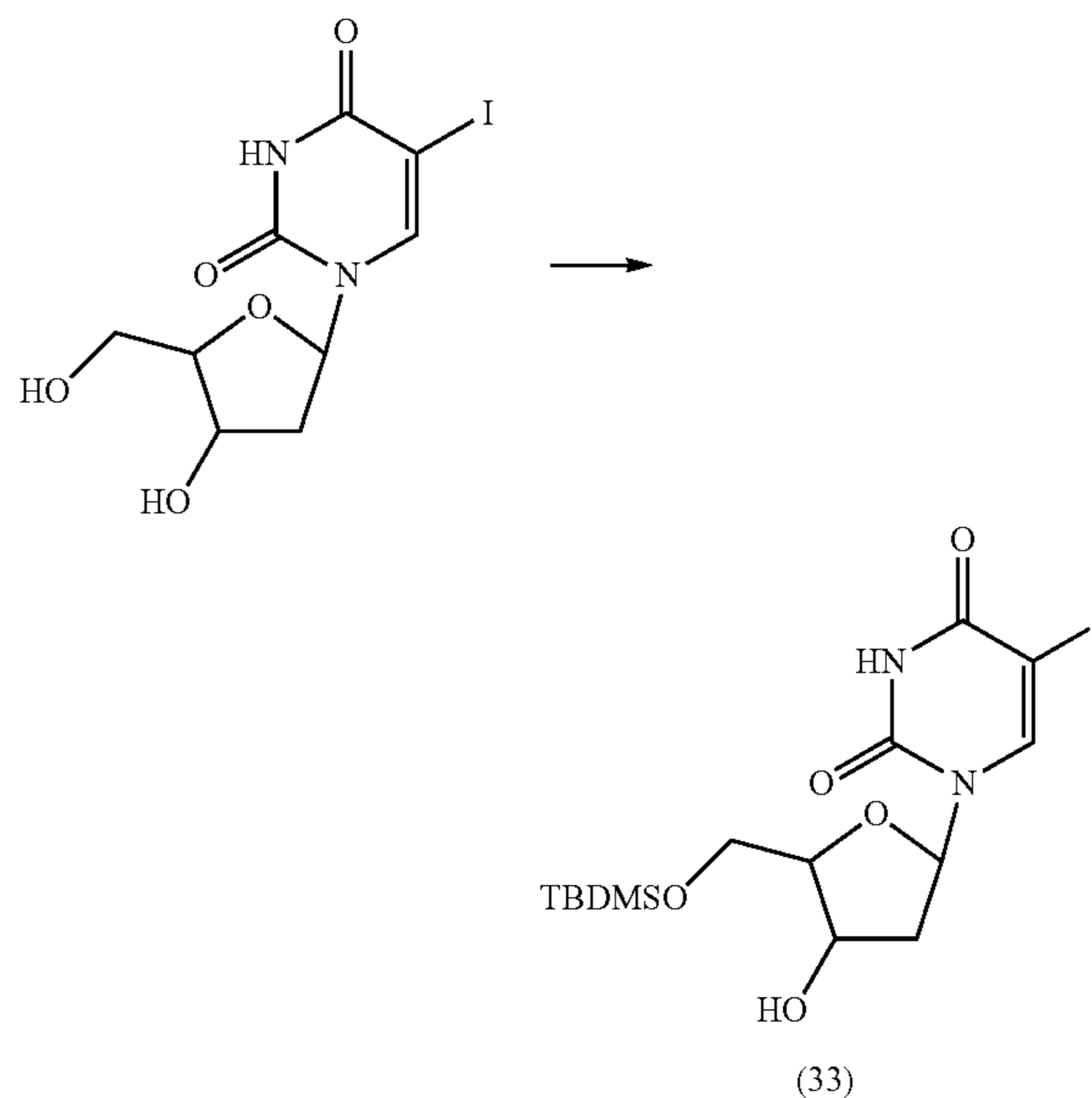
5'-O-(t-Butyldimethylsilyl)-5-iodo-2'-deoxyuridine (33)
