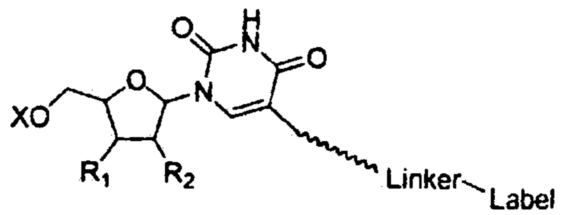
Uridine C5-linker
