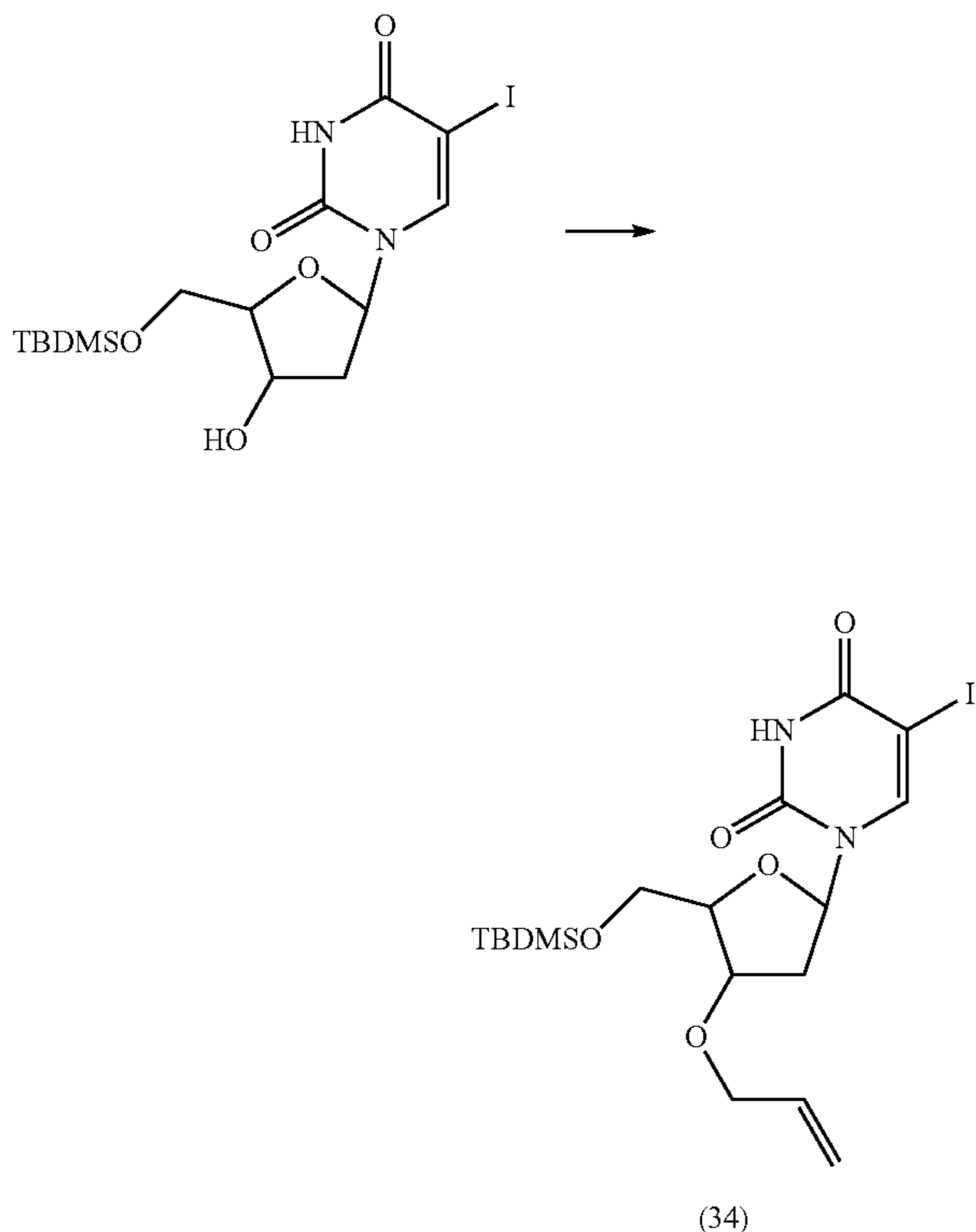
3'-O-Allyl-5'-O-t-butyl dimethylsilyl-5-iodo-2'-deoxyuridine (34)
