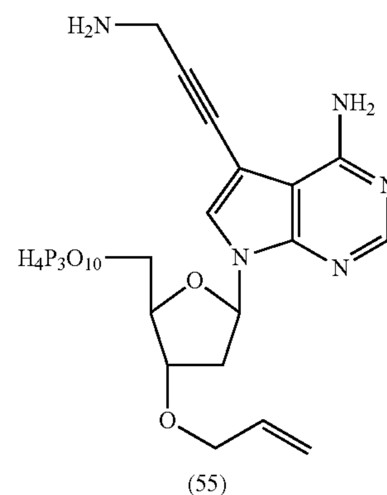
3'-O-Allyl-7-[3-aminoprop-1-ynyl]-7-deaza-2'-deoxyadenosine 5'-O-nucleoside triphosphate (55)
