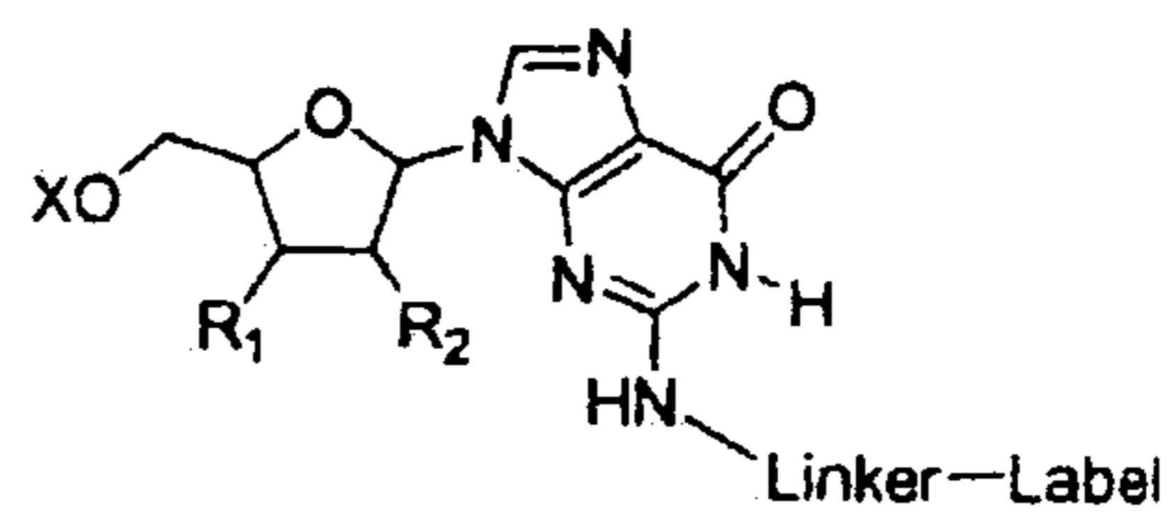
Guanosine N2-linker
