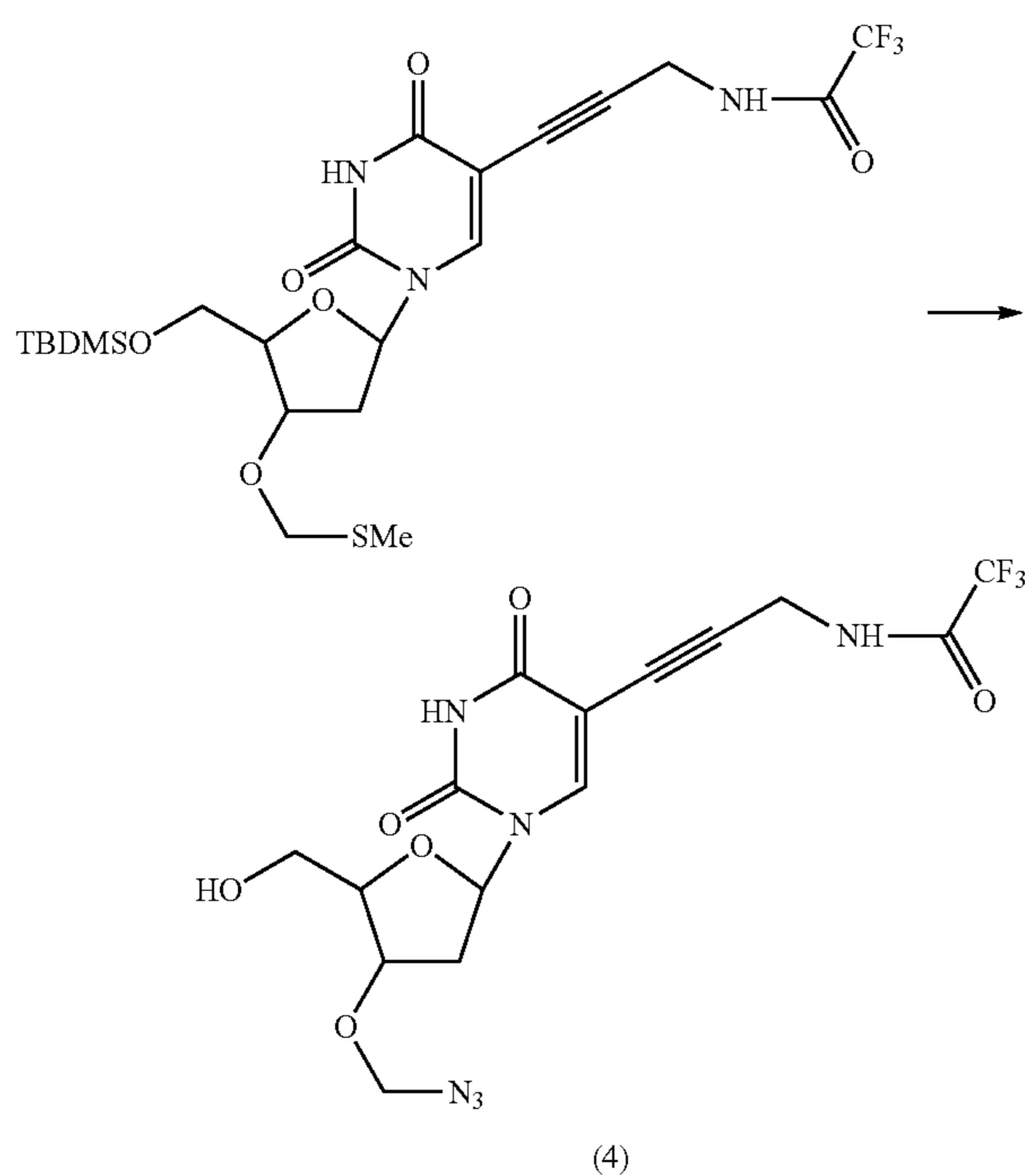
3'-O-Azidomethyl-5-[3-(2,2,2-trifluoroacetamido)-prop-1-ynyl]-2'-deoxyuridine (4)
