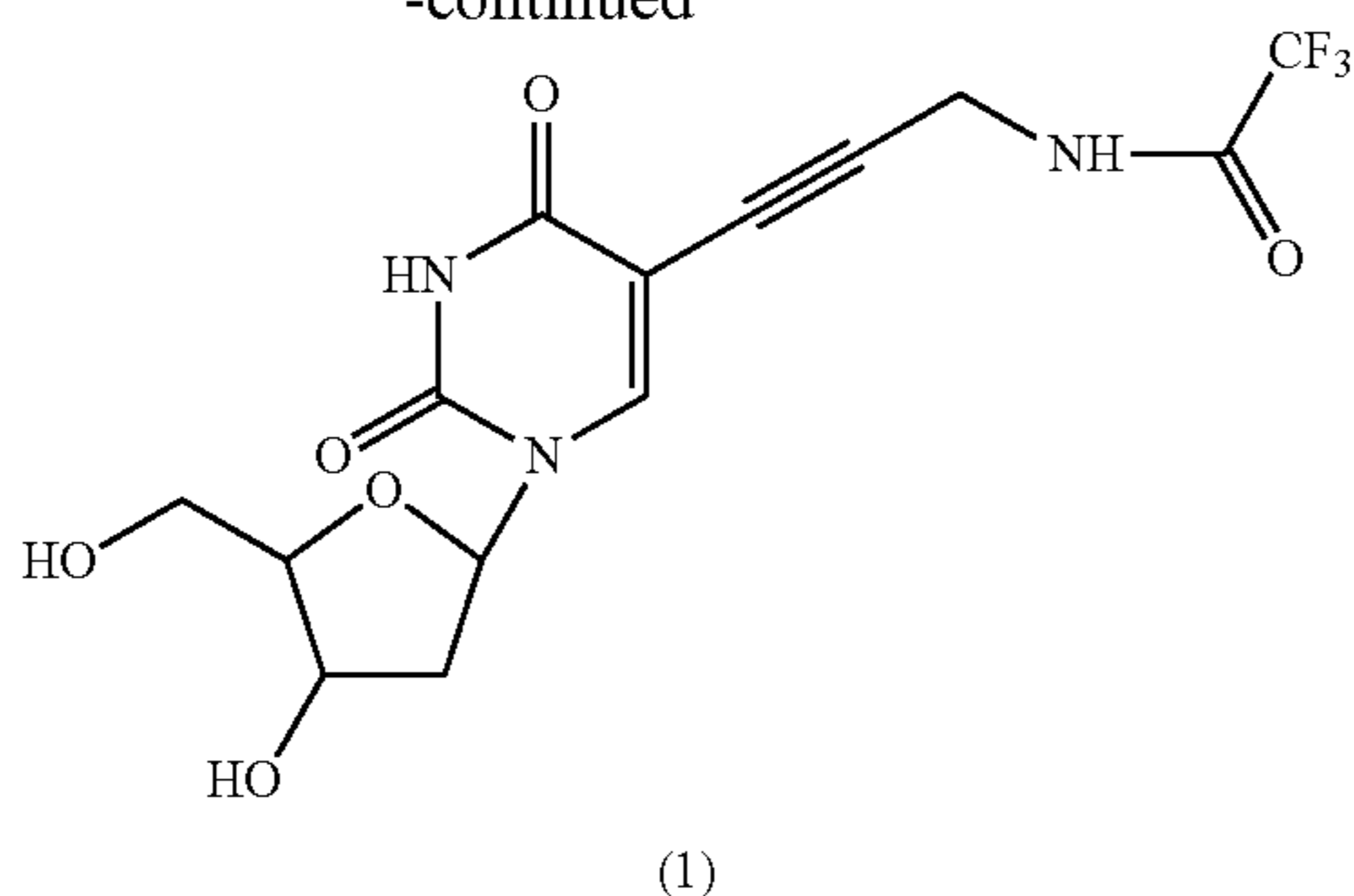
5-[3-(2,2,2-trifluoroacetamido)-prop-1-ynyl]-2'-deoxyuridine (1)
