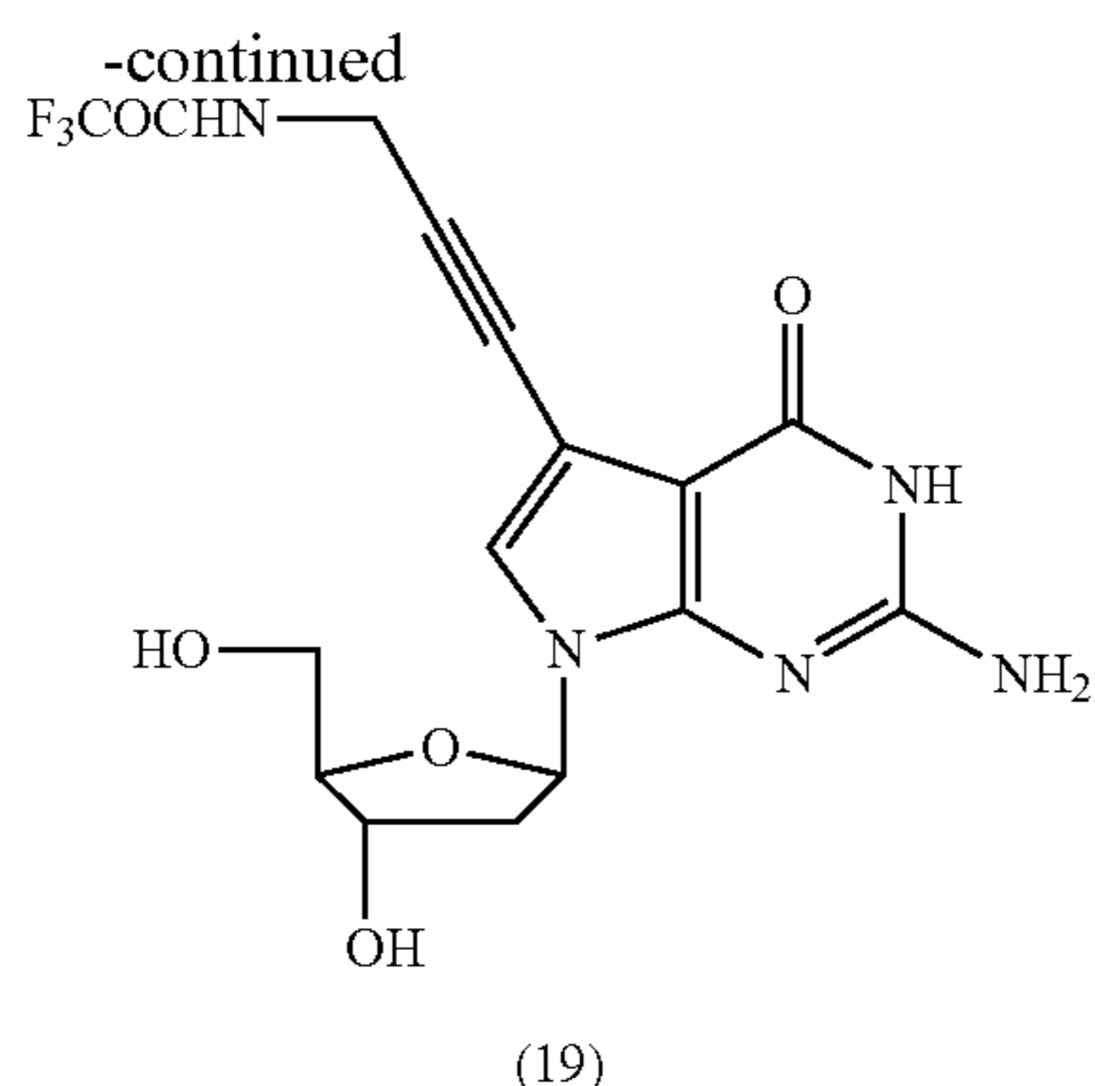
7-Deaza-[3-(2,2,2-trifluoroacetamido)-prop-1-ynyl]- 2'-deoxyguanosine (19)
