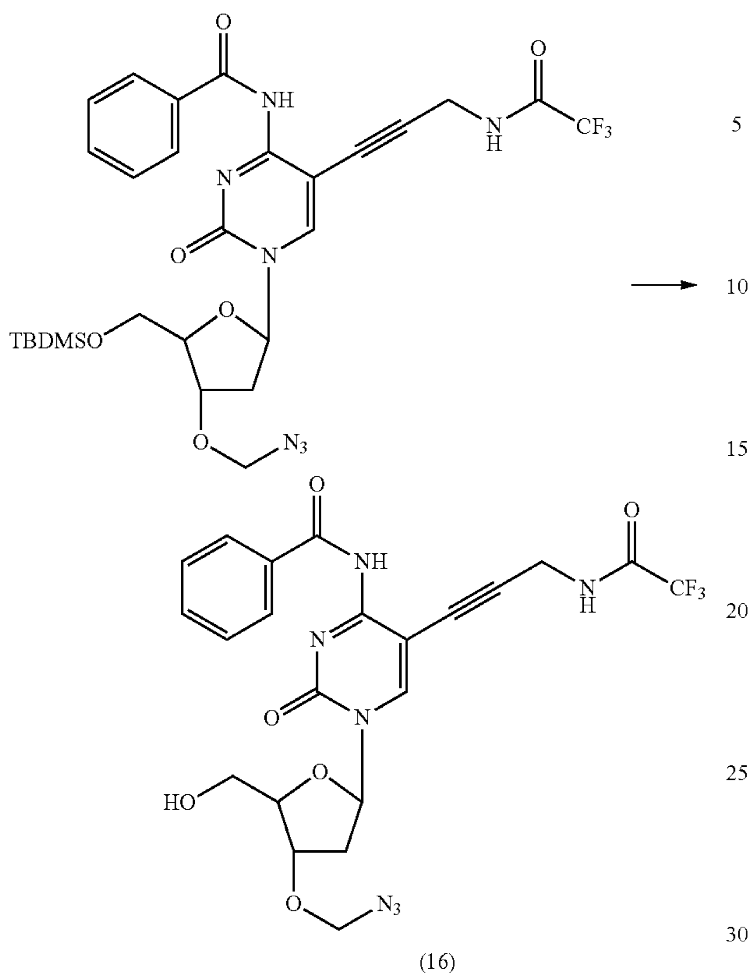
4-N-Benzoyl-3'-O-azidomethyl-5-[3-(2,2,2-trifluoroacetamido)-prop-1-ynyl]-2'-deoxycytidine (16)
