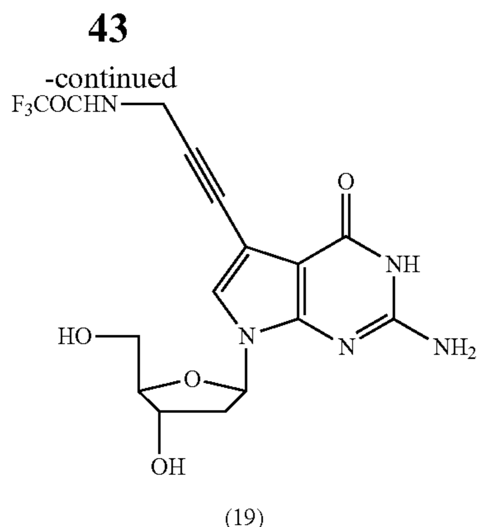
7-Deaza-[3-(2,2,2-trifluoroacetamido)-prop-1-ynyl]- 2'-deoxyguanosine (19)
