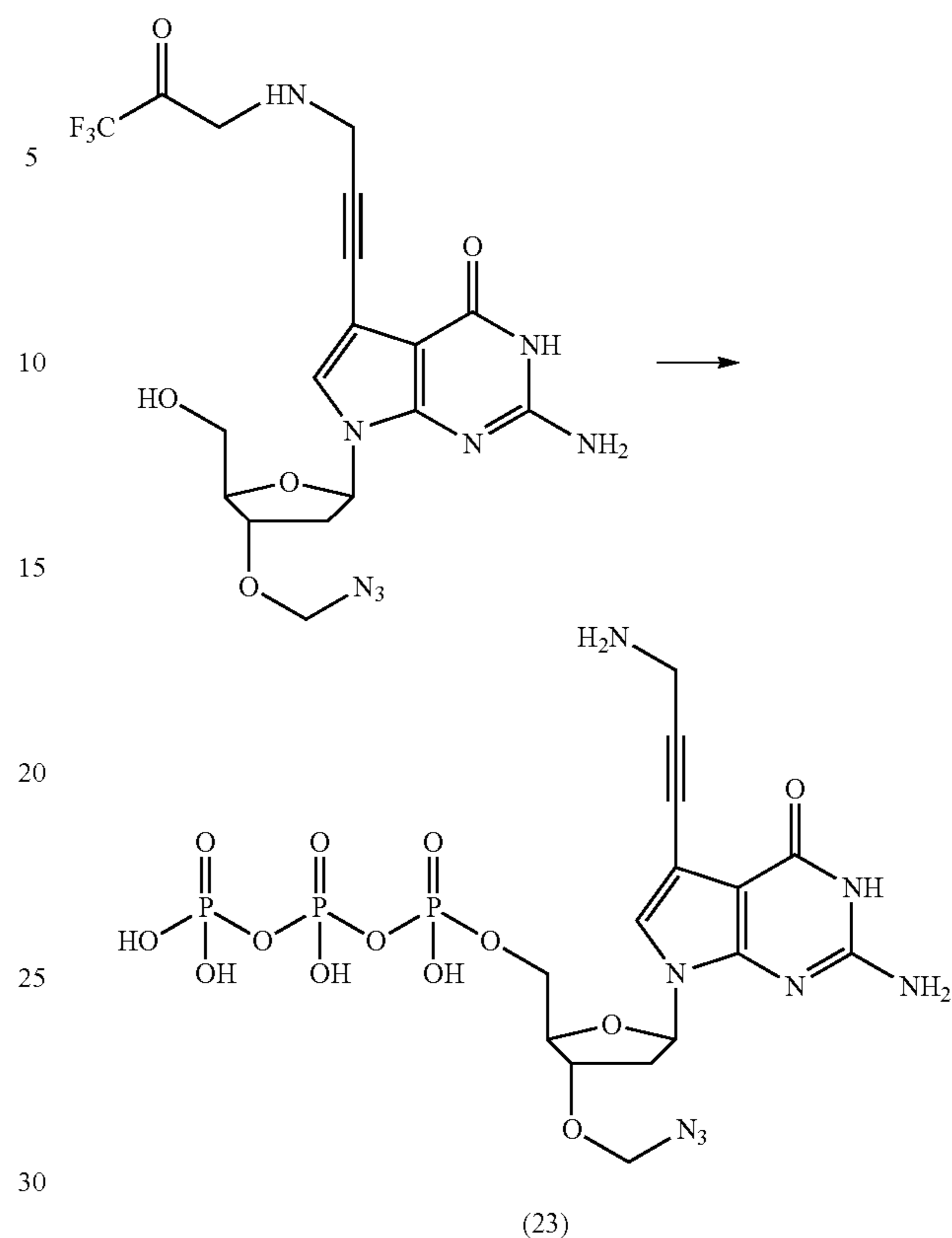
3'-O-Azidomethyl-7-deaza-7-[3-(2,2,2-trifluoroacetamido)-prop-1-ynyl]-2'-deoxyguanosine 5'-O-nucleoside triphosphate (23)
