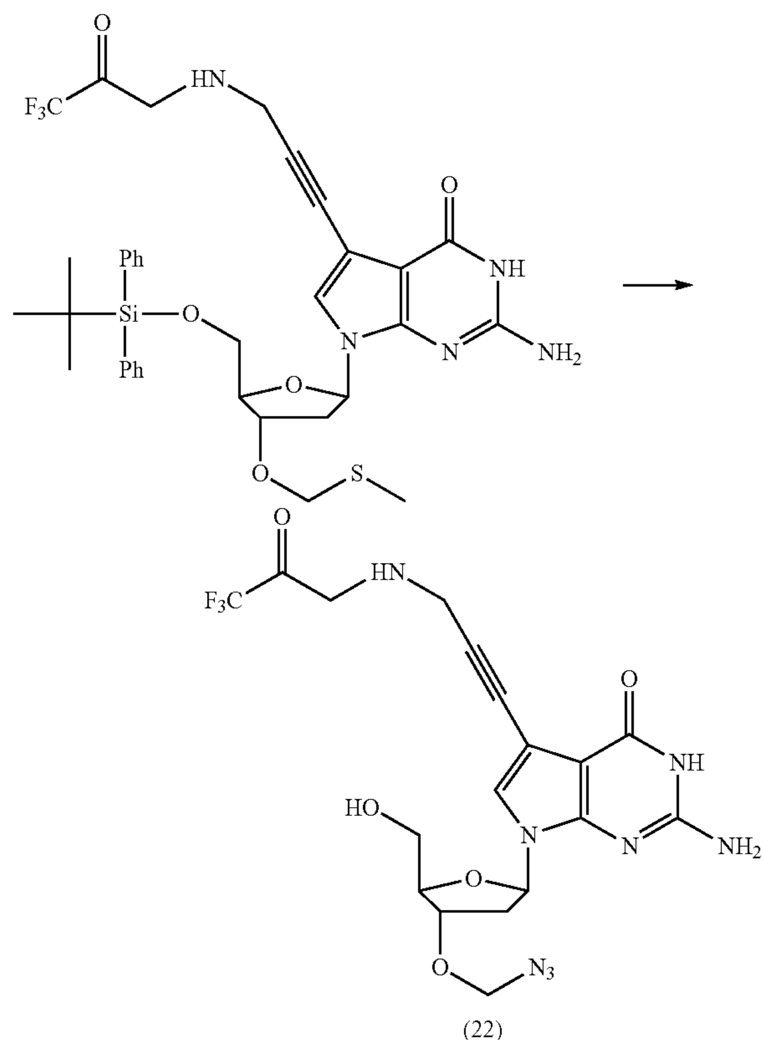
3'-O-Azidomethyl-7-deaza-7-[3-(2,2,2-trifluoroacetamido)-prop-1-ynyl]-2'-deoxyguanosine (22)
