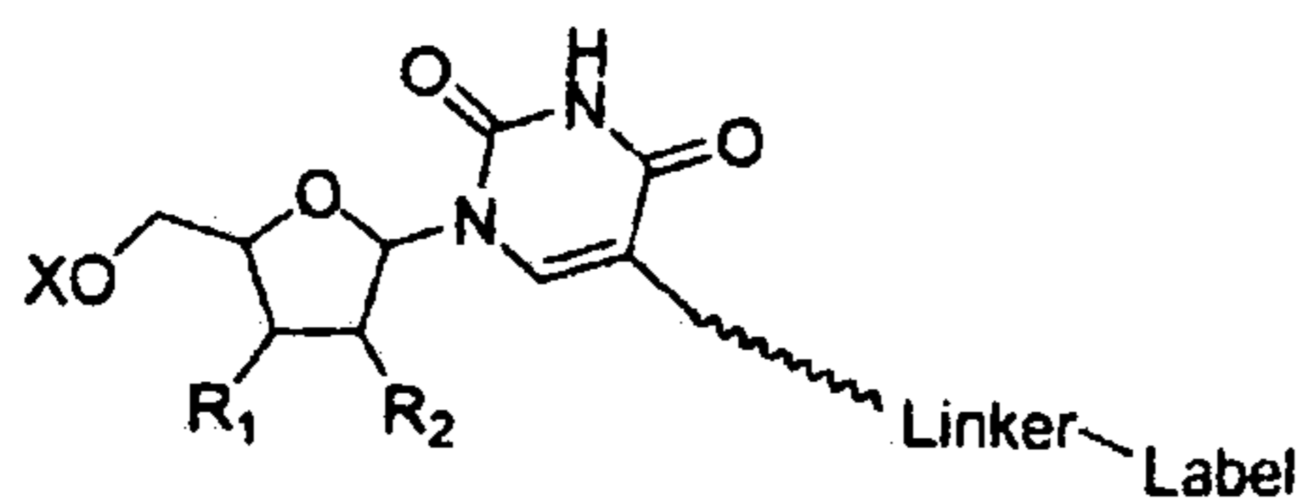
Uridine C5-linker
