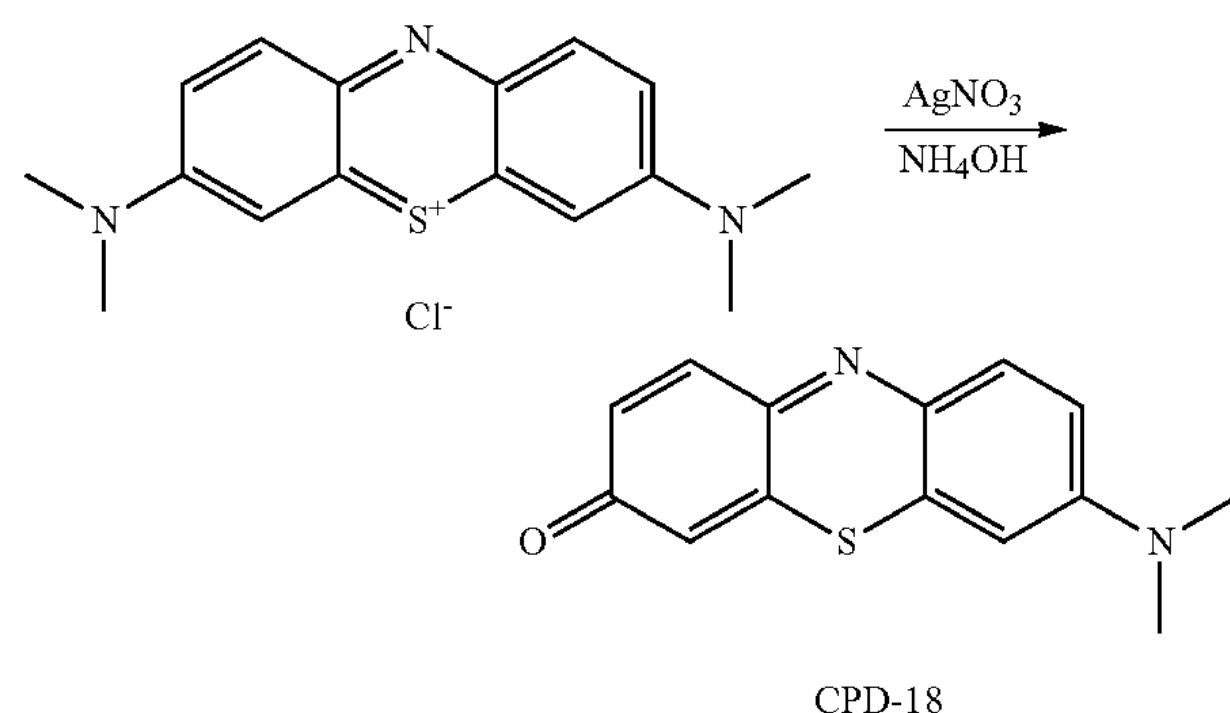
Scheme 7
