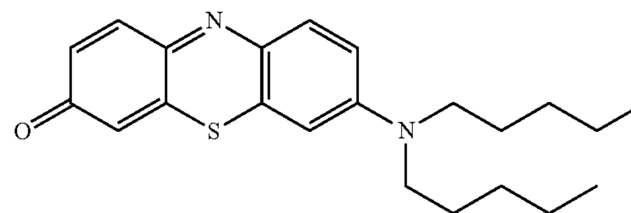
7-(dipentylamino)-3H-phenothiazine-3-one.
