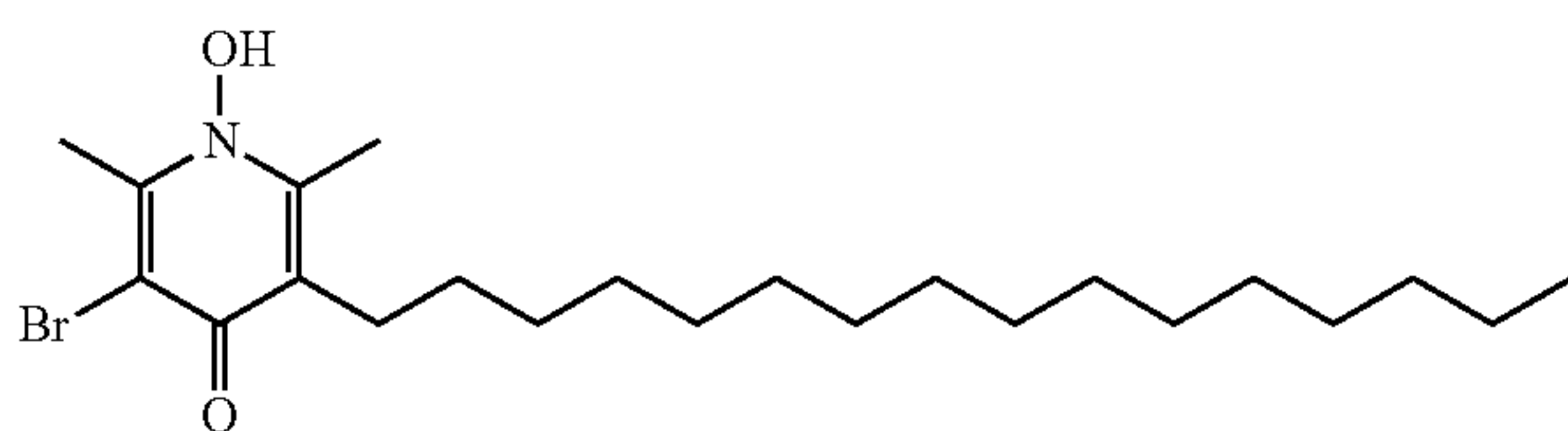
3-bromo-5-hexadecyl-1-hydroxy-2,6-dimethylpyridin-4(1H)-one (CPD-11)
