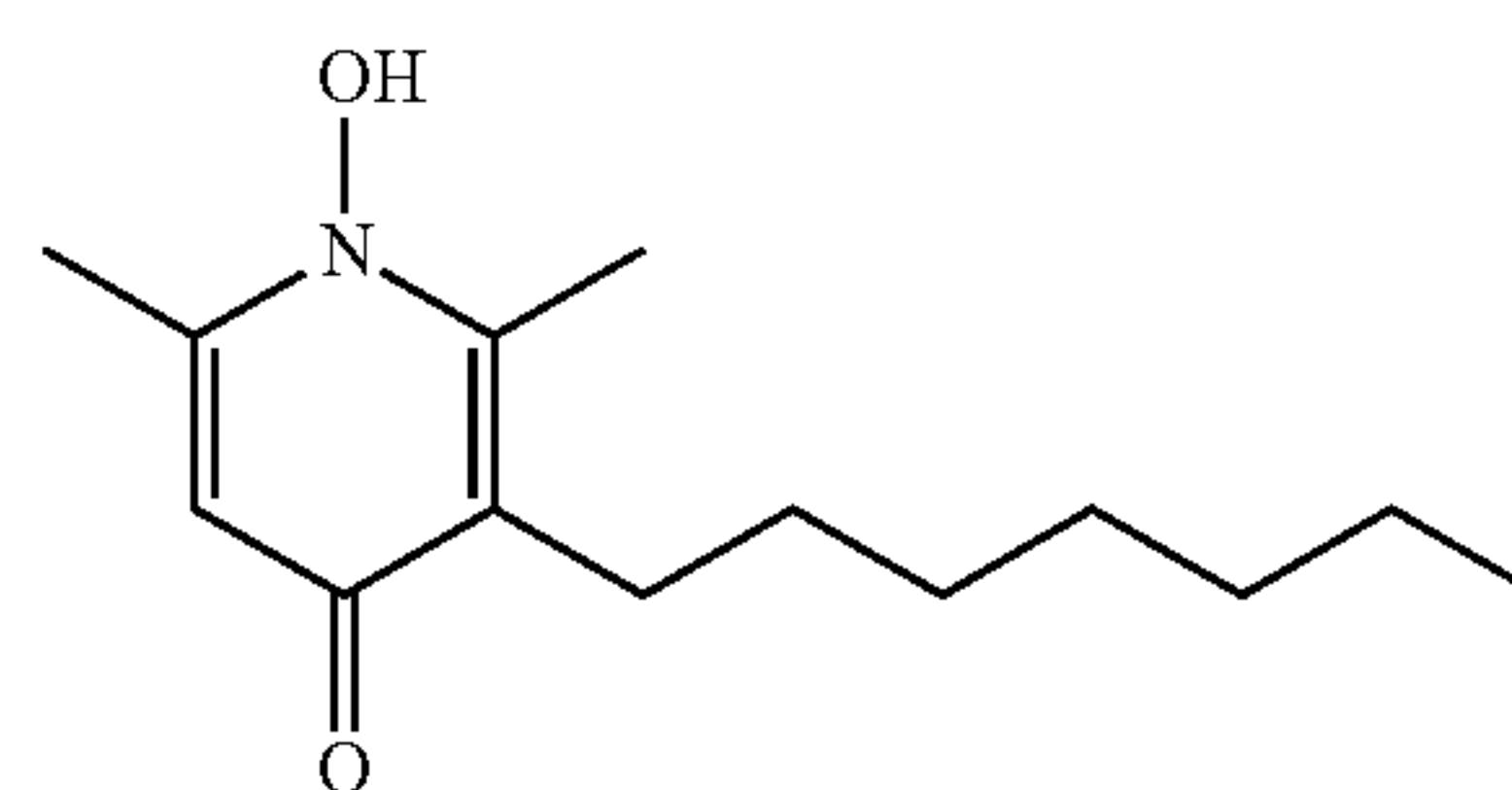
3-heptyl-1-hydroxy-2,6-dimethylpyridin-4(1H)-one (CPD-6)
