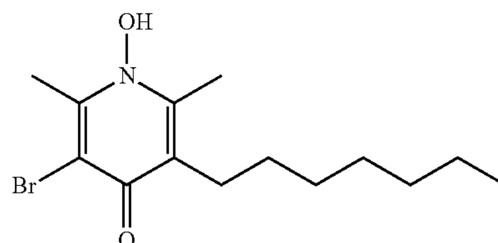
3-bromo-5-heptyl-1-hydroxy-2,6-dimethylpyridin-4(1H)-one (CPD-9)
