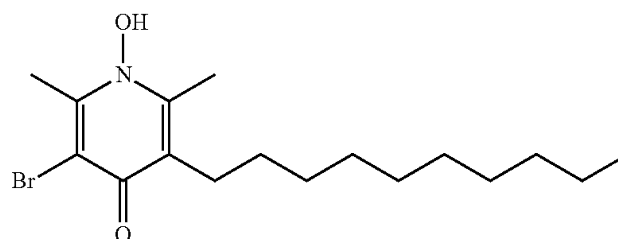
3-bromo-5-decyl-1-hydroxy-2,6-dimethylpyridin-4(1H)-one (CPD-10)
