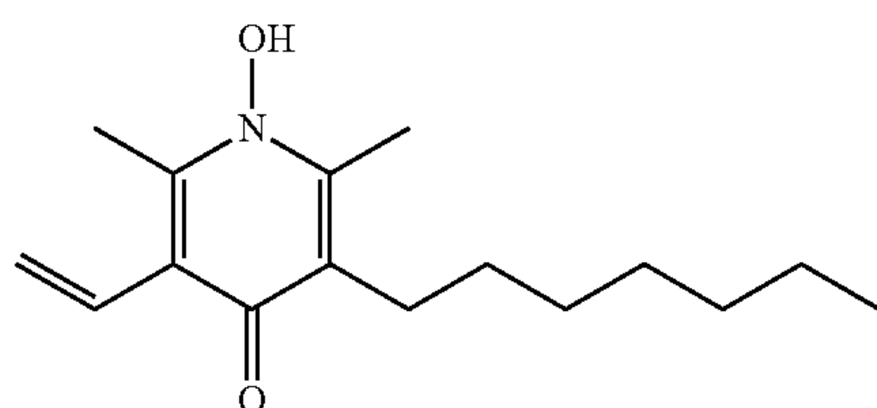
3-heptyl-1-hydroxy-2,6-dimethyl-5-vinylpyridin-4(1H)-one (CPD-1)
