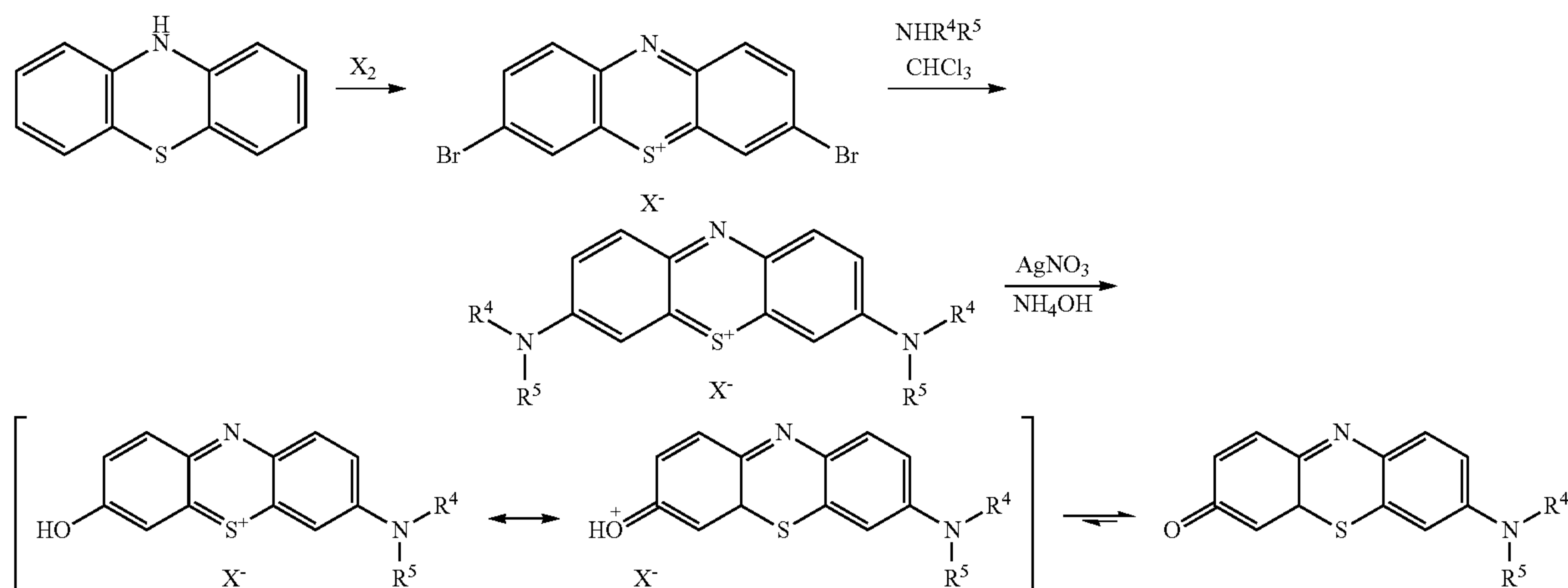
Scheme 6
