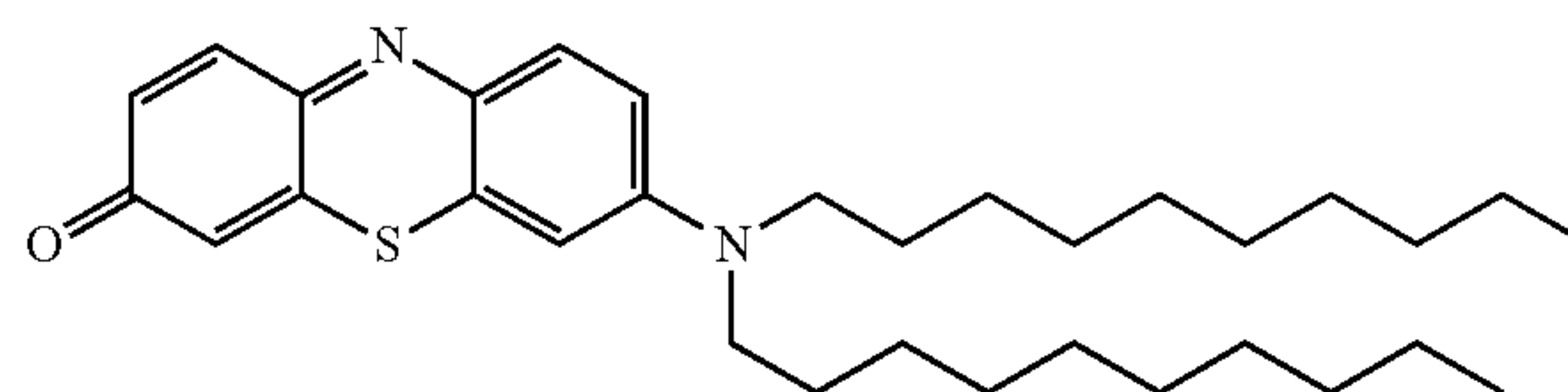
7-(didecylamino)-3H-phenothiazine-3-one; or
