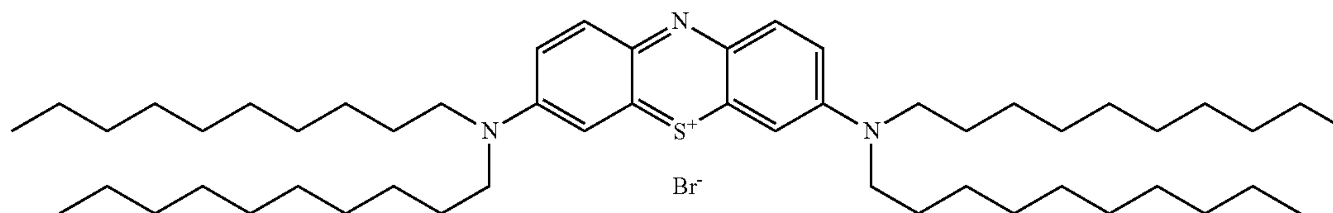
3,7-bis(didecylamino)phenothiazin-5-ium bromide 15 (CPD-14)
