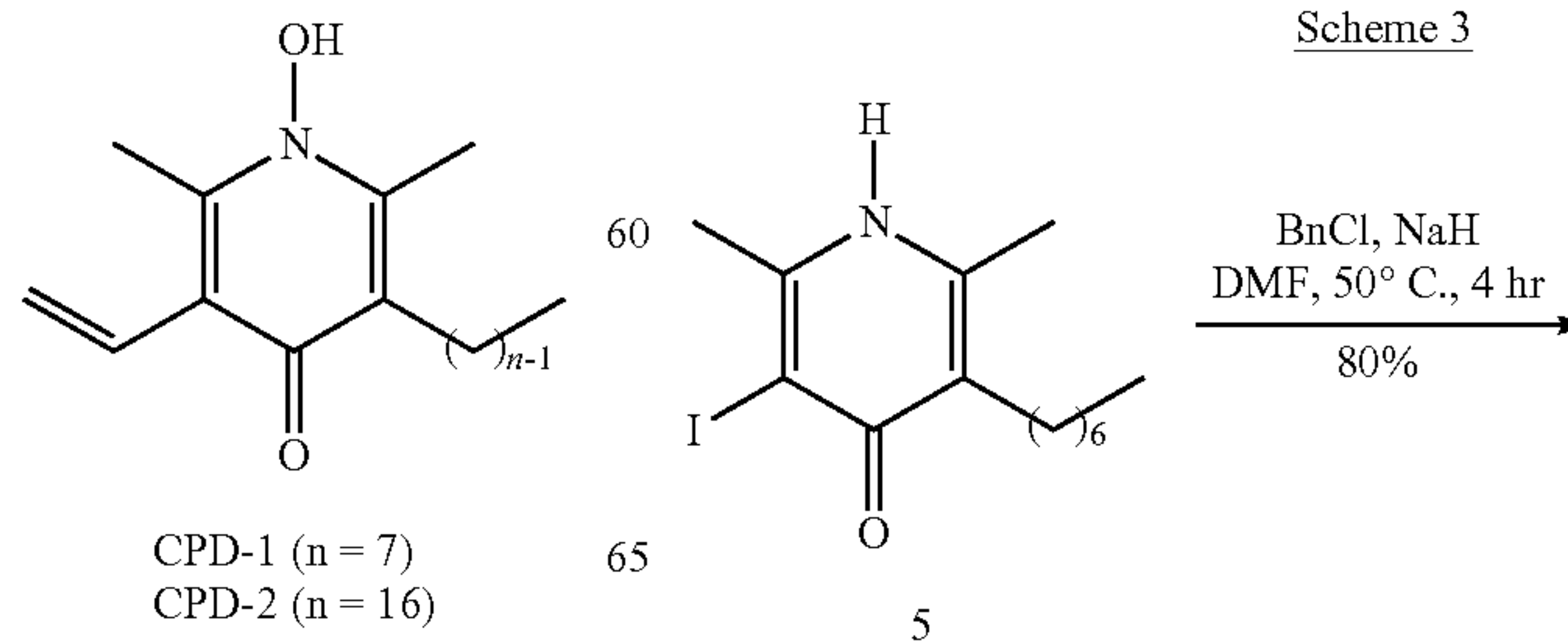
Scheme 3
