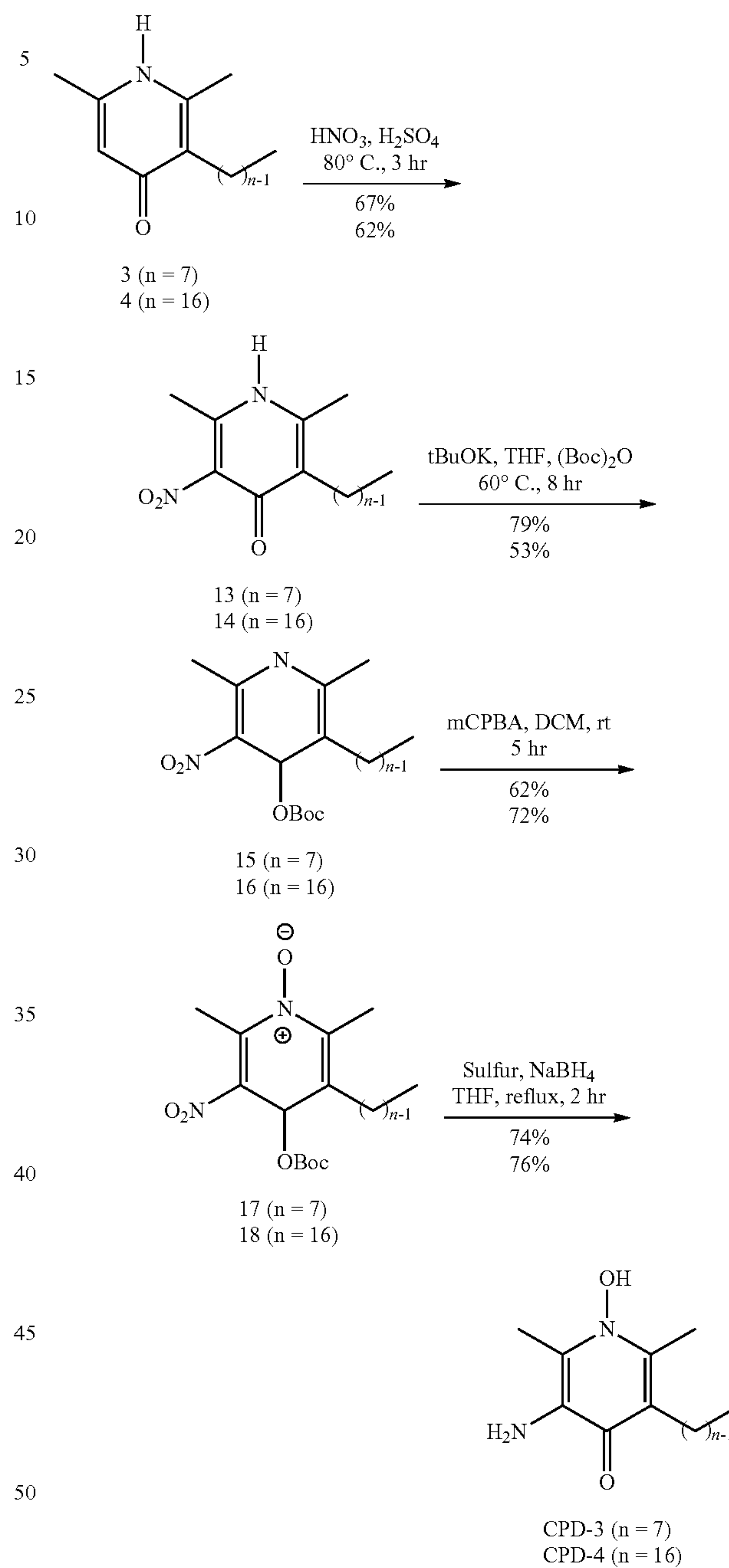
Scheme 2
