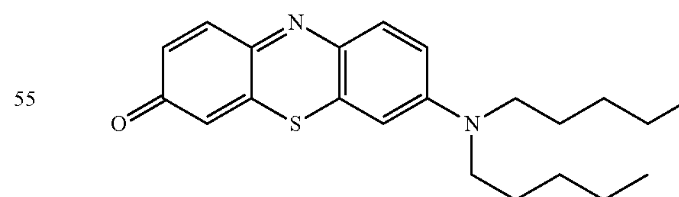
3,7-bis(dipentylamino)phenothiazin-5-ium bromide 50 (CPD-15)
