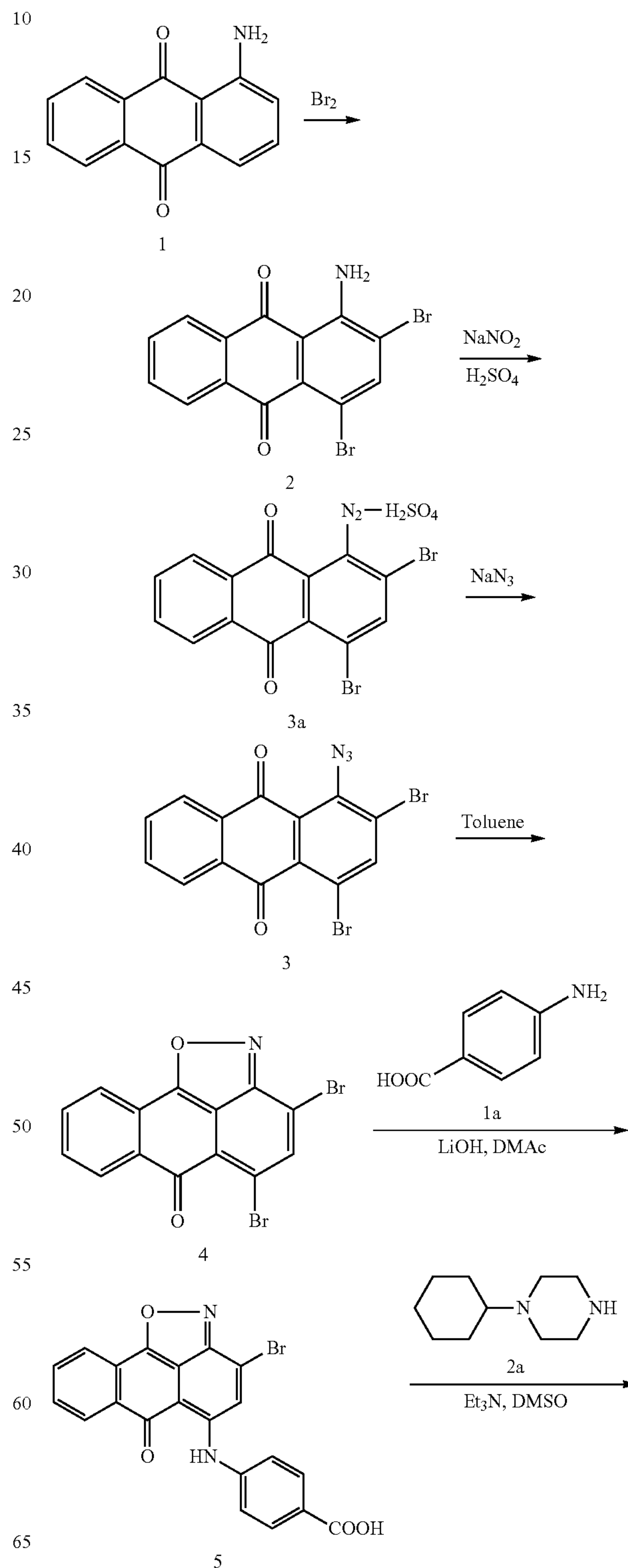
Sodium 4-((3-(4-cyclohexylpiperazin-1-yl)-6-oxo-6H-anthra[1,9-cd]isoxazol-5-yl)amino)benzoate
