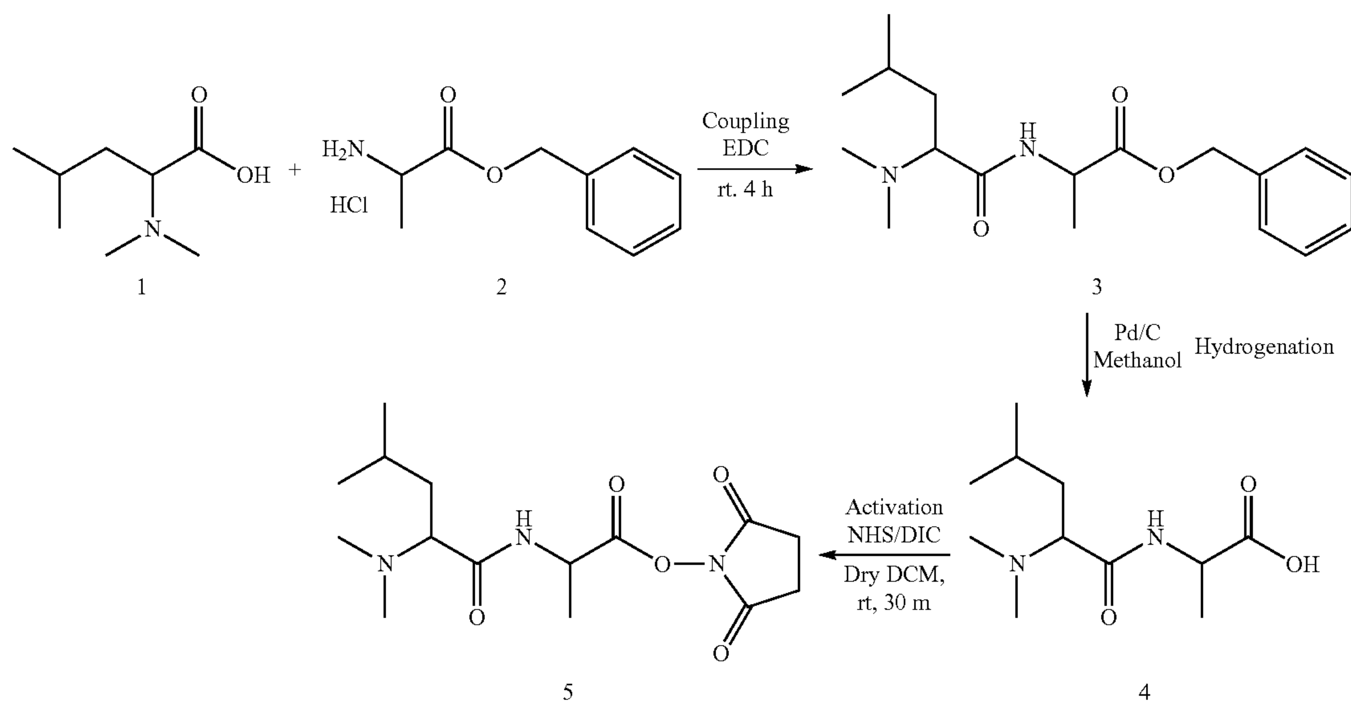
Scheme 5 - Alternate general synthesis route of 8-plex reagent
