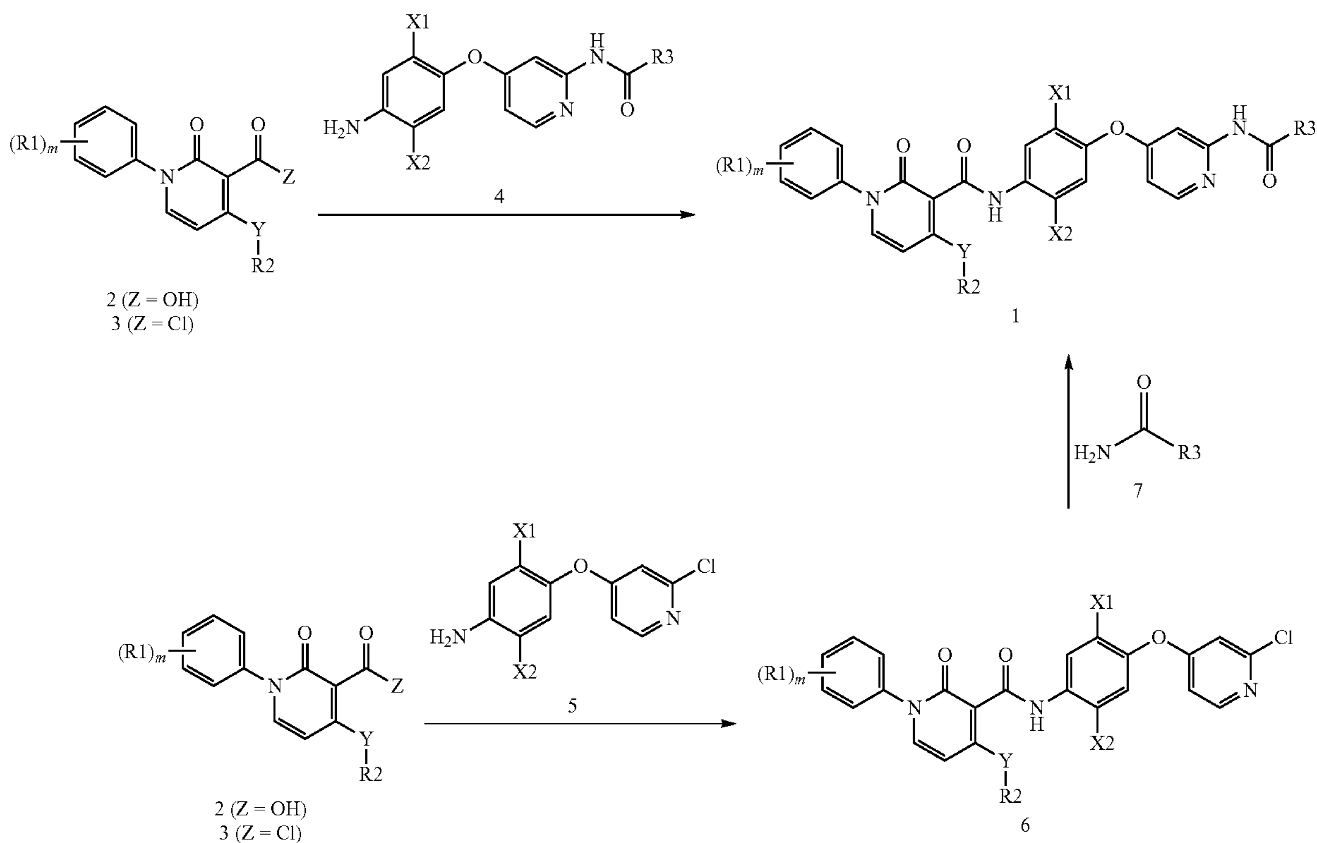
Scheme 1
