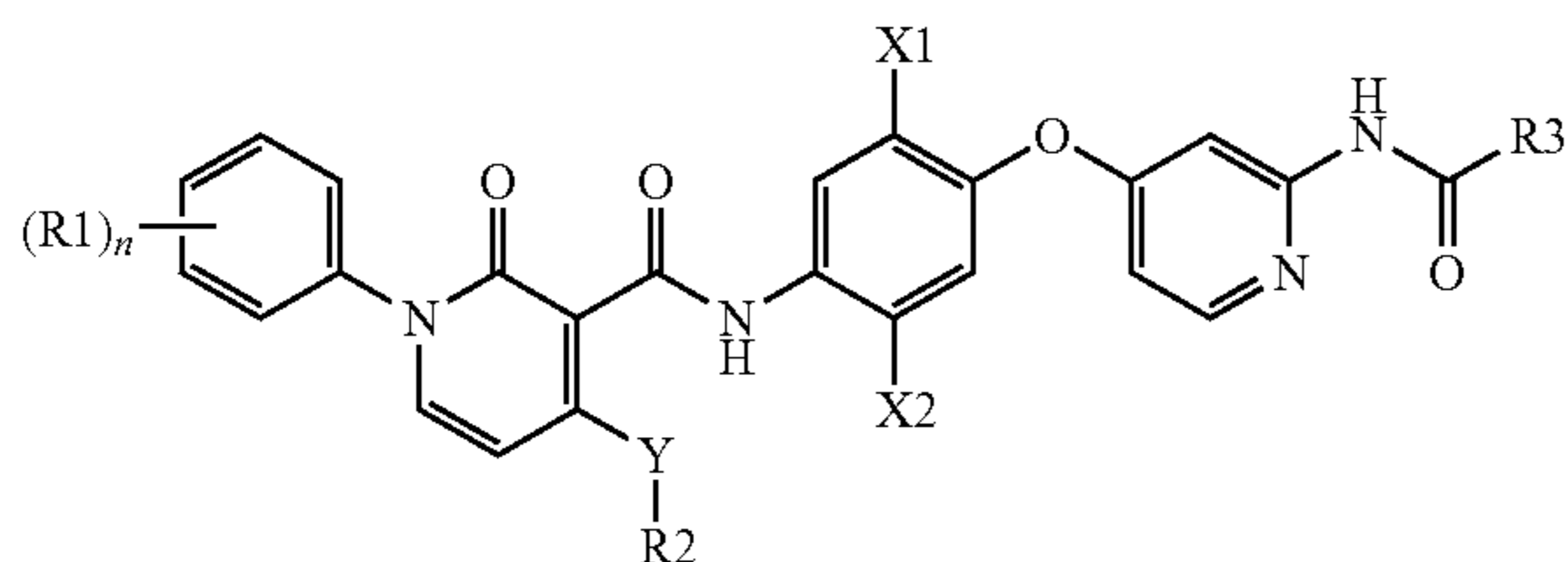
Formula I
