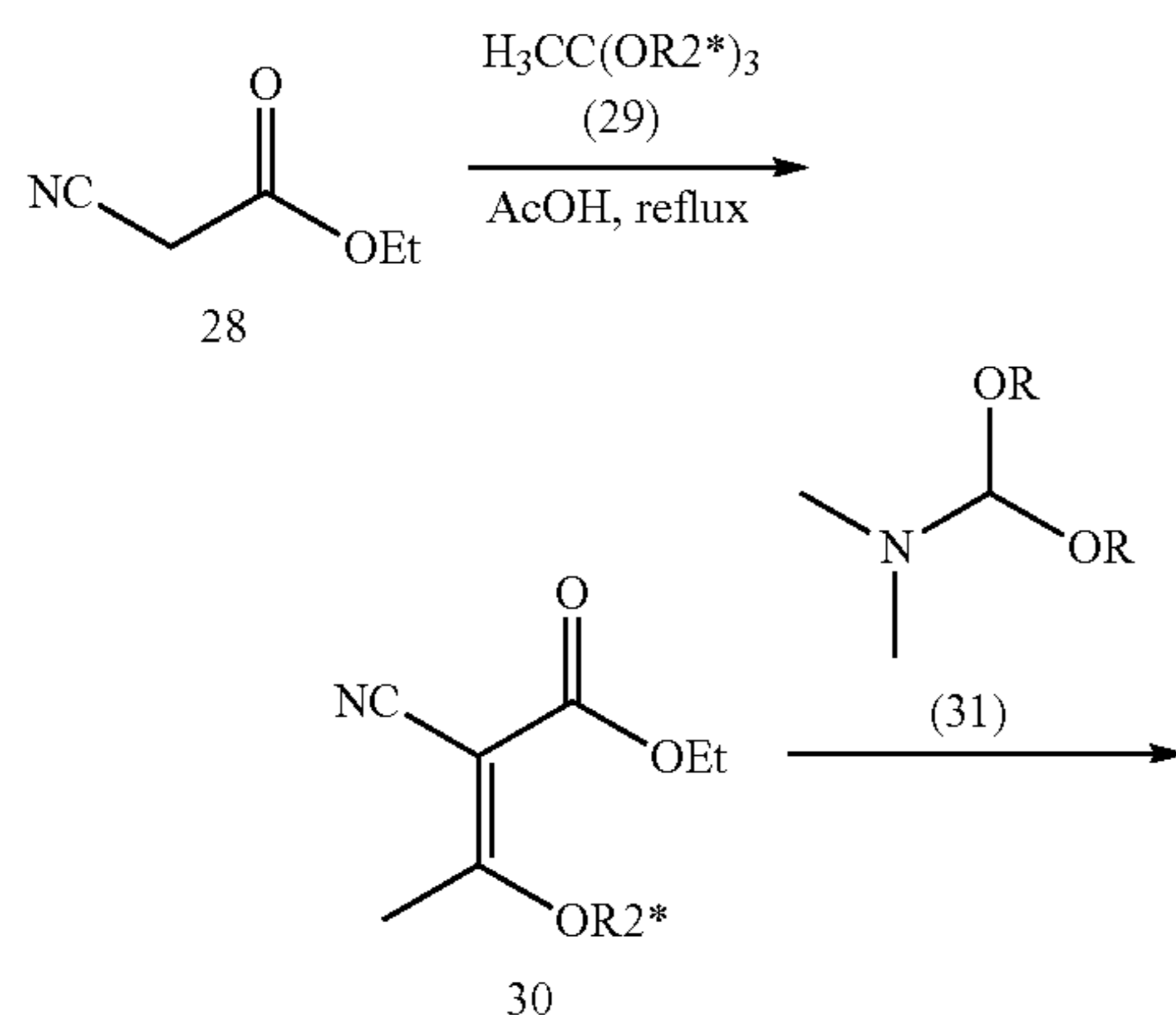
Scheme 6
