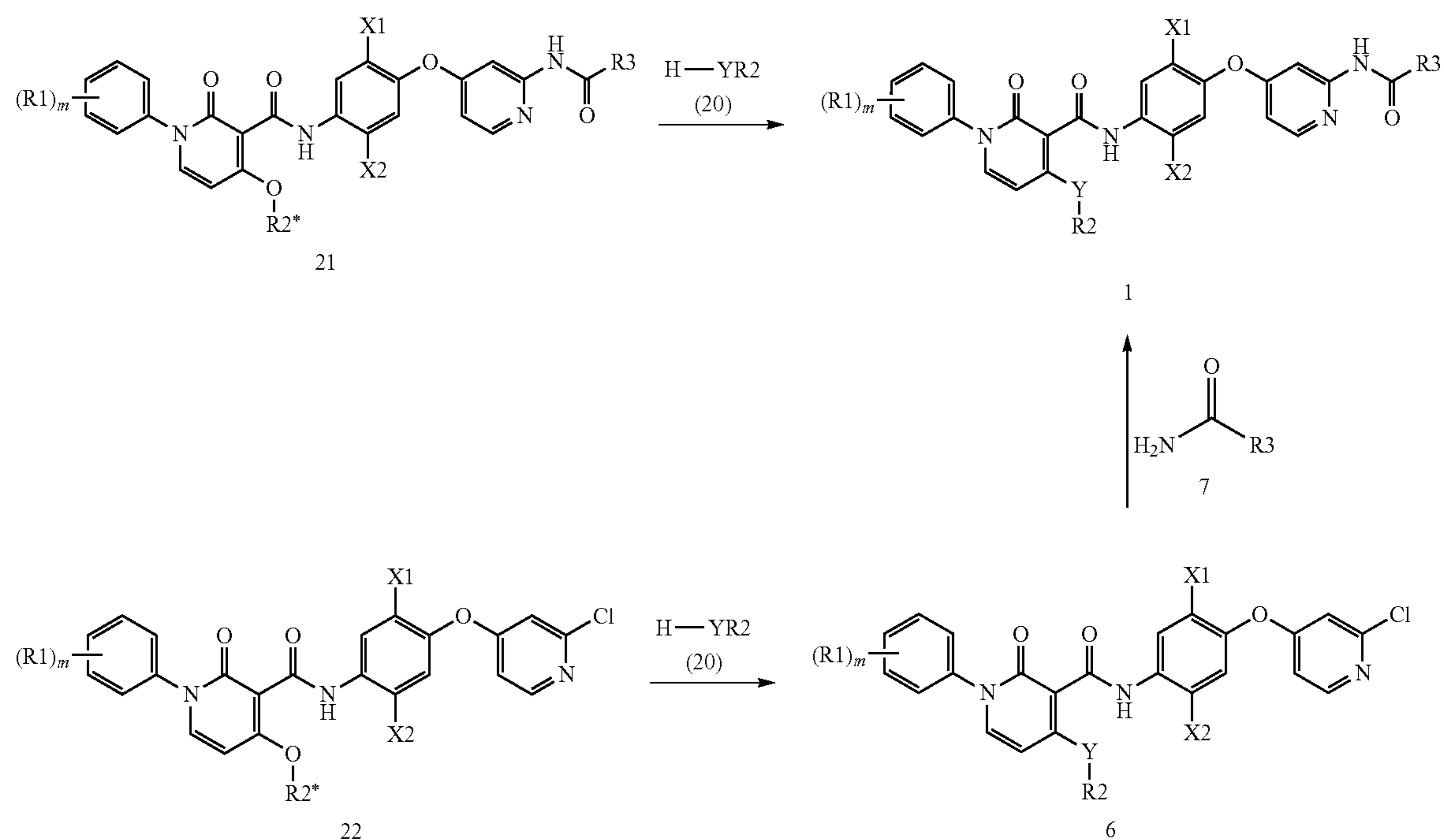
Scheme 4
