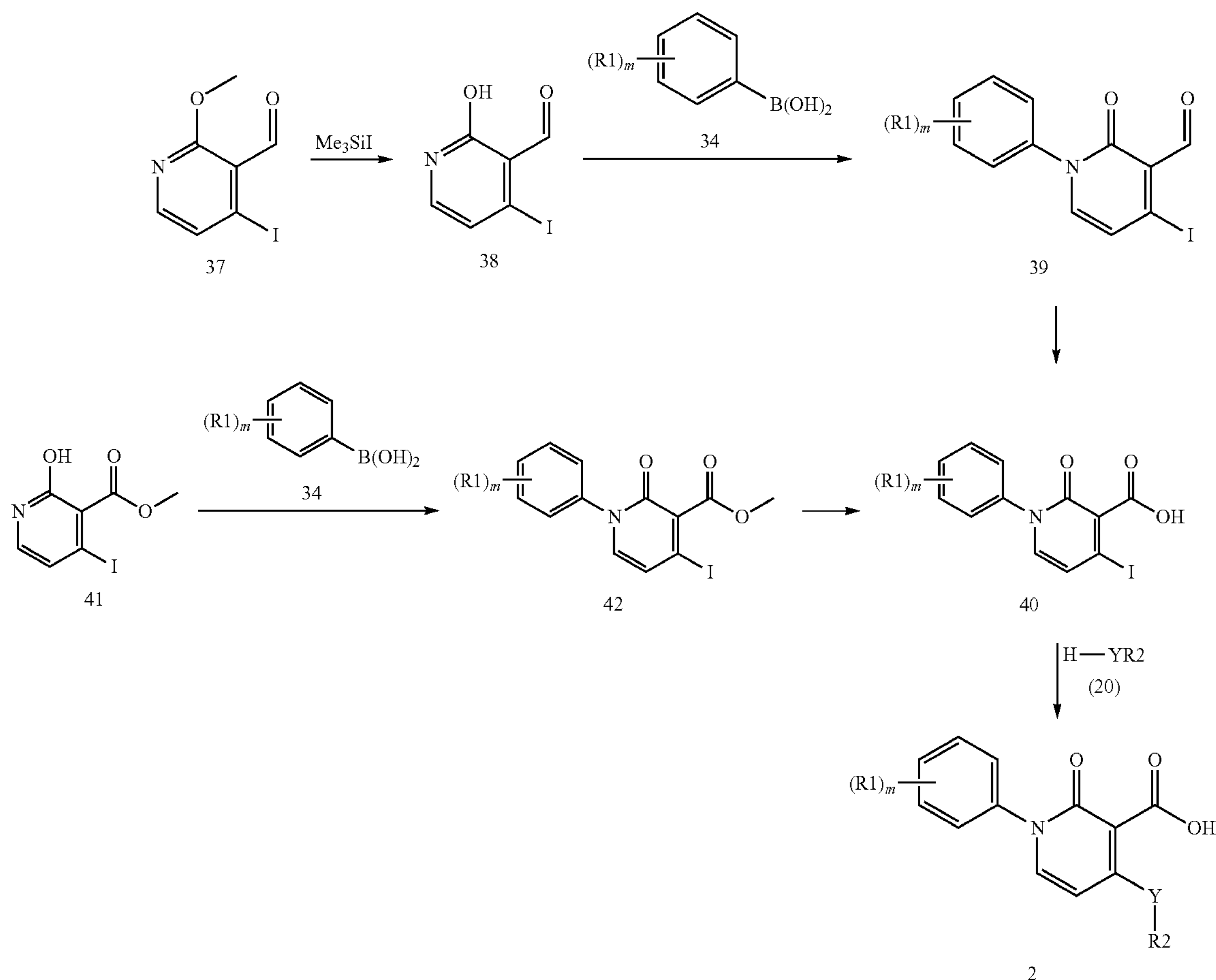
Scheme 7
