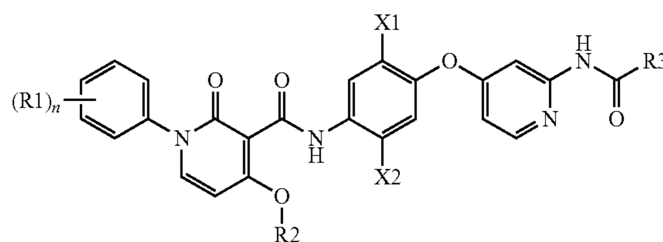
Formula Ia.1
