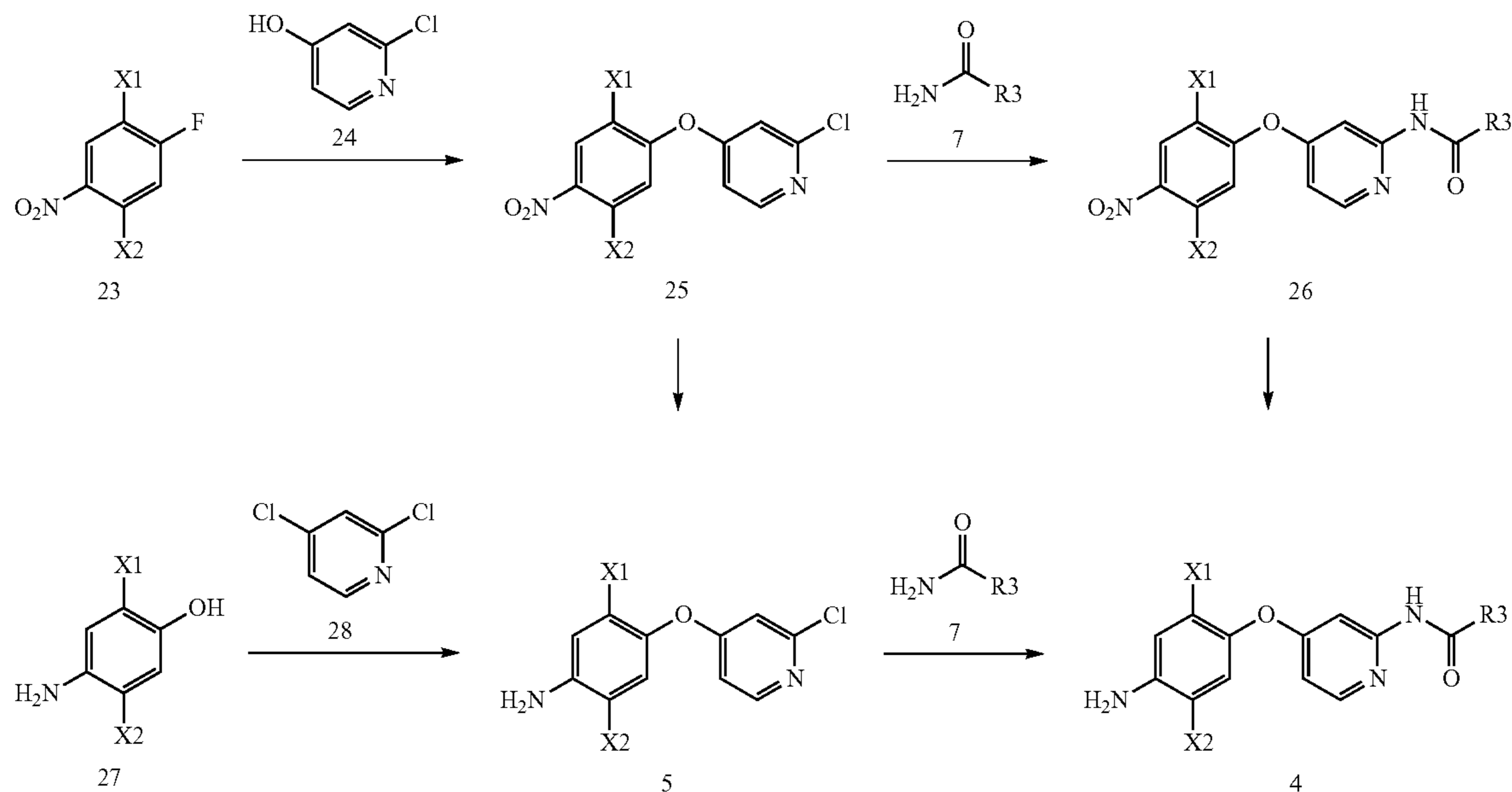
Scheme 5
