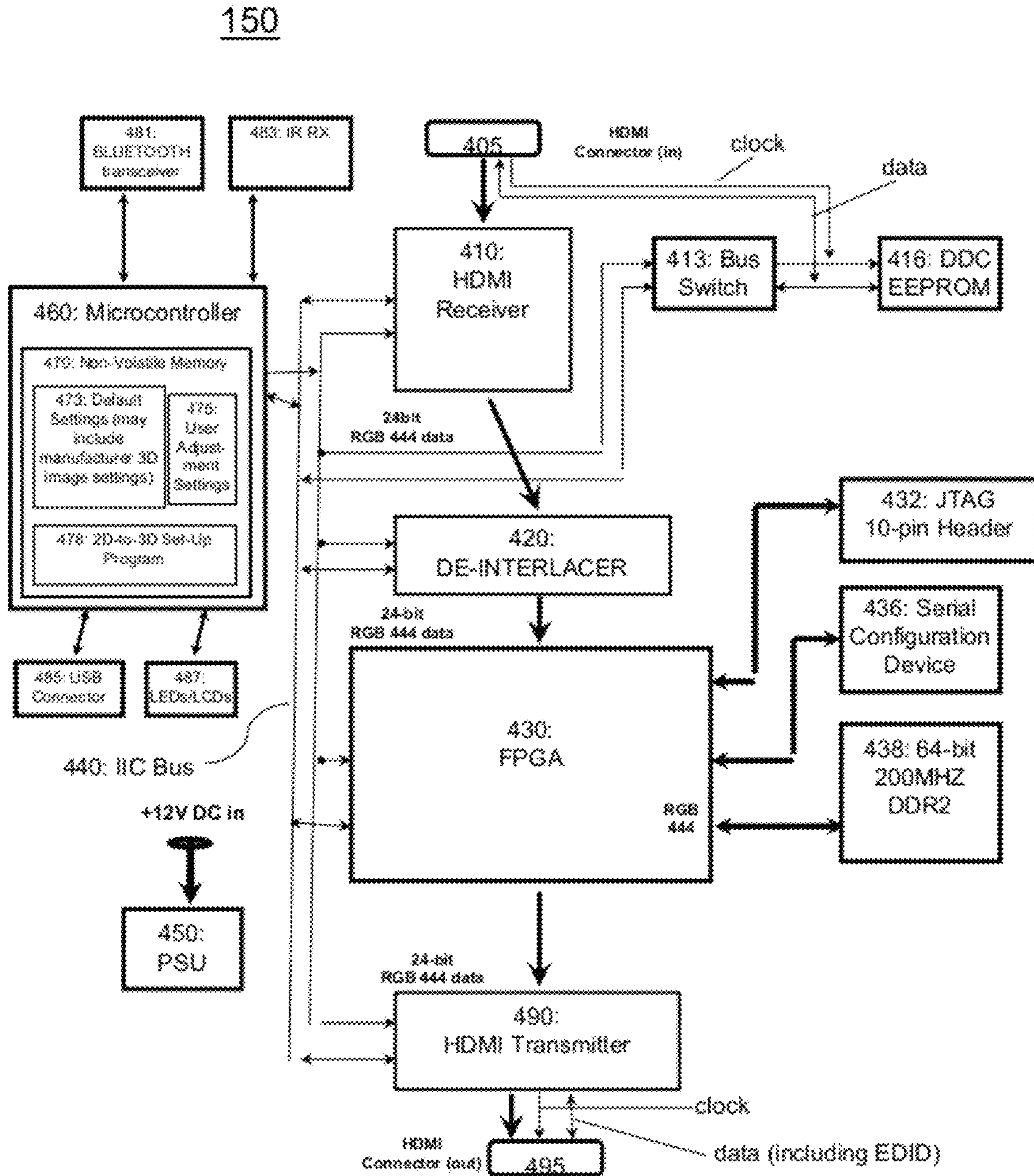
FIG. 4: 2D-to-3D converter block diagram
