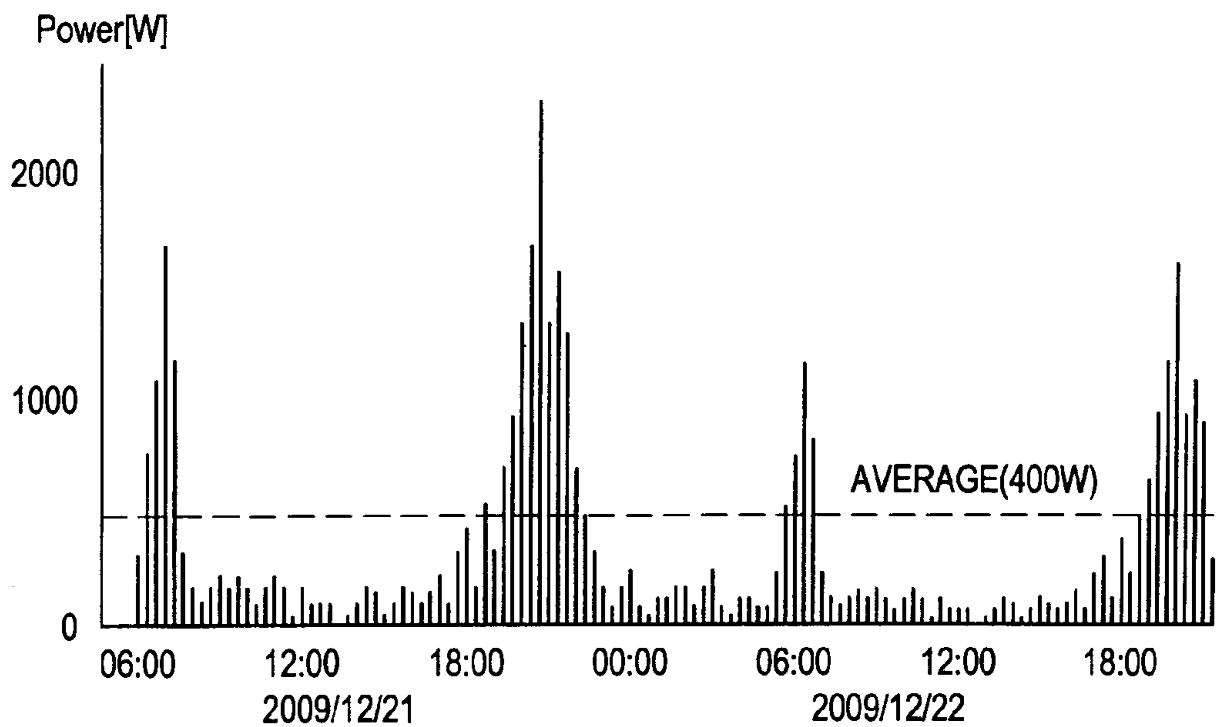
(B) EXAMPLE OF POWER CONSUMPTION PATTERN
