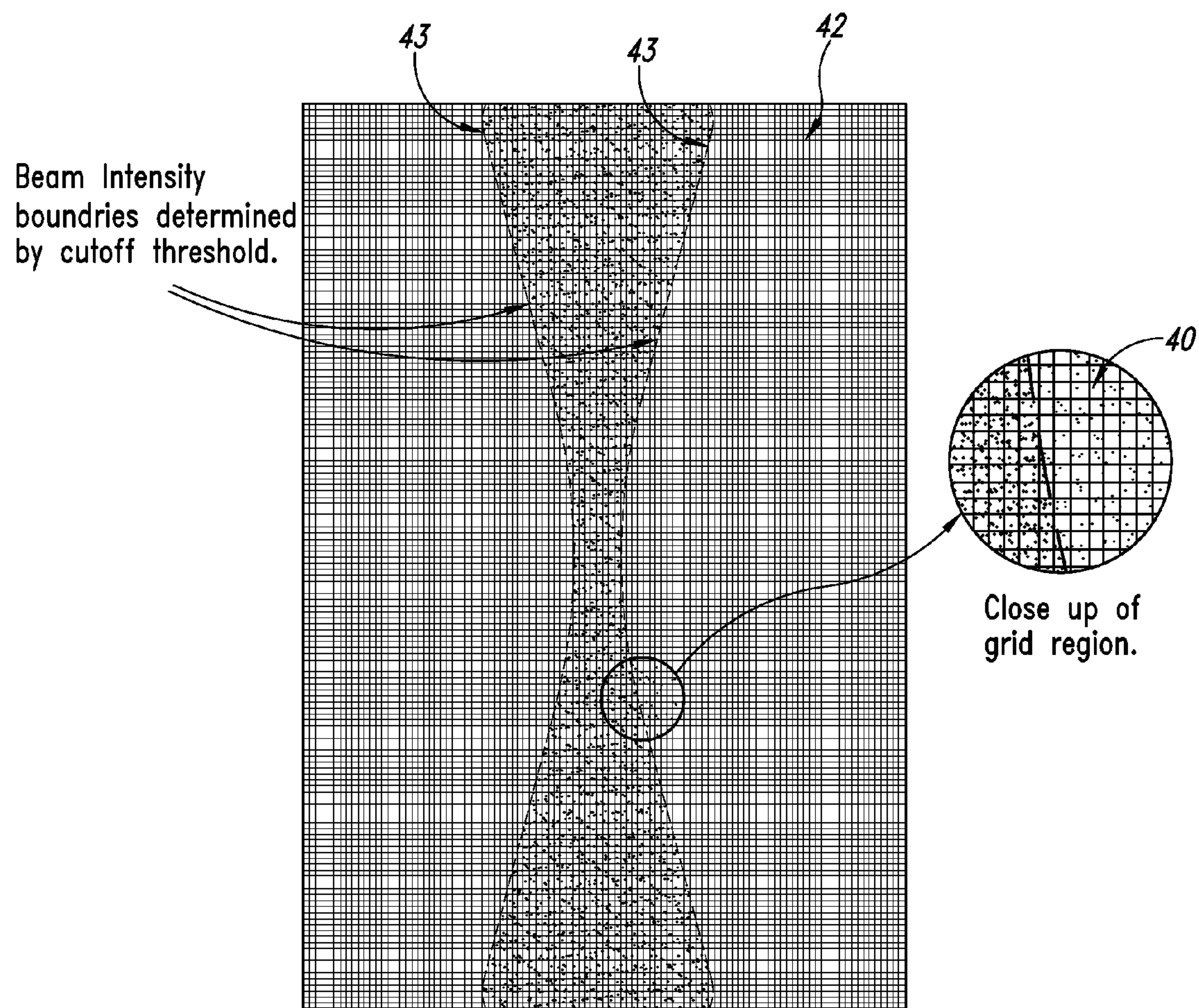
Maximum Intensity of transmit beam at grid of field points, showing boundaries determined by cutoff threshold. The magnitude of the intensity is indicated by the darkness of the grayscale at the field point.
