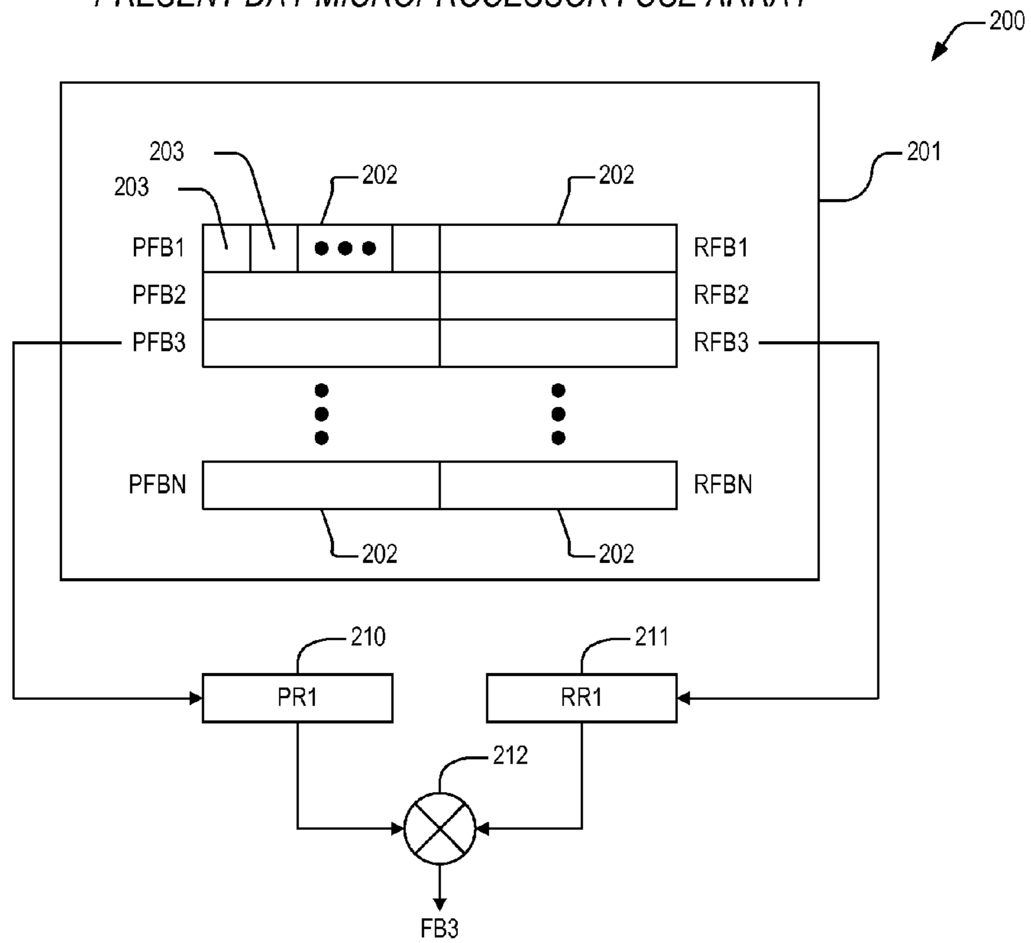
FIG. 2 (Prior Art)
