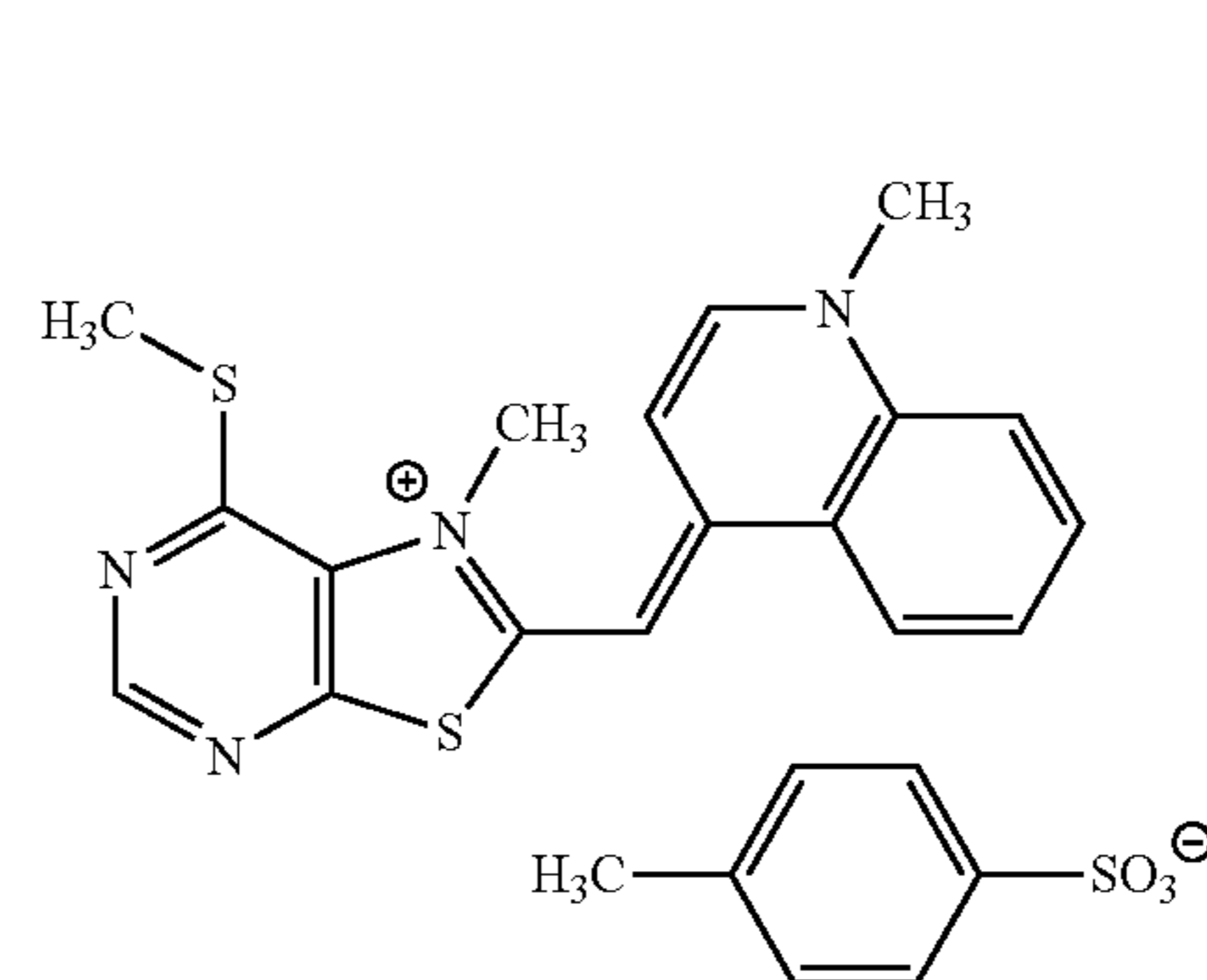
Compound 35
