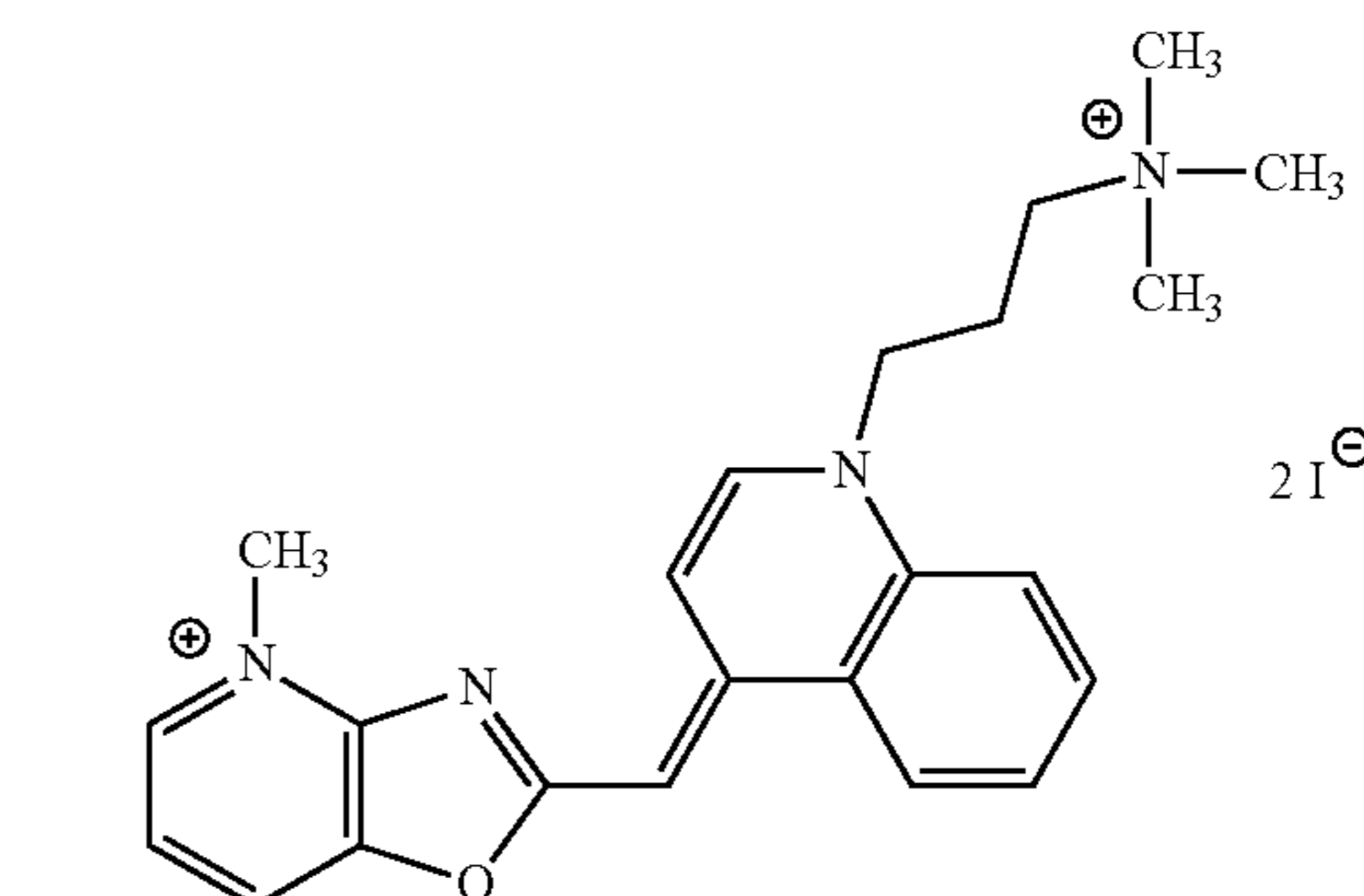
Compound 27
