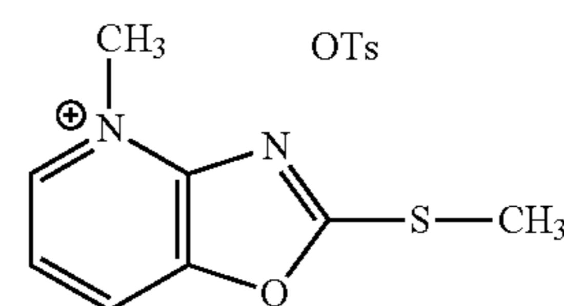
4-methyl-2-methylthioxazolopyridinium tosylate
