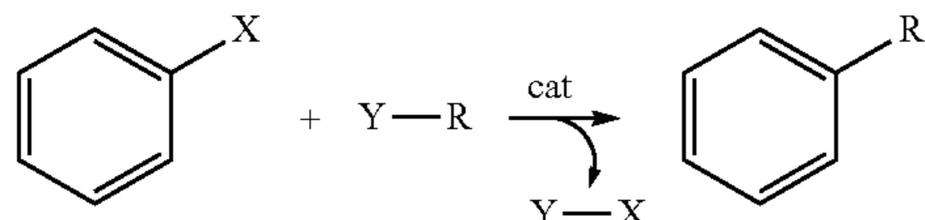
Scheme 2-1. New mode of arene functionalization vs. traditional cross-coupling approach.
