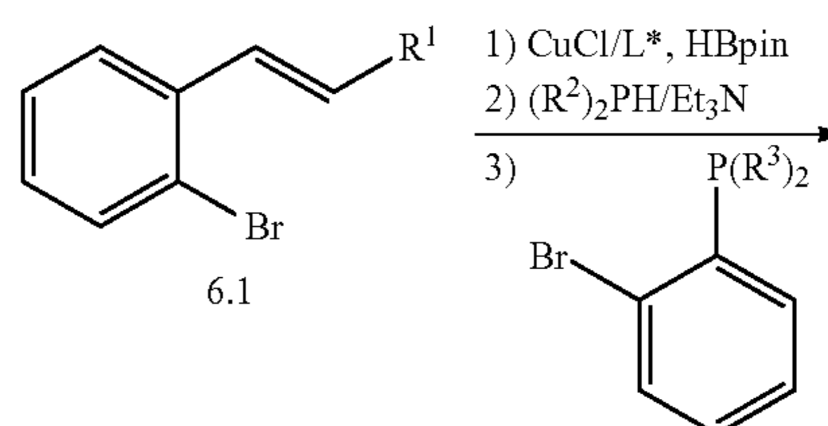
Scheme 6. Trans-spanning ligands.
