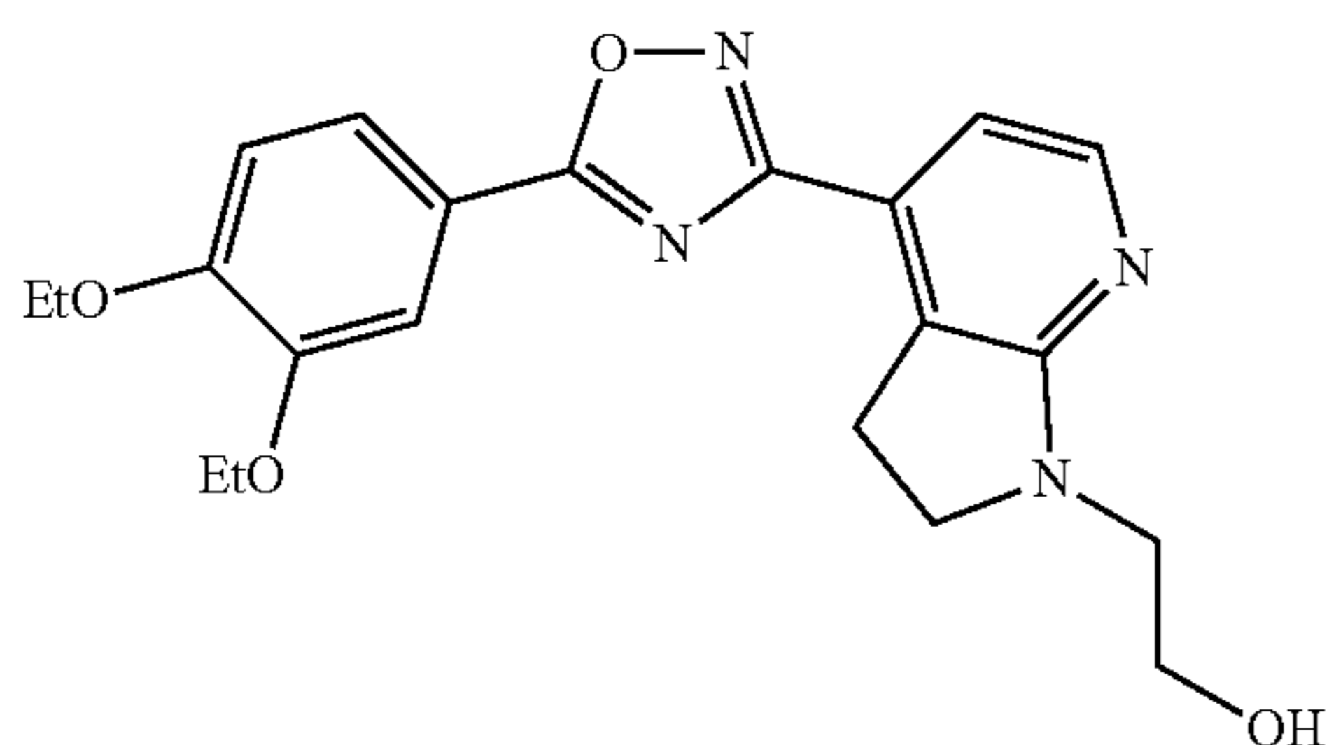
2-(4-(5-(3,4-diethoxyphenyl)-1,2,4-oxadiazol-3-yl)indolin-1-yl)ethanol
