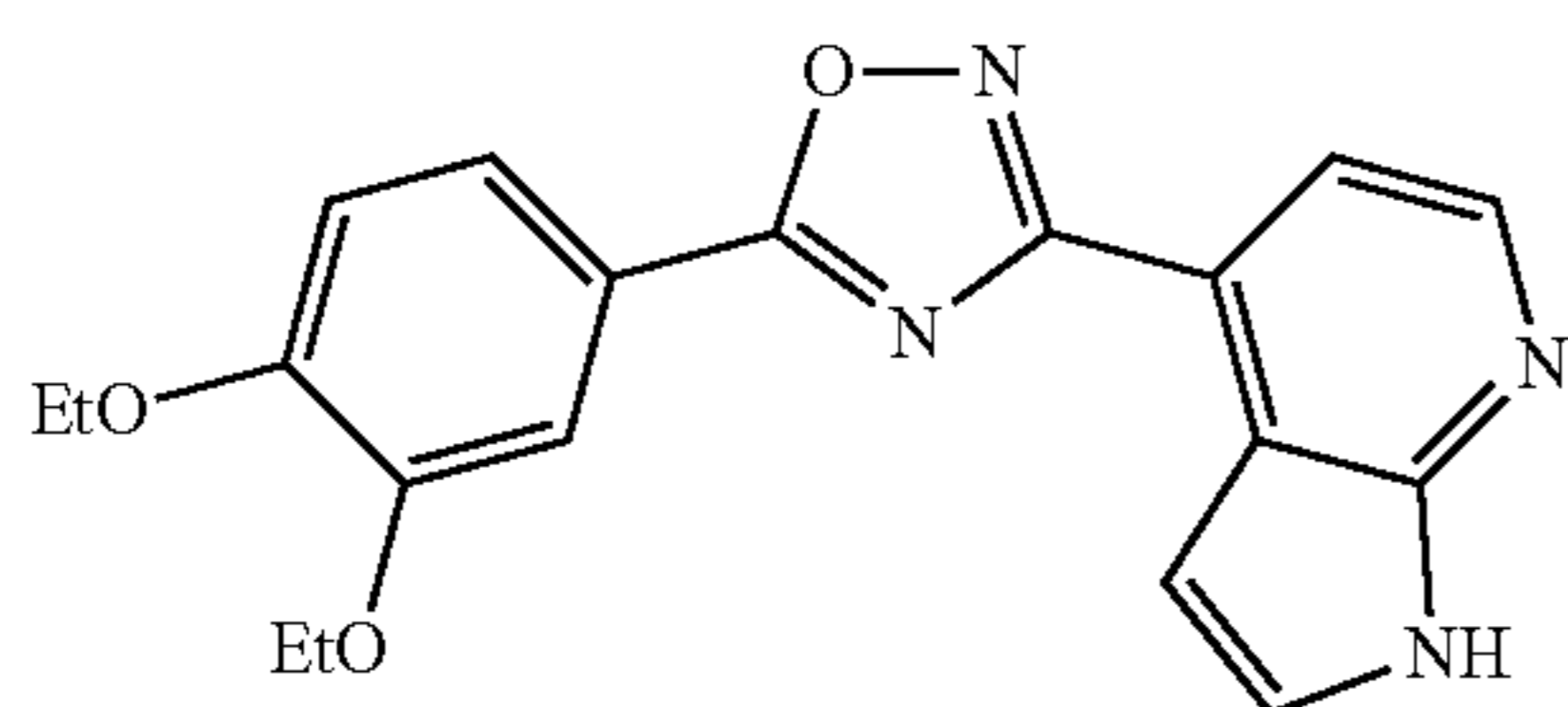
5-(3,4-diethoxyphenyl)-3-(1H-pyrrolo[2,3-b]pyridin-4-yl)-1,2,4-oxadiazole
