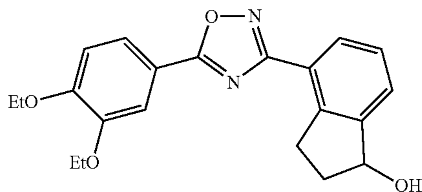
4-(5-(3,4-diethoxyphenyl)-1,2,4-oxadiazol-3-yl)-2,3-dihydro-1H-inden-1-ol
