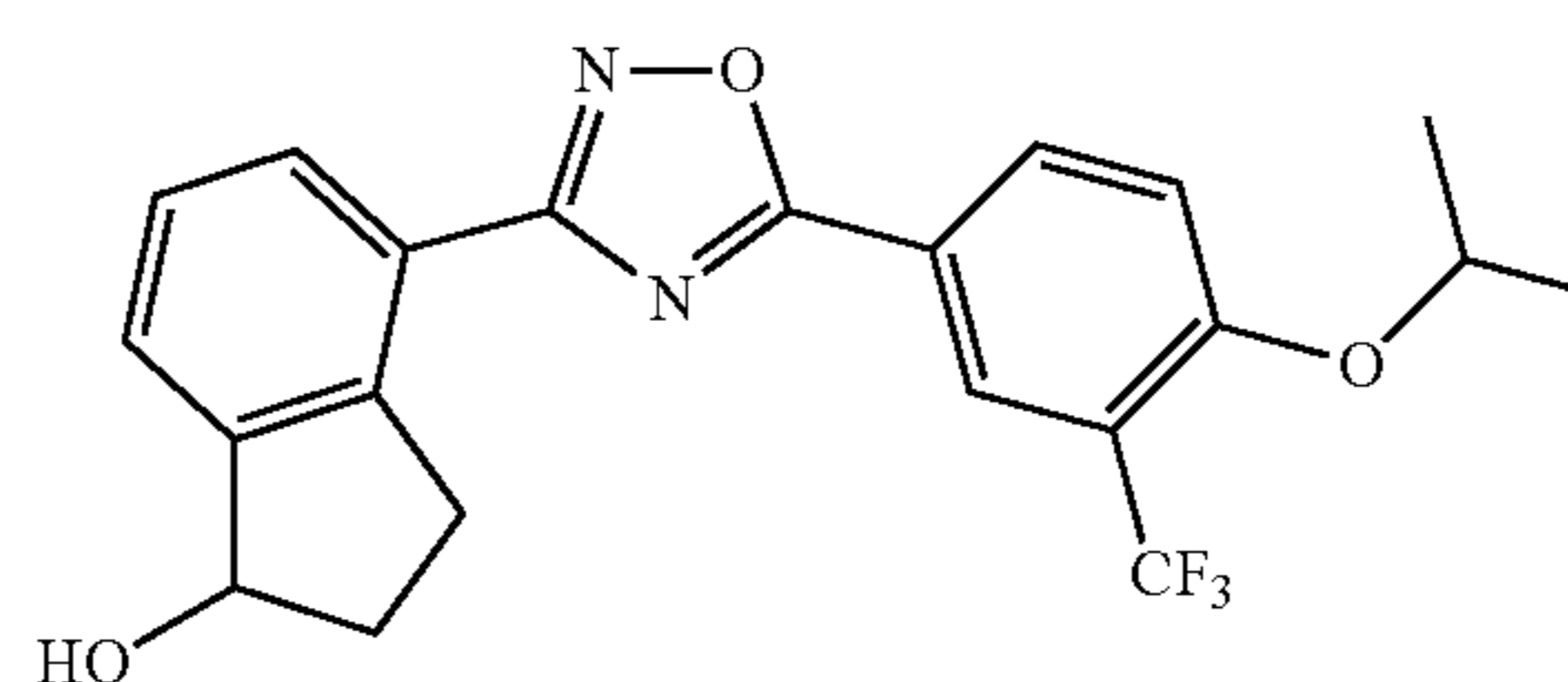
4-(5-(4-isopropoxy-3-(trifluoromethyl)phenyl)-1,2,4-oxadiazol-3-yl)-2,3-dihydro-1H-inden-1-ol
