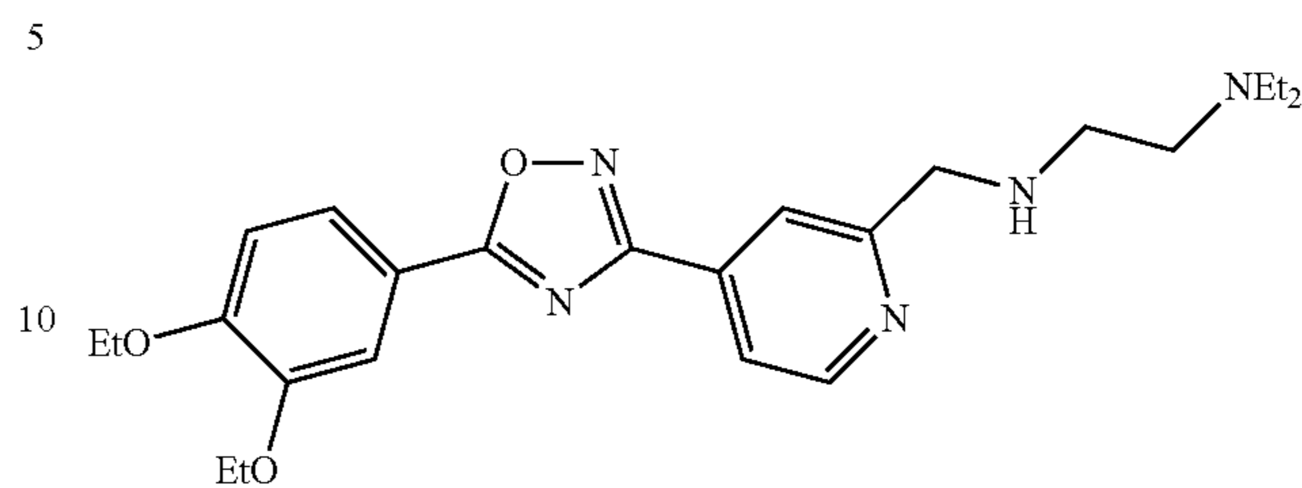
N1-((4-(5-(3,4-diethoxyphenyl)-1,2,4-oxadiazol-3-yl)pyridin-2-yl)methyl)-N2,N2-diethylethane-1,2-diamine
