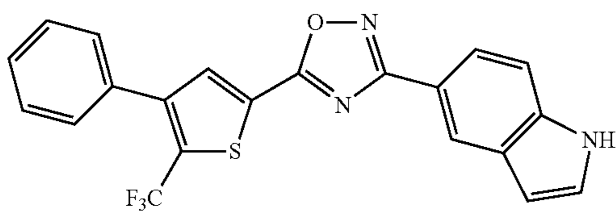
3-(1H-indol-5-yl)-5-(4-phenyl-5-(trifluoromethyl)thiophen-2-yl)-1,2,4-oxadiazole
