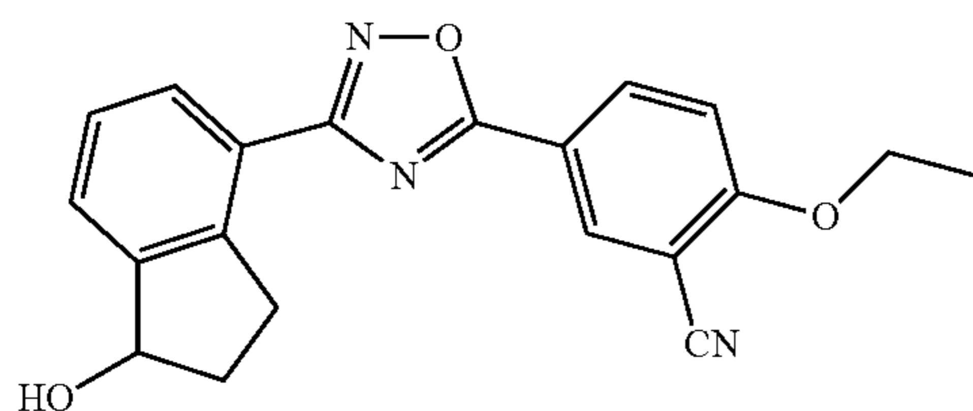
2-ethoxy-5-(3-(1-hydroxy-2,3-dihydro-1H-inden-4-yl)-1,2,4-oxadiazol-5-yl)benzonitrile
