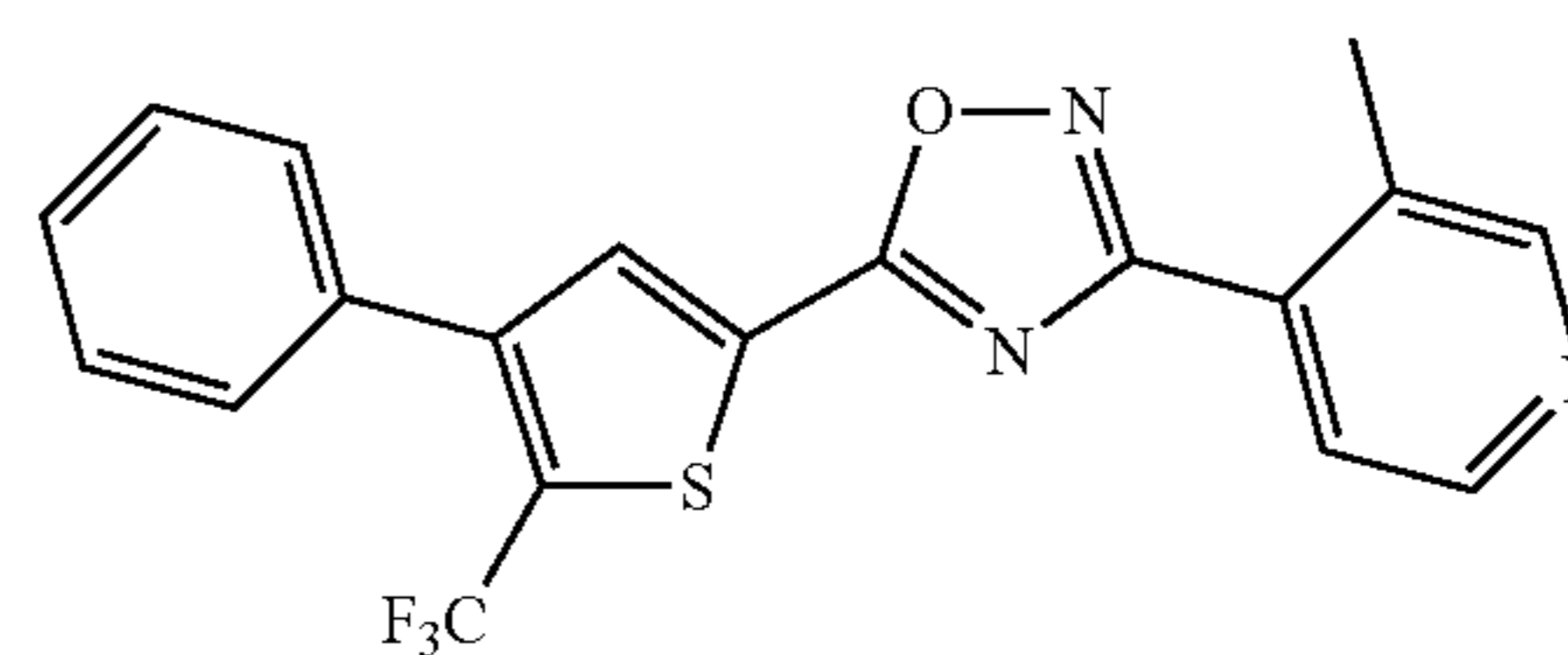
3-(3-methylpyridin-4-yl)-5-(4-phenyl-5-(trifluoromethyl)thiophen-2-yl)-1,2,4-oxadiazole
