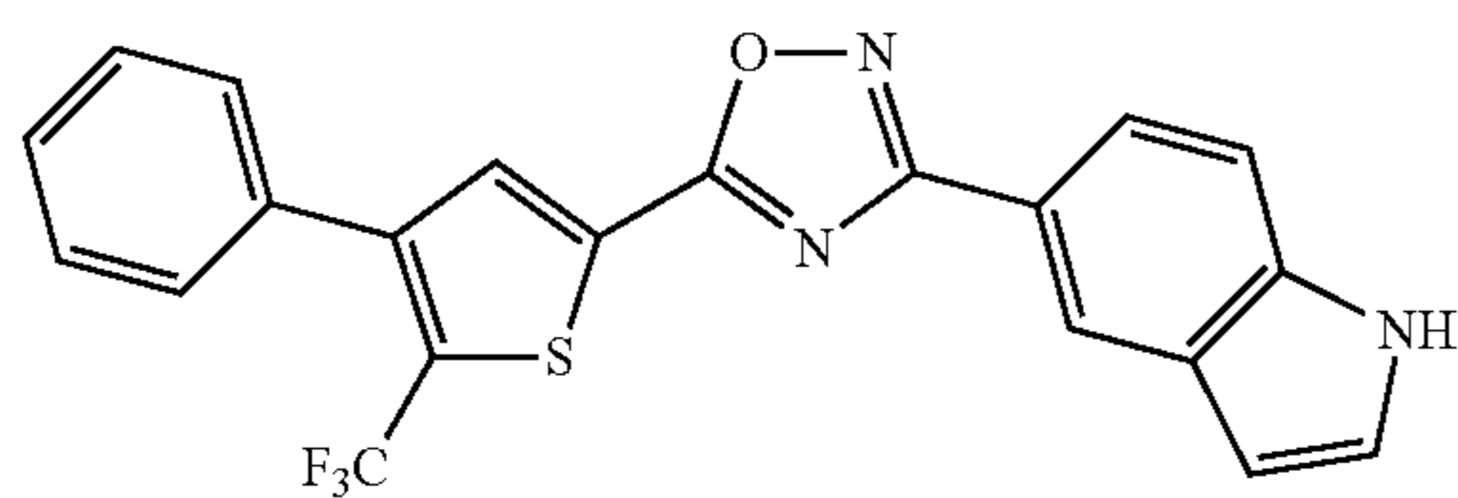
3-(1H-indol-5-yl)-5-(4-phenyl-5-(trifluoromethyl)thiophen-2-yl)-1,2,4-oxadiazole
