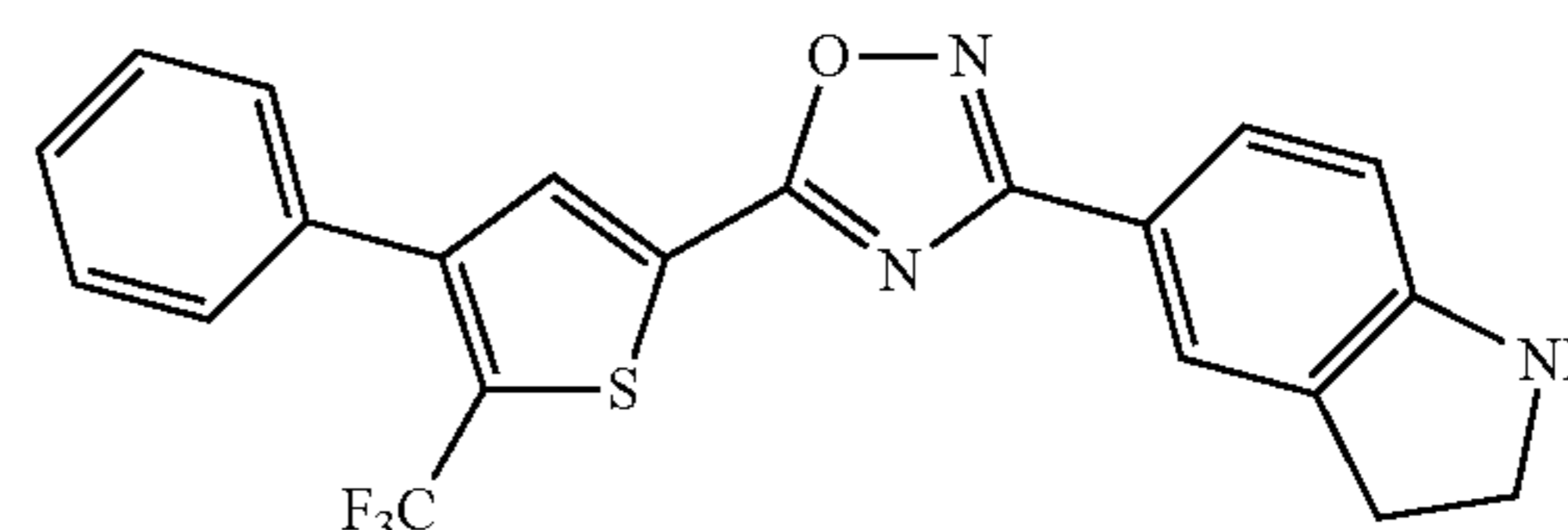
3-(indolin-5-yl)-5-(4-phenyl-5-(trifluoromethyl)thiophen-2-yl)-1,2,4-oxadiazole
