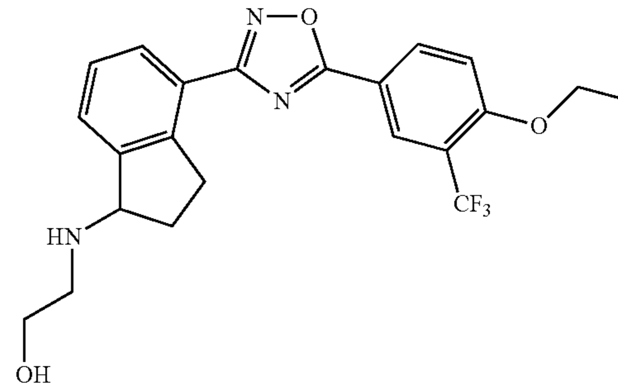
2-(4-(5-(4-ethoxy-3-(trifluoromethyl)phenyl)-1,2,4-oxadiazol-3-yl)-2,3-dihydro-1H-inden-1-ylamino)ethanol
