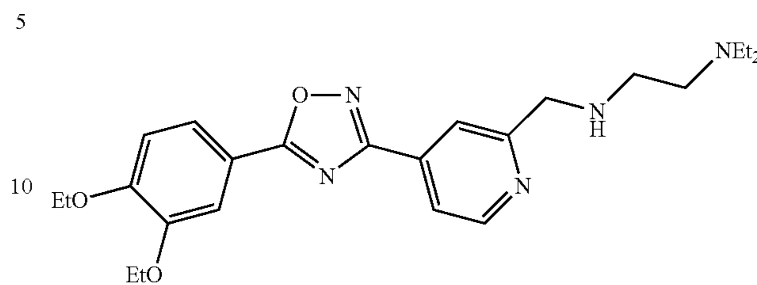
N1-((4-(5-(3,4-diethoxyphenyl)-1,2,4-oxadiazol-3-yl)pyridin-2-yl)methyl)-N2,N2-diethylethane-1,2-diamine
