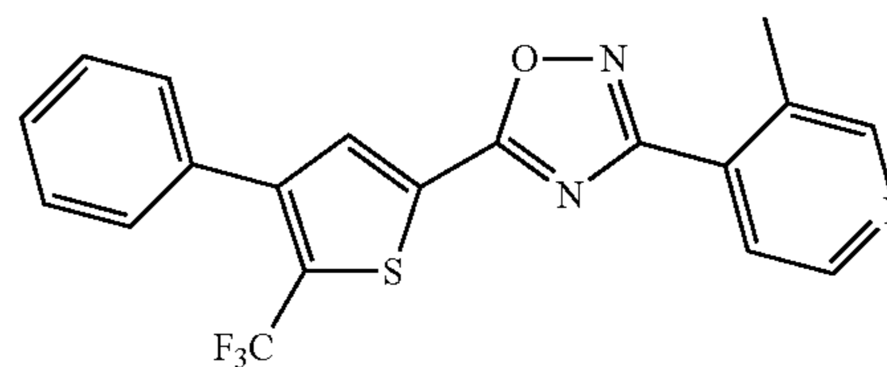
3-(3-methylpyridin-4-yl)-5-(4-phenyl-5-(trifluoromethyl)thiophen-2-yl)-1,2,4-oxadiazole
