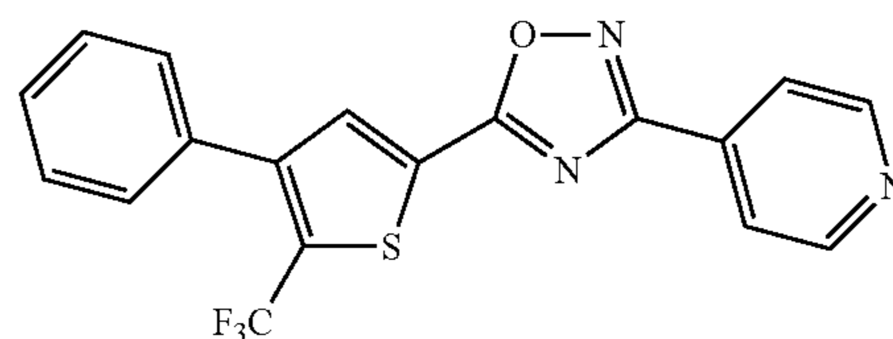
4-[5-(4-Phenyl-5-trifluoromethyl-thiophen-2-yl)-[1,2,4]oxadiazol-3-yl]pyridine
