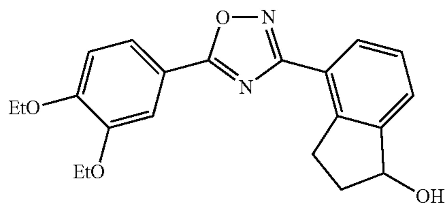
4-(5-(3,4-diethoxyphenyl)-1,2,4-oxadiazol-3-yl)-2,3-dihydro-1H-inden-1-ol
