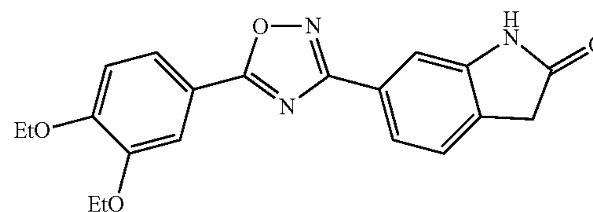
6-(5-(3,4-diethoxyphenyl)-1,2,4-oxadiazol-3-yl)indolin-2-one
