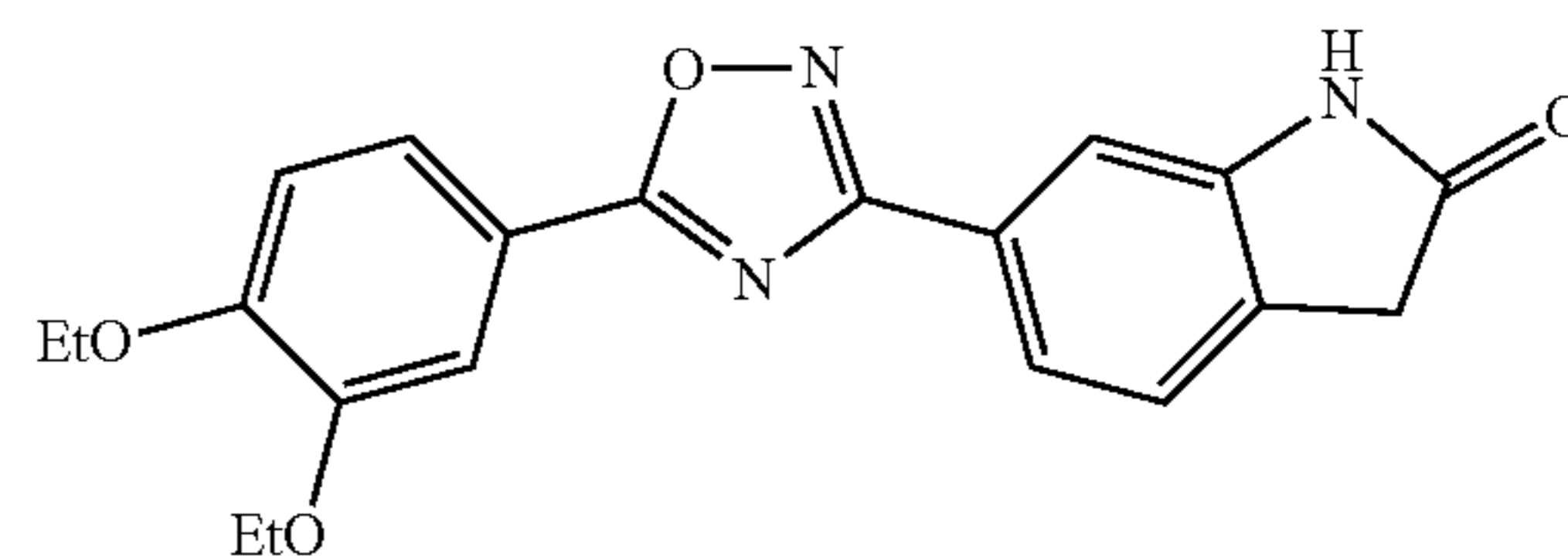
6-(5-(3,4-diethoxyphenyl)-1,2,4-oxadiazol-3-yl)indolin-2-one
