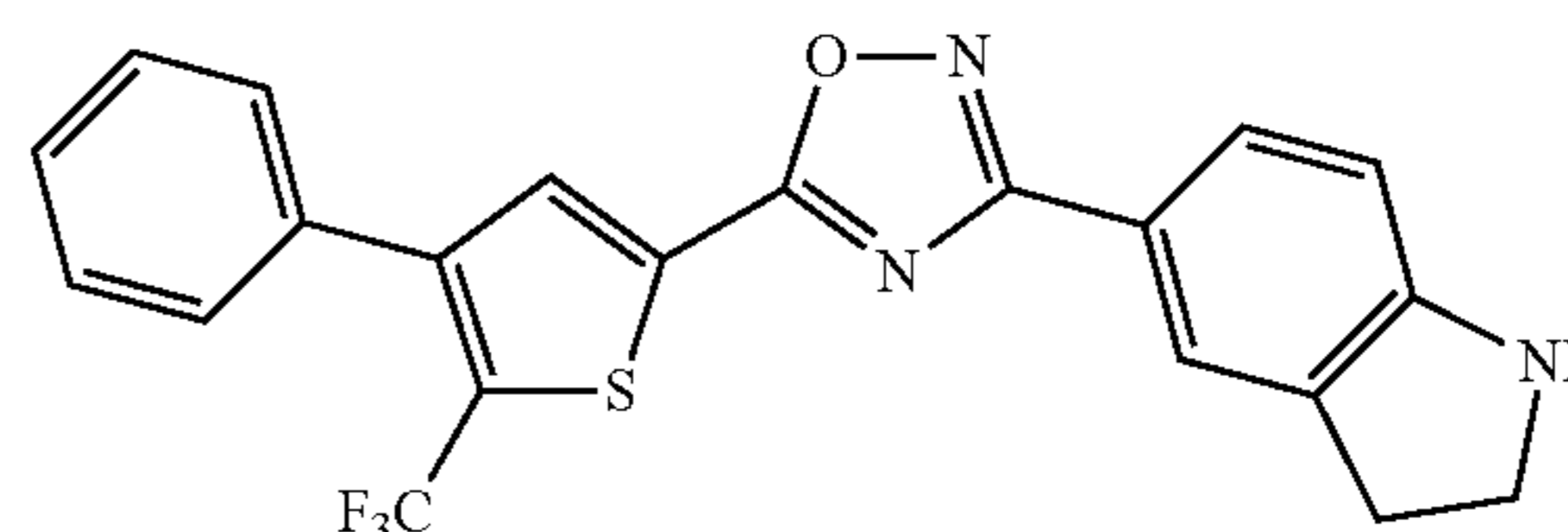
3-(indolin-5-yl)-5-(4-phenyl-5-(trifluoromethyl)thiophen-2-yl)-1,2,4-oxadiazole
