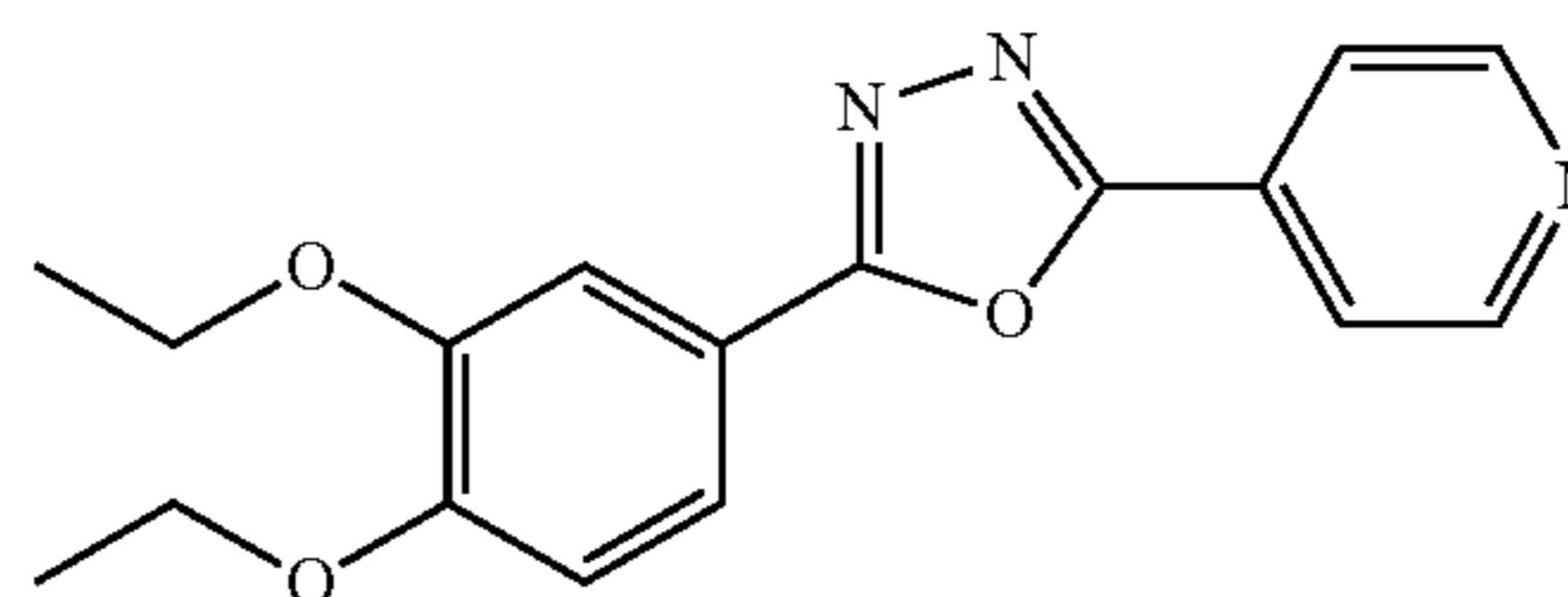
2-(3,4-diethoxyphenyl)-5-(pyridin-4-yl)-1,3,4-oxadiazole (25)
