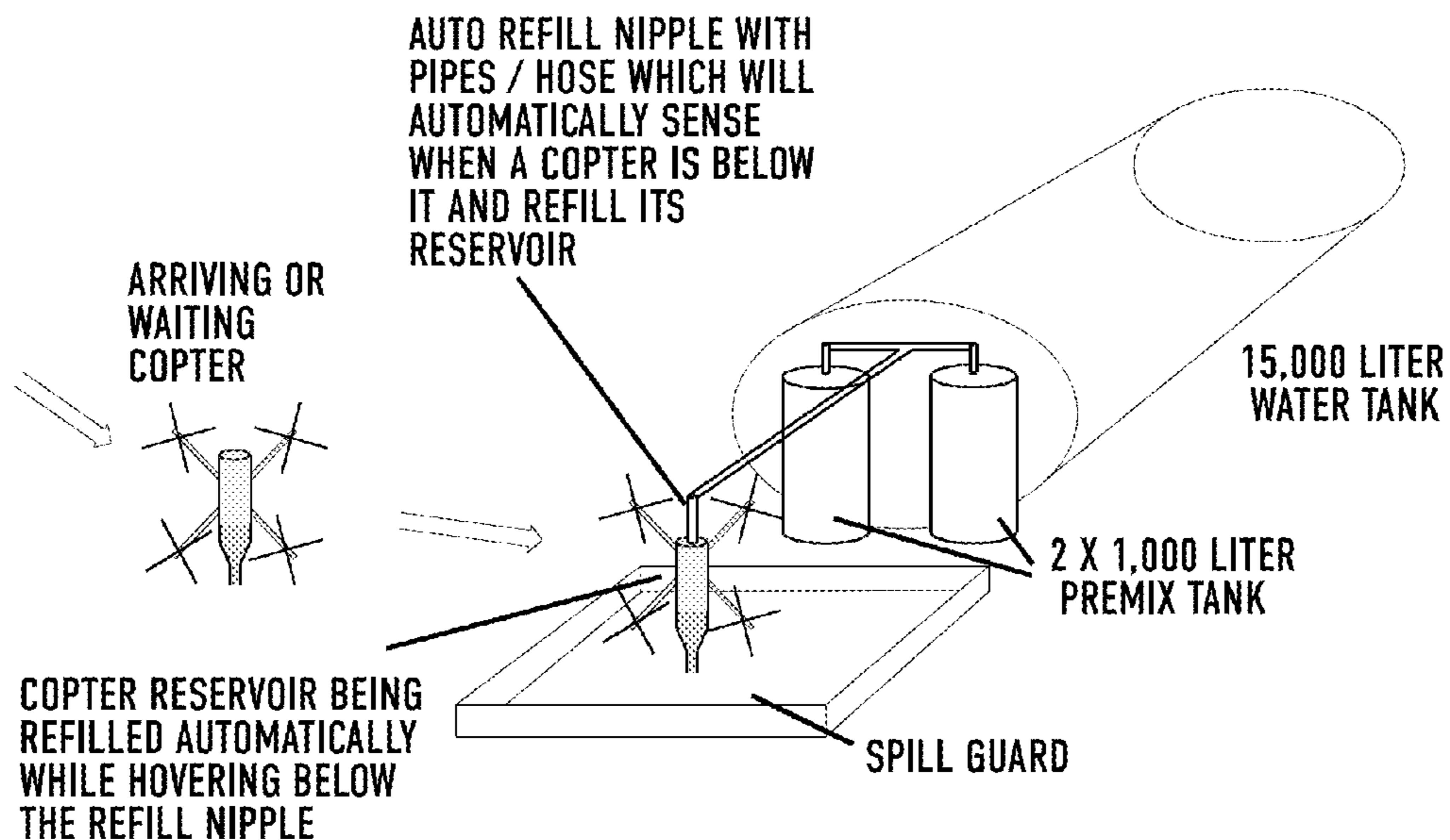
FIGURE 20 REFILLING RESERVOIR FOR CROP DUSTING
