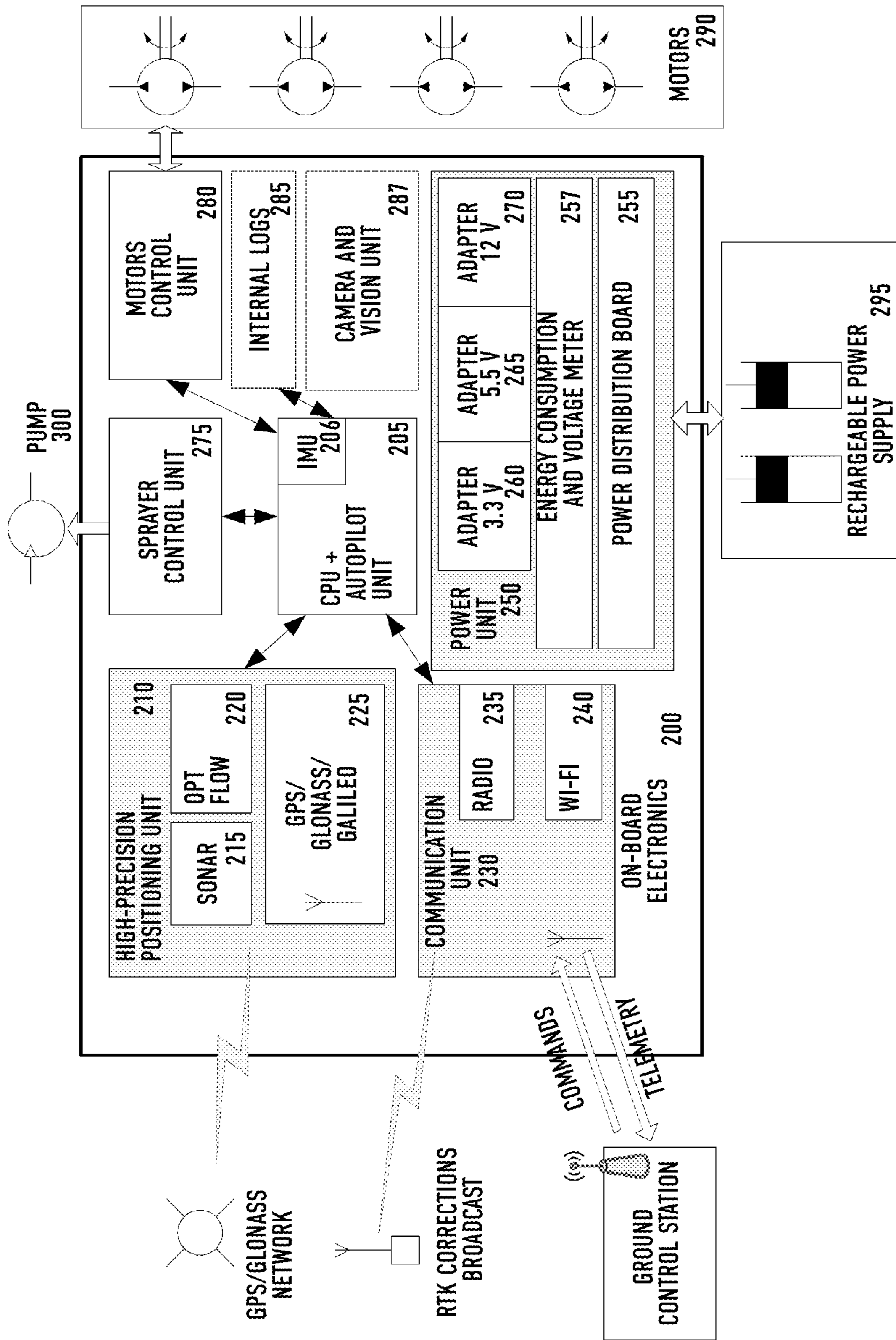
FIGURE 10 ONBOARD ELECTRONICS FOR AERIAL FARM ROBOT
