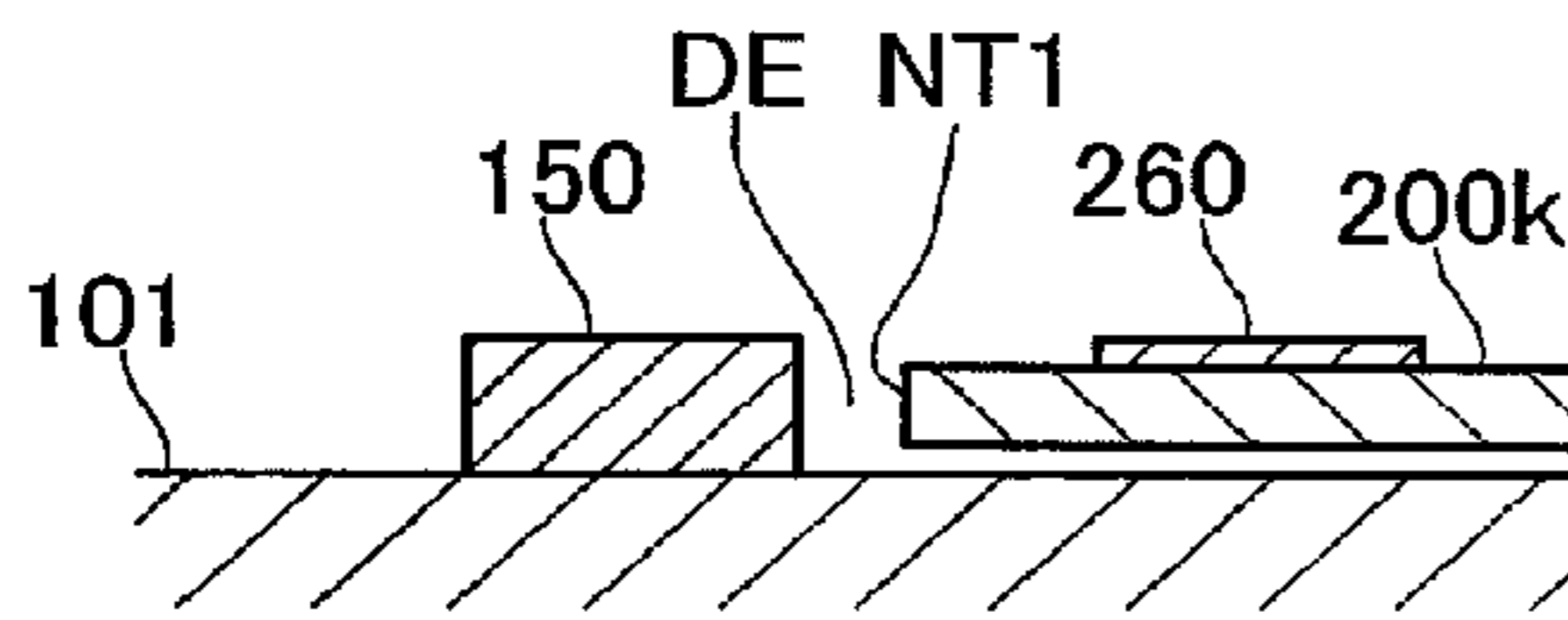
A-A CROSS SECTION
