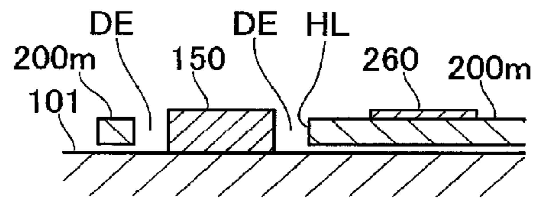
B-B CROSS SECTION
