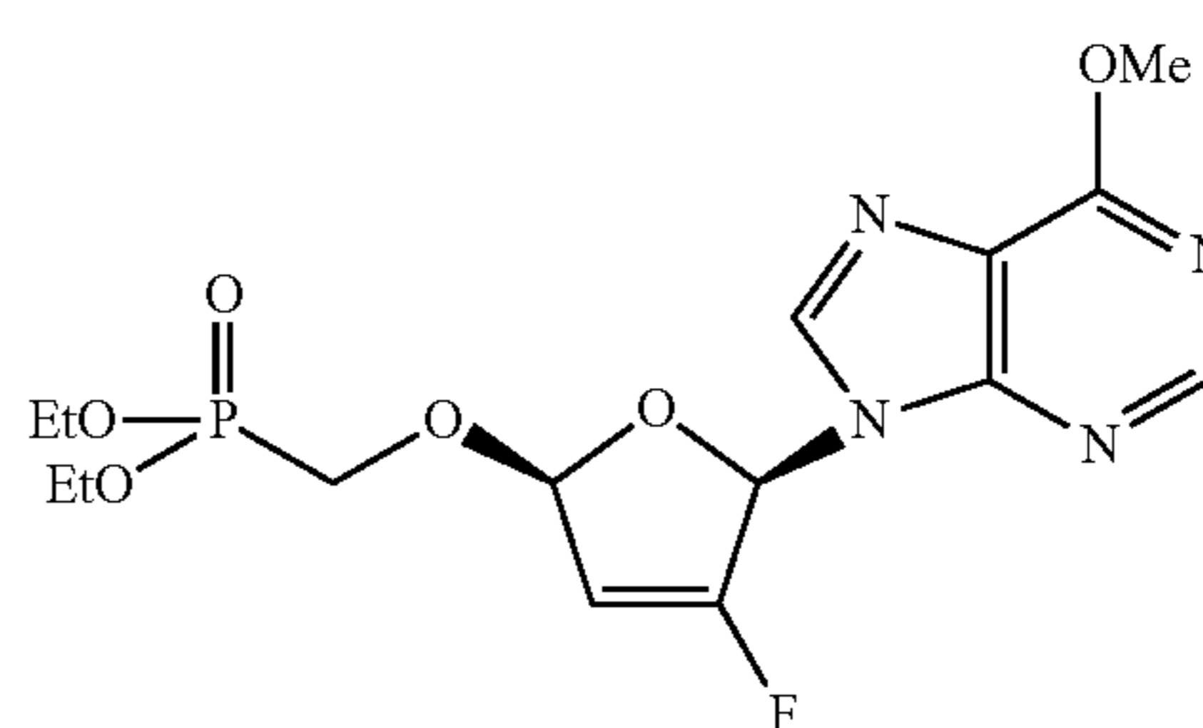
(2'R,5'R)-6-Methoxy-9-[3-fluoro-2,5-dihydro-5-(diethoxyphosphinyl)methoxy-2-furanyl]purine (7)
