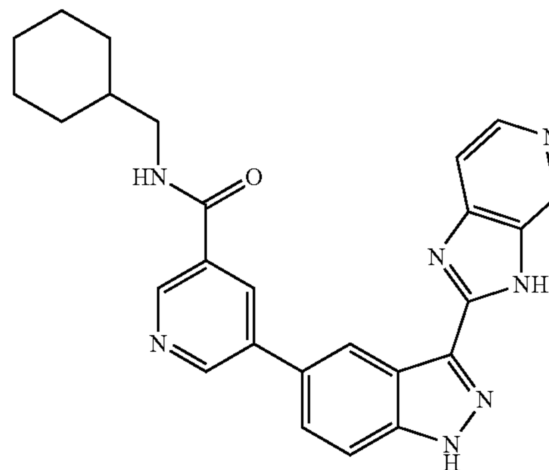
5-(3-(3H-imidazo[4,5-c]pyridin-2-yl)-1H-indazol-5-yl)-N-(cyclohexyl methyl)nicotinamide 2
