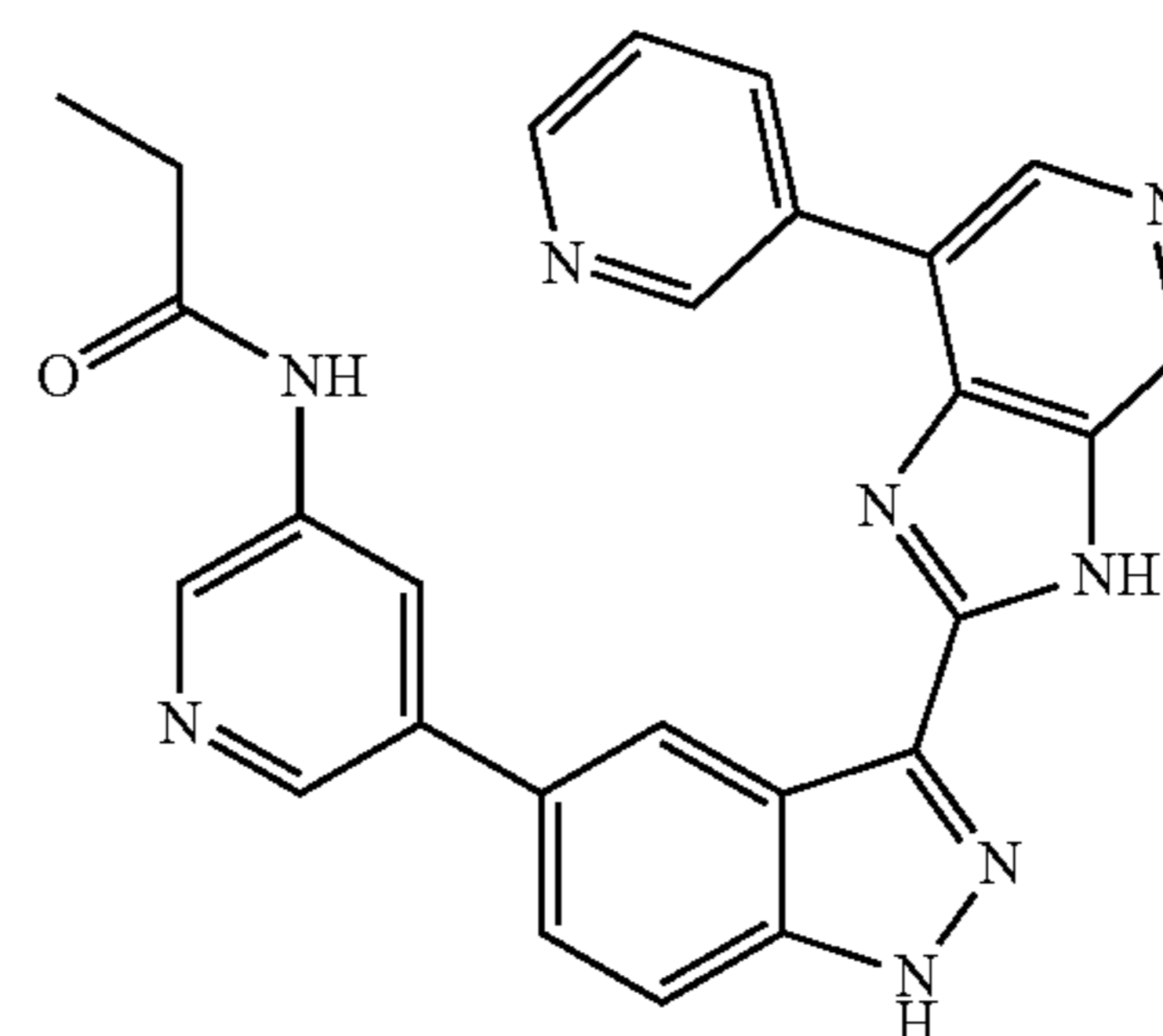
N-(5-(3-(7-(pyridin-3-yl)-3H-imidazo[4,5-c]pyridin-2-yl)-1H-indazol-5-yl)pyridin-3-yl)propionamide 4
