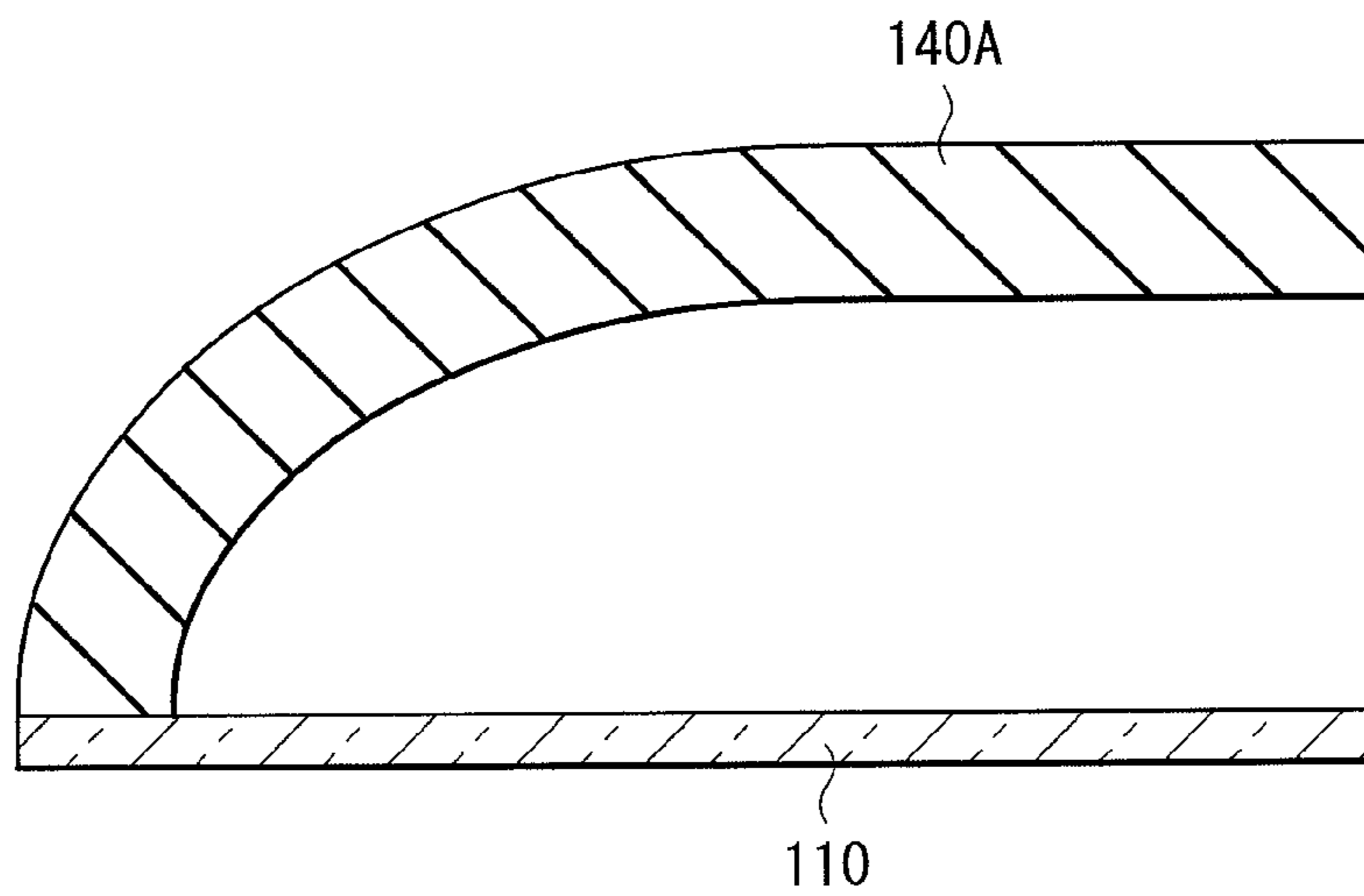
FIG. 4 RELATED ART
