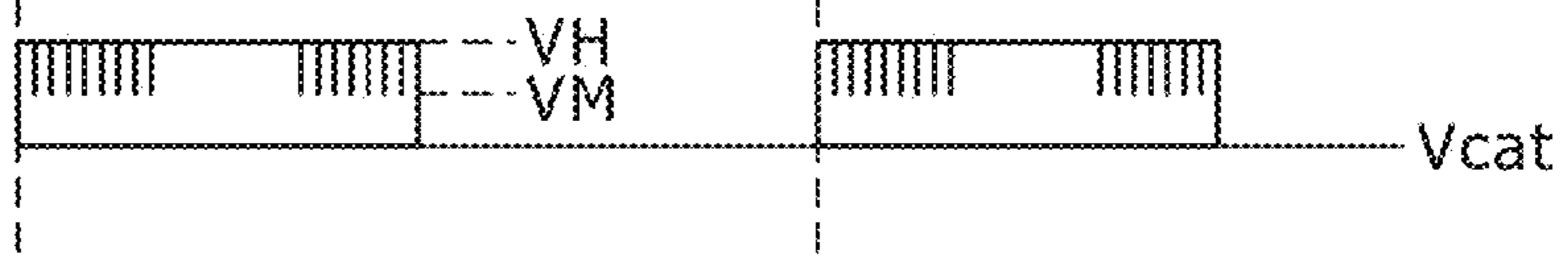
FIG. 39B DUTY45% MOVING IMAGE IMPROVEMENT SYSTEM
