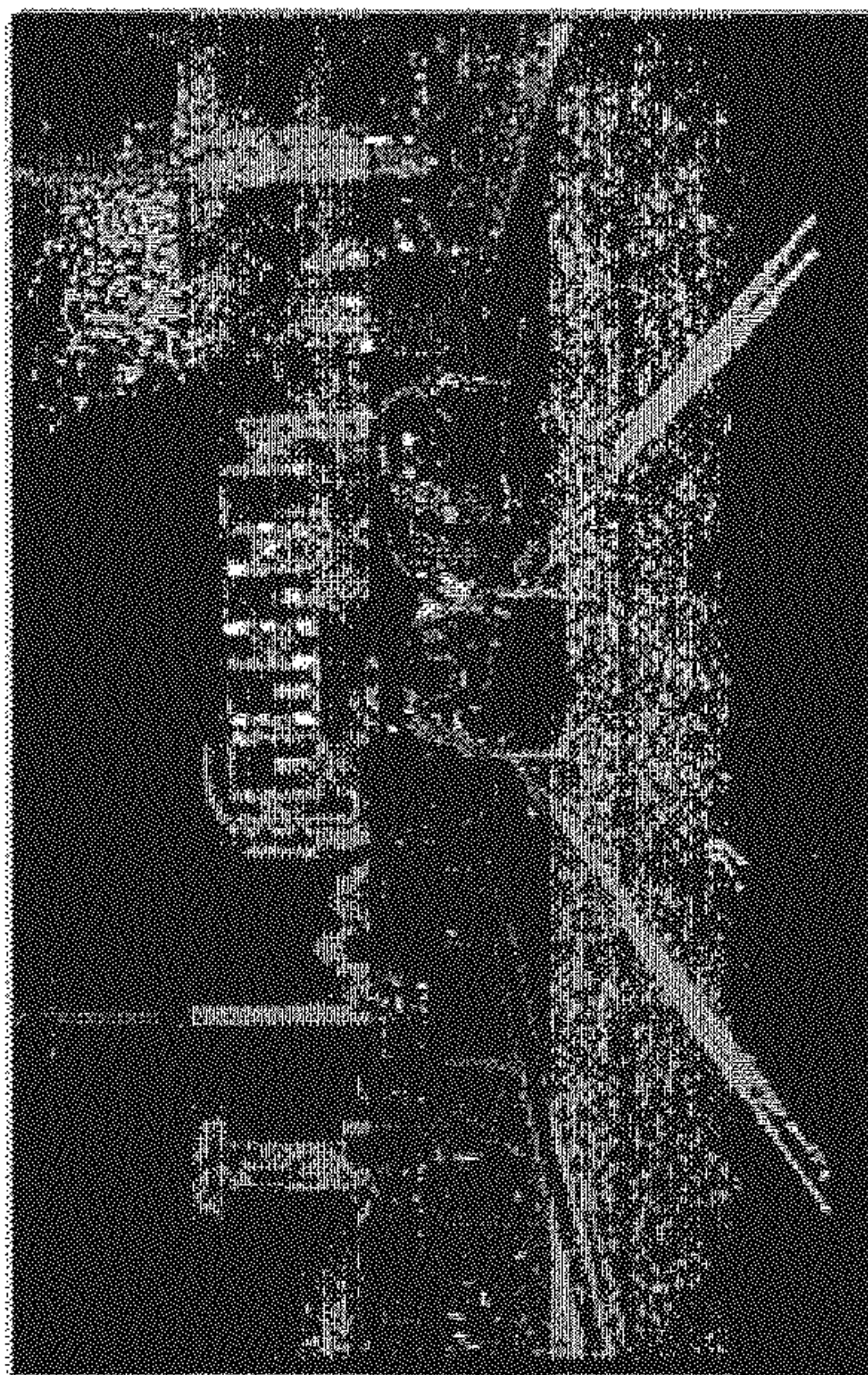
DISPARITY MAP
