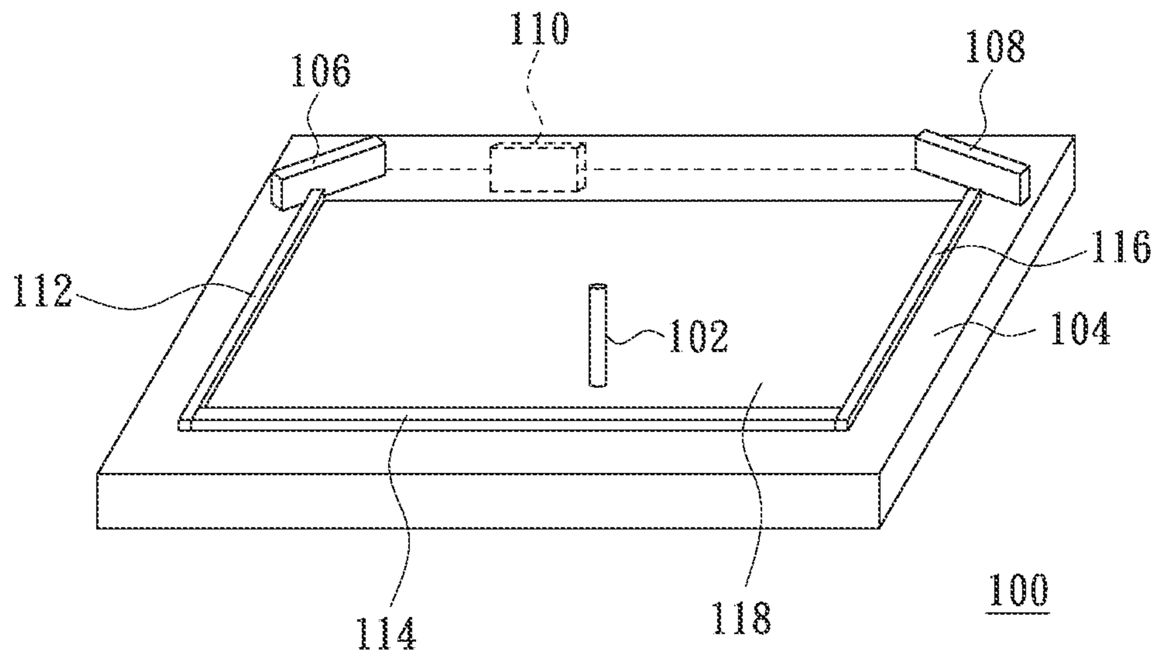
FIG. 1 (Prior Art)
