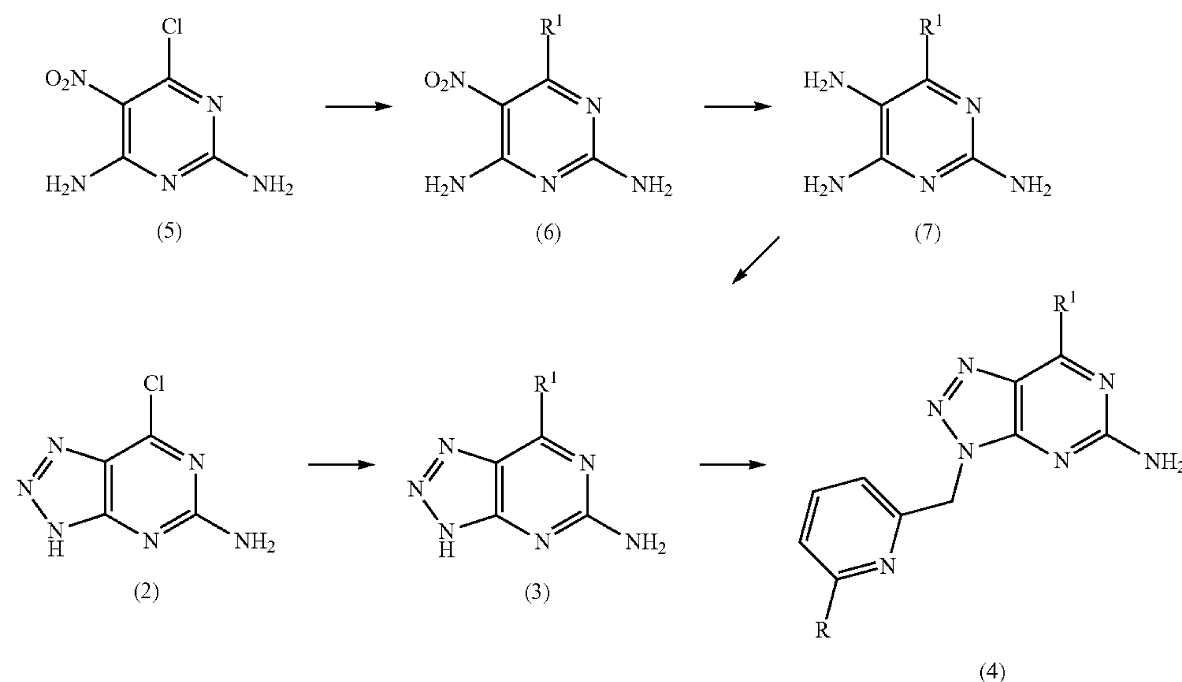
Reaction Scheme 1
