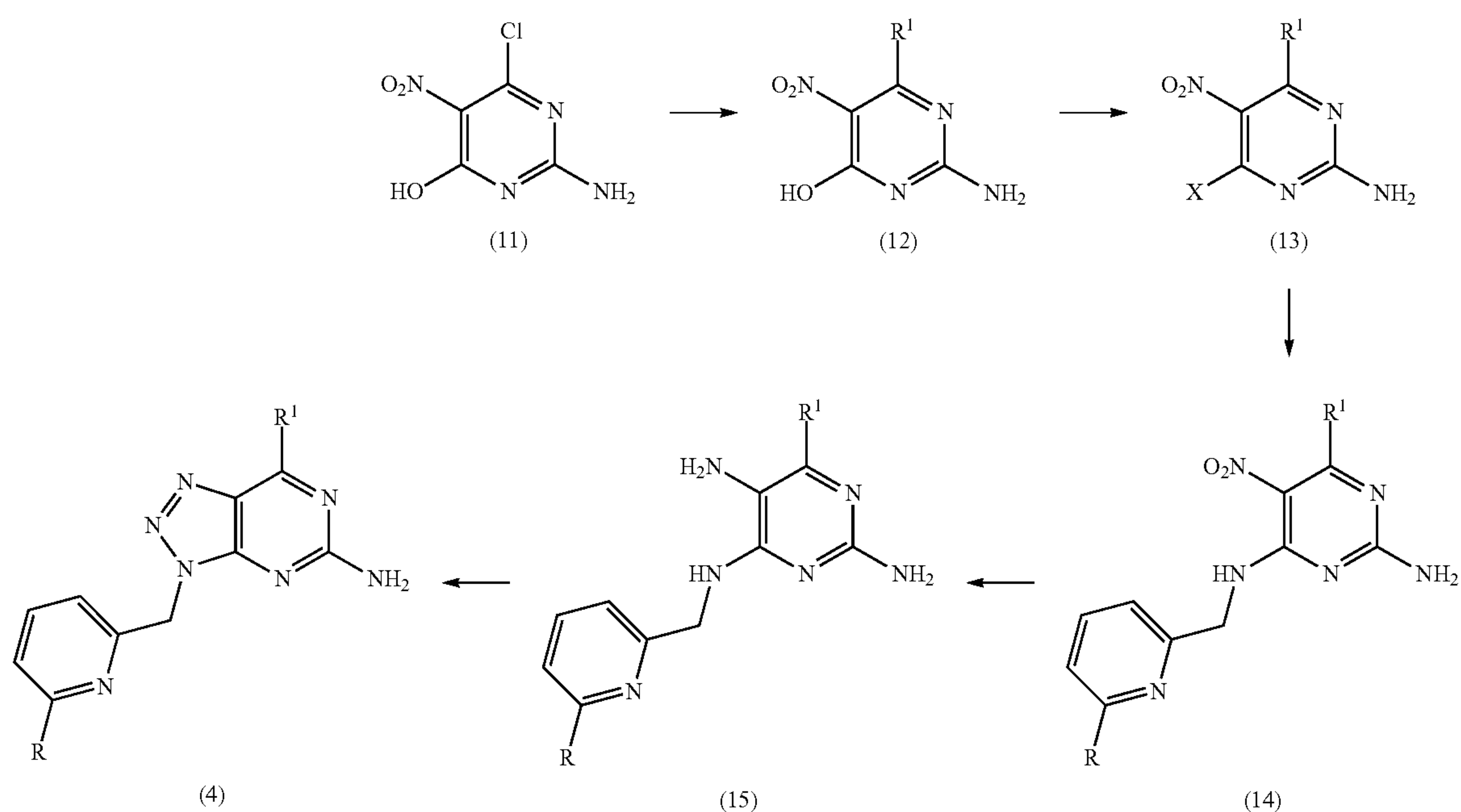
Reaction Scheme 3
