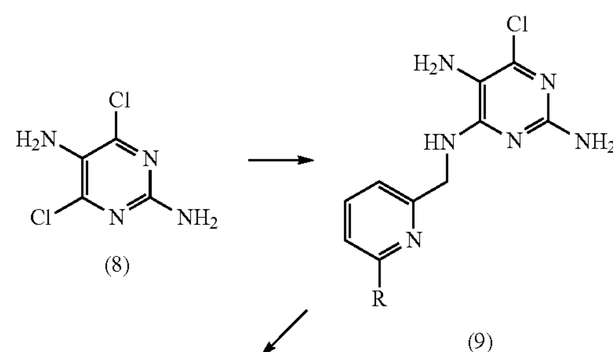
Reaction Scheme 2
