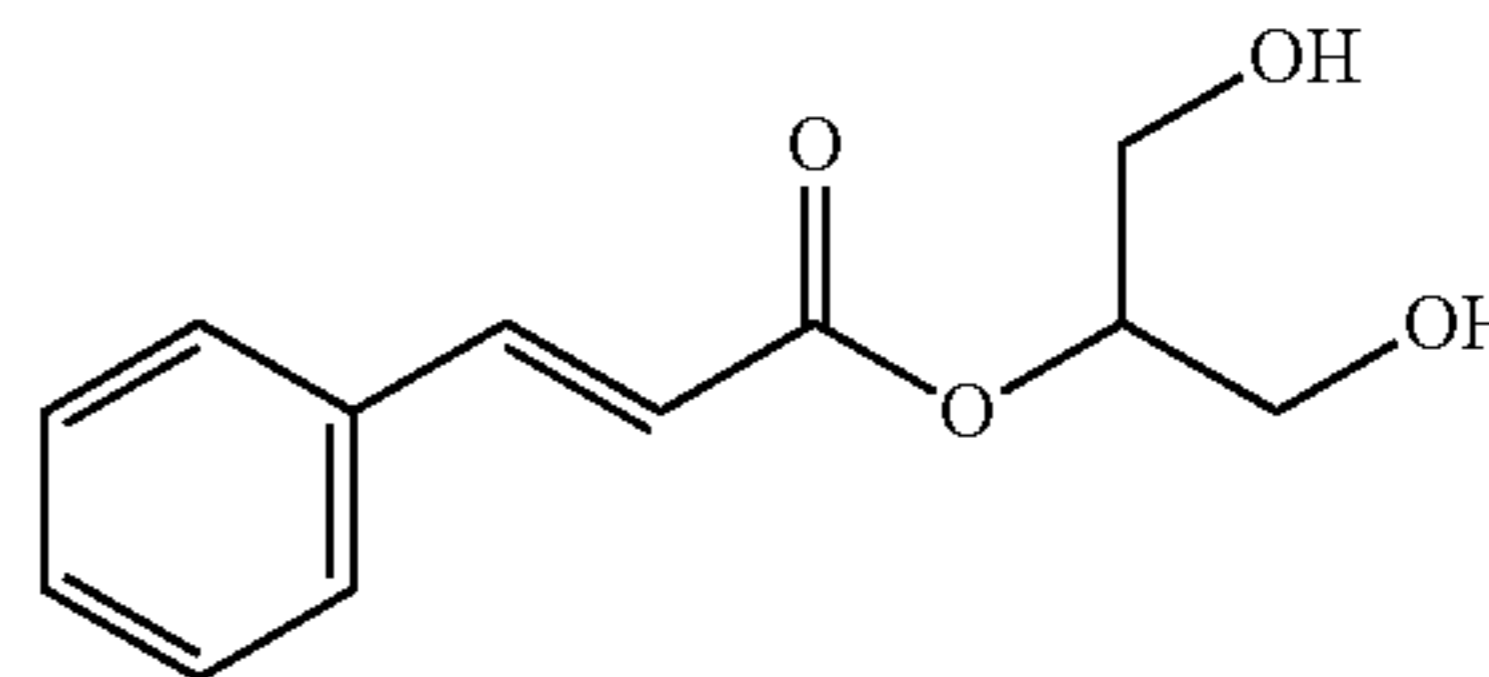
Glyceryl Mono-Cinnamate
