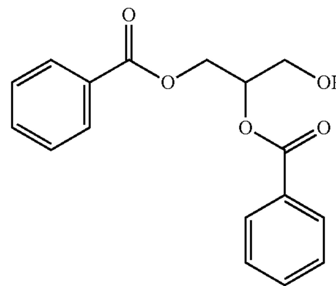
Glyceryl Di-Benzoate
