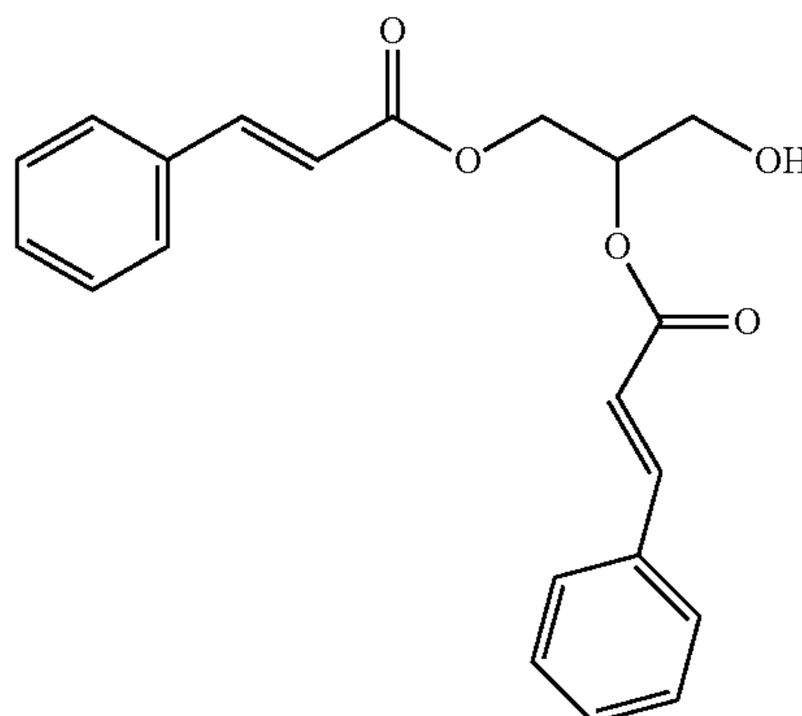
Glyceryl Di-Cinnamate
