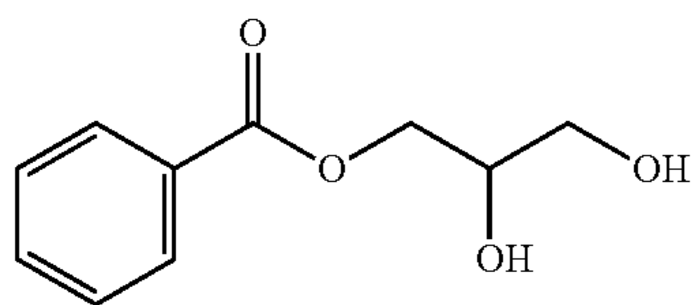
Glyceryl Mono-Benzoate
