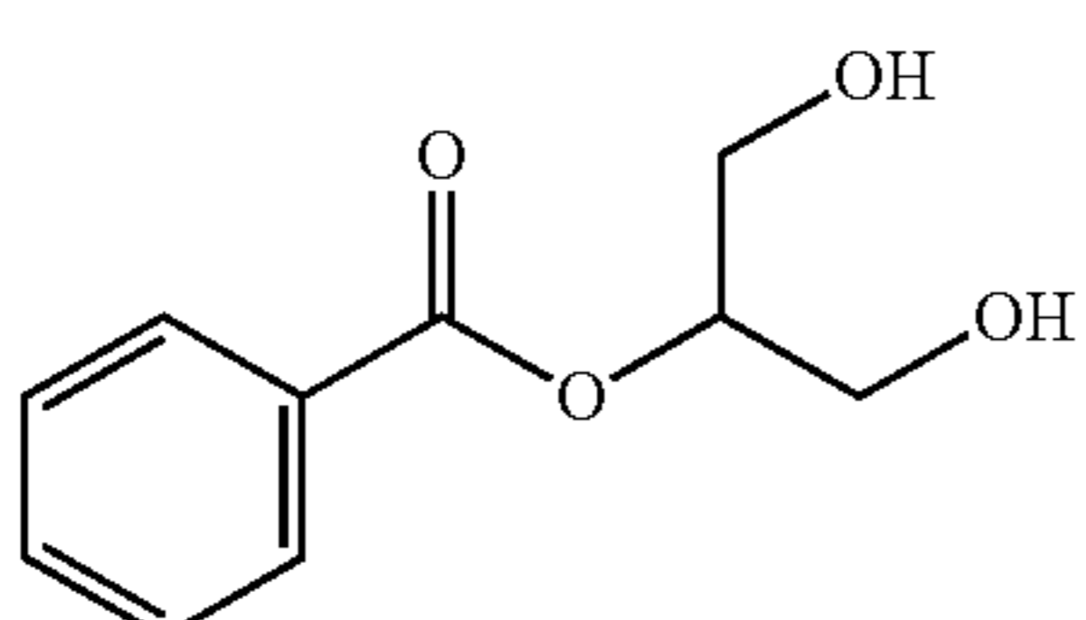
Glyceryl Mono-Benzoate
