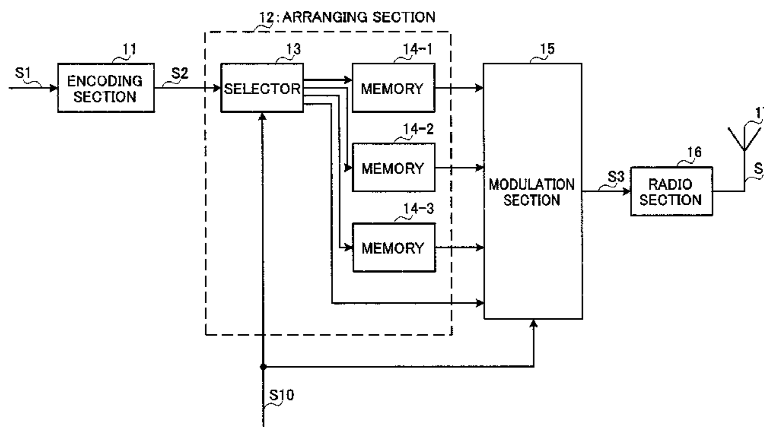
10 TRANSMITTING APPARATUS
