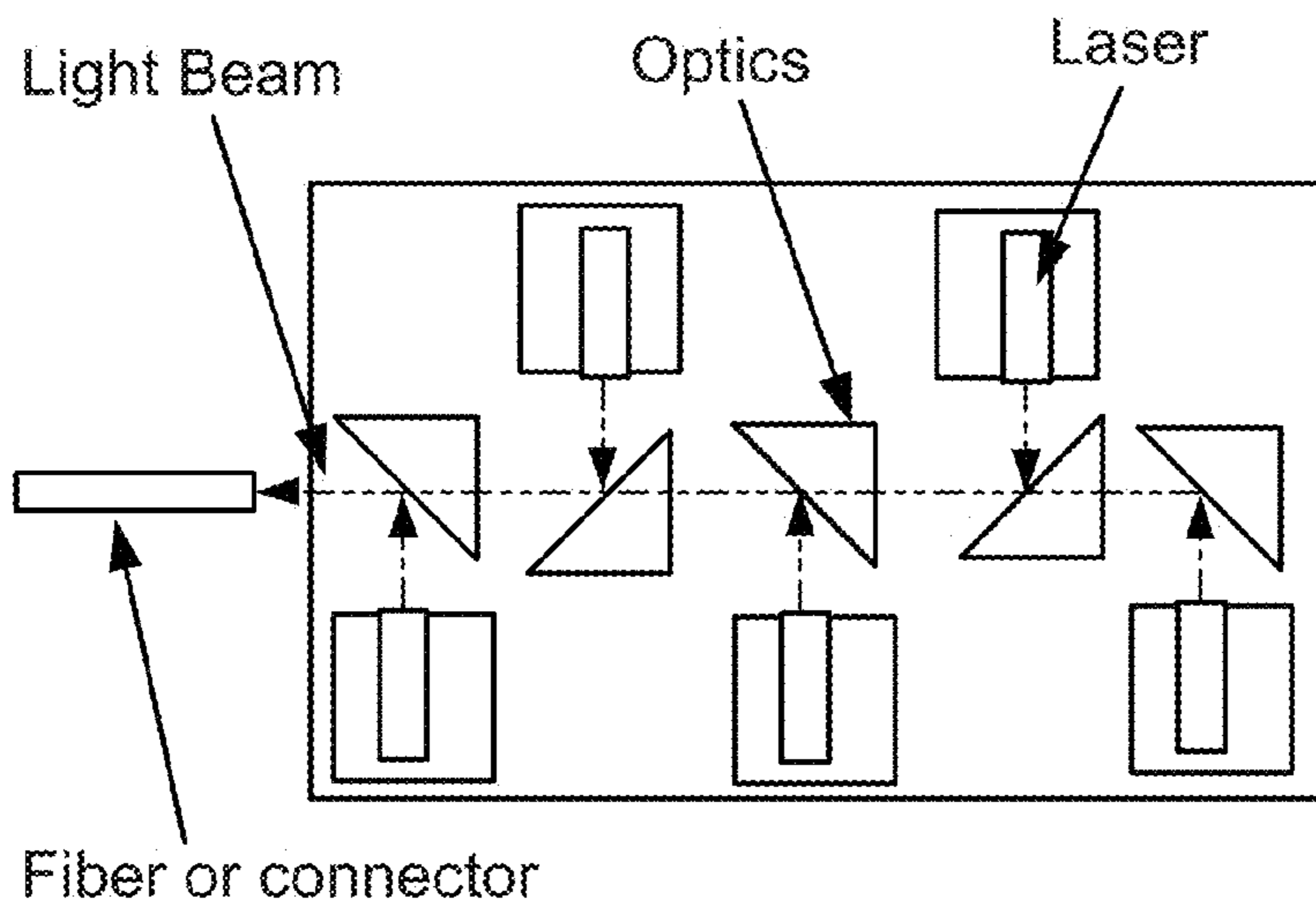
2 row configuration
