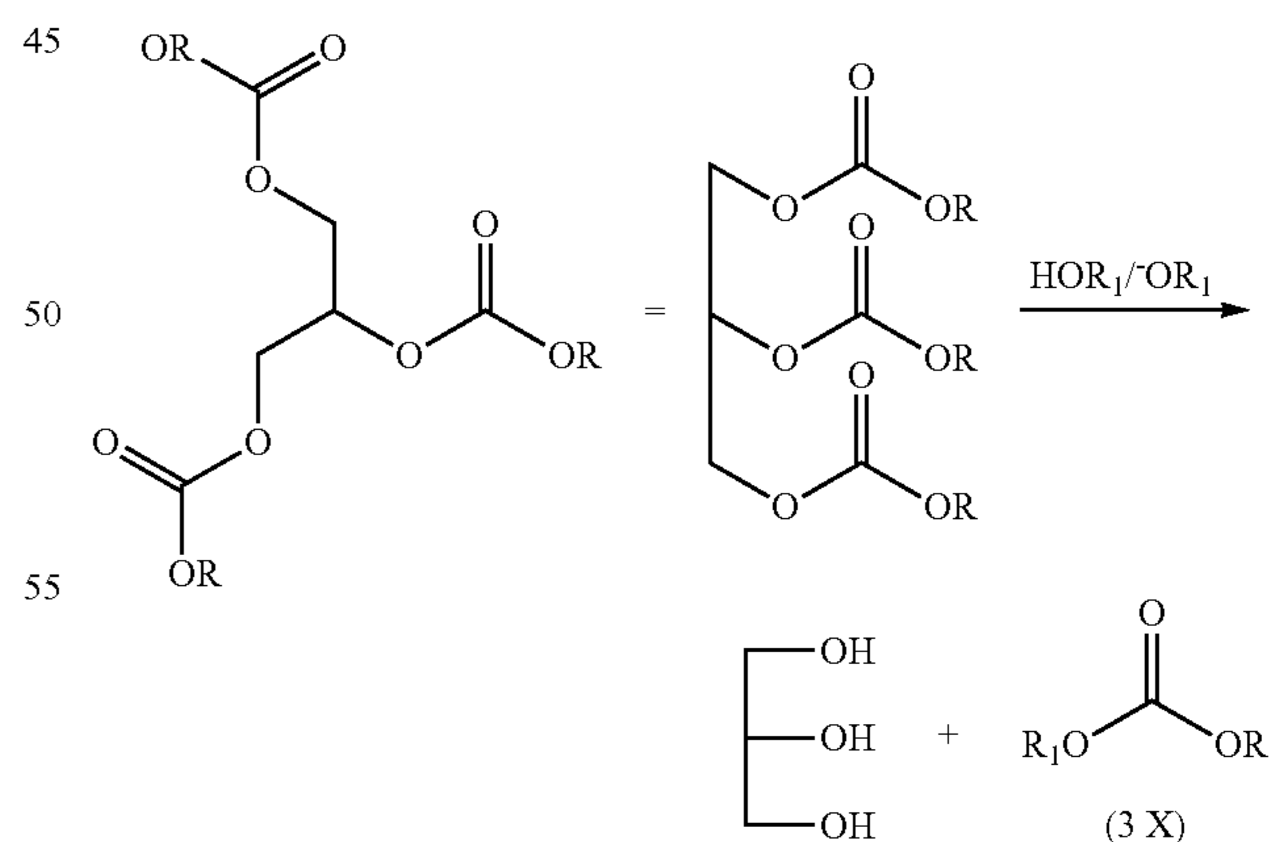
Scheme 1. Illustrative transesterification of tryglycerides with methanol (HOR 1 ) with catalytic OH - to make biodiesel.
