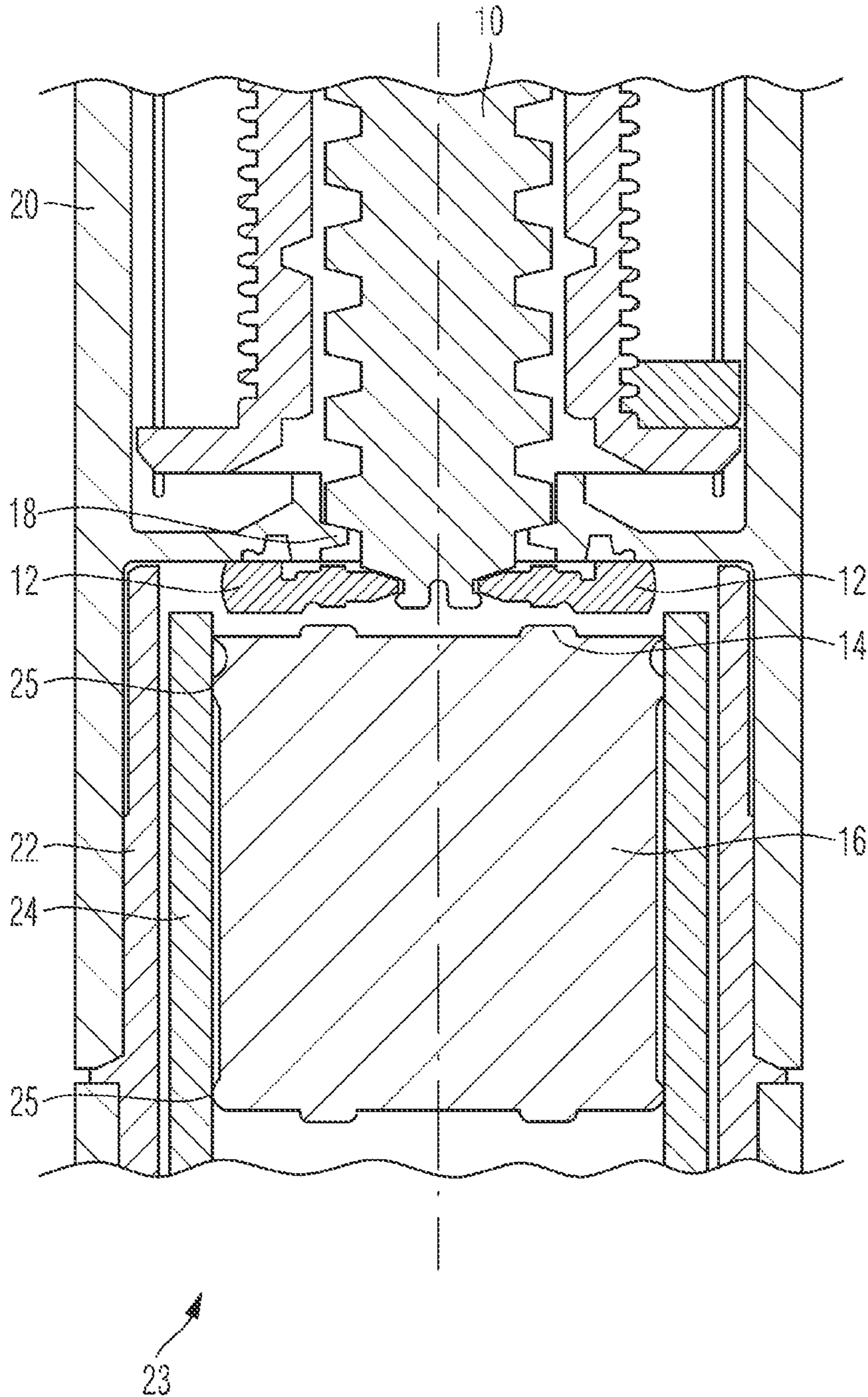
Fig. 1 prior art
