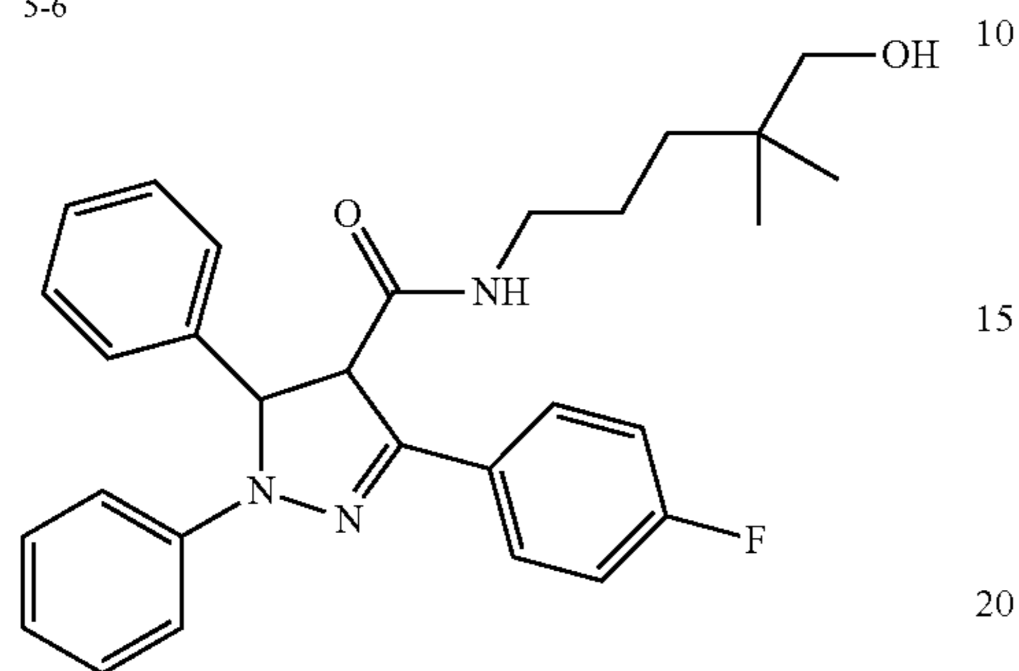
Compound 5
