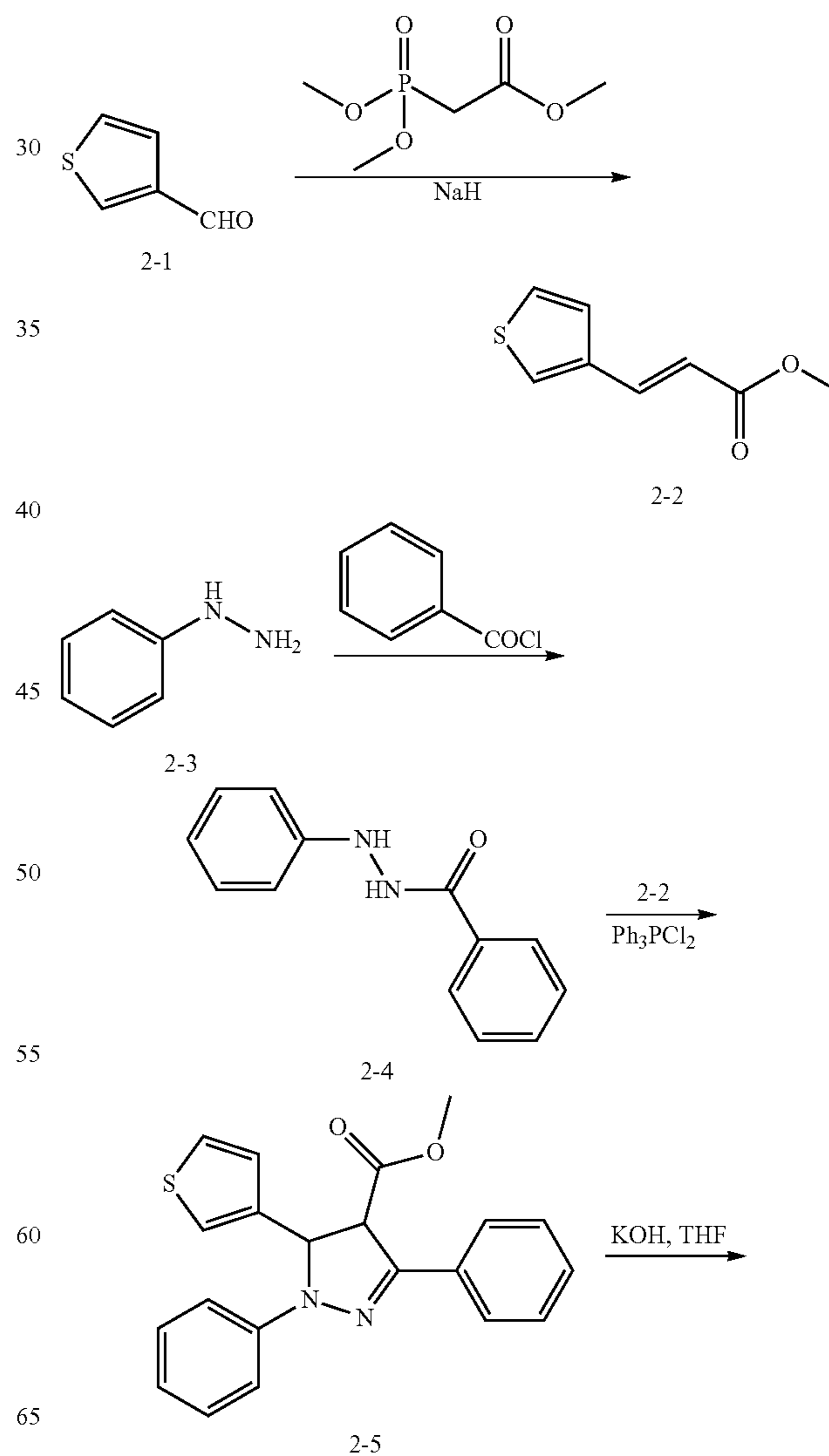
Synthesis Scheme 2
