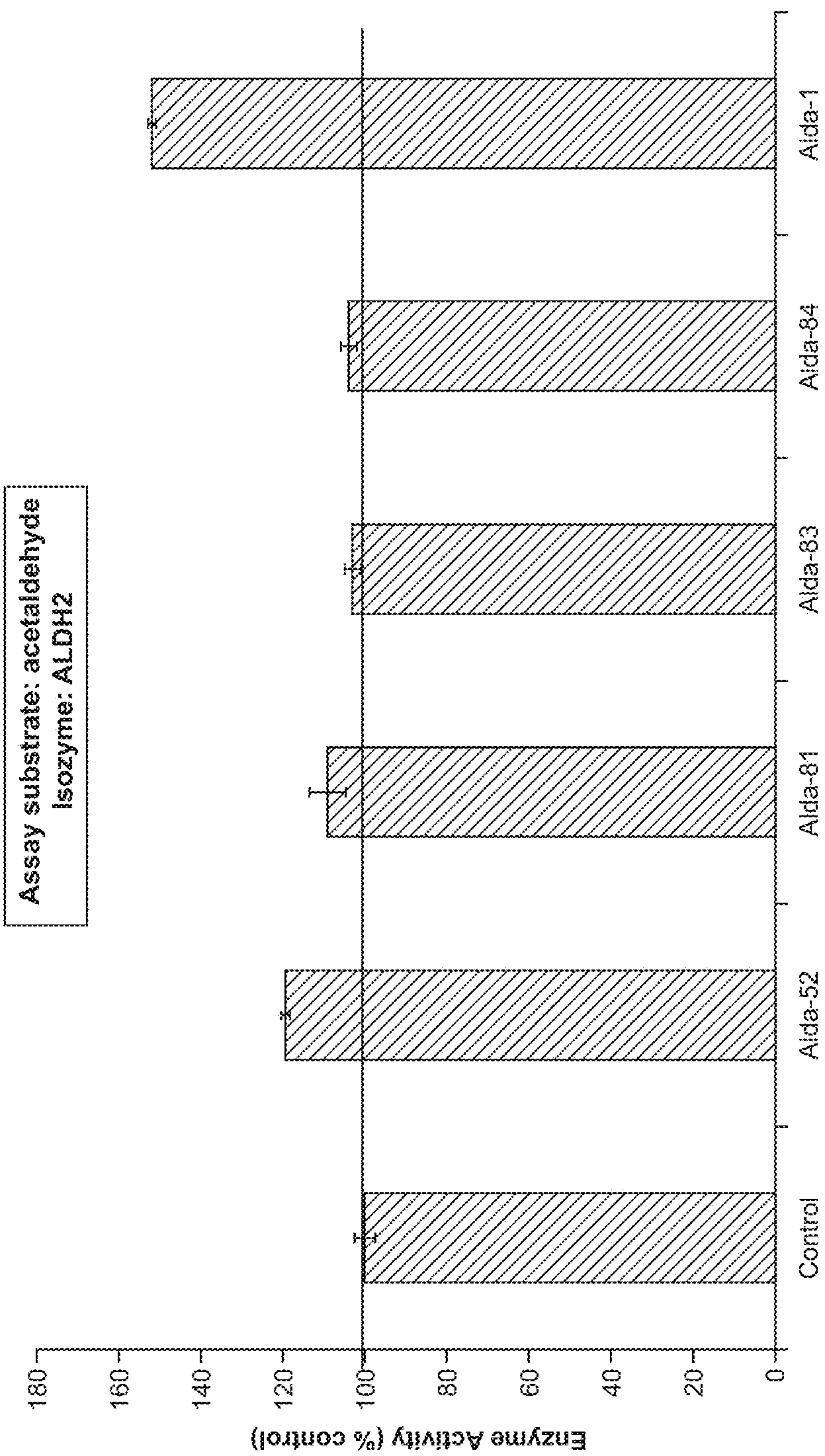
Aida-52, Aida-81, Aida-1 activate ALDH2 using acetaldehyde as a substrate
