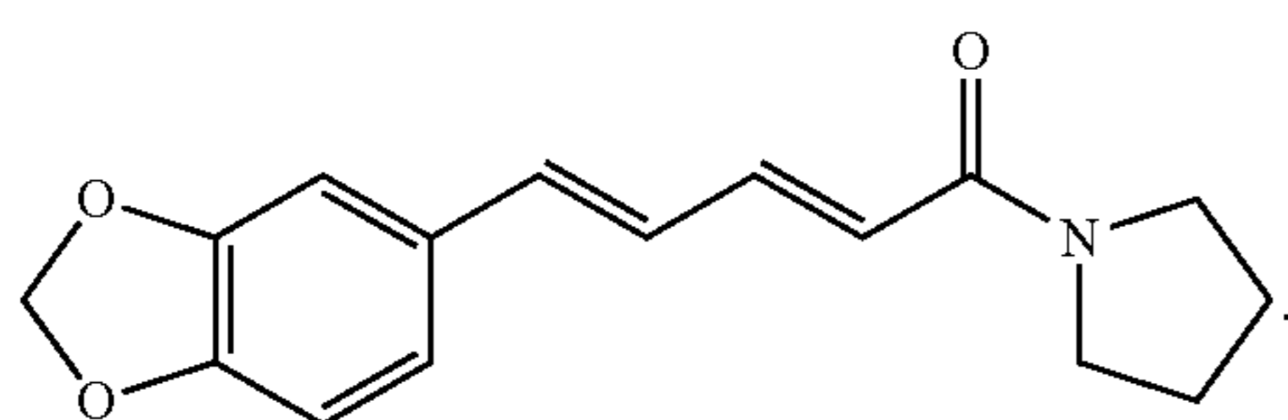
C_{16}H_{17}NO_3 Exact Mass: 271.12 Mol. Wt.: 271.31
