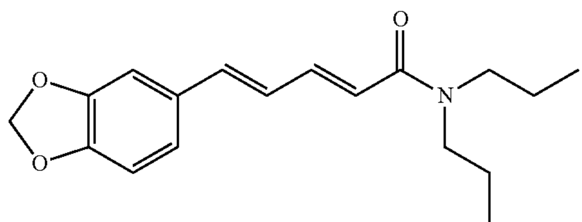
C_{18}H_{23}NO_3 Exact Mass: 301.17 Mol. Wt.: 301.38
