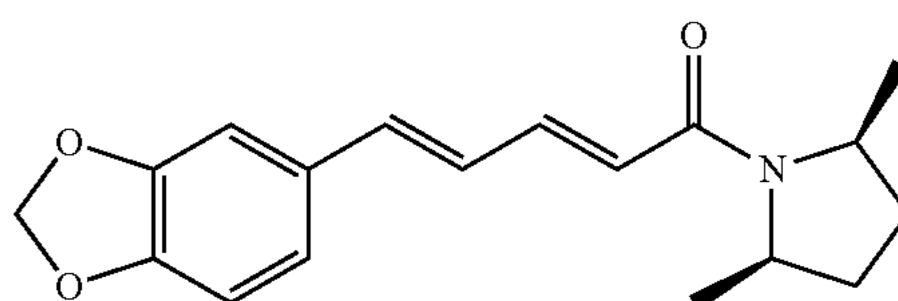
C_{18}H_{21}NO_3 Exact Mass: 299.15 Mol. Wt.: 299.36
