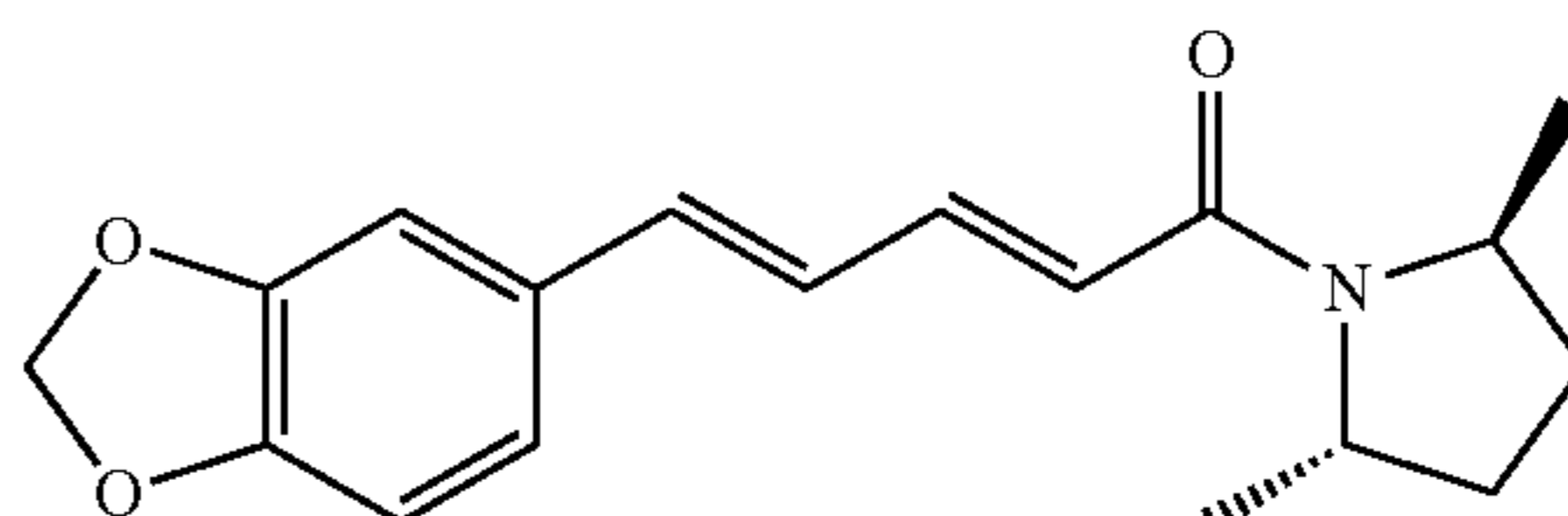
C_{18}H_{21}NO_3 Exact Mass: 299.15 Mol. Wt.: 299.36
