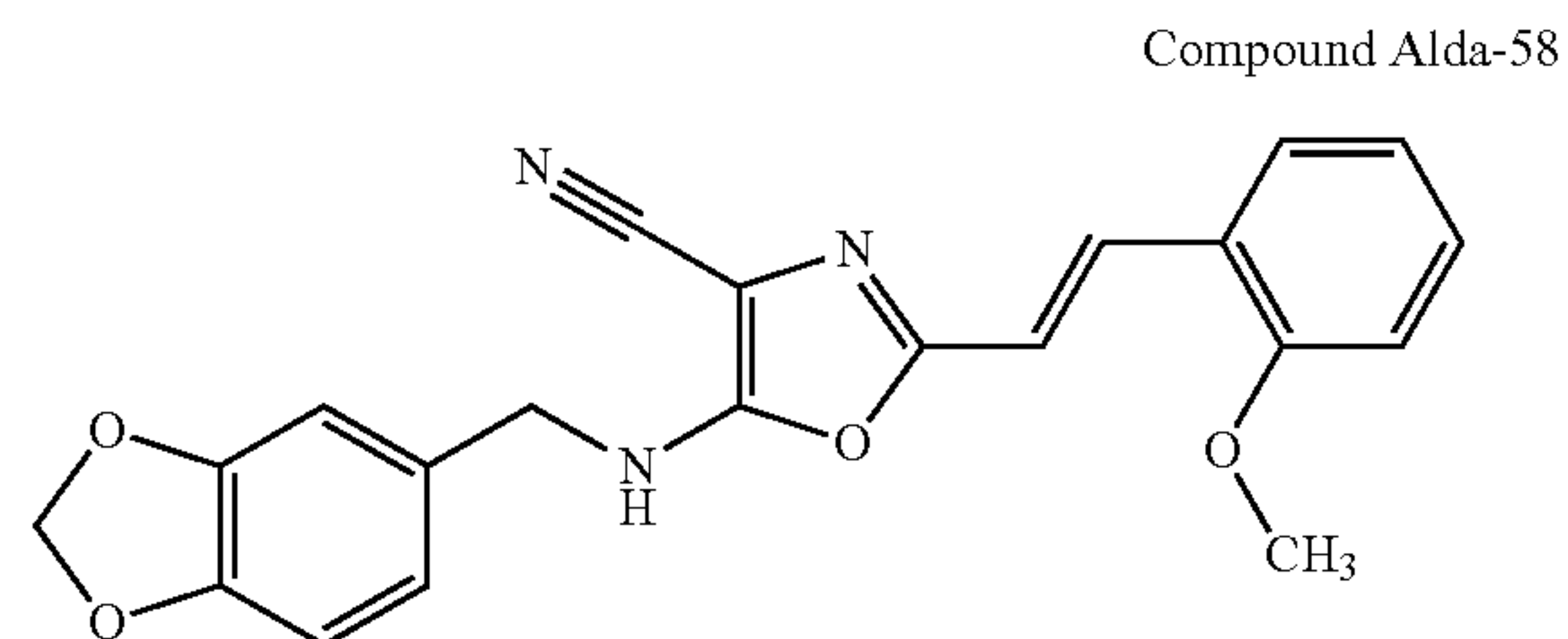
Compound Alda-58: 5-[(benzo[1,3]dioxol-5-ylmethyl)-amino]-2-[2-(2-methoxy-phenyl)-vinyl]-oxazole-4-carbonitrile
