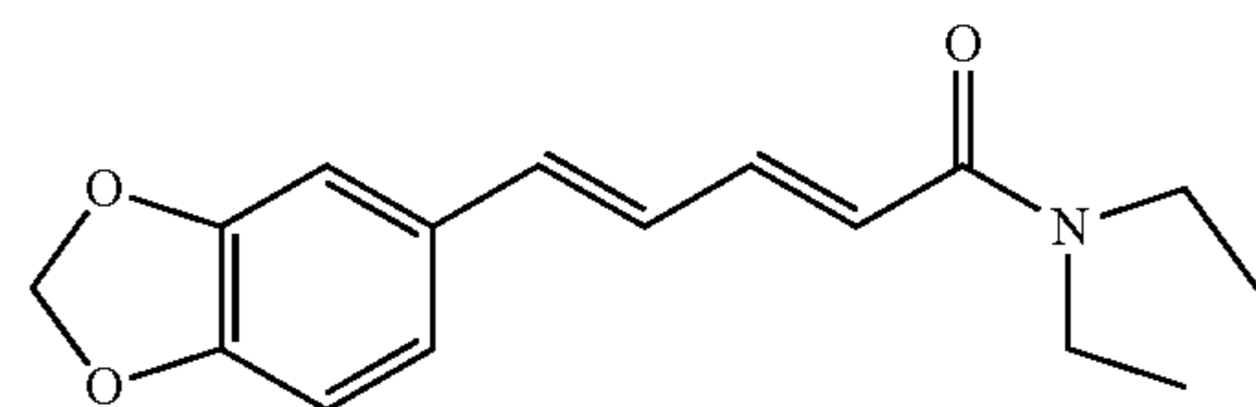
C_{16}H_{19}NO_3 Exact Mass: 273.14 Mol. Wt.: 273.33
