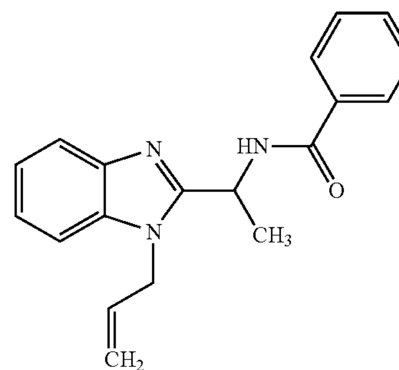
Compound Alda-81: N-[1-(1-allyl-1H-benzimidazol-2-yl)-ethyl]-benzamide
