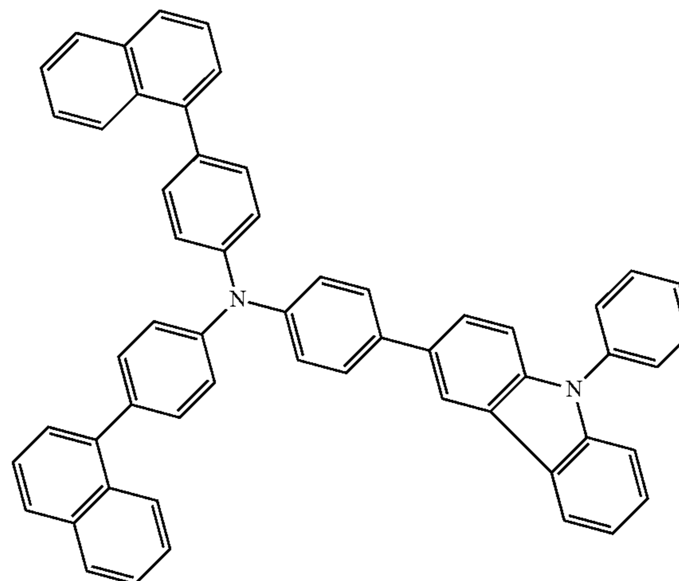
PCBNBB
