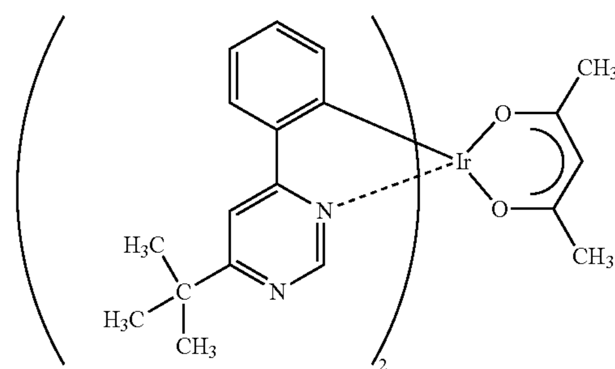
[Ir(tBuppm)_2(acac)]
