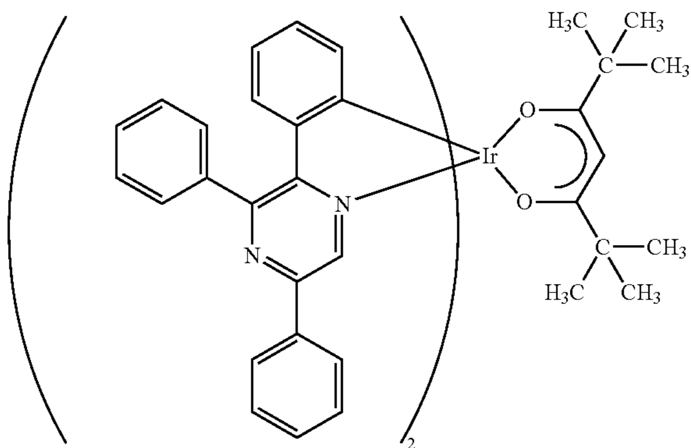
[Ir(tppr) 2 (dpm)]
