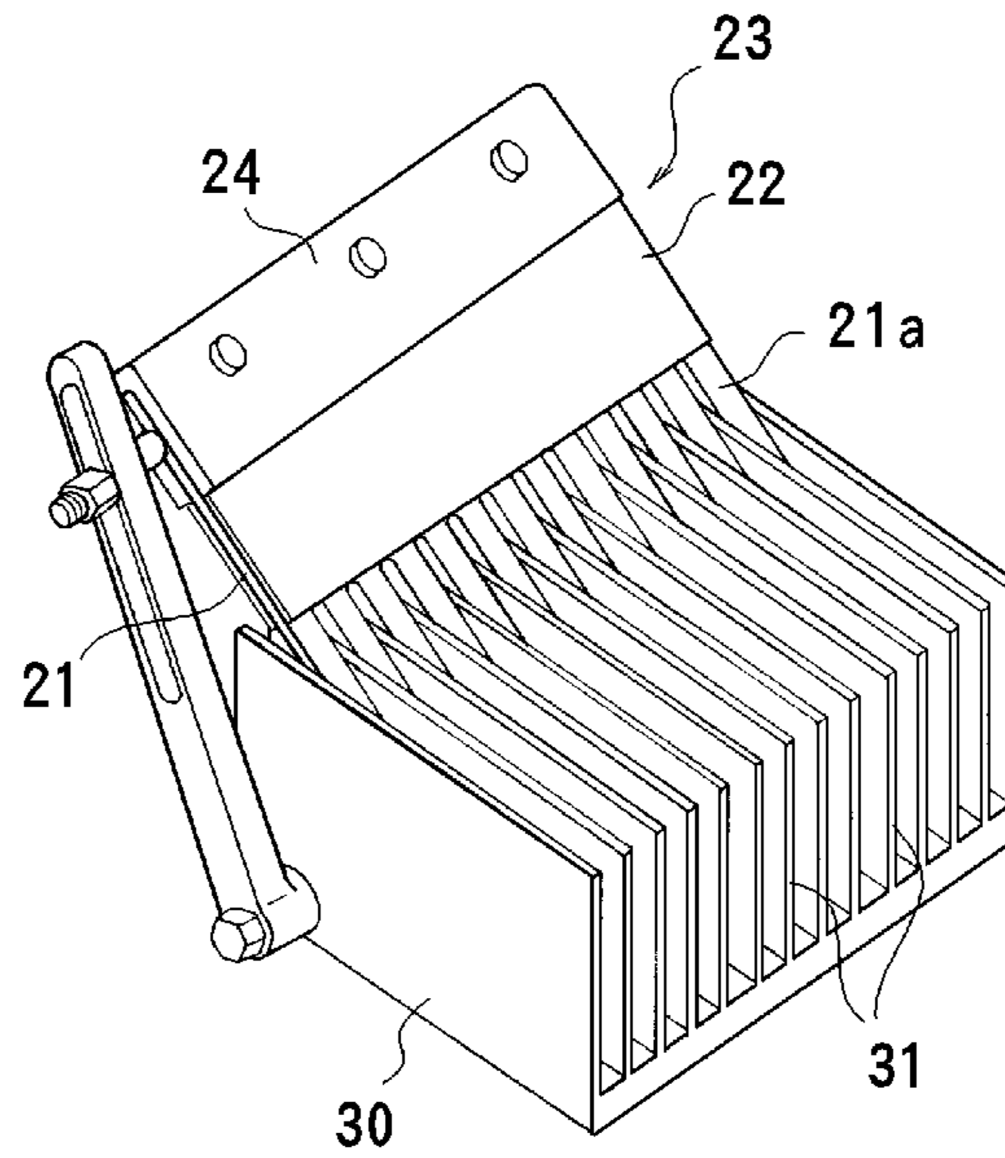
FIG. 5 PRIOR ART
