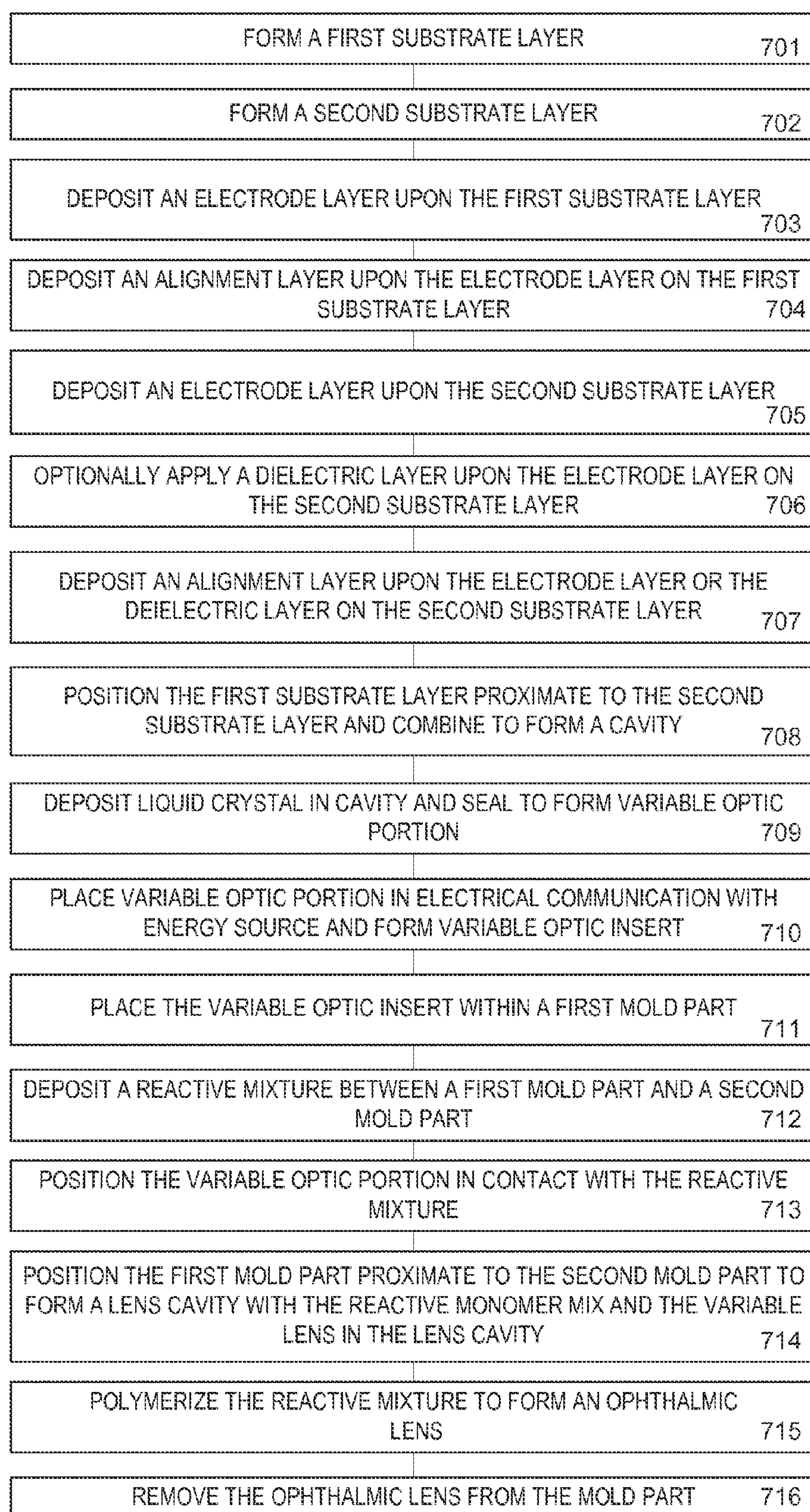
Figure 7
