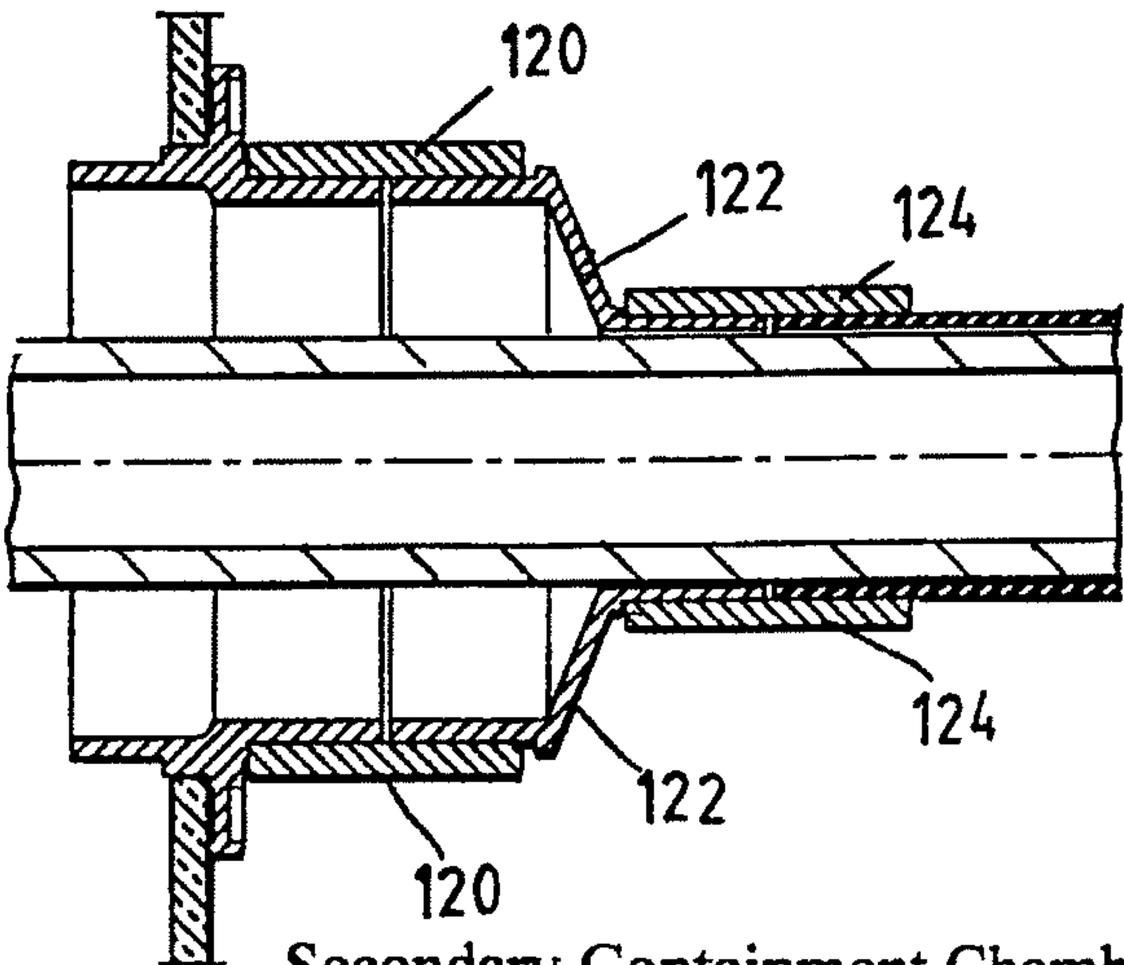
Secondary Containment Chamber Connection of 63/54 Pipe
