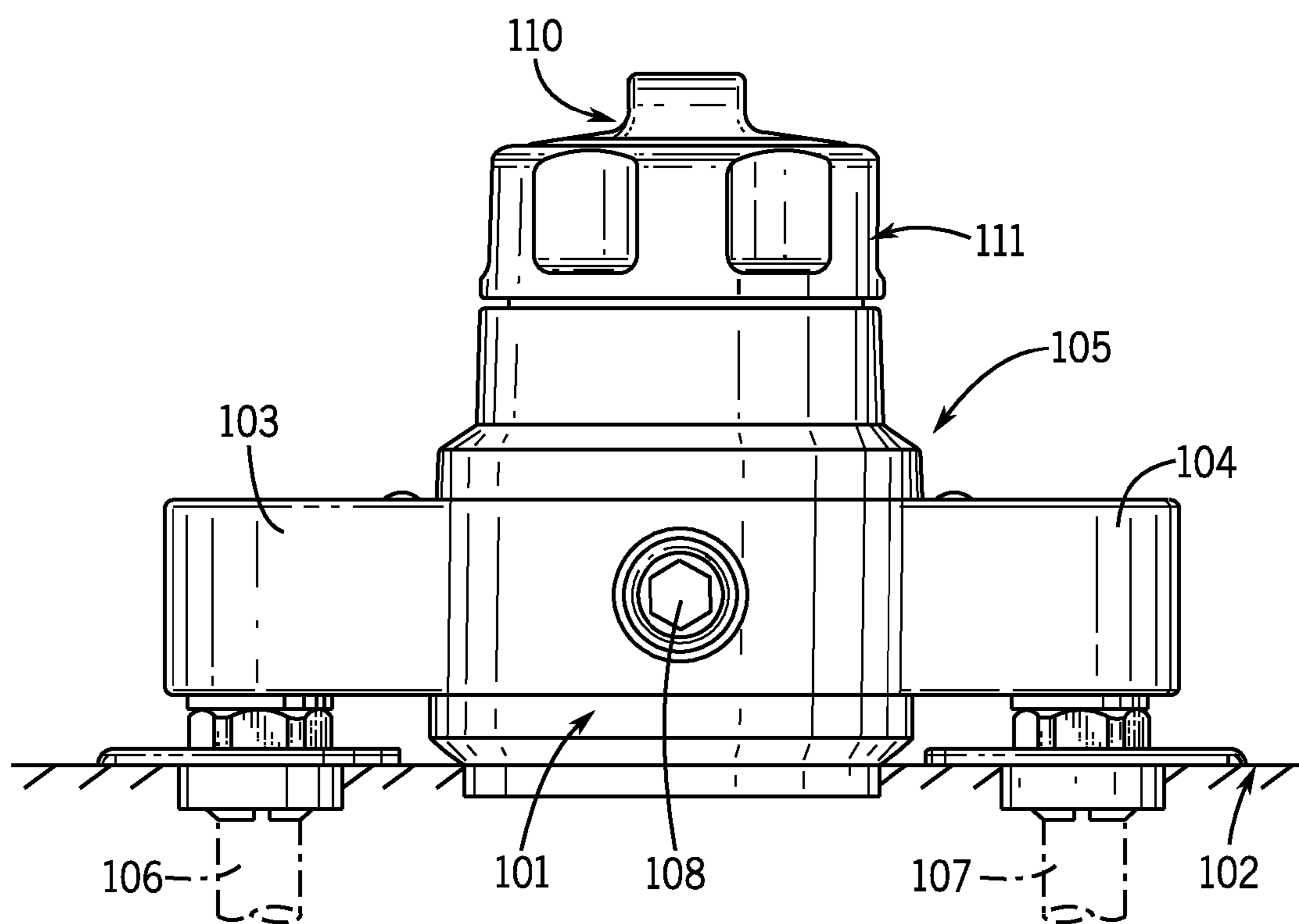
FIG. 13 PRIOR ART
