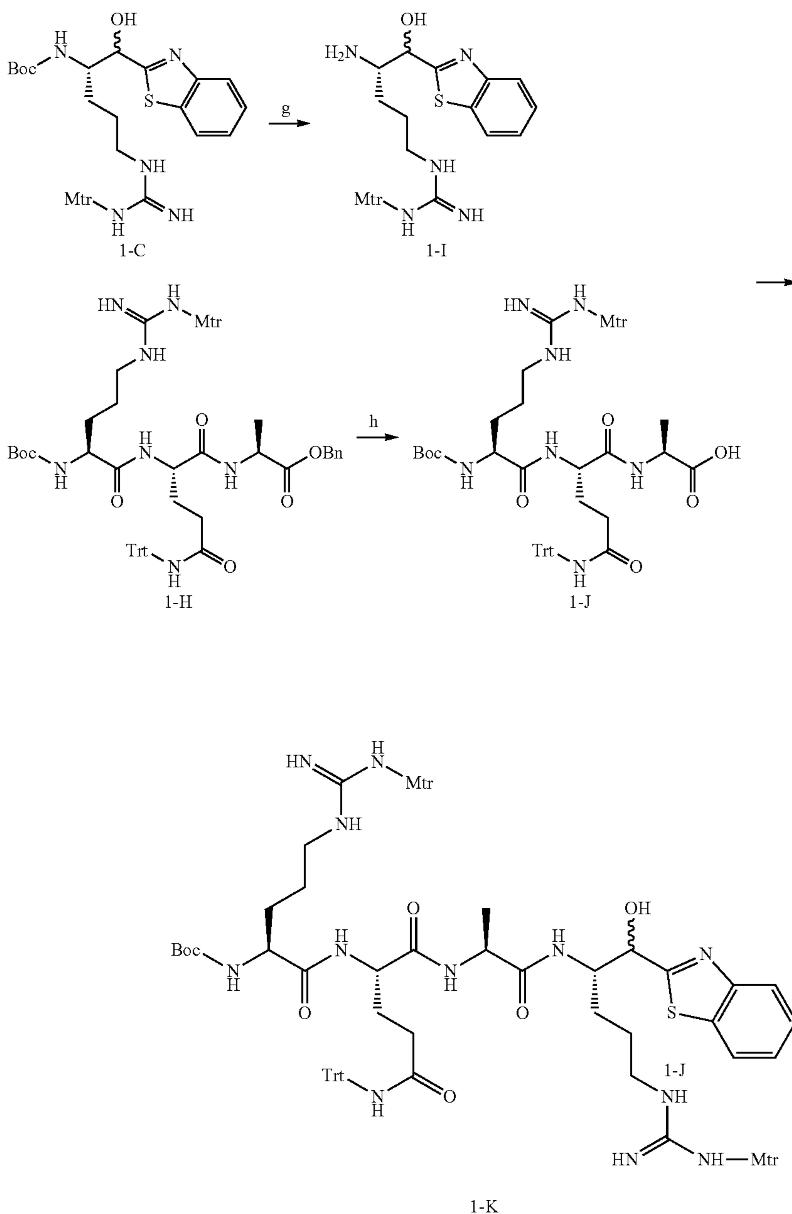
Scheme 3:
