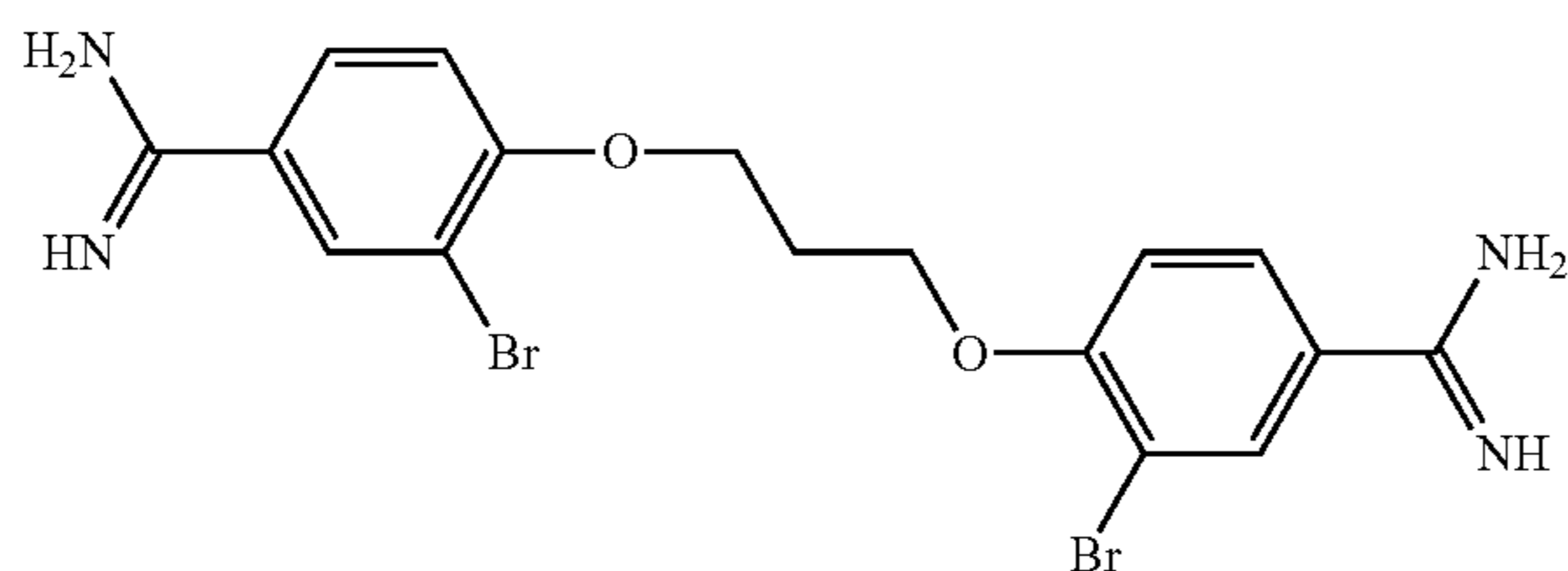
3,3'-dibromo-4,4'-propanediyldioxy-bis-benzamidine
