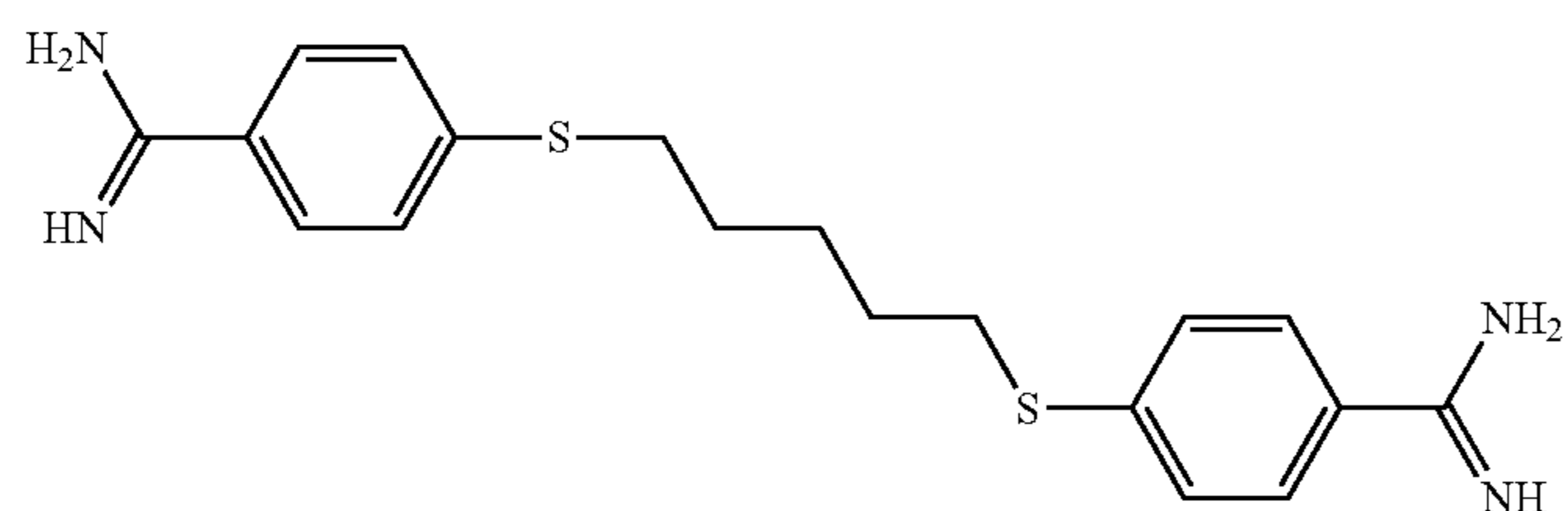
1,5-Bis-(4-amidion-phenylmercapto)-pentane
