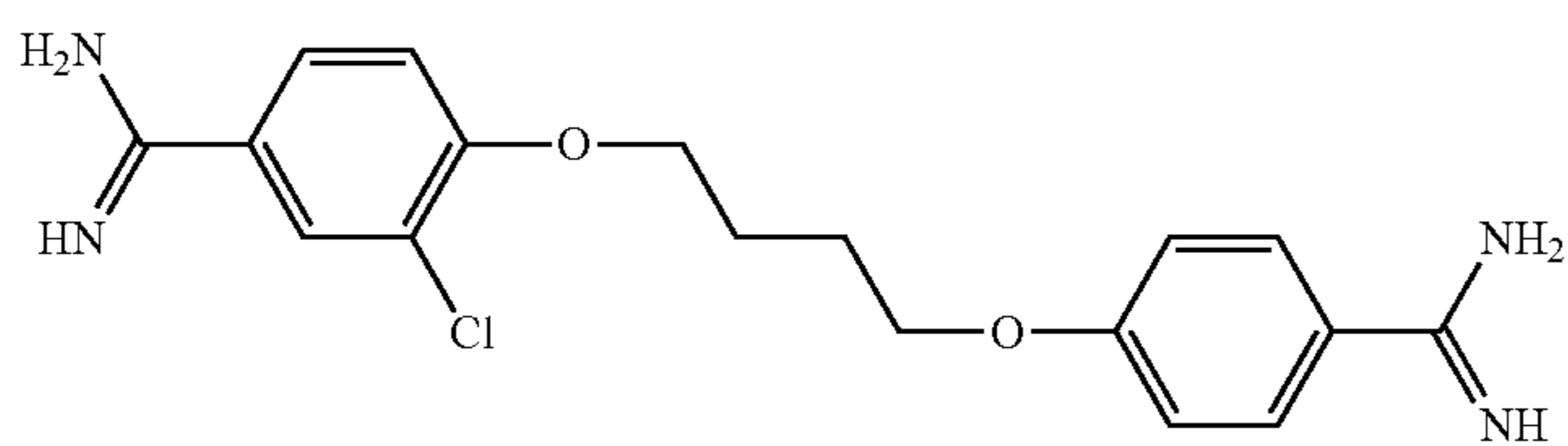
3-chloro-4,4'-butanediyldioxy-bis-benzamidine
