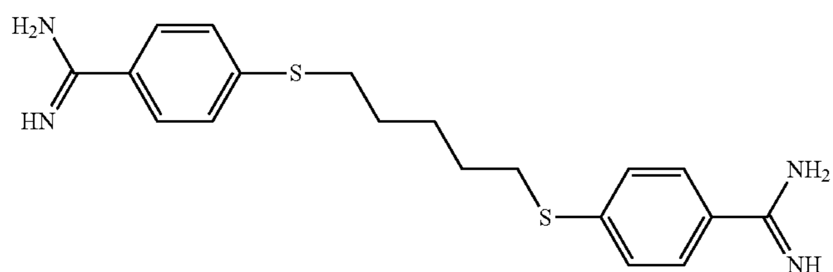
1,5-Bis-(4-amidion-phenylmercapto)-pentane
