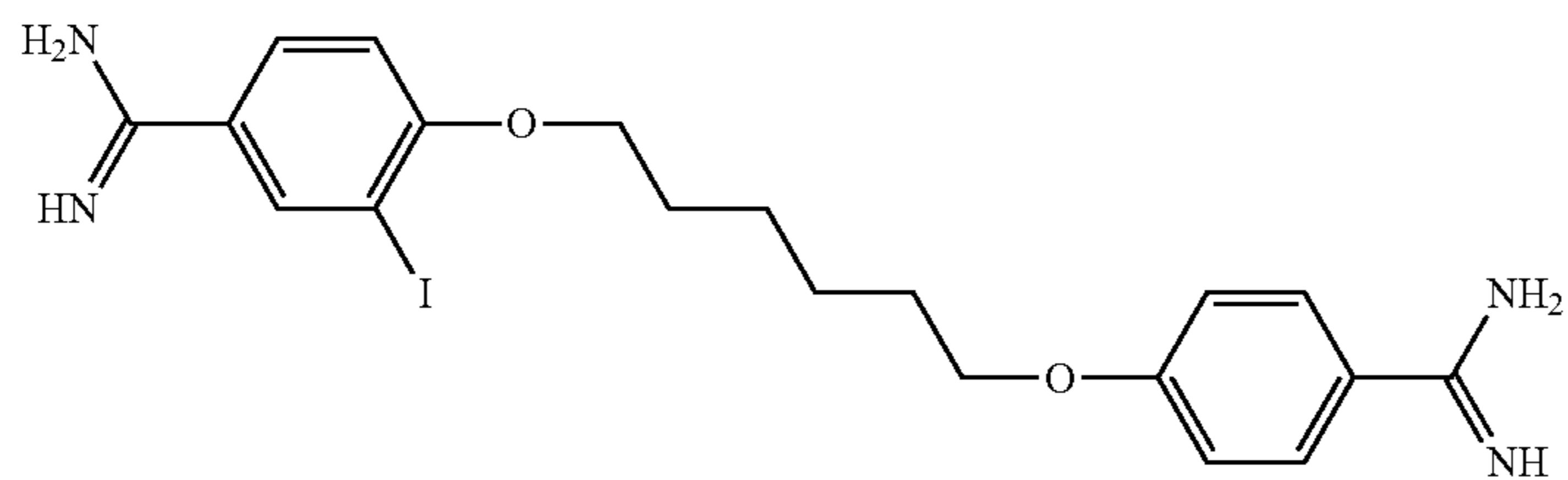
3-iodo-4,4'-hexanediyldioxy-bis-benzamidine
