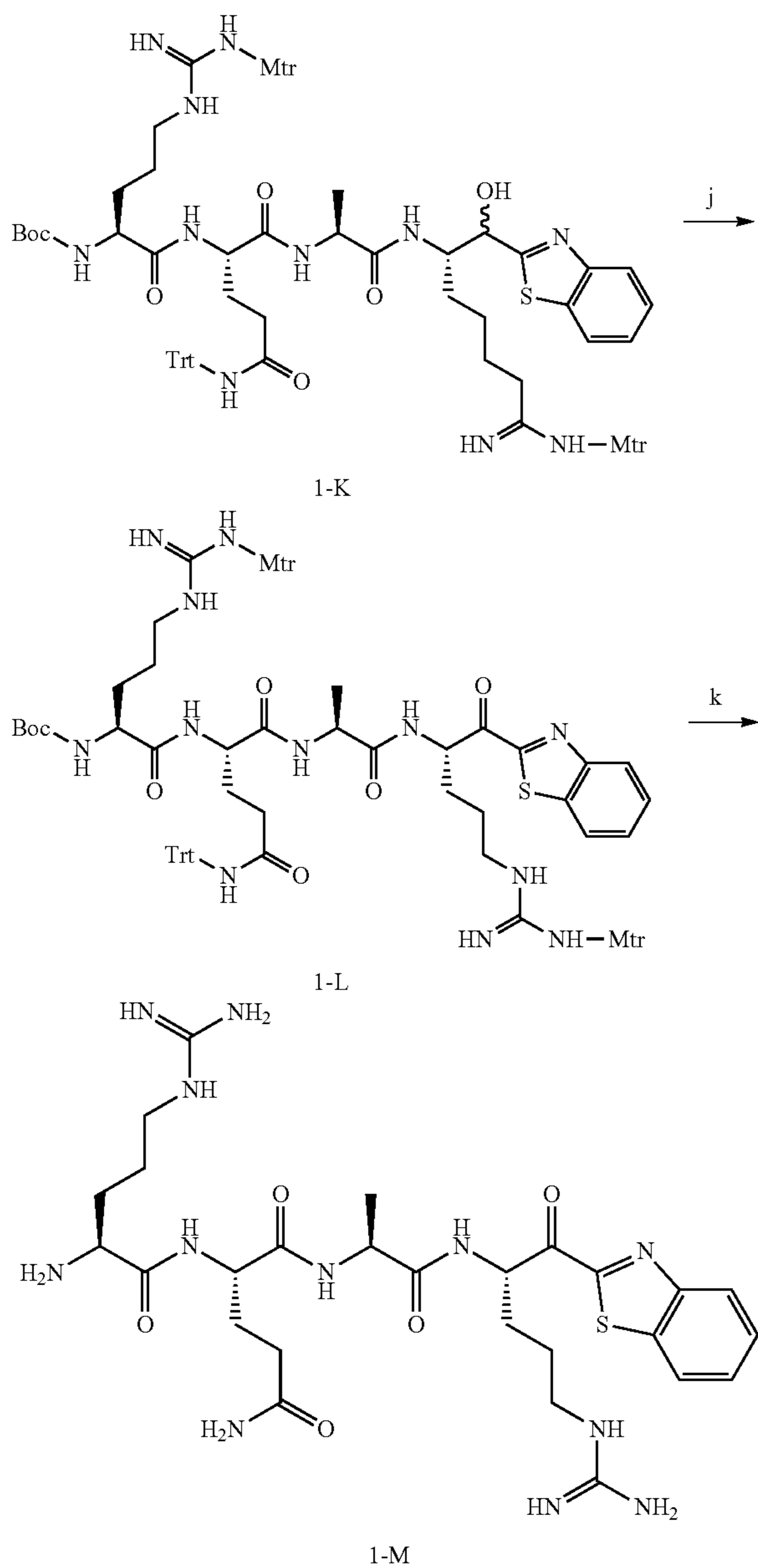
Scheme 4
