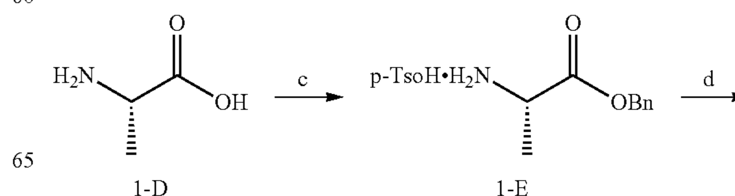
Scheme 2
