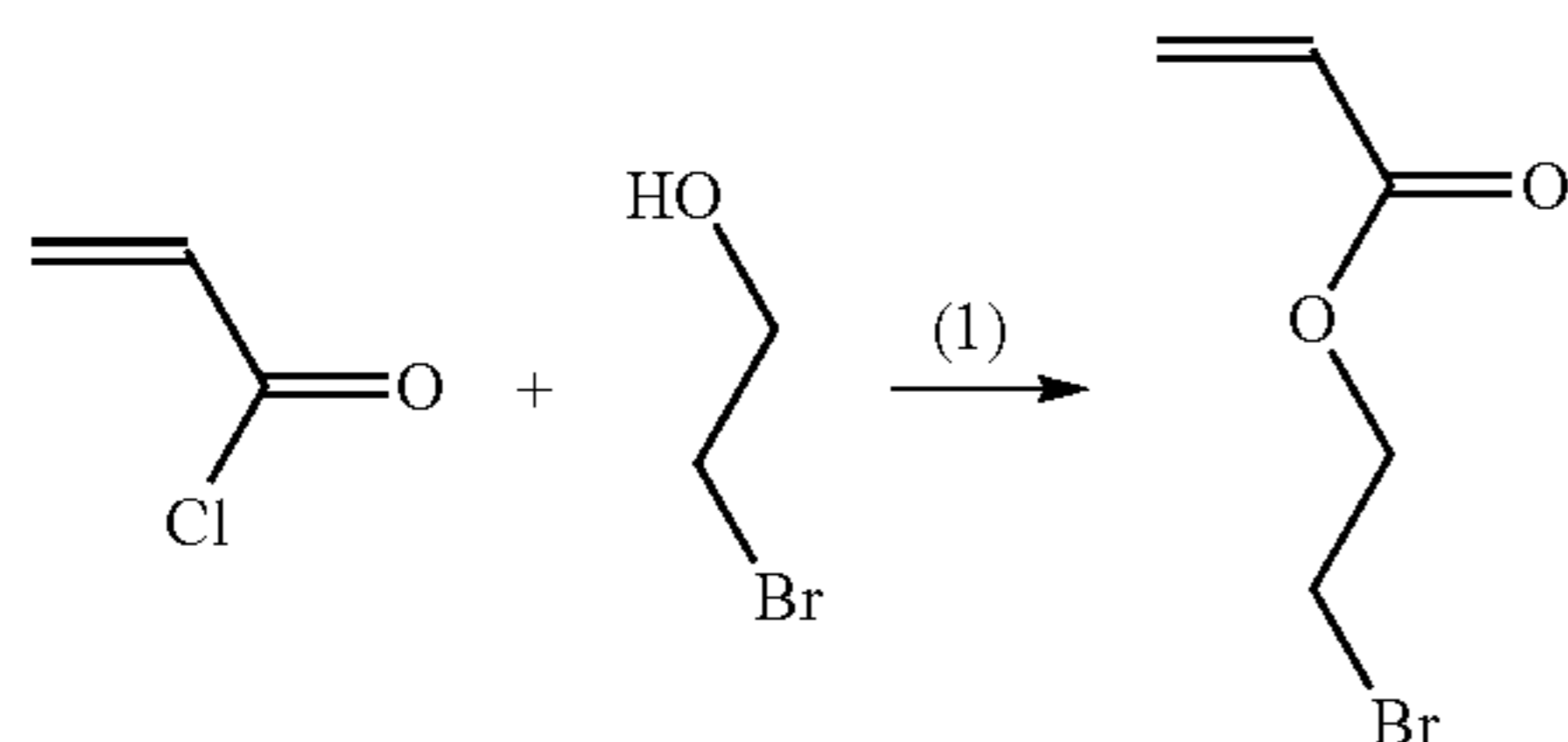
Scheme 6. Synthesis of 2-bromoethyl acrylate (BrEA) monomer
