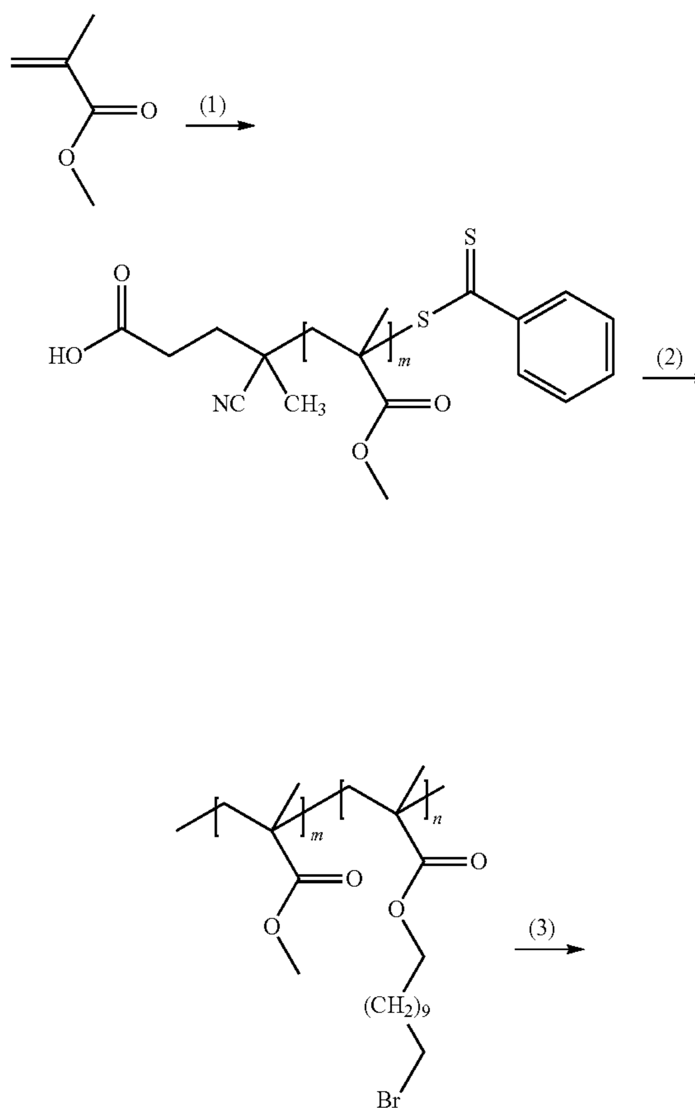
Scheme 3. Synthesis of poly(MMA-b-MUBIm-OH) block copolymers
