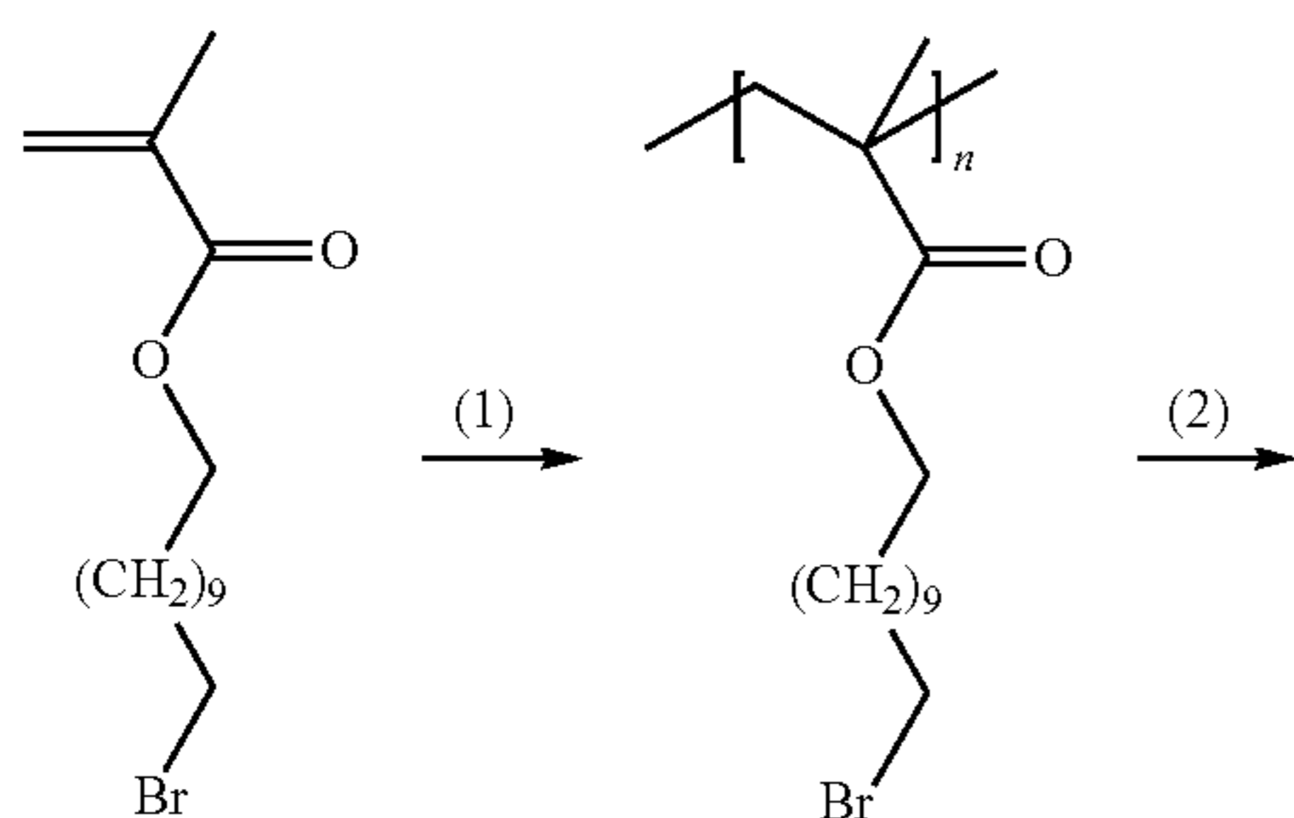
Scheme 4. Synthesis of poly(MUBIm-OH) homopolymer
