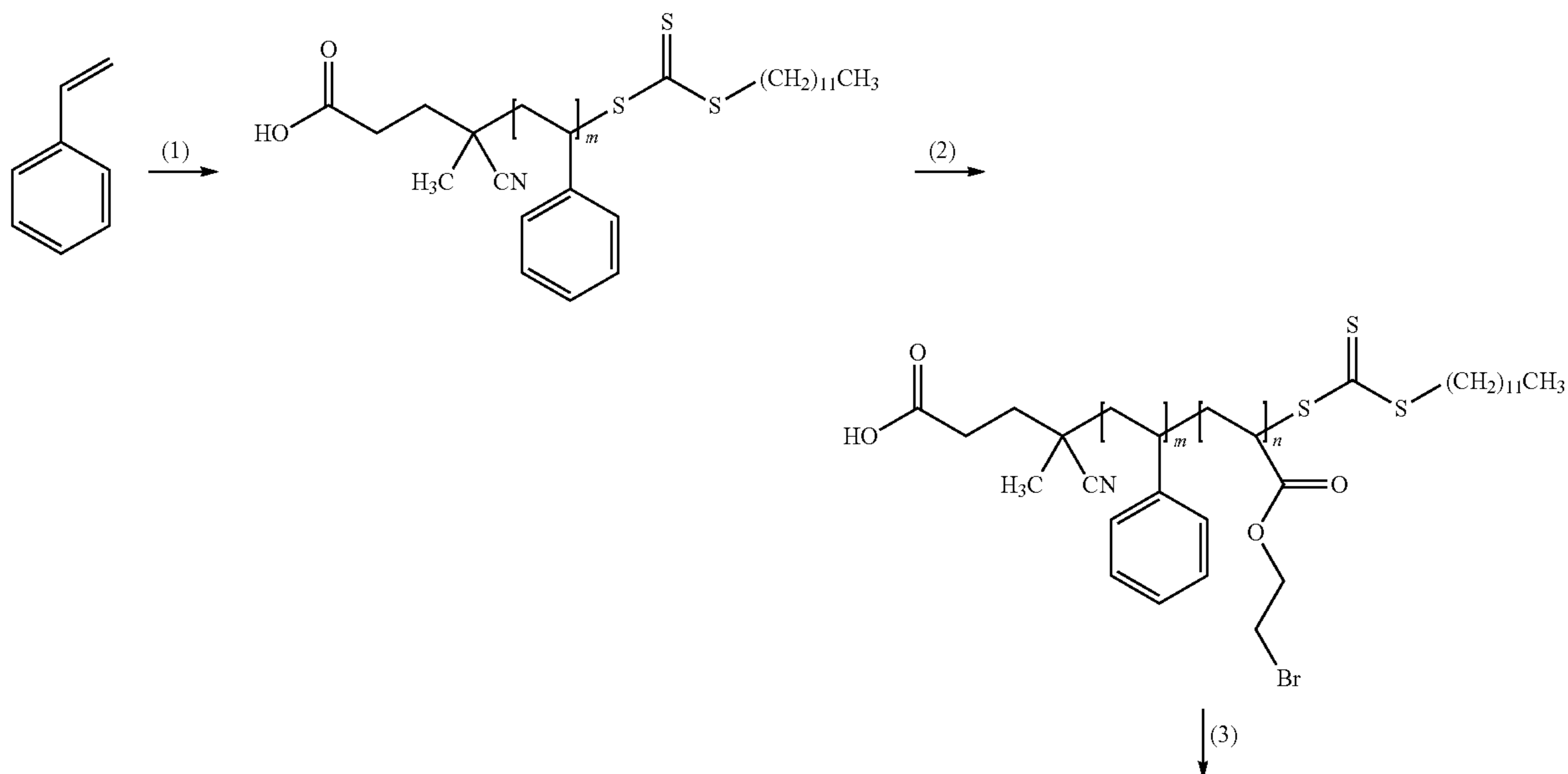
Scheme 5. Synthesis of poly(S-b-AEBIm-TFSI) block copolymers.
