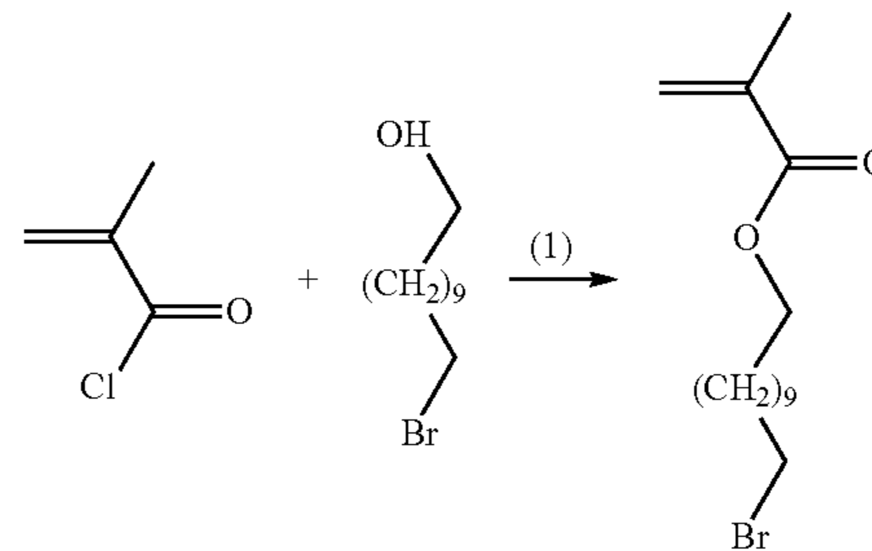
Scheme 2. Synthesis of 11-Bromoundecyl methacrylate (BrUMA) monomer
