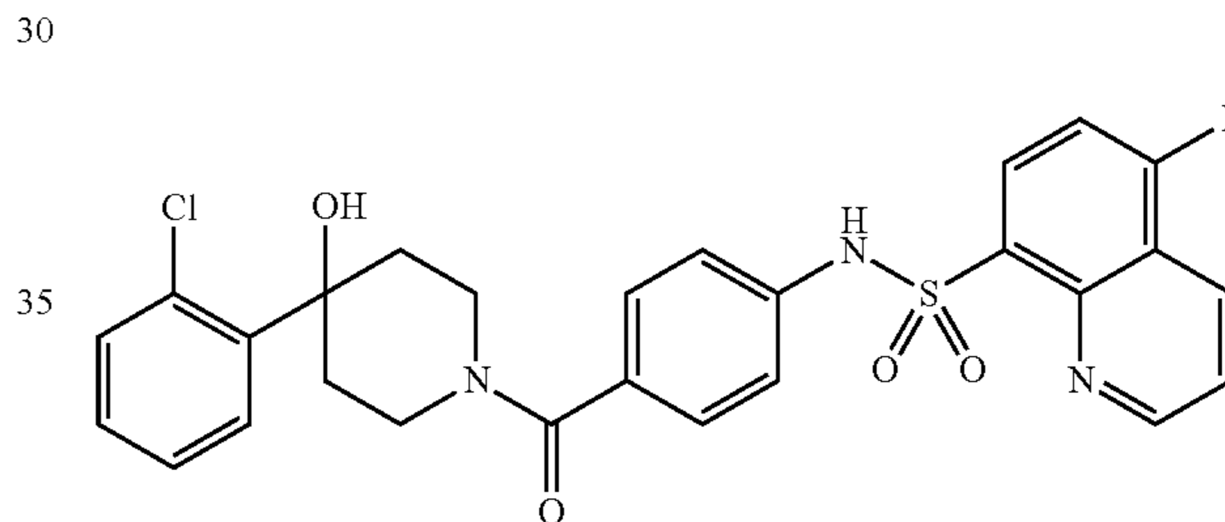
N-(4-(4-(2-chlorophenyl)-4-hydroxypiperidine-1-carbonyl)phenyl)-5-fluoroquinoline-8-sulfonamide
