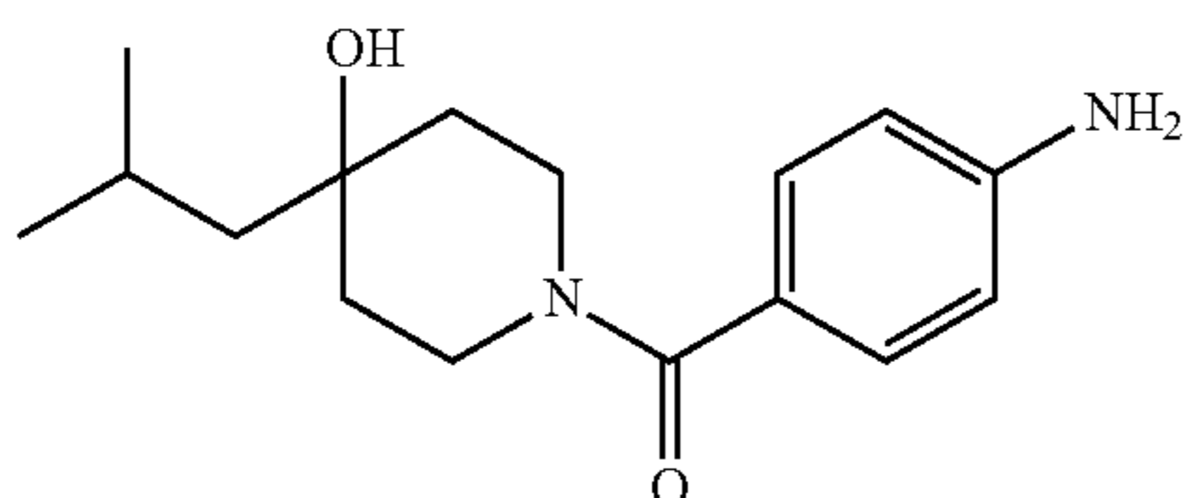
1C: (4-aminophenyl)(4-hydroxy-4-isobutylpiperidin-1-yl)methanone
