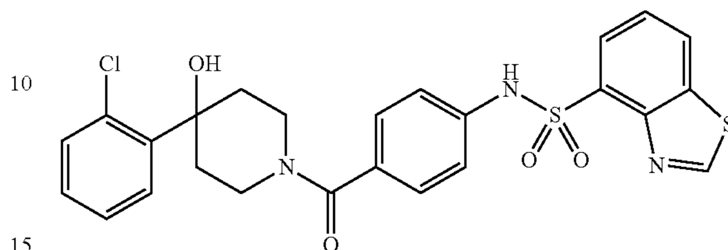
1C: (4-aminophenyl)(4-hydroxy-4-isobutylpiperidin-1-yl)methanone
